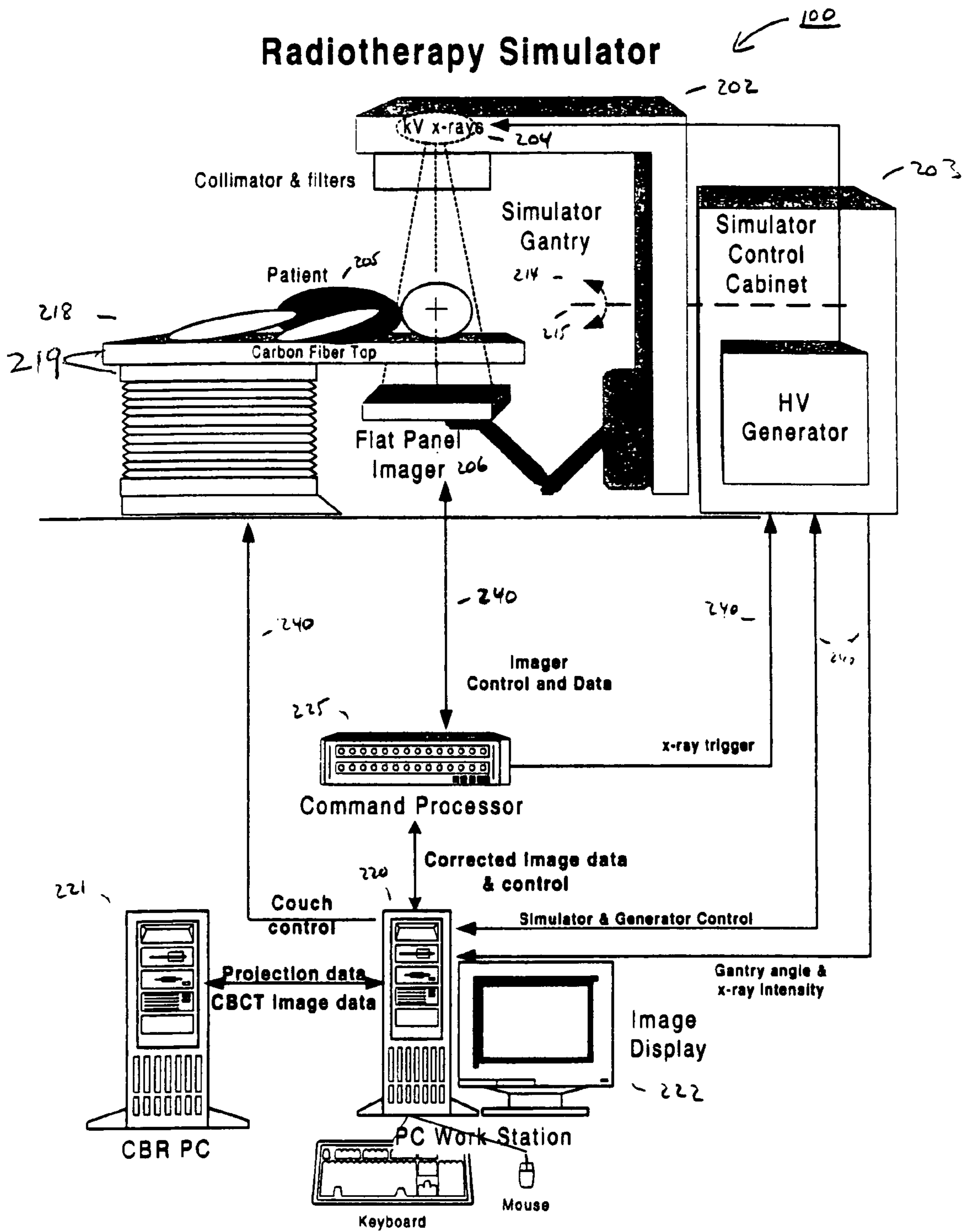
Figure 1- Simulator kV Cone Beam CT Diagram
