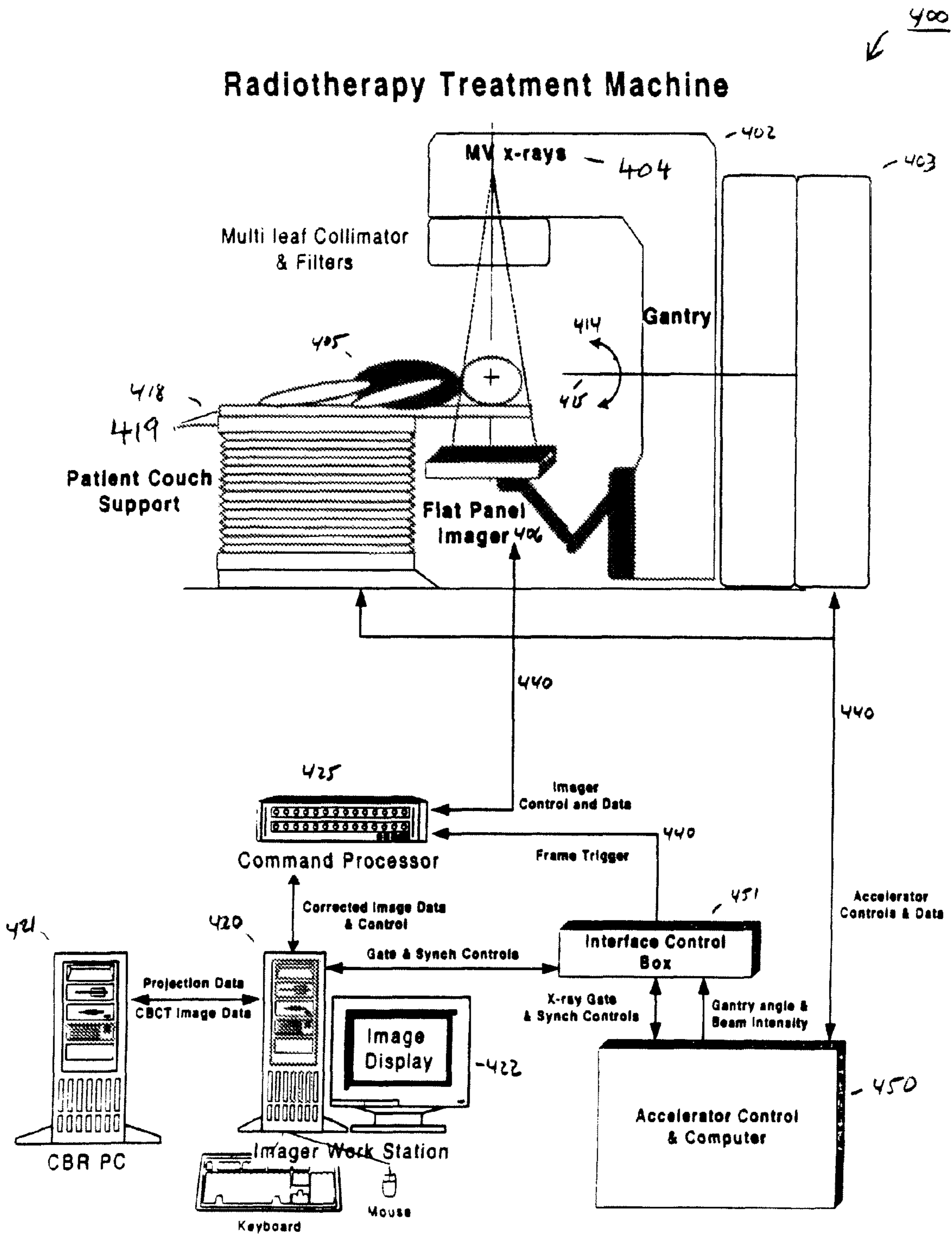
Figure 3- MV Cone Beam CT Diagram
