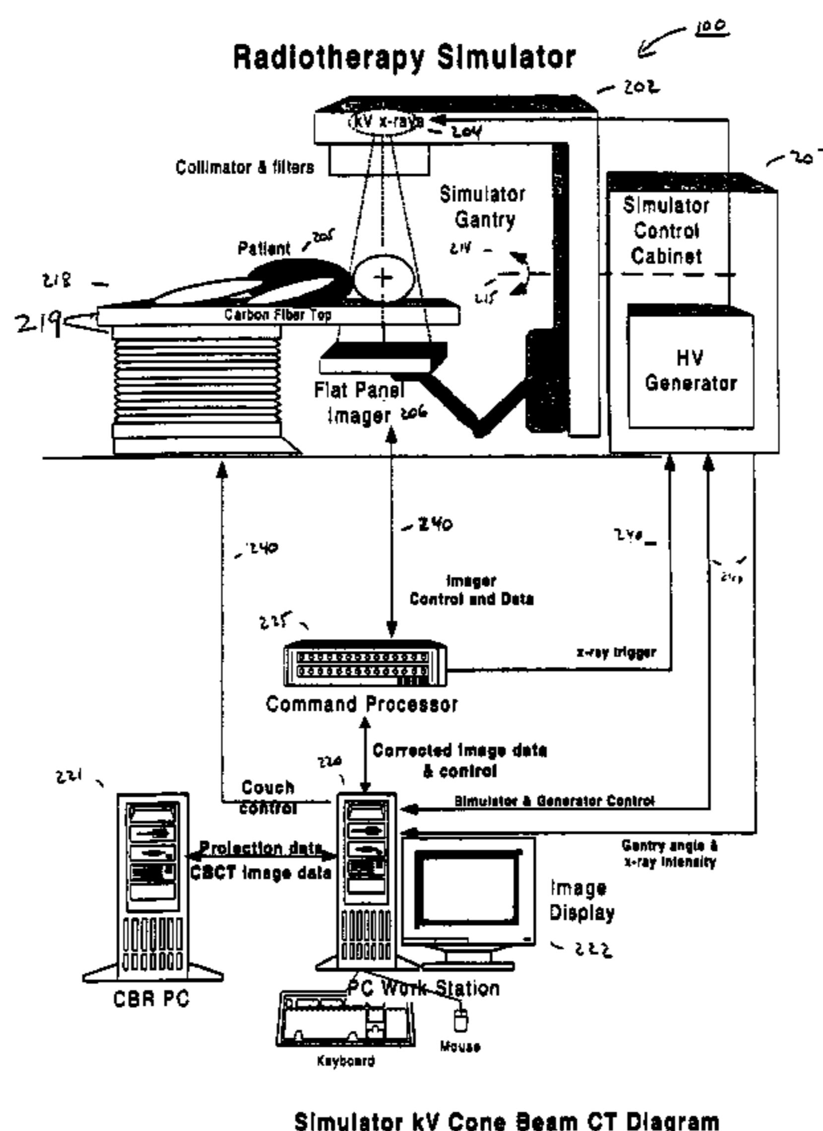
Simulator kV Cone Beam CT Diagram
