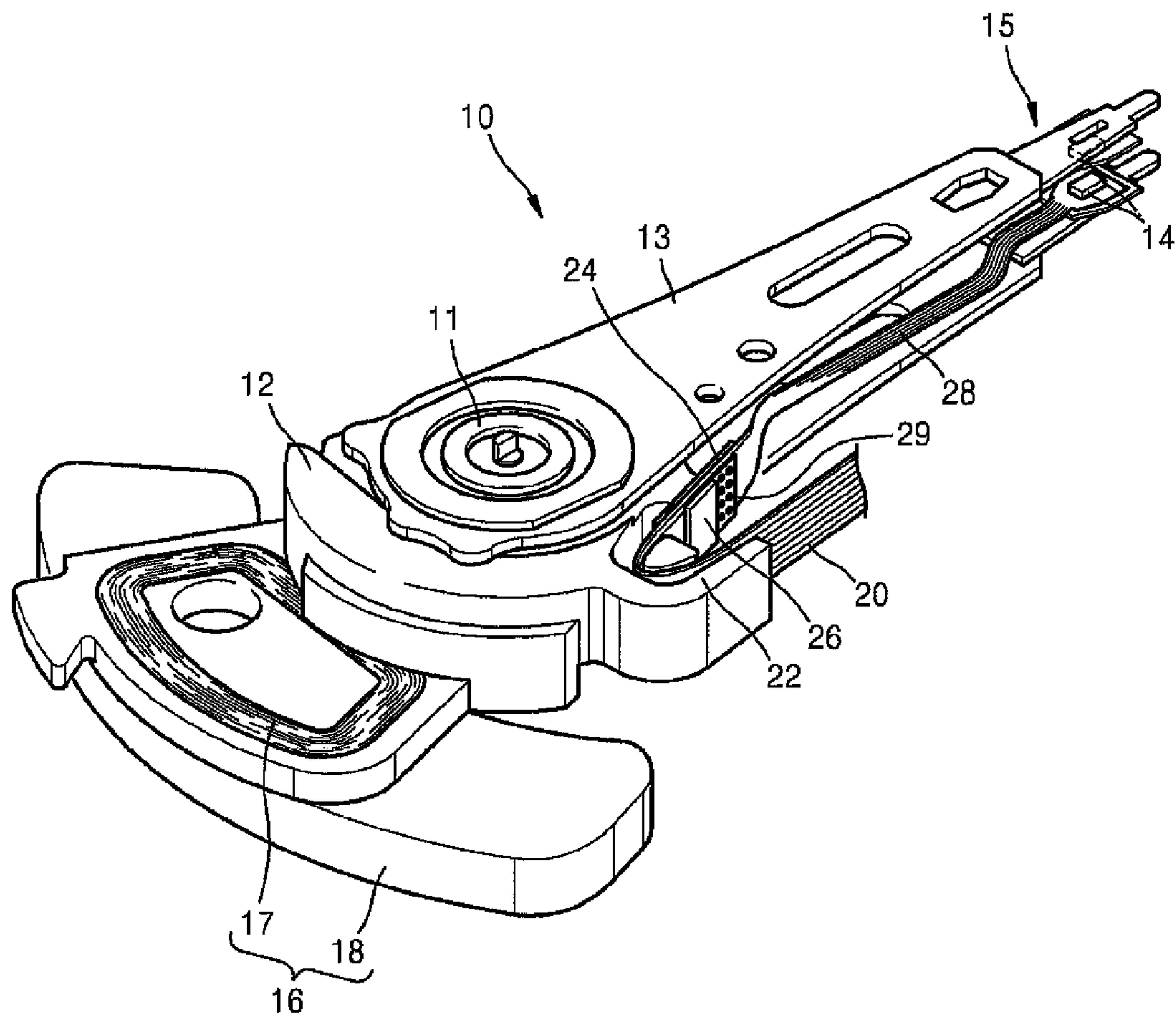
FIG. 2 (PRIOR ART)
