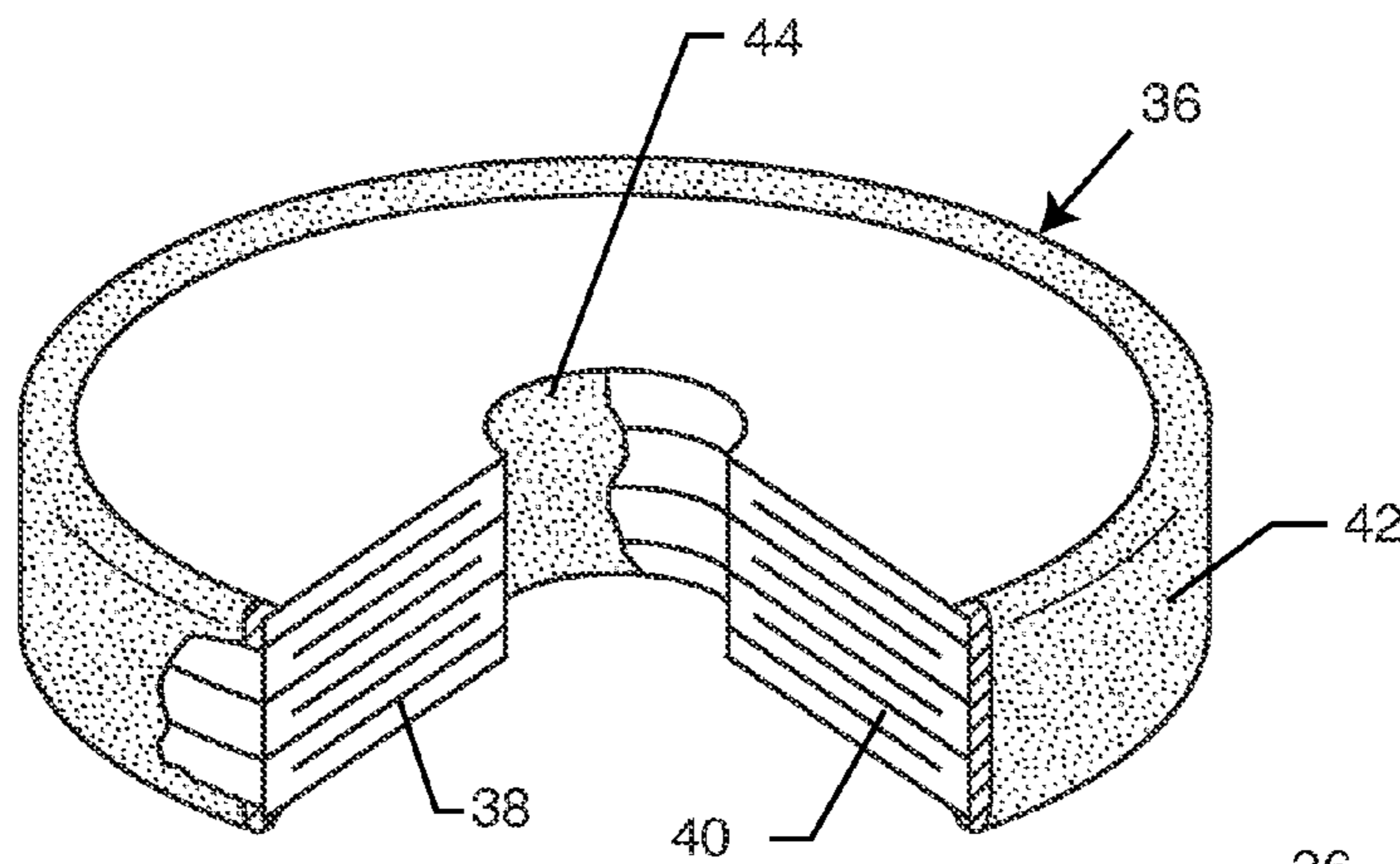
FIG. 3 PRIOR ART
