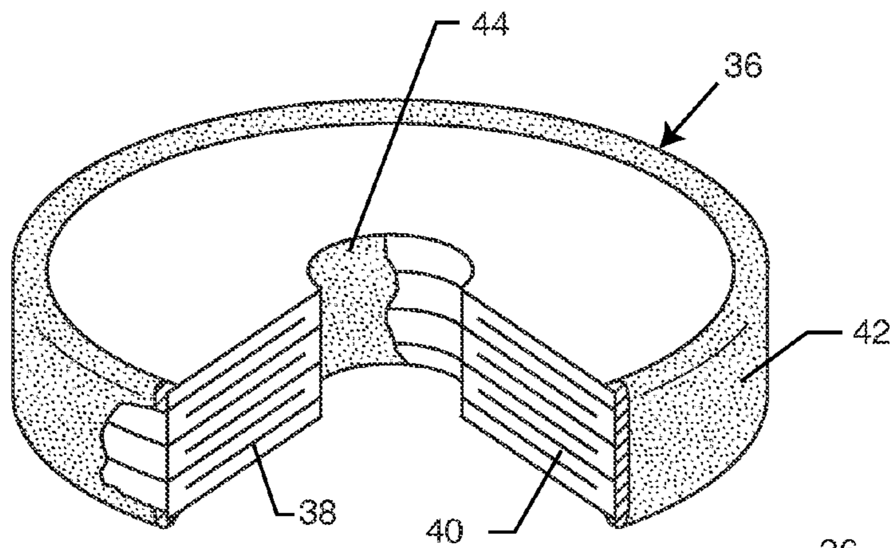
FIG. 3 PRIOR ART
