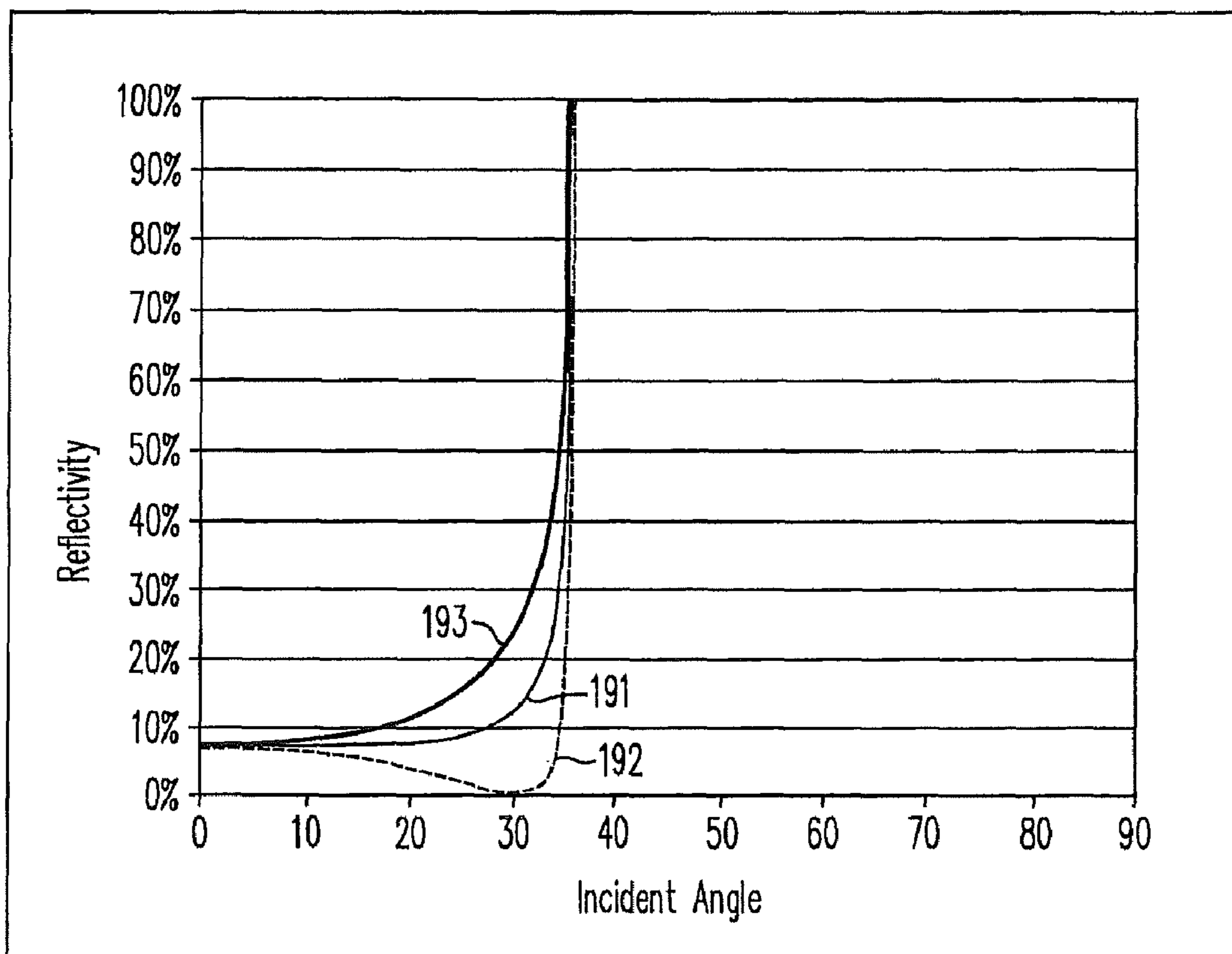
FIG. 11B (Prior Art)
