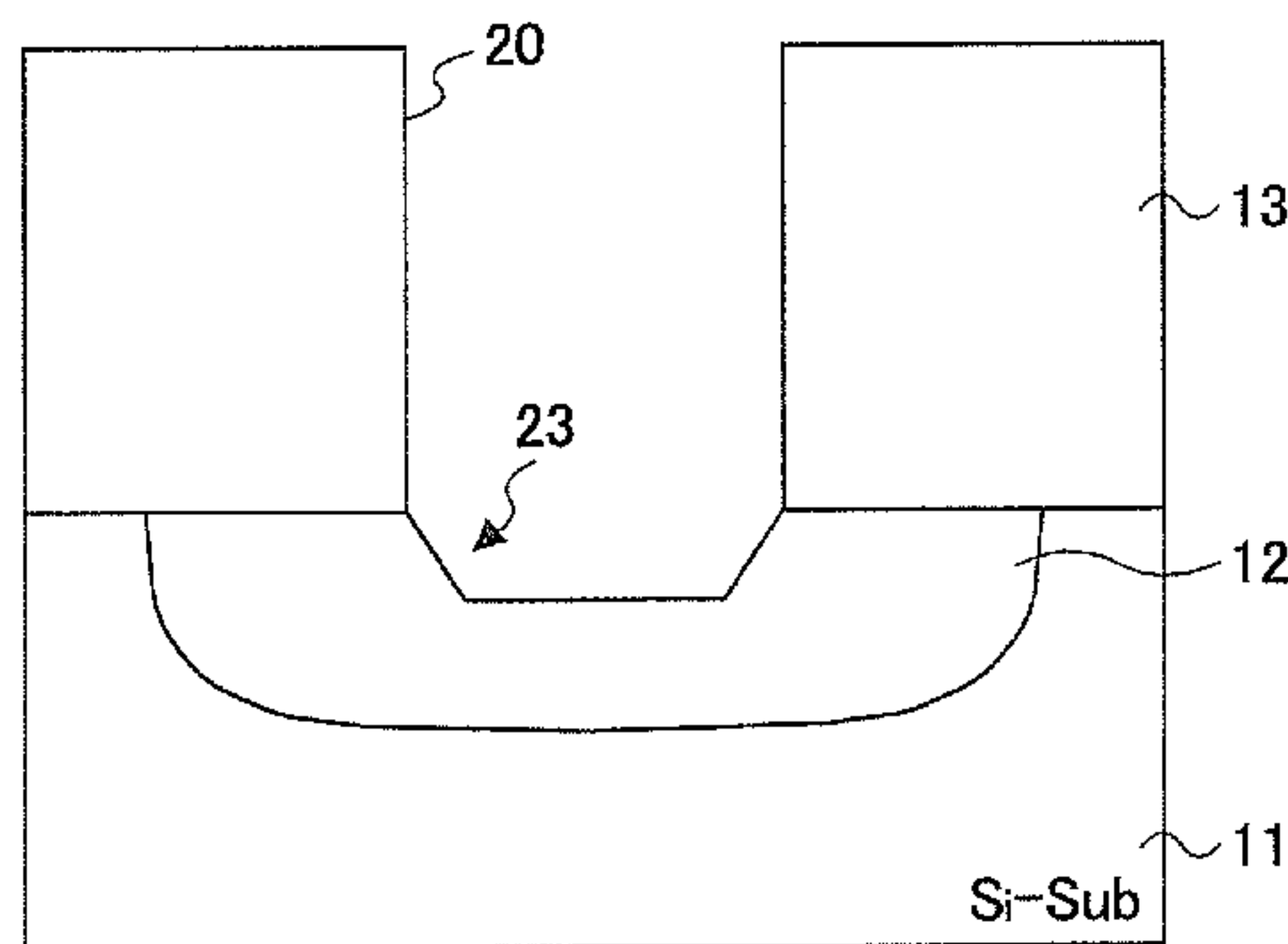
REMOVE DAMAGED SILICON BY THERMALLY DECOMPOSED ATOMIC HYDROGEN
