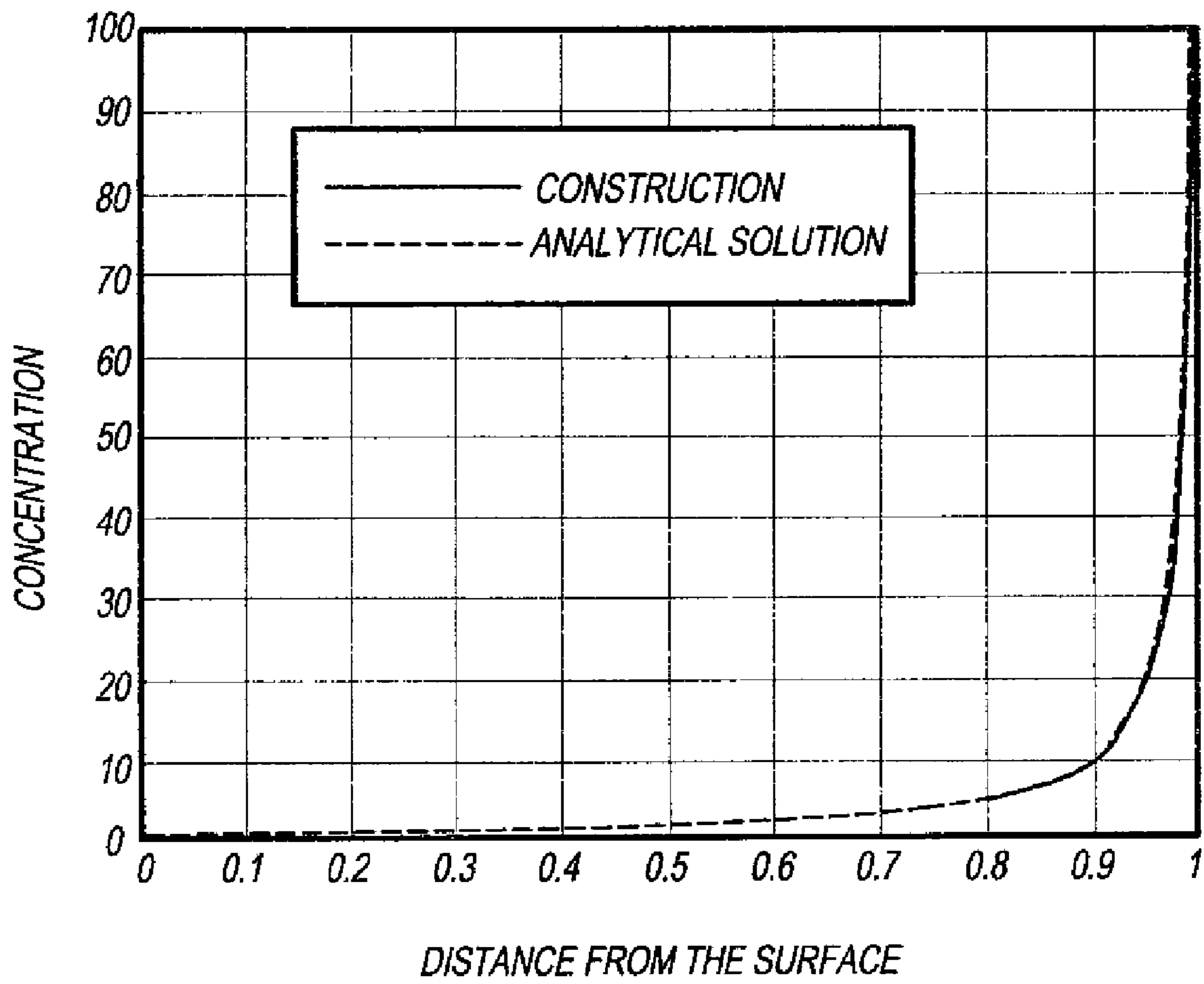
CONSTRUCTION OF IDEAL CONCENTRATION, dx=0.001
