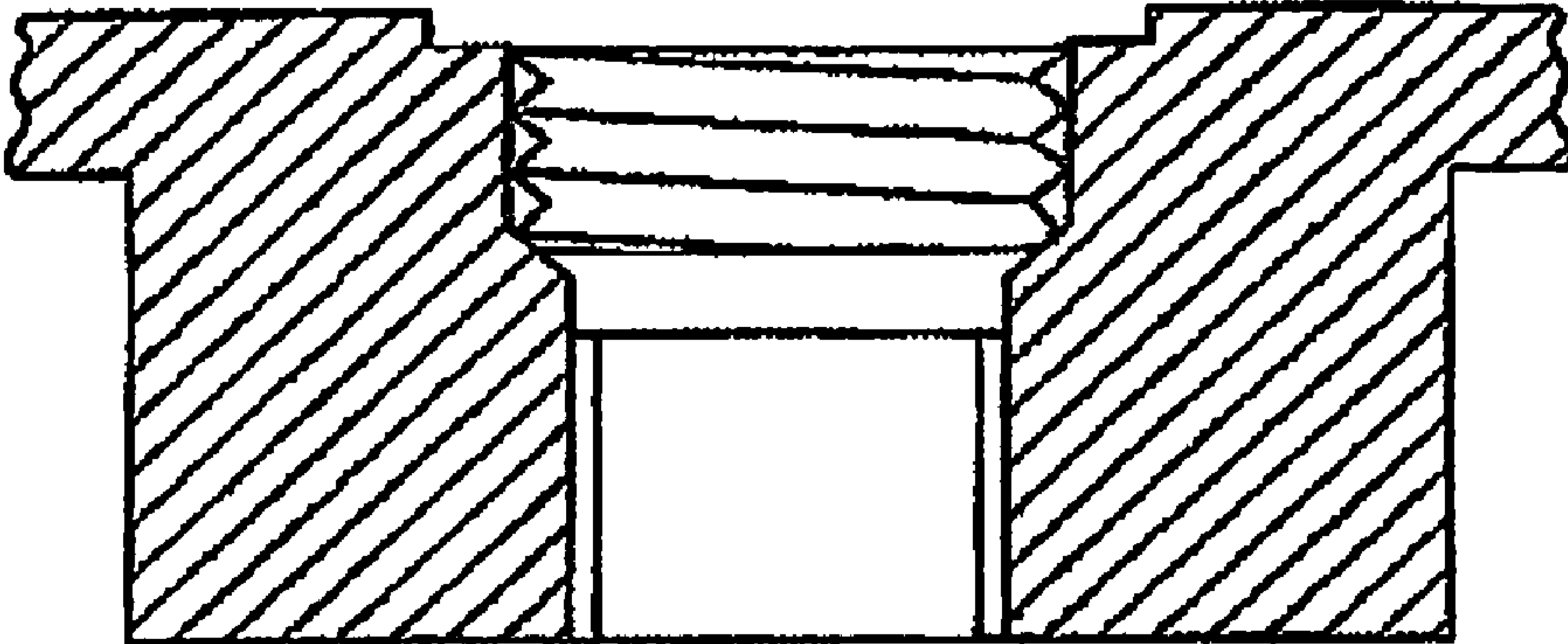
FIG. 5 PRIOR ART
