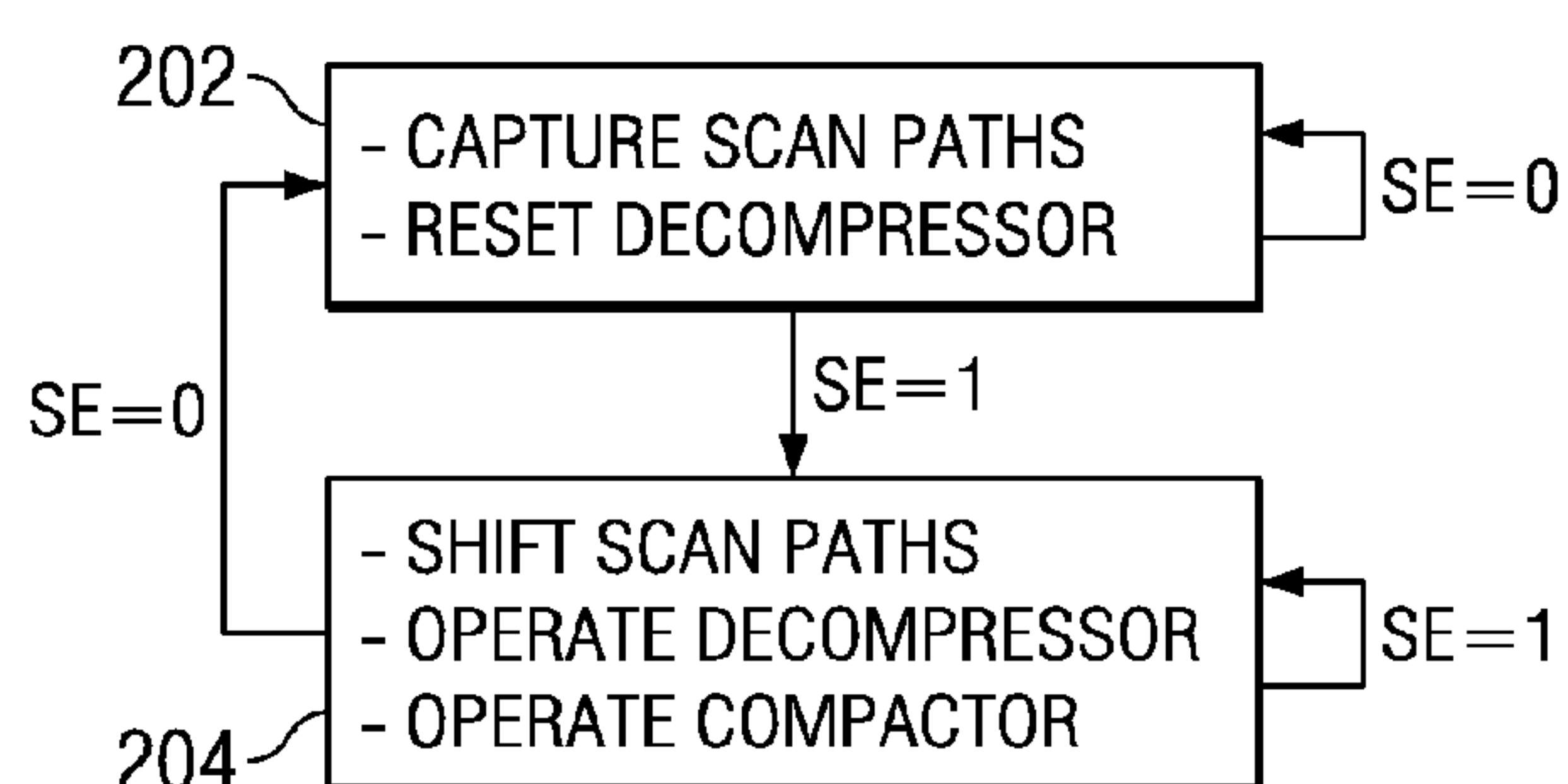
FIG. 2 (PRIOR ART)
