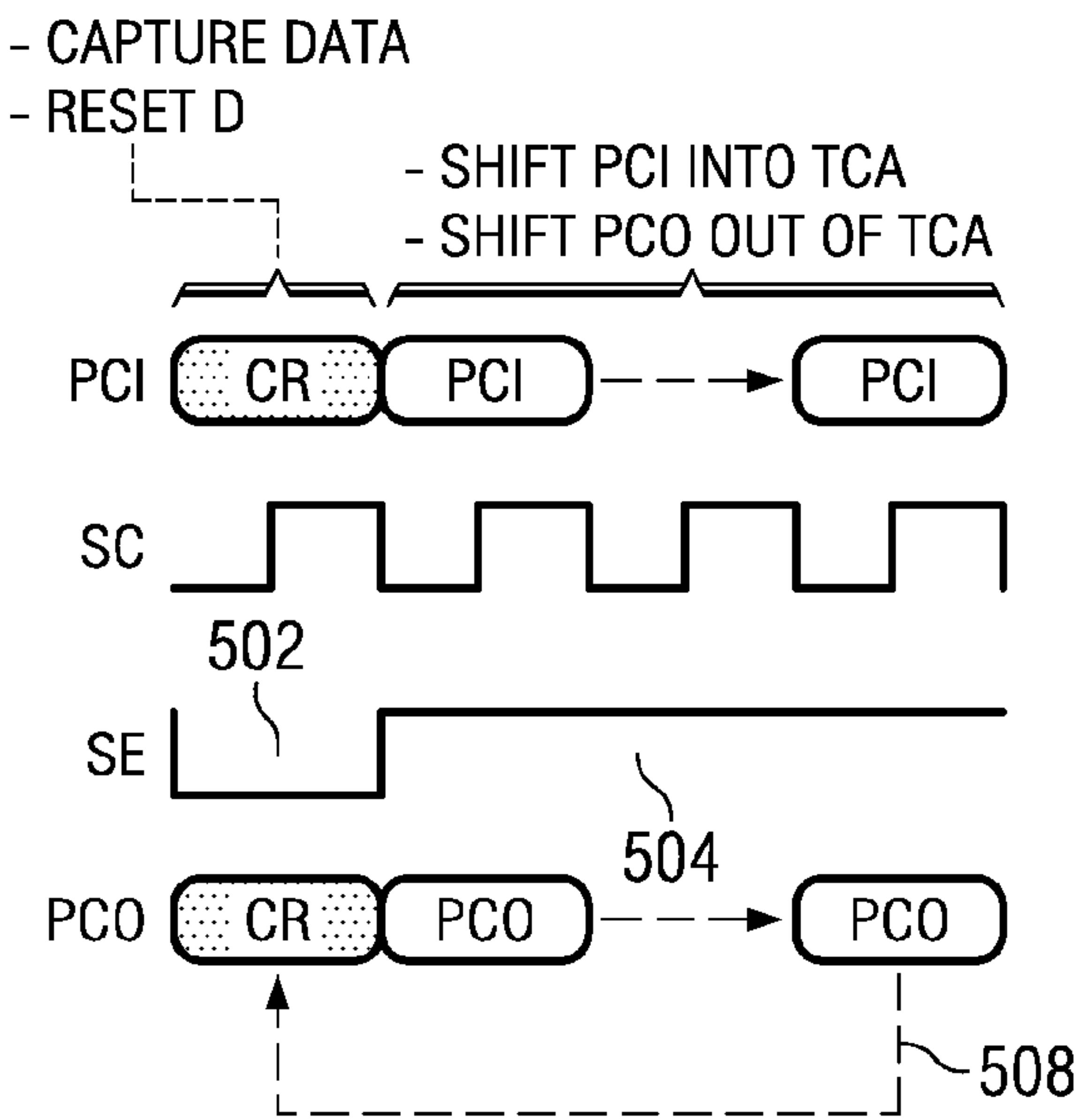
FIG. 5 (PRIOR ART)
