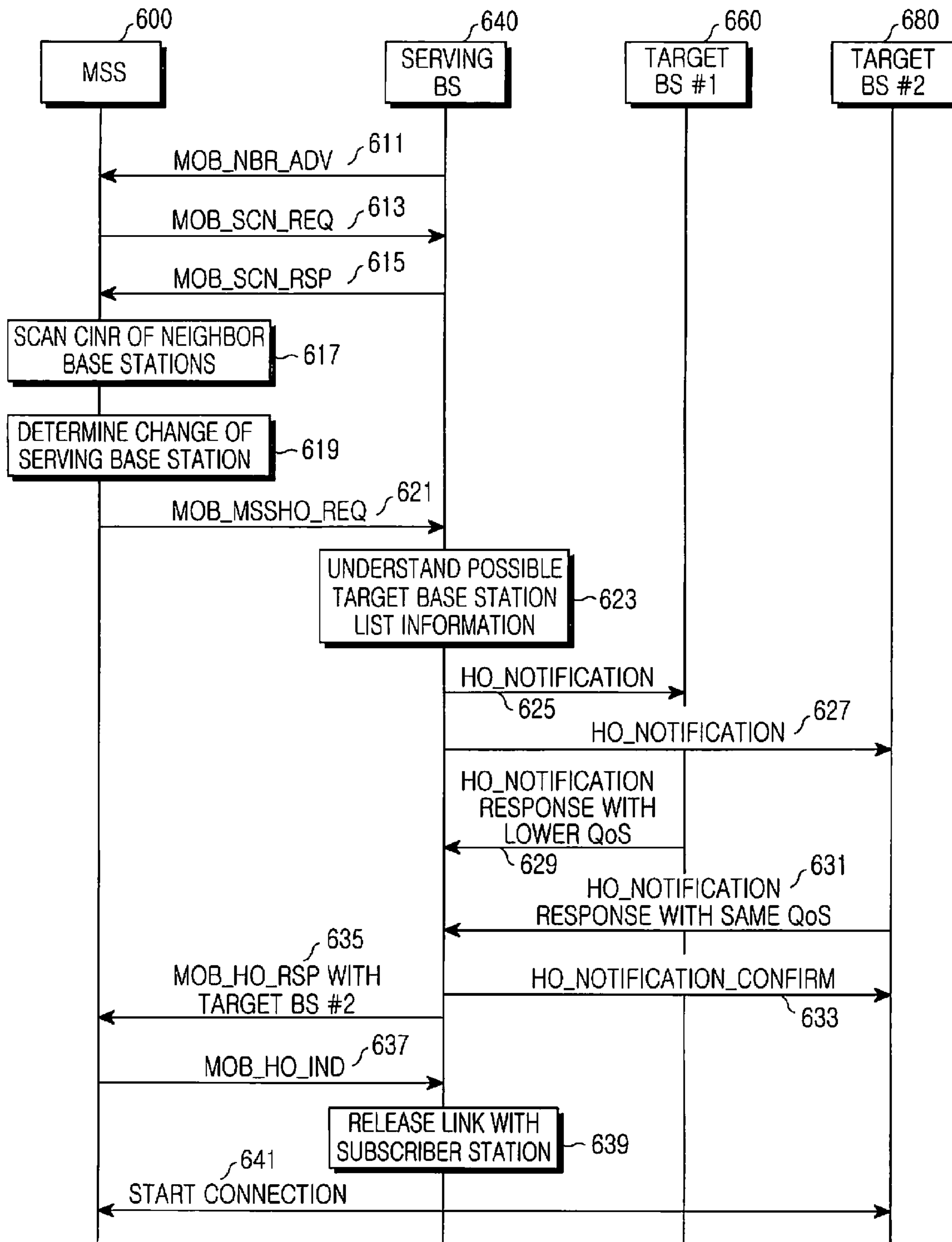
FIG.6 (PRIOR ART)
