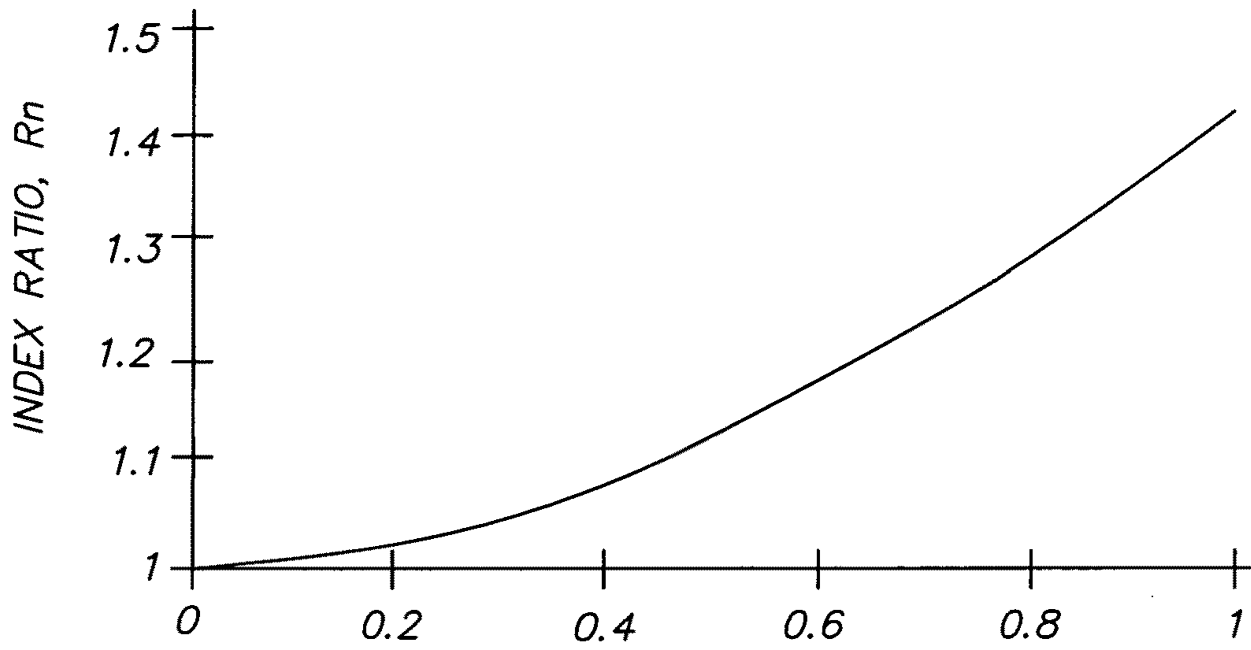
FIG. 3 NUMERICAL APERTURE OF INJECTED LIGHT IN AIR
