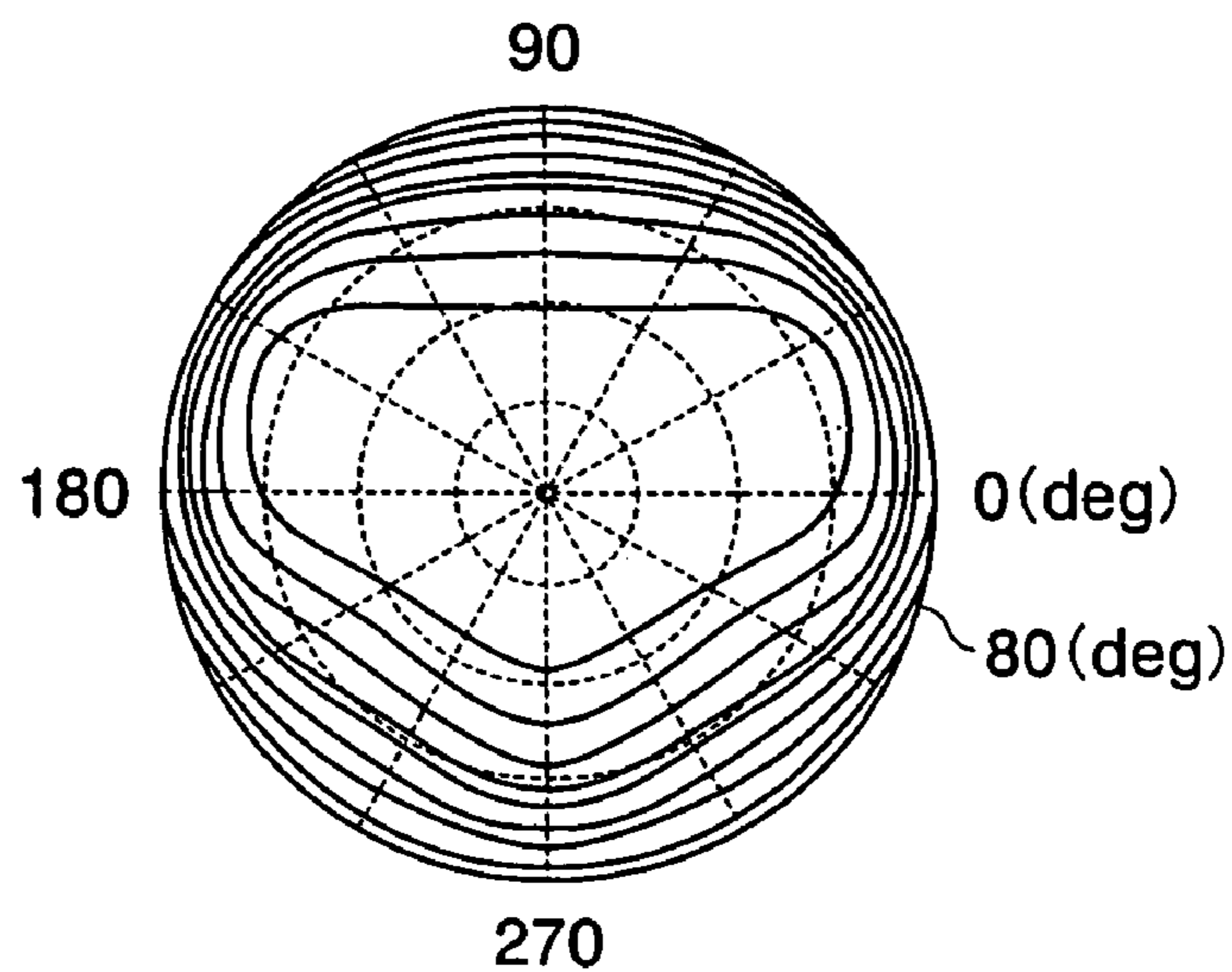
EQUI-TRANSMITTANCE DIAGRAM APPLIED VOLTAGE OF 9V
