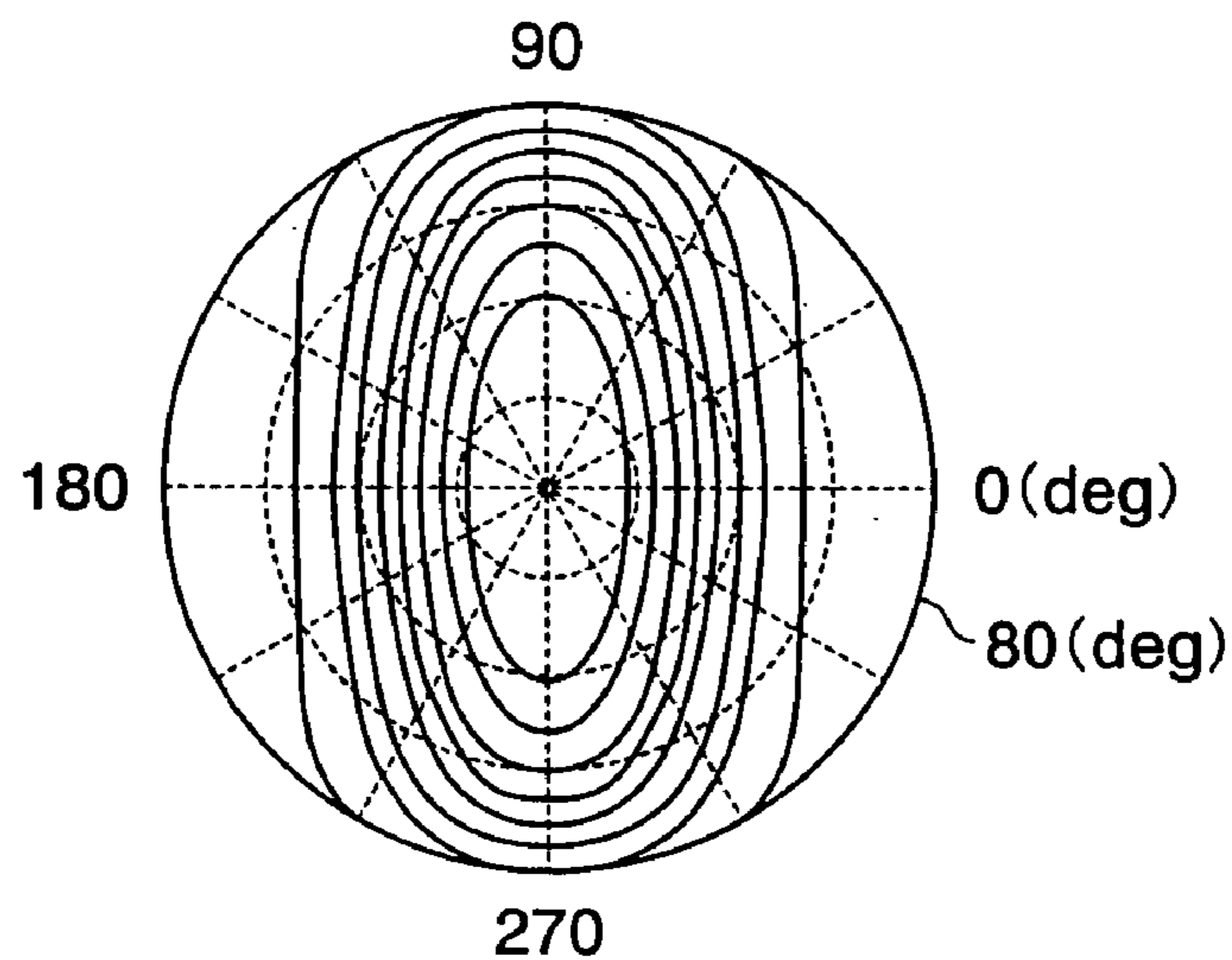
EQUI-TRANSMITTANCE DIAGRAM APPLIED VOLTAGE OF 2V
