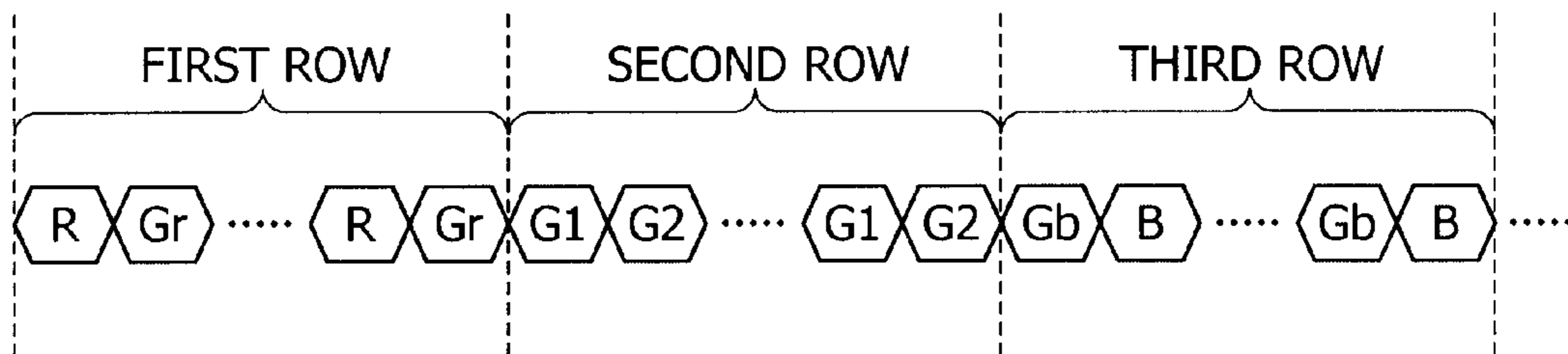
TIMING CHART OF ALL PIXEL MODE
