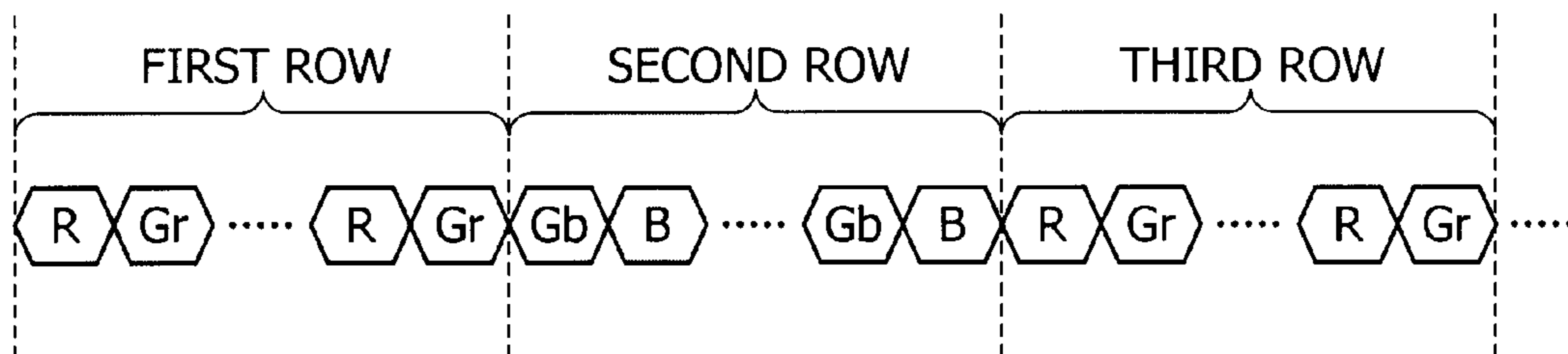
TIMING CHART OF BAYER MODE
