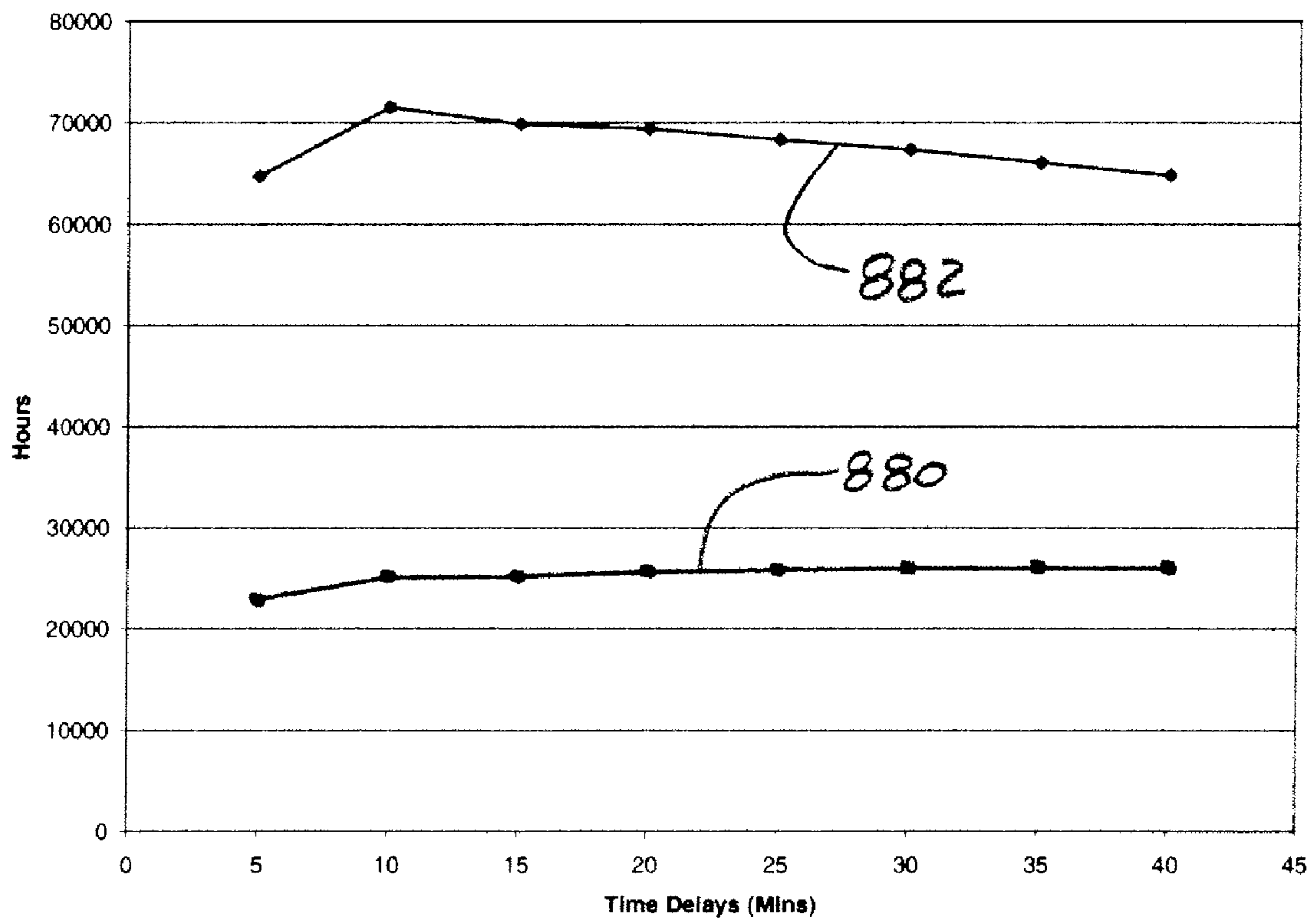
Calendar Life and Lamp Life vs. Time Delays
