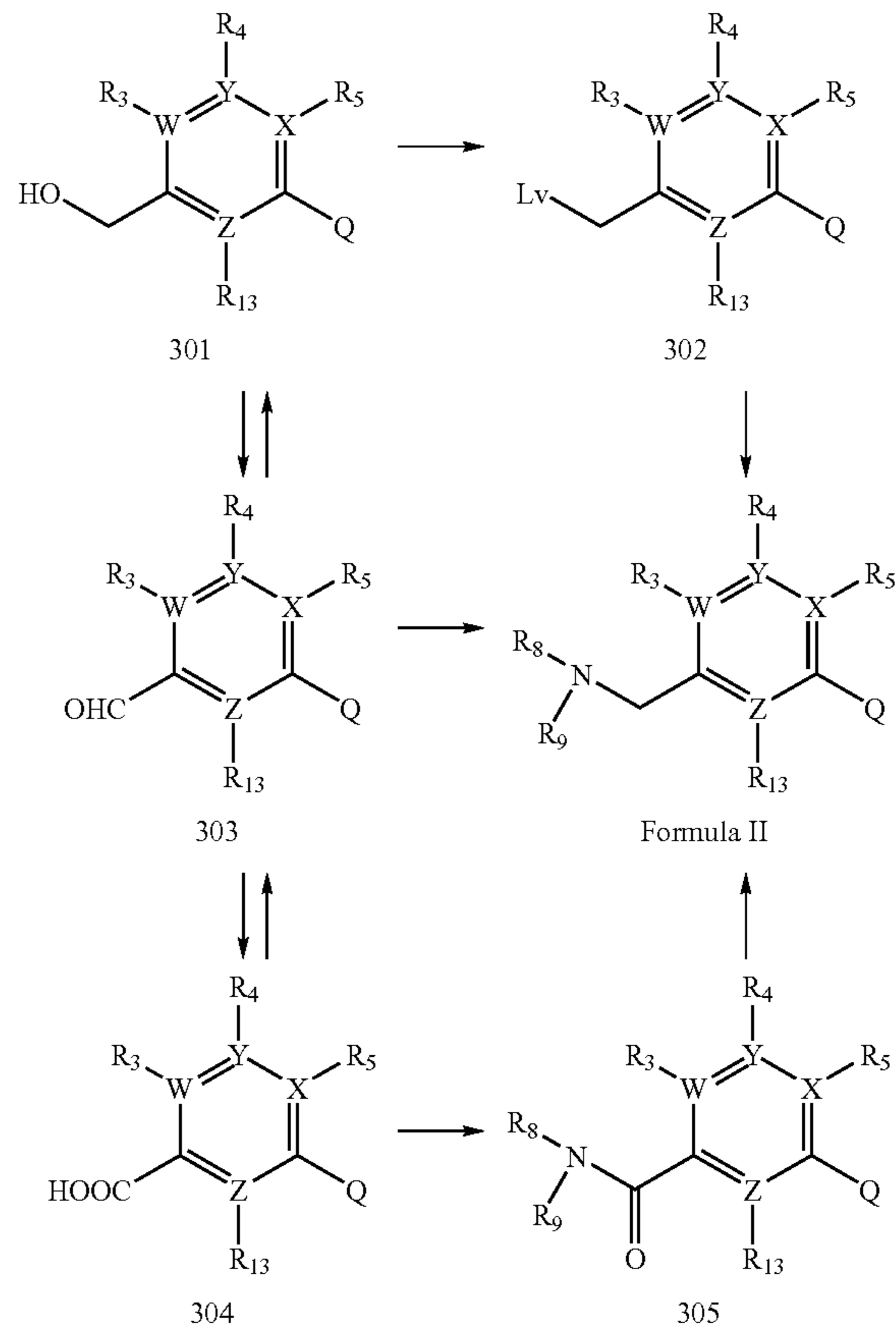
REACTION SCHEME 3
