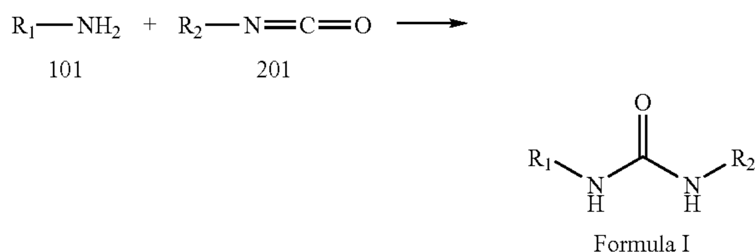
REACTION SCHEME 2
