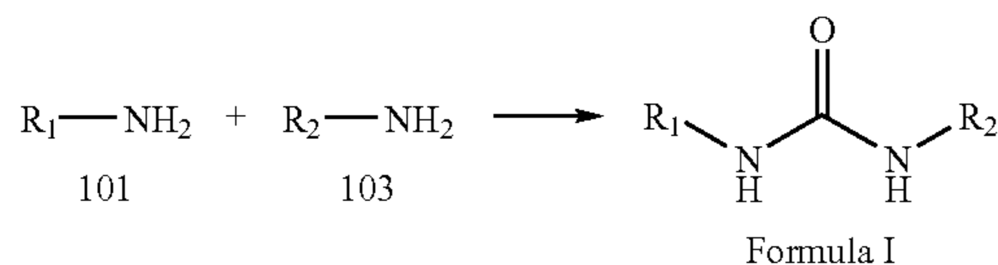
REACTION SCHEME 1
