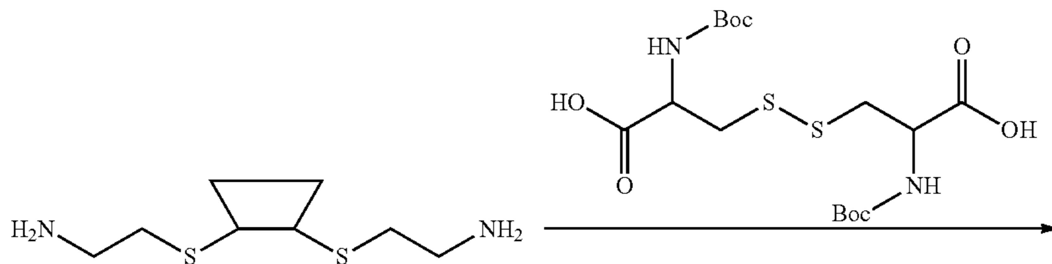
Scheme VII
