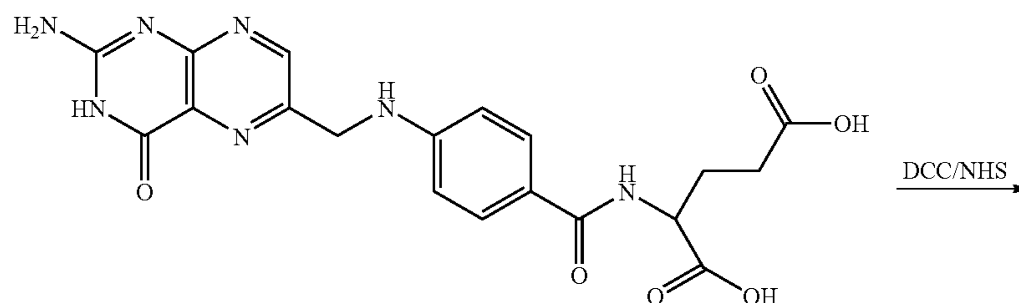
Scheme XXXXIX
