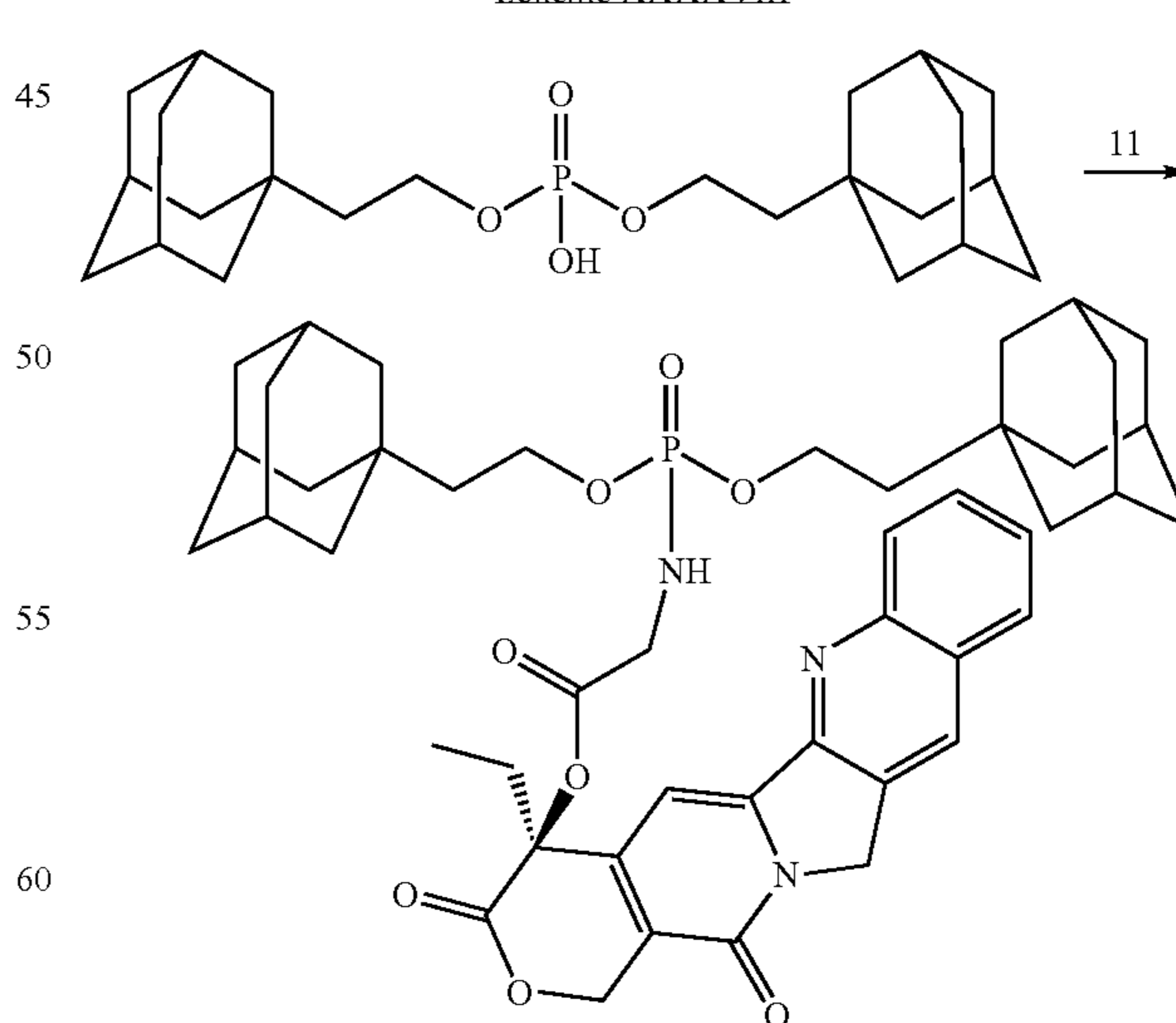
Scheme XXXXVIII
