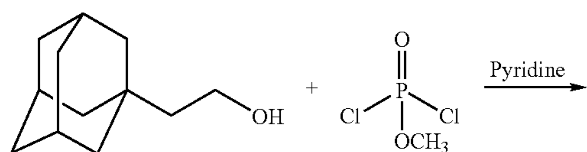
Scheme XXXXVII
