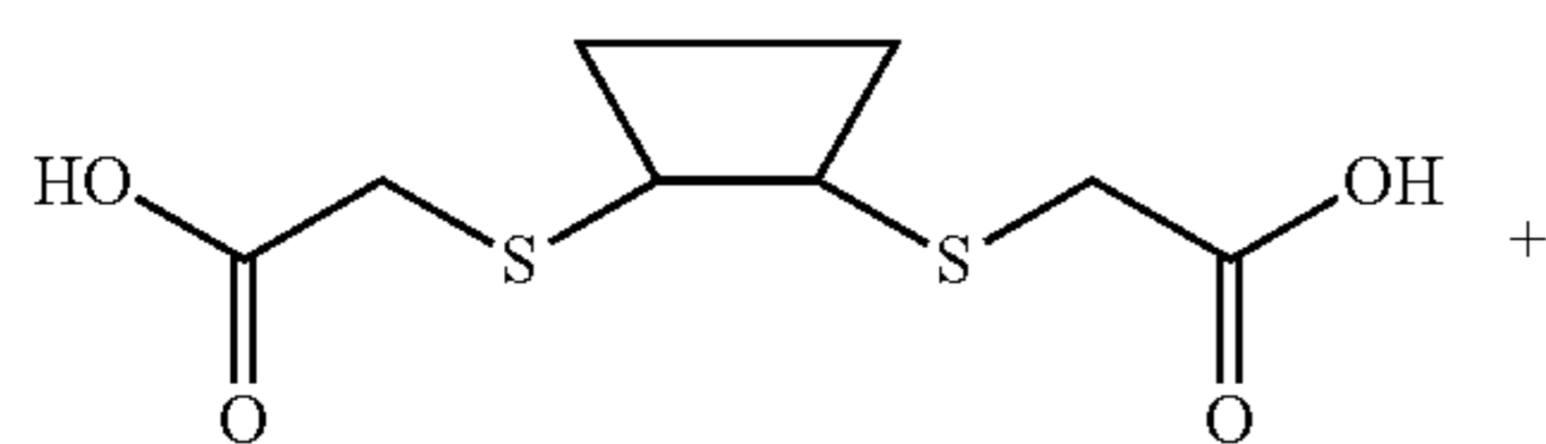
Scheme VIII
