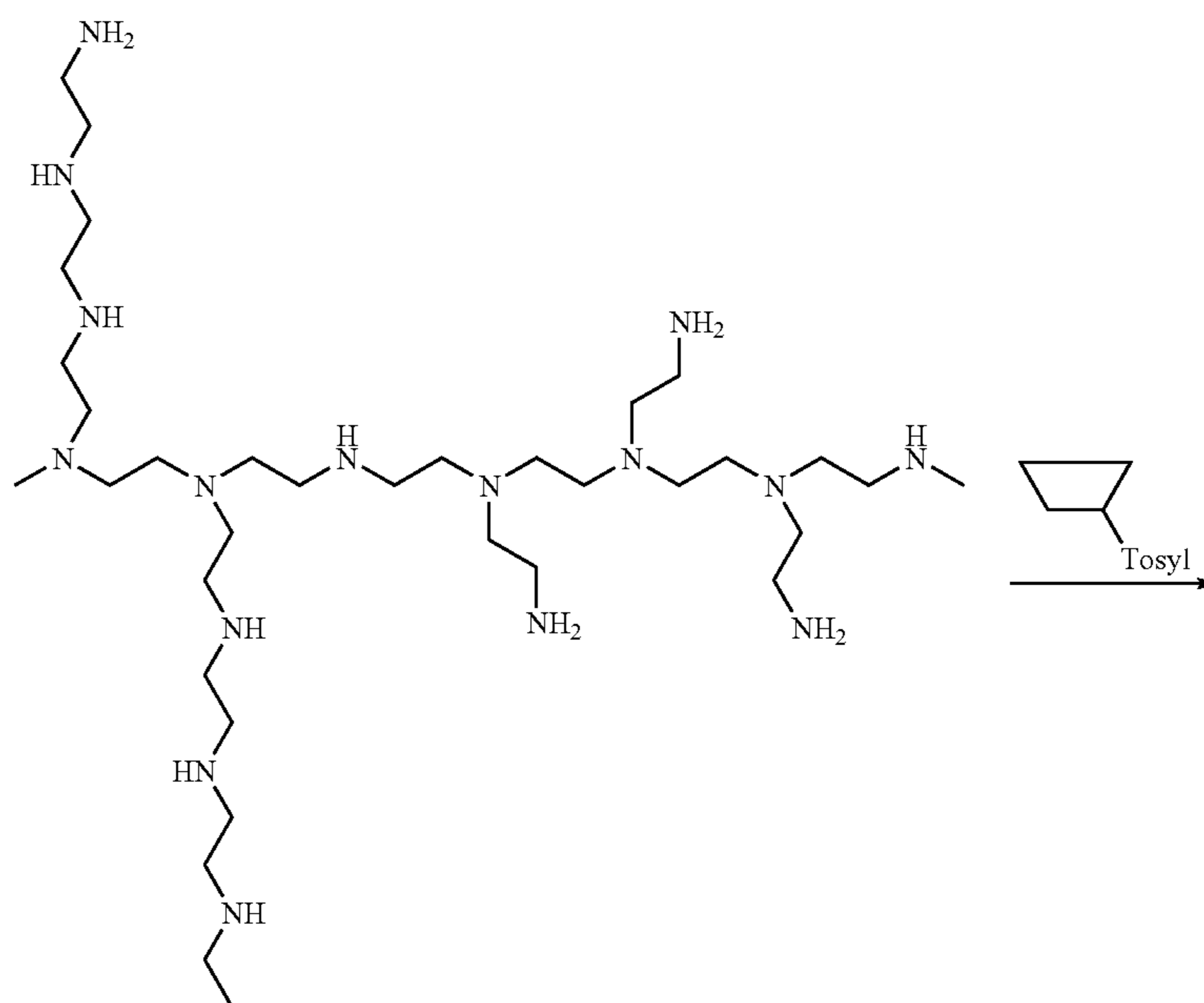
Scheme XXXXIV
