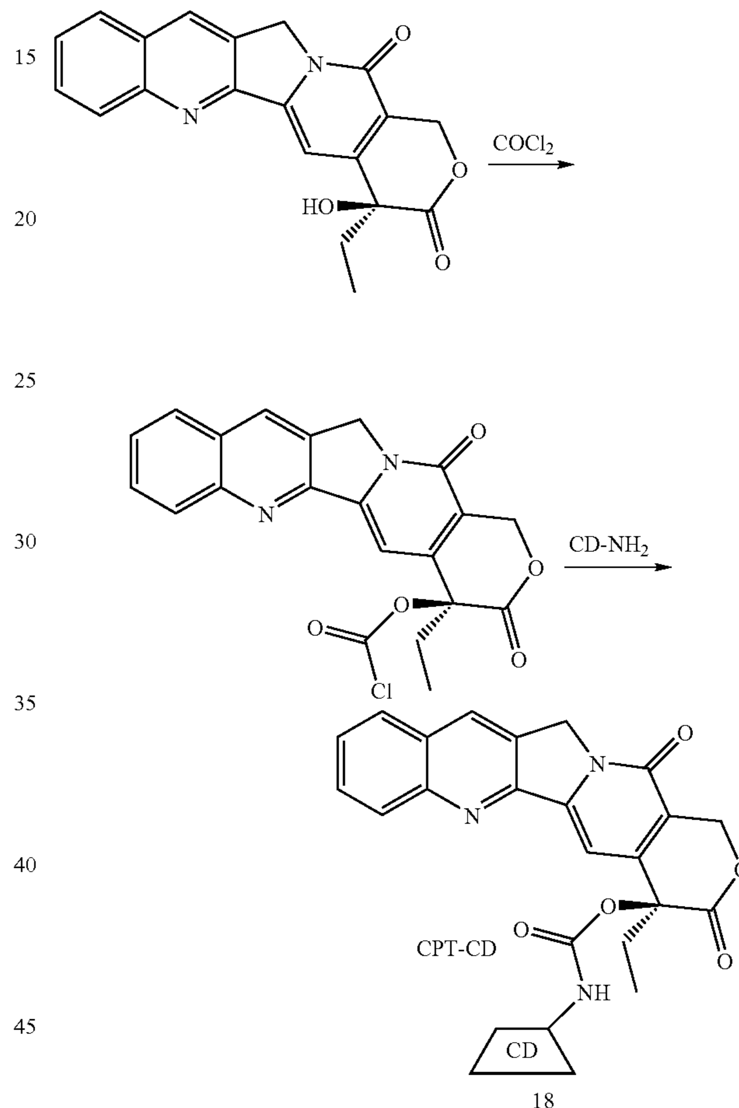
Scheme XXVIII
