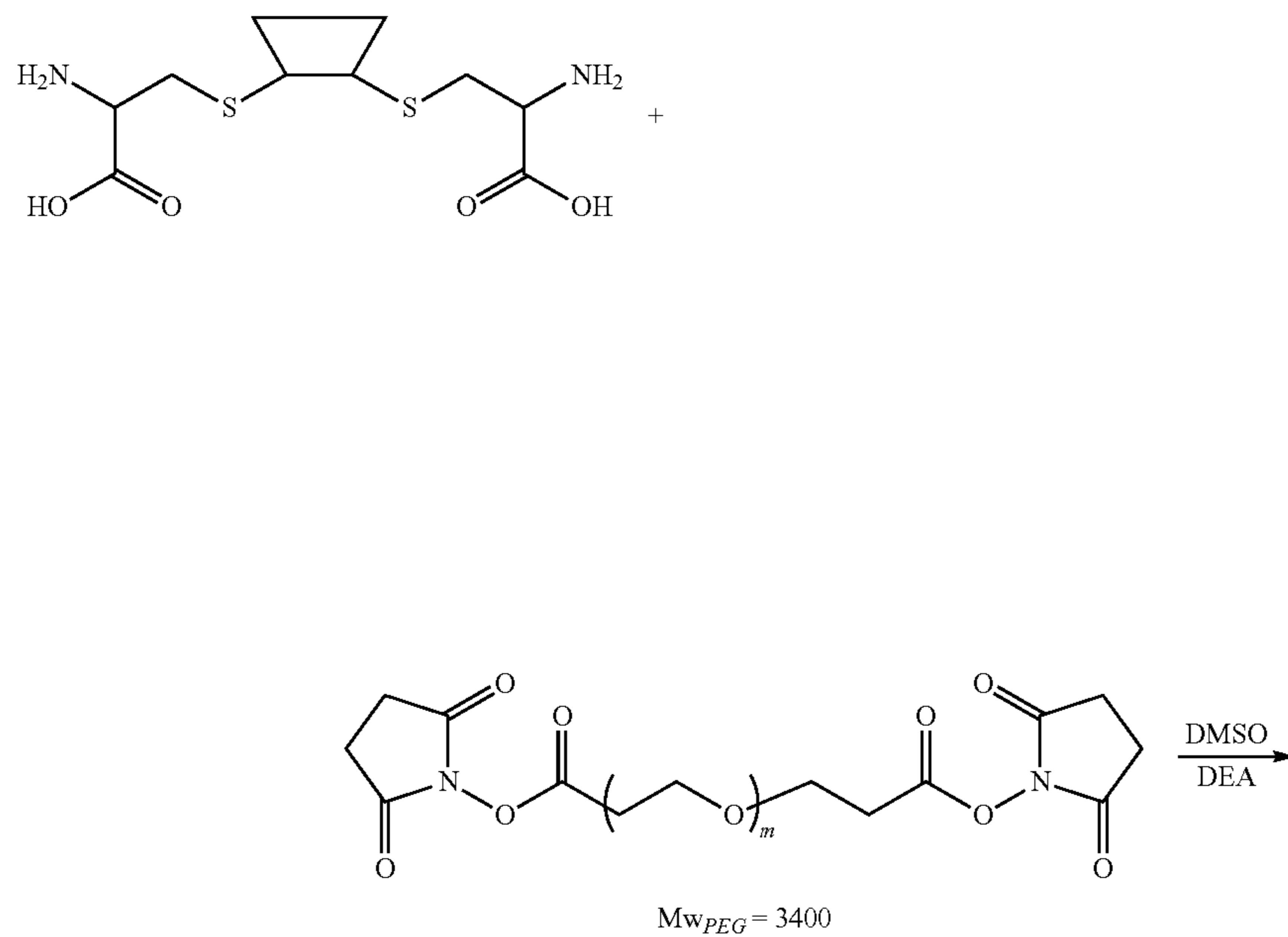
Scheme XIII
