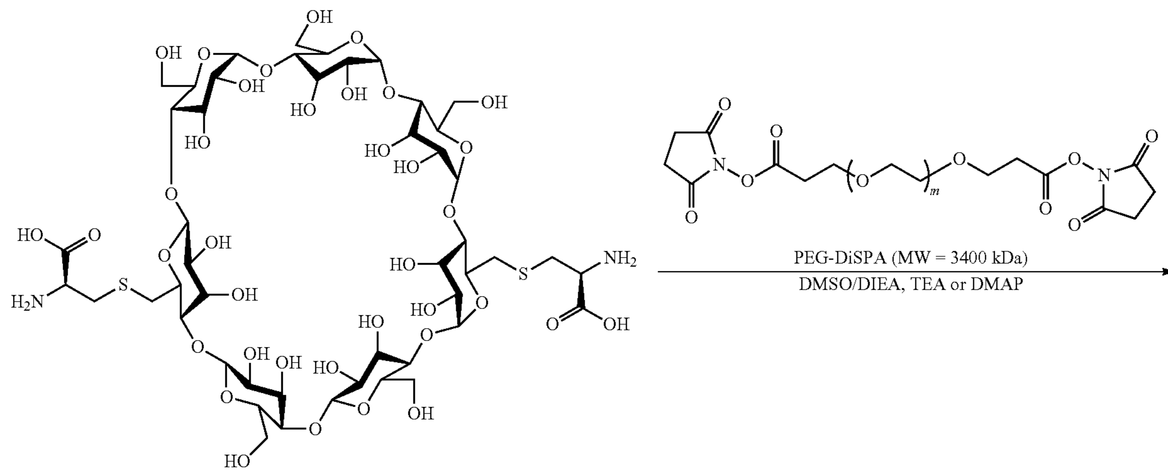
Scheme XXXVIIIa
