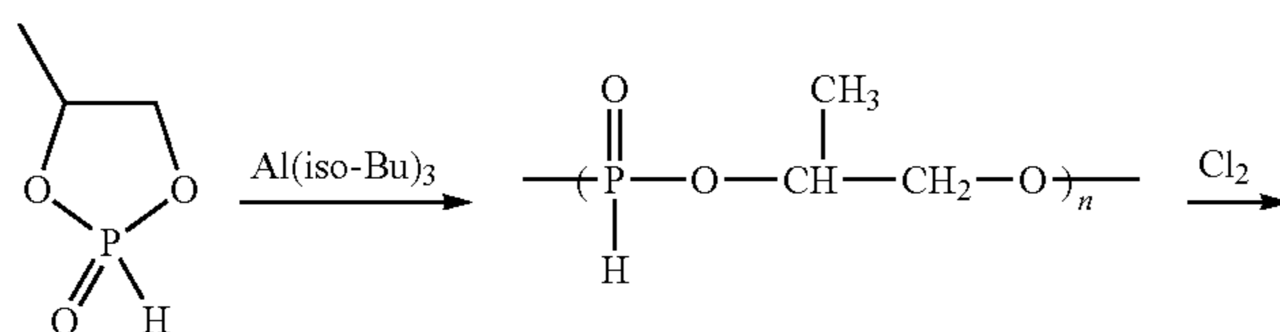
Scheme IX
