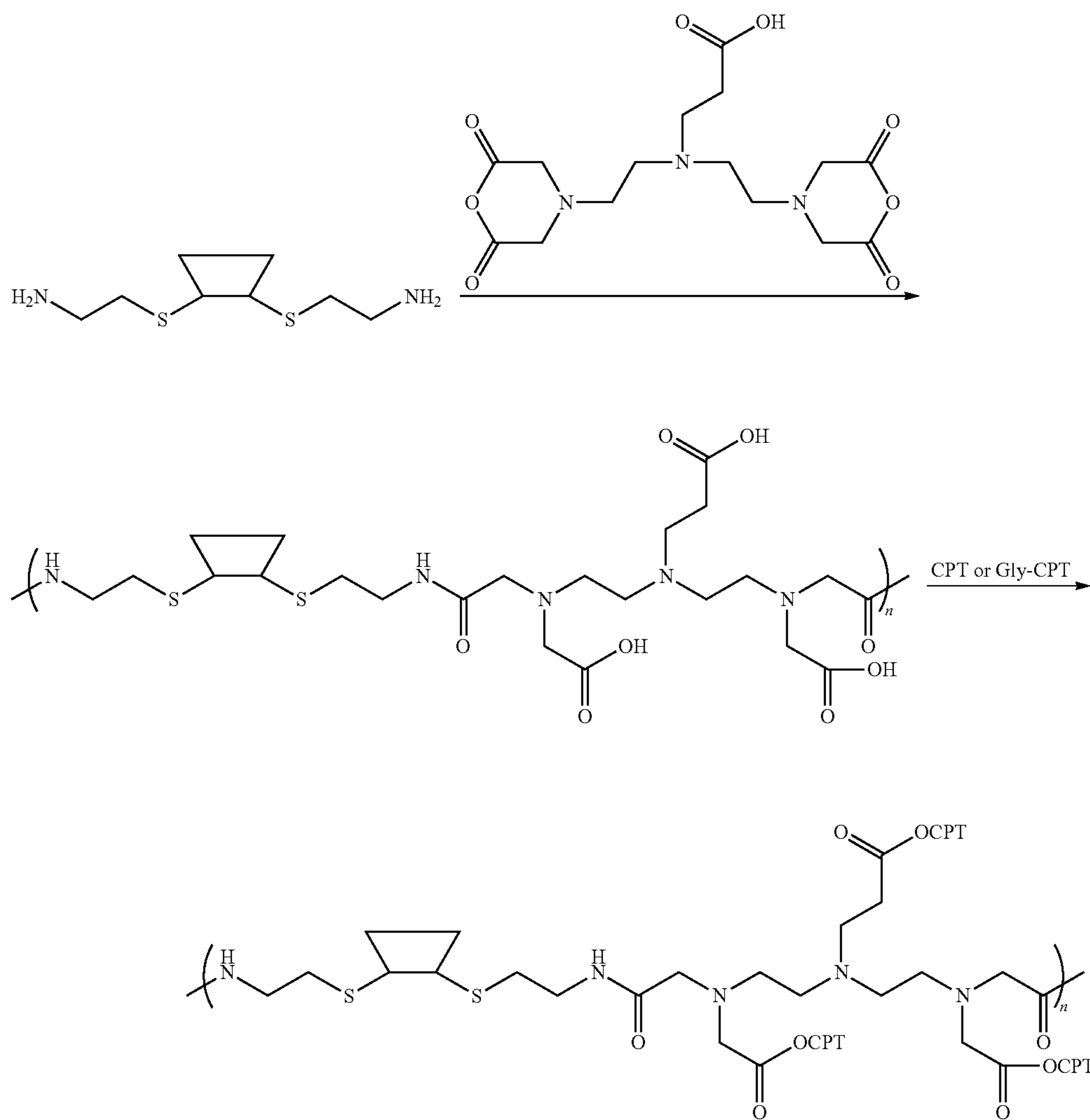
Scheme V
