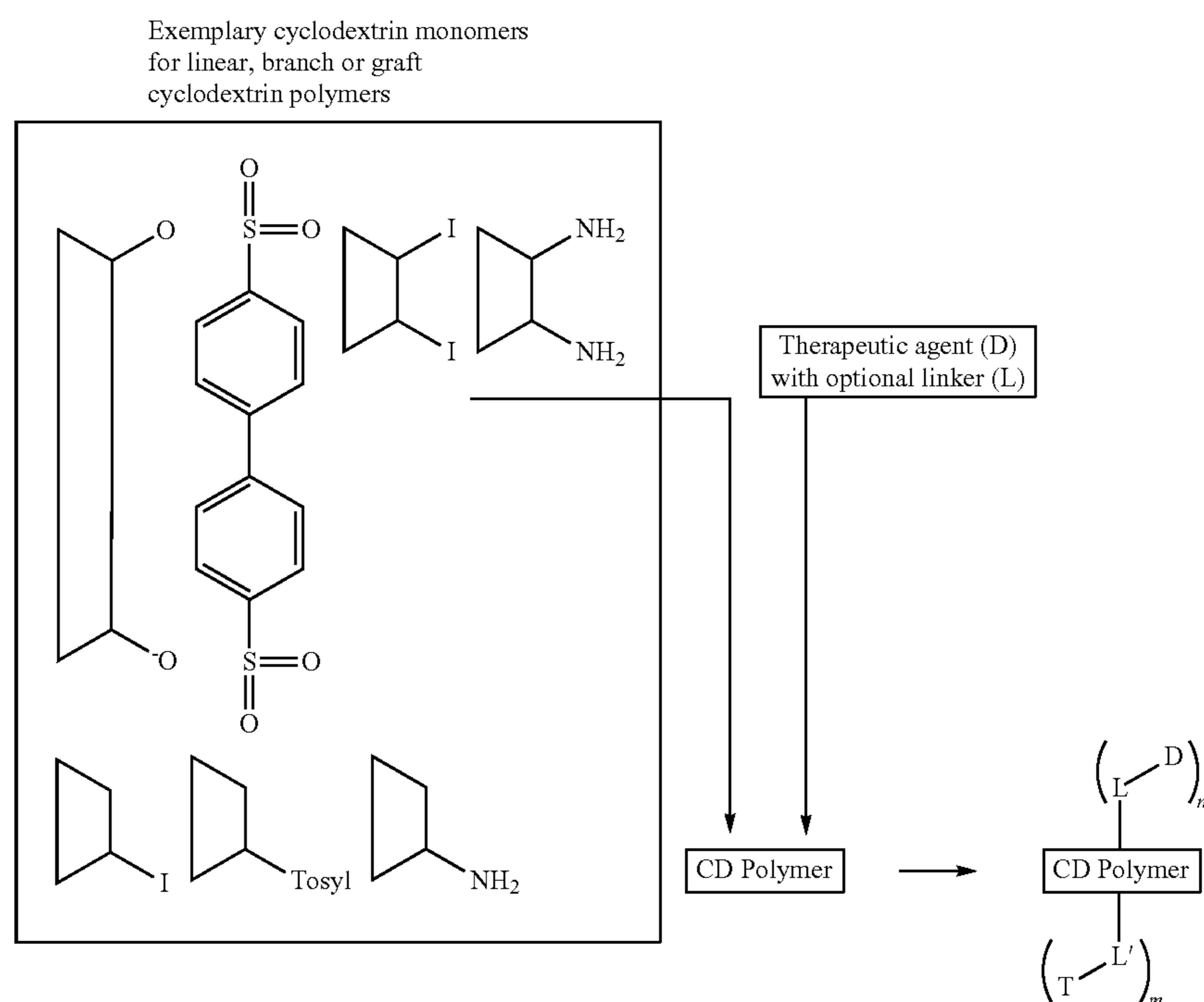
Scheme II
