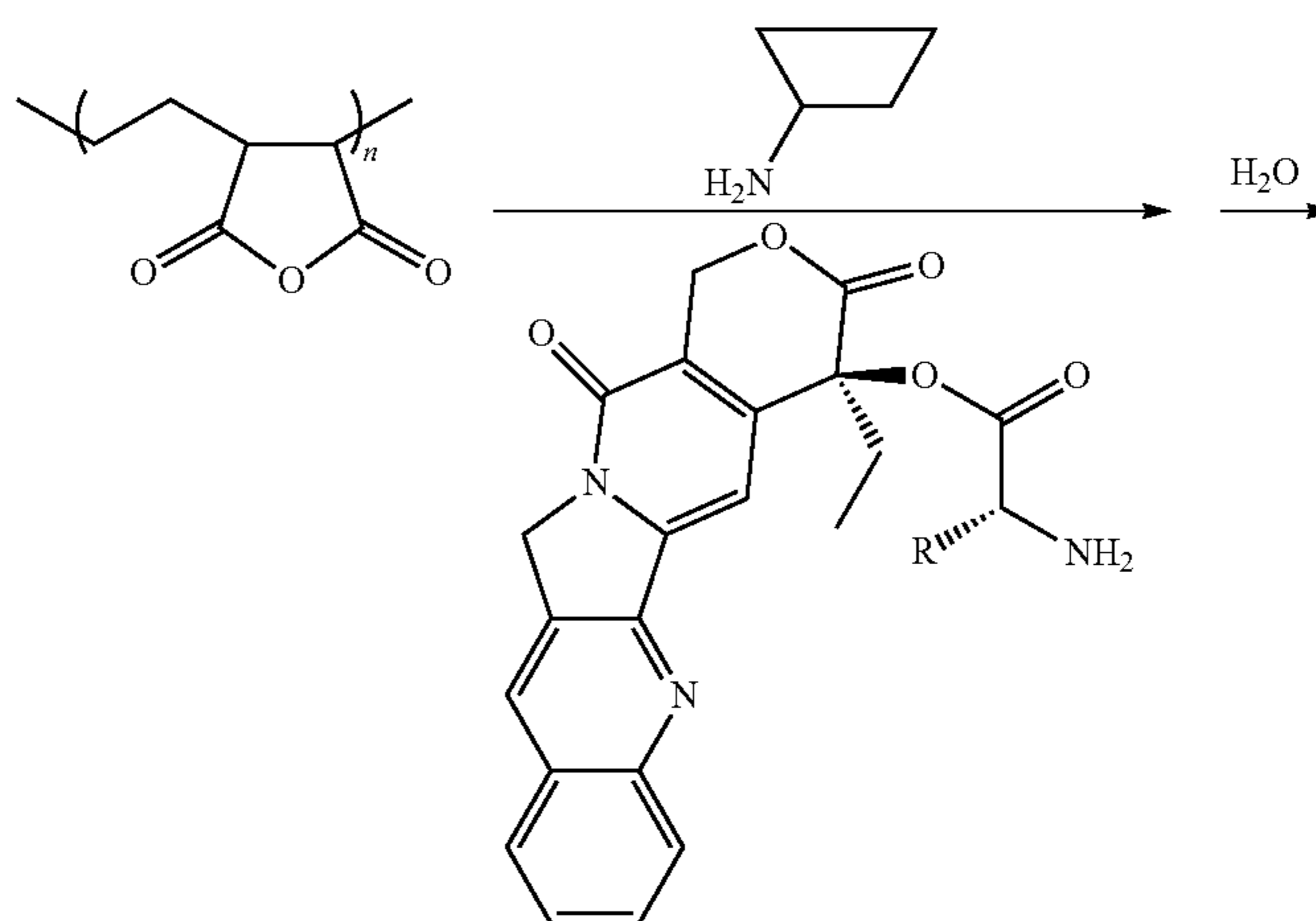
Scheme XI
