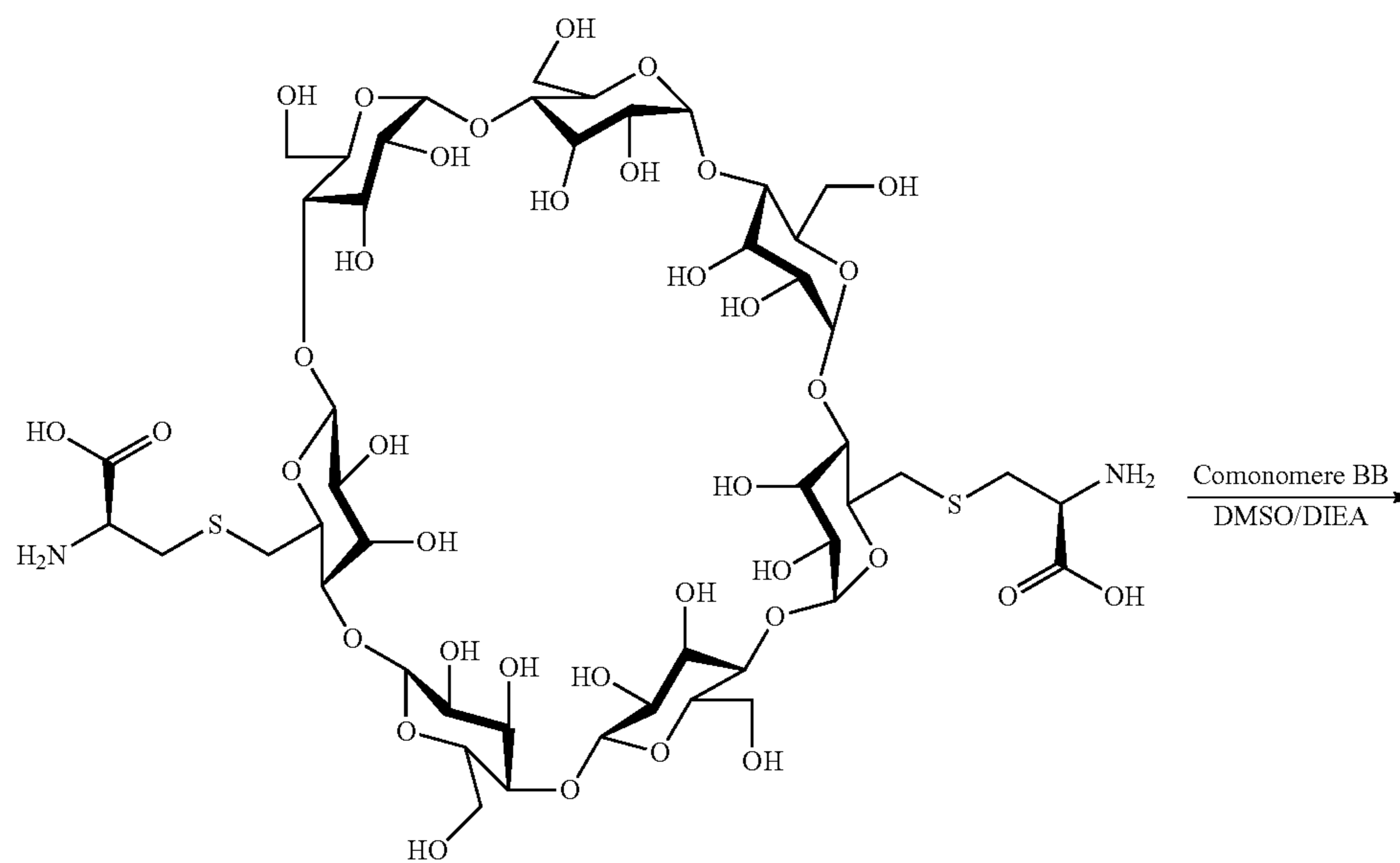
Scheme XXXVIIIb
