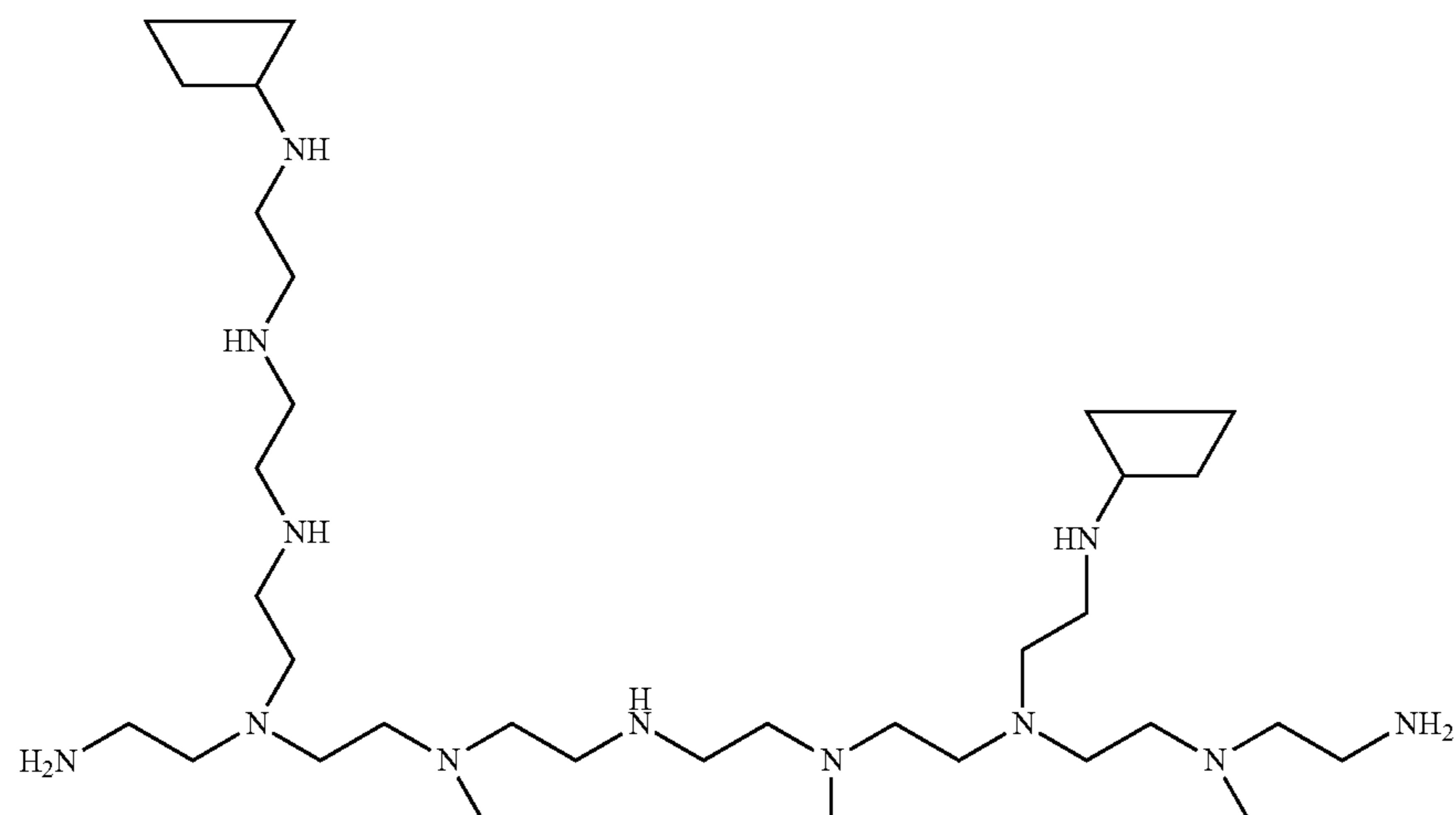
Scheme XXXXV
