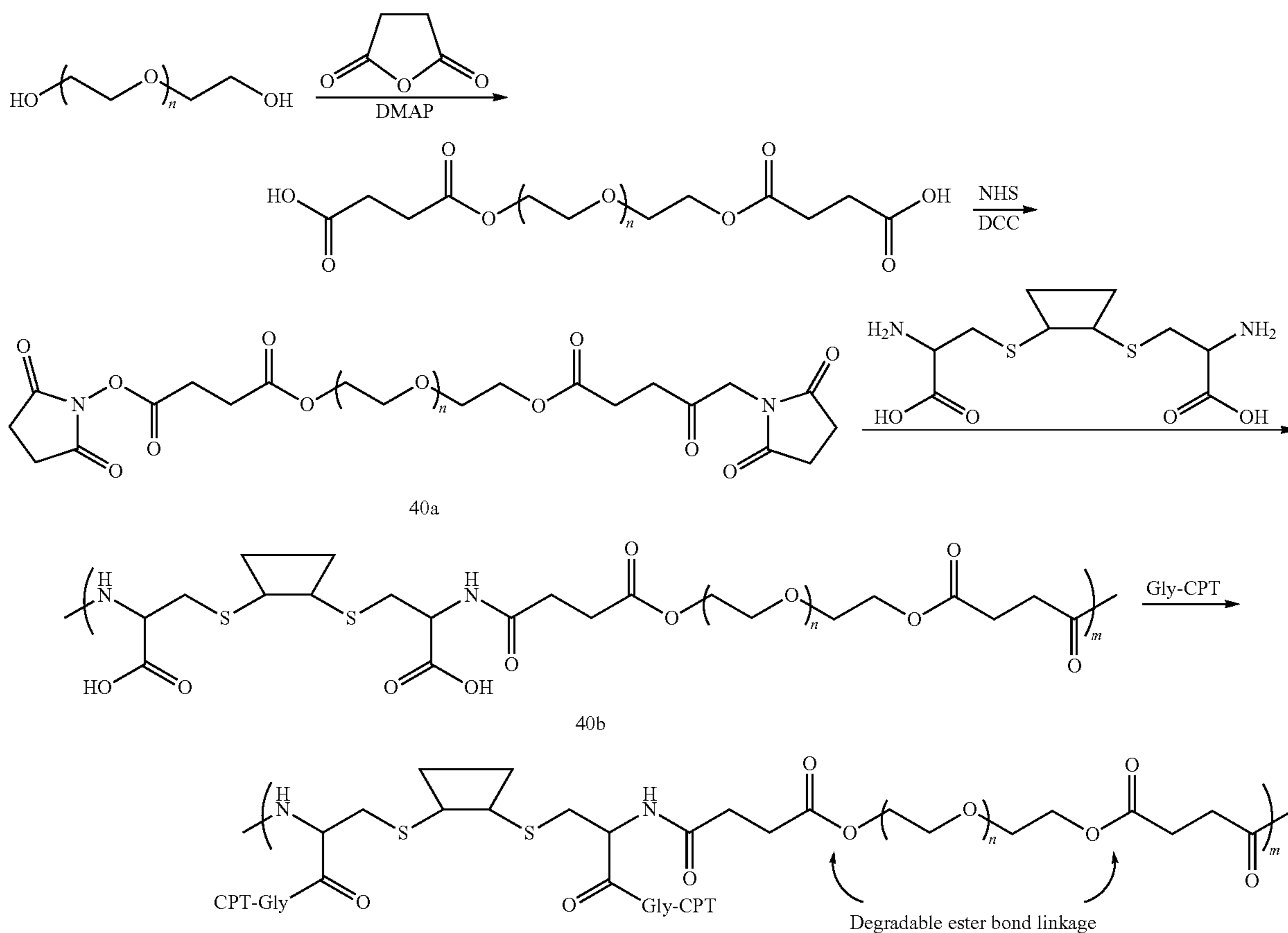
Scheme XXXXI
