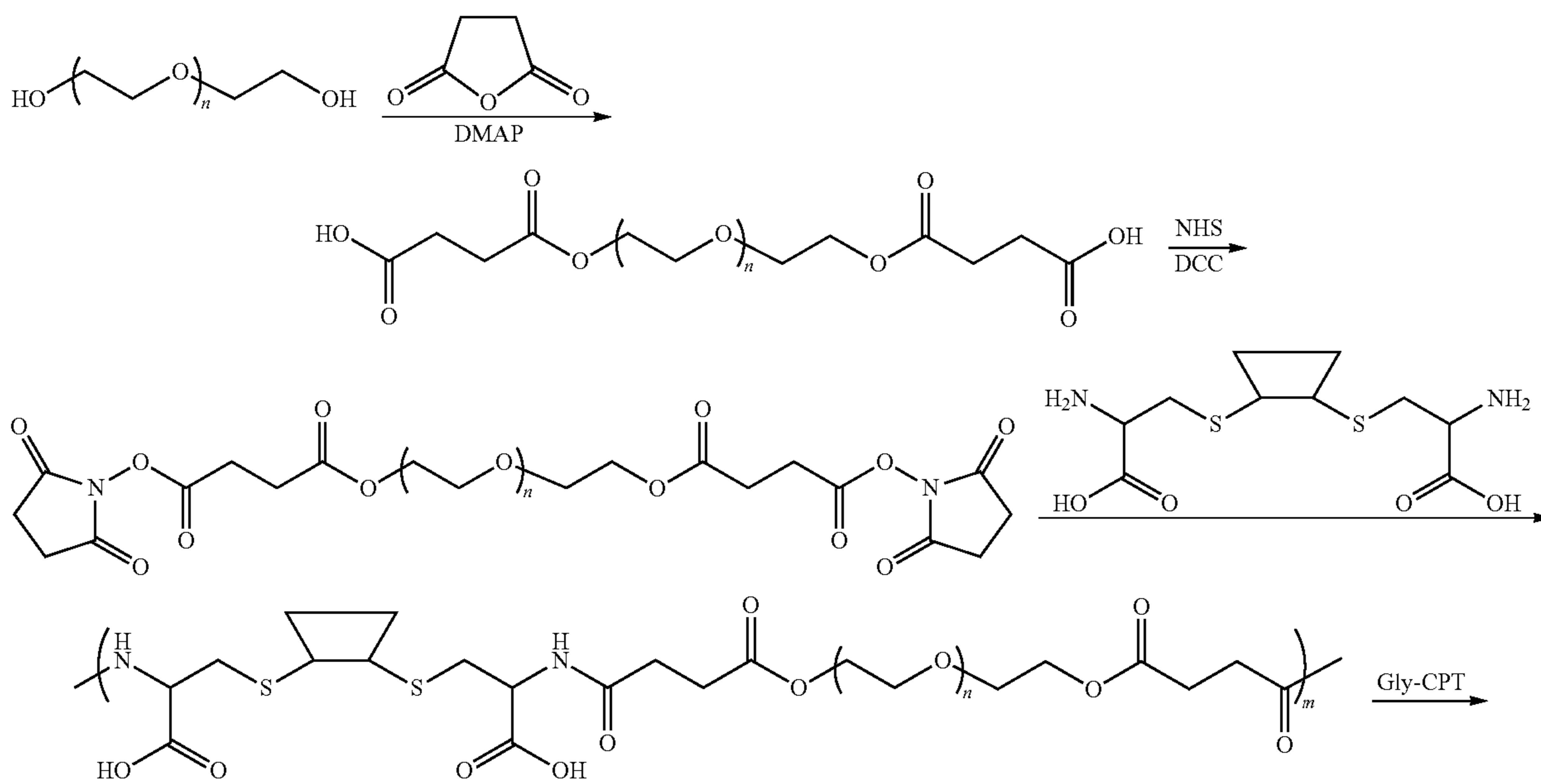
Scheme XIV
