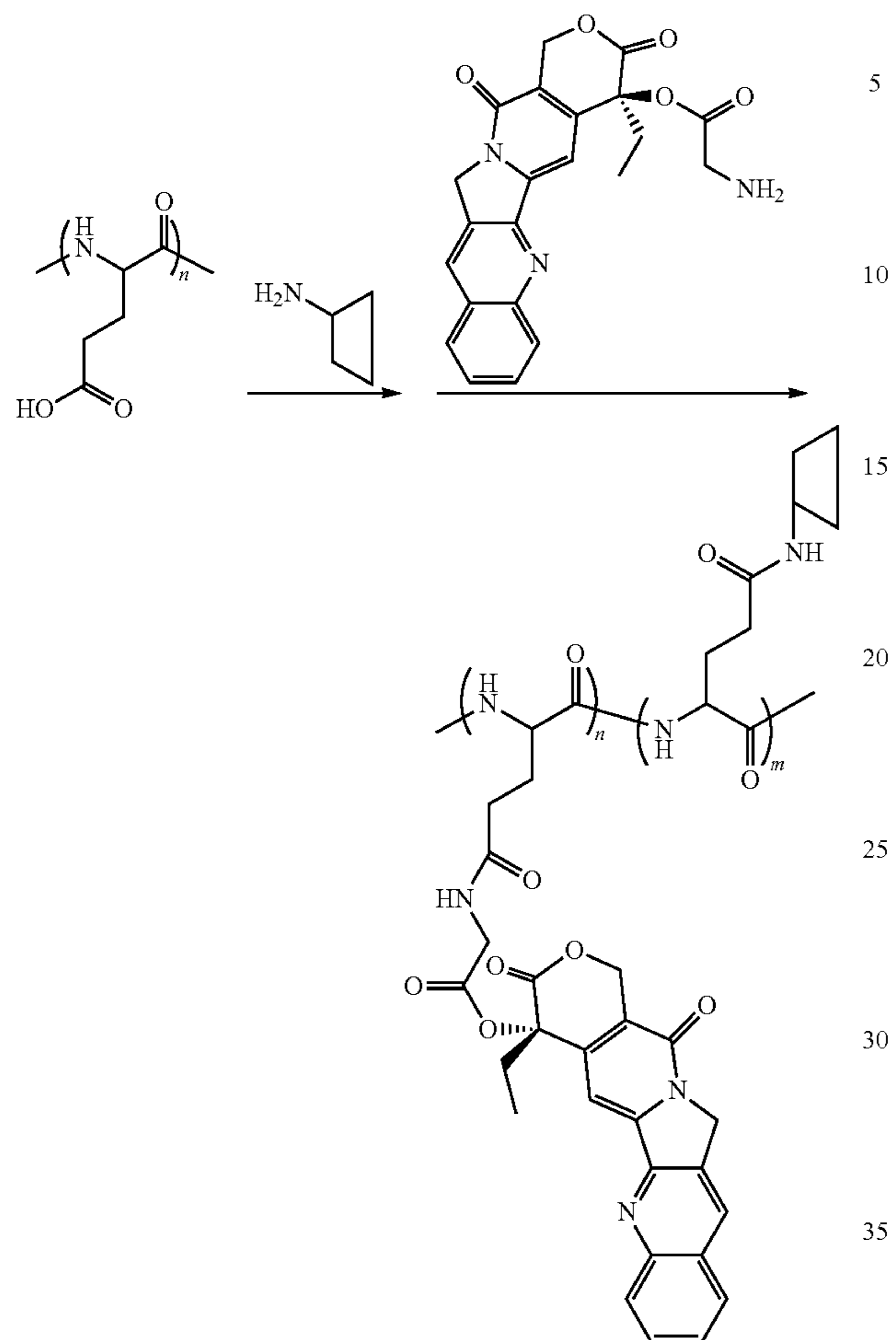
Scheme XII
