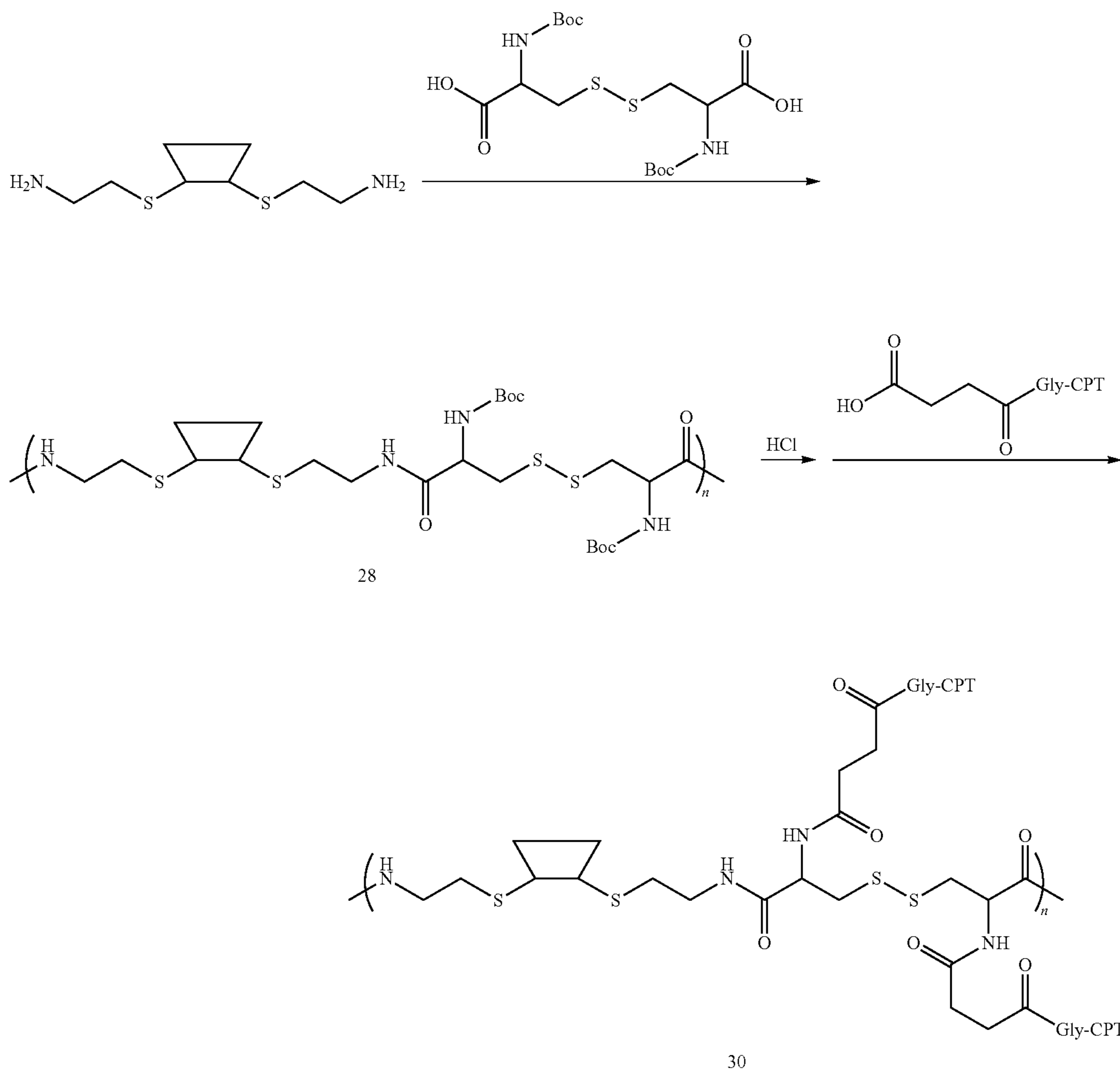
Scheme XXXIII
