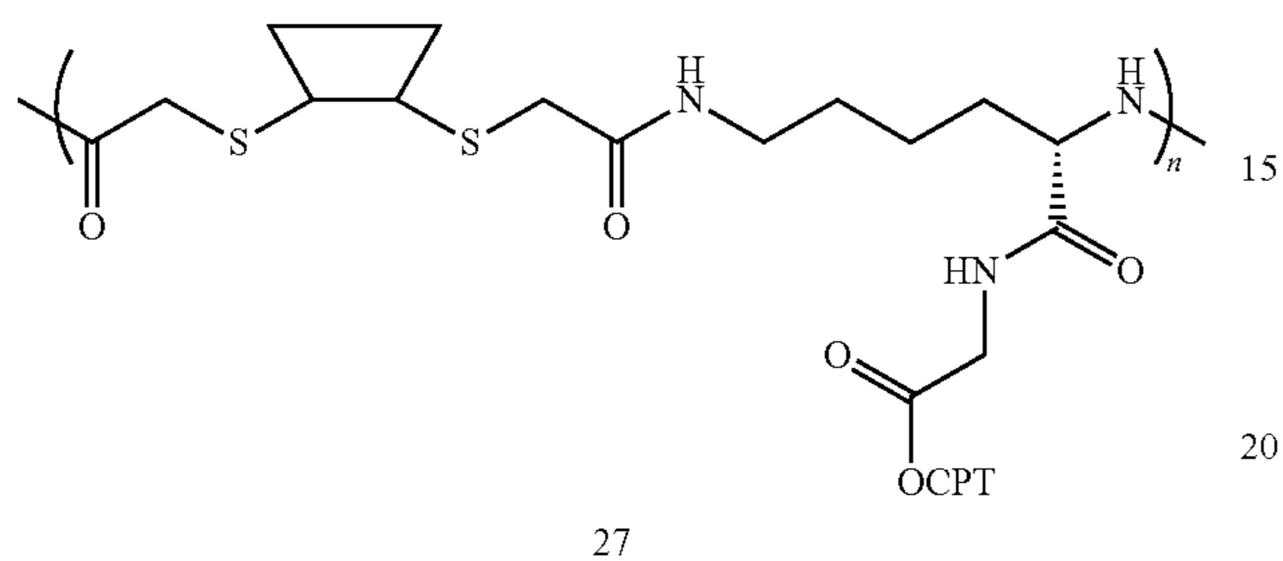
Scheme XXXIII
