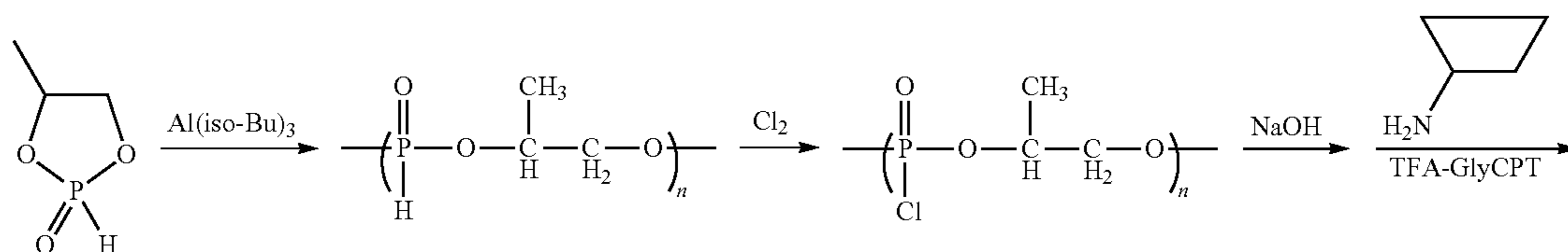
Scheme XXXIV
