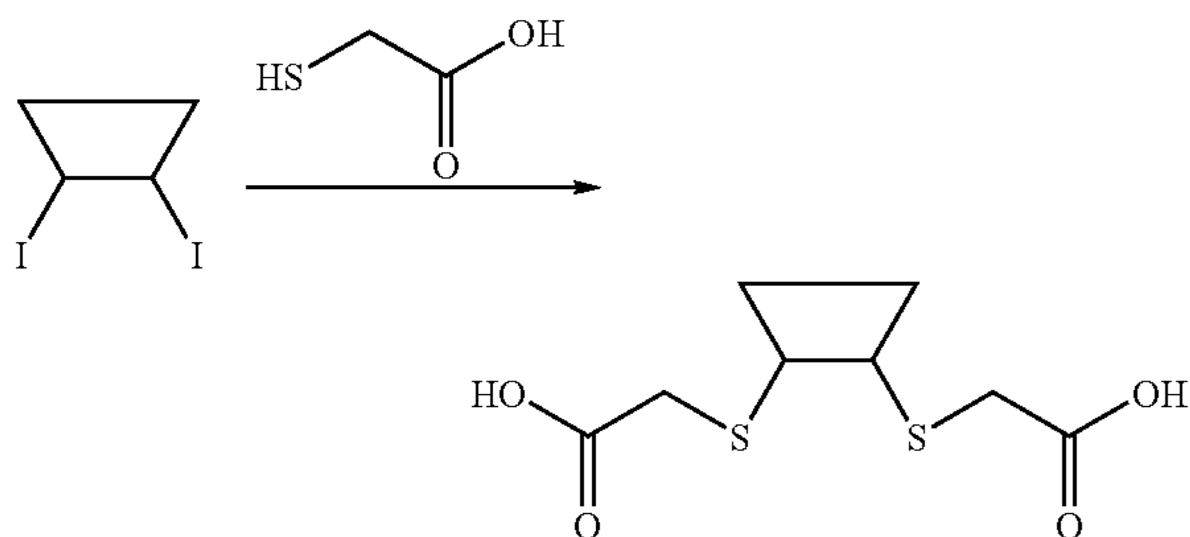
Scheme XIX
