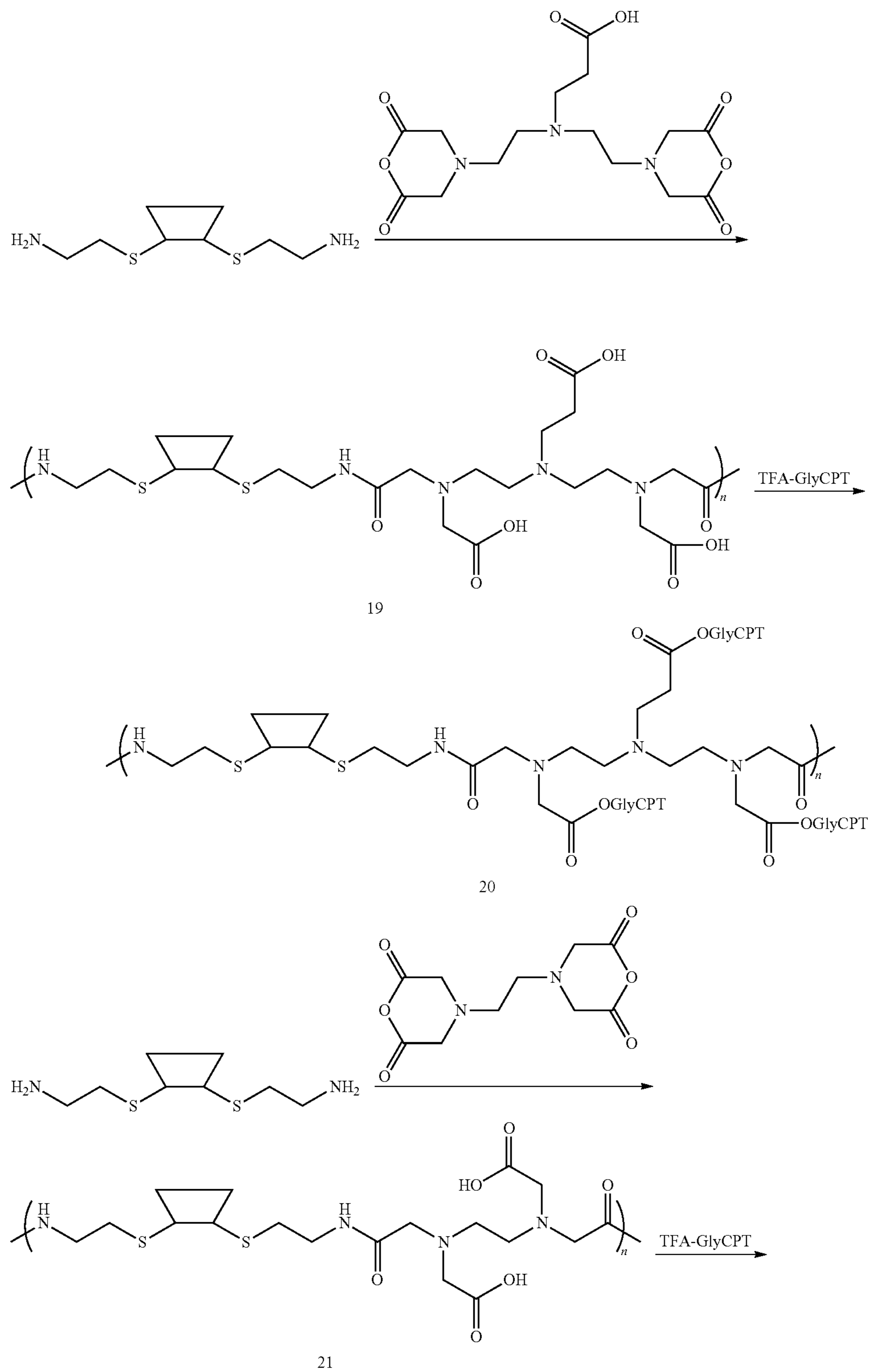
Scheme XXIX
