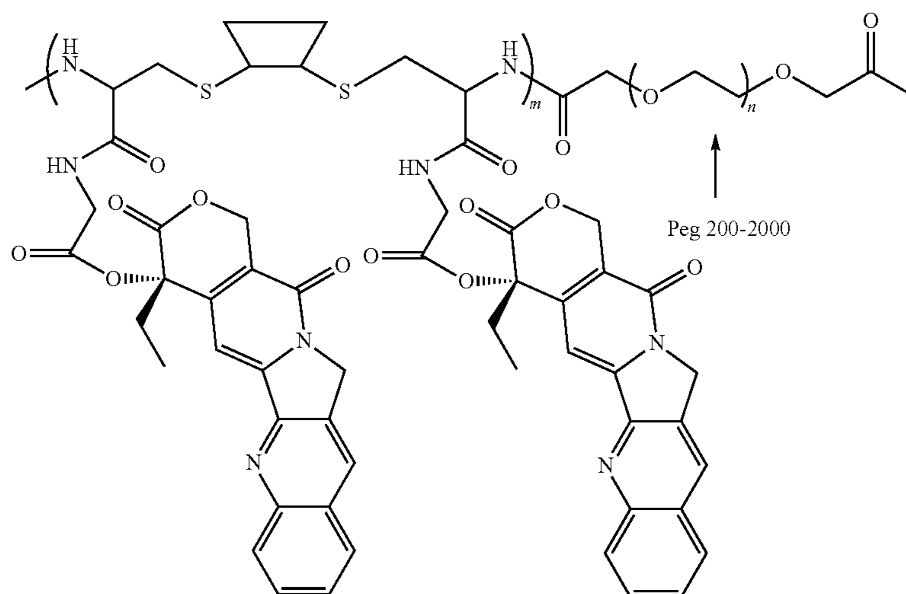
Scheme XXXXII
