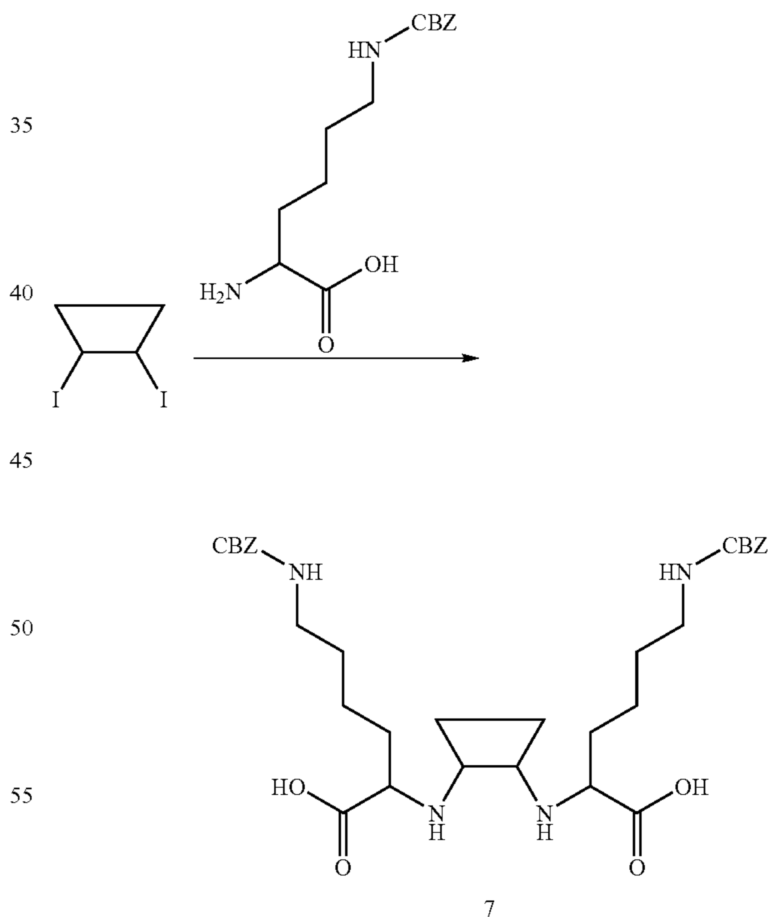
Scheme XXI
