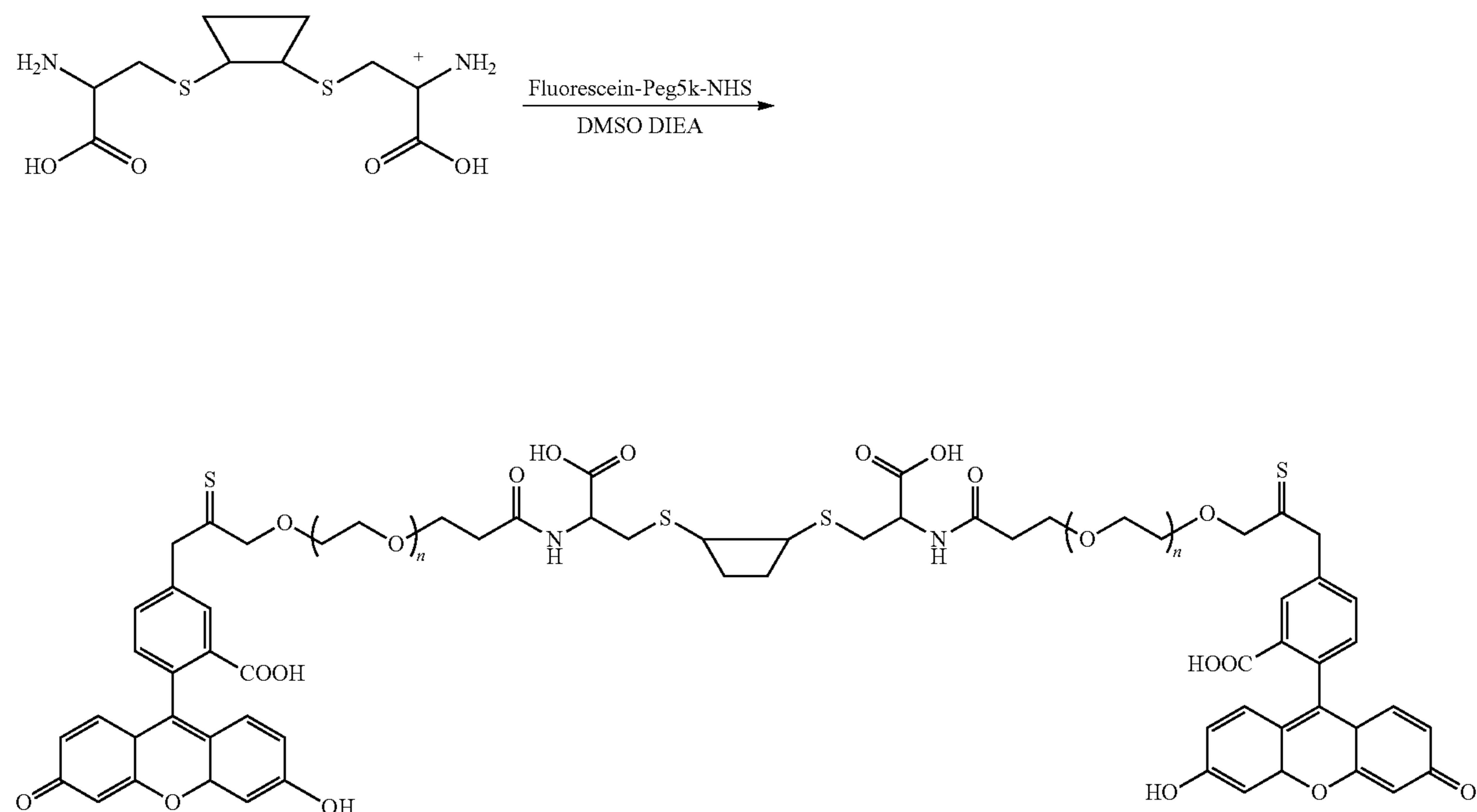
Scheme XXXX
