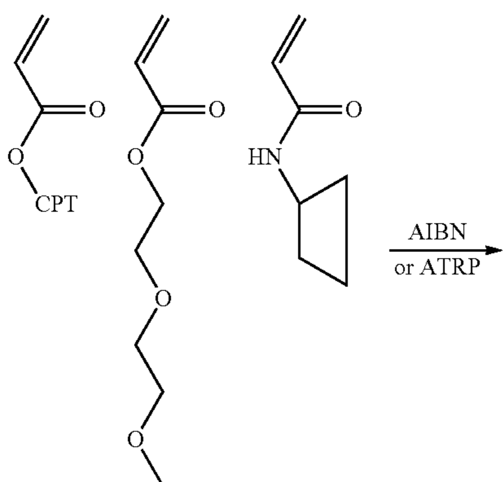
Scheme X
