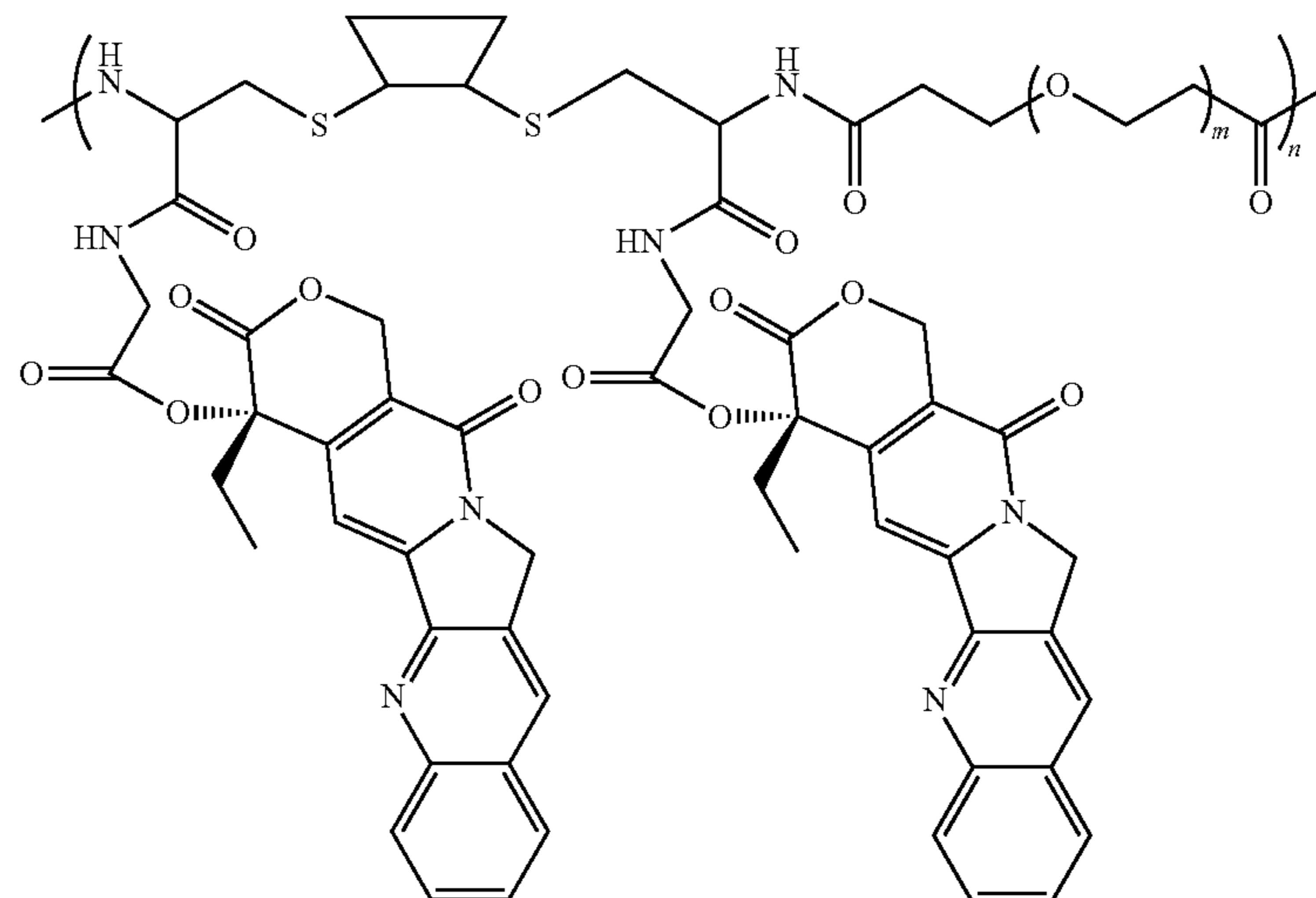
Scheme XXXXIII
