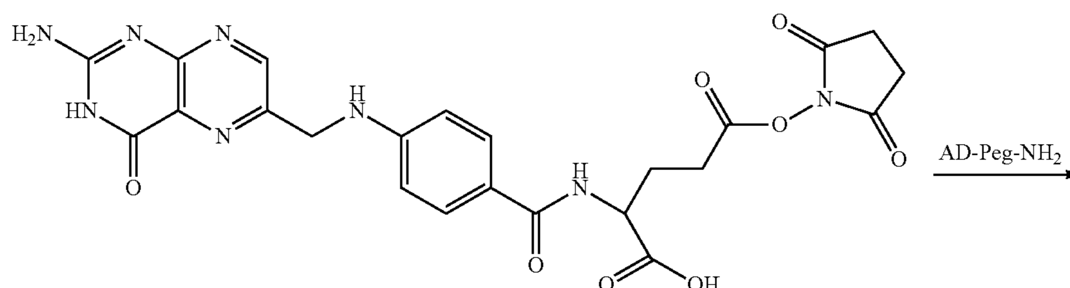
Scheme L
