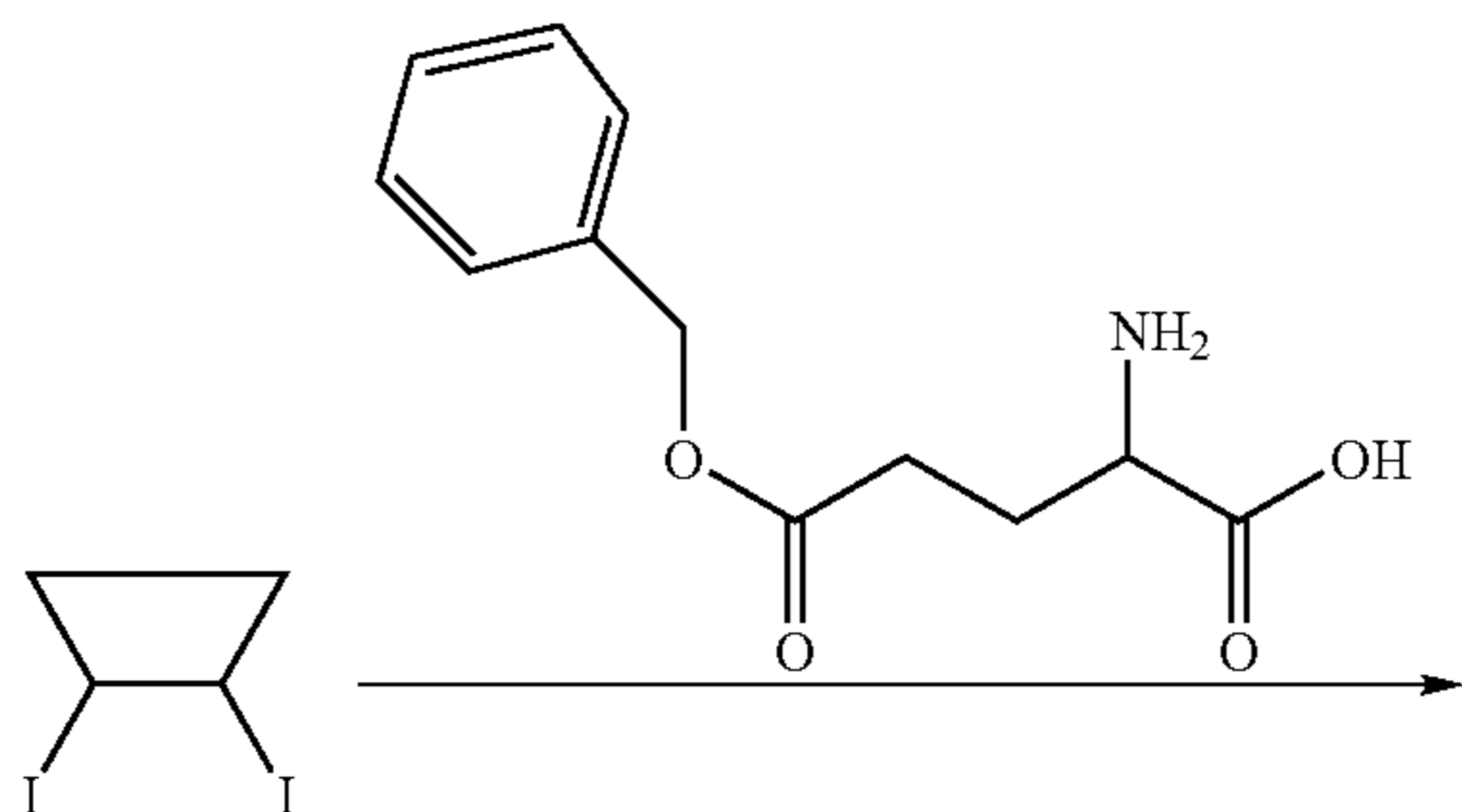
Scheme XX
