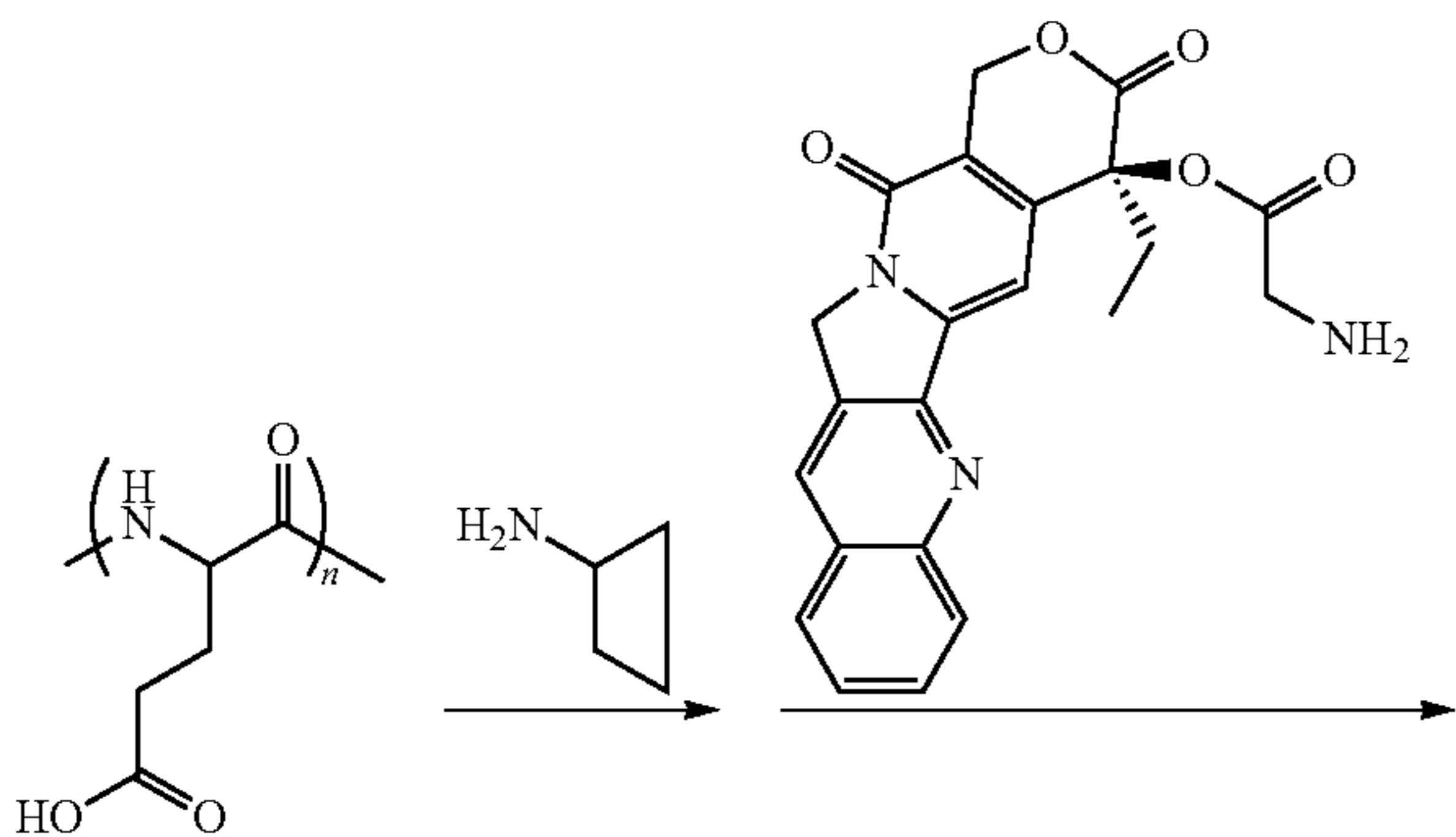
Scheme XXXVII
