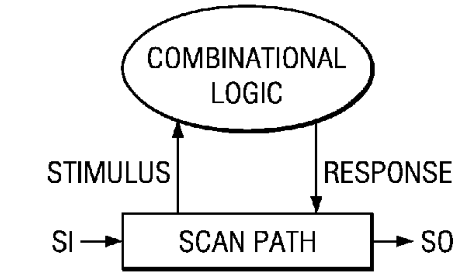
FIG. 3 (PRIOR ART)
