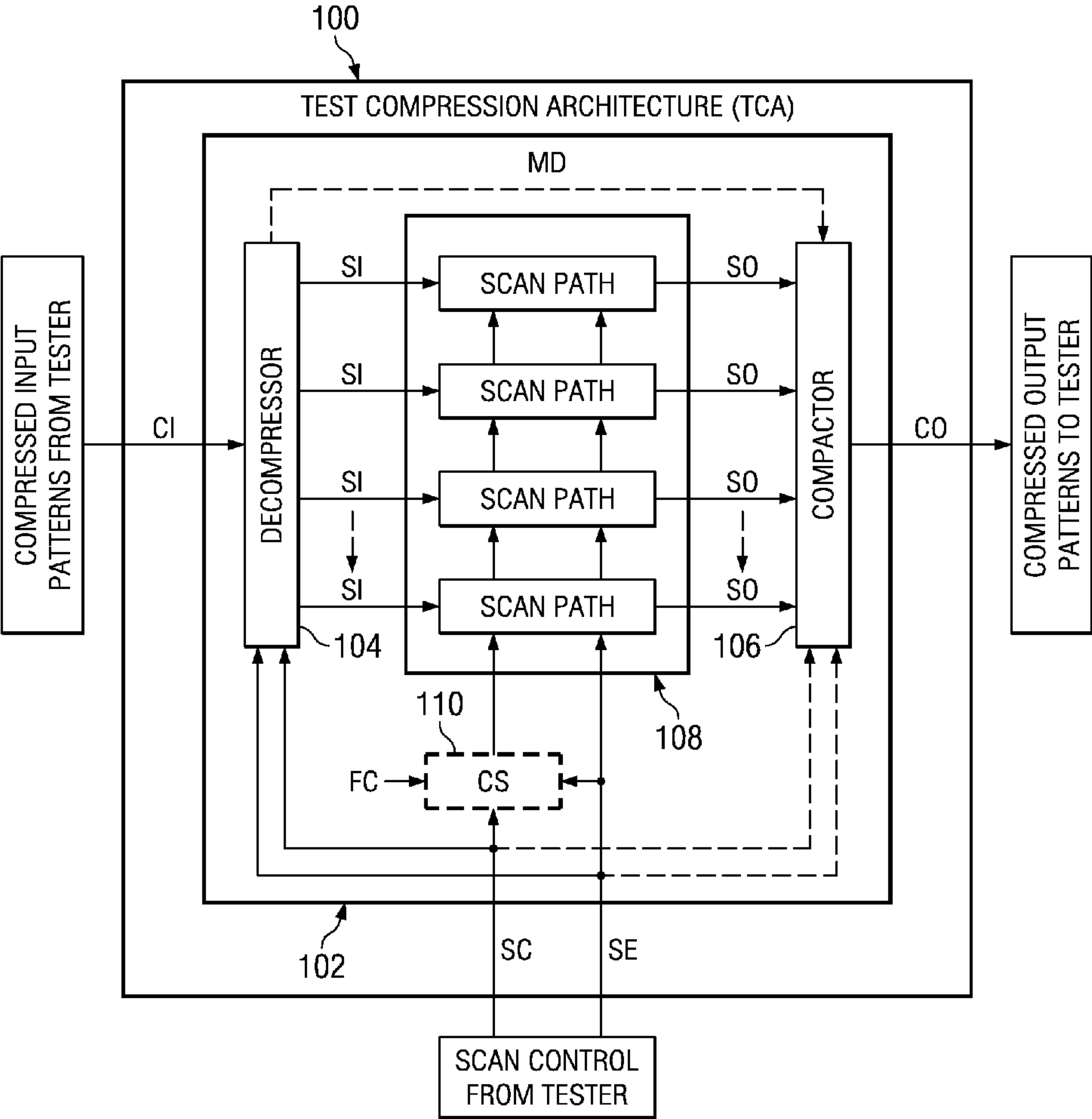
FIG. 1 (PRIOR ART)
