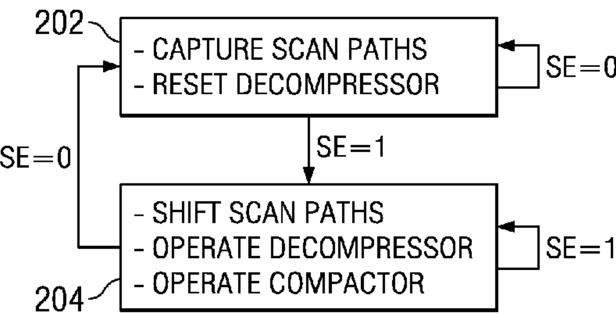
FIG. 2 (PRIOR ART)
