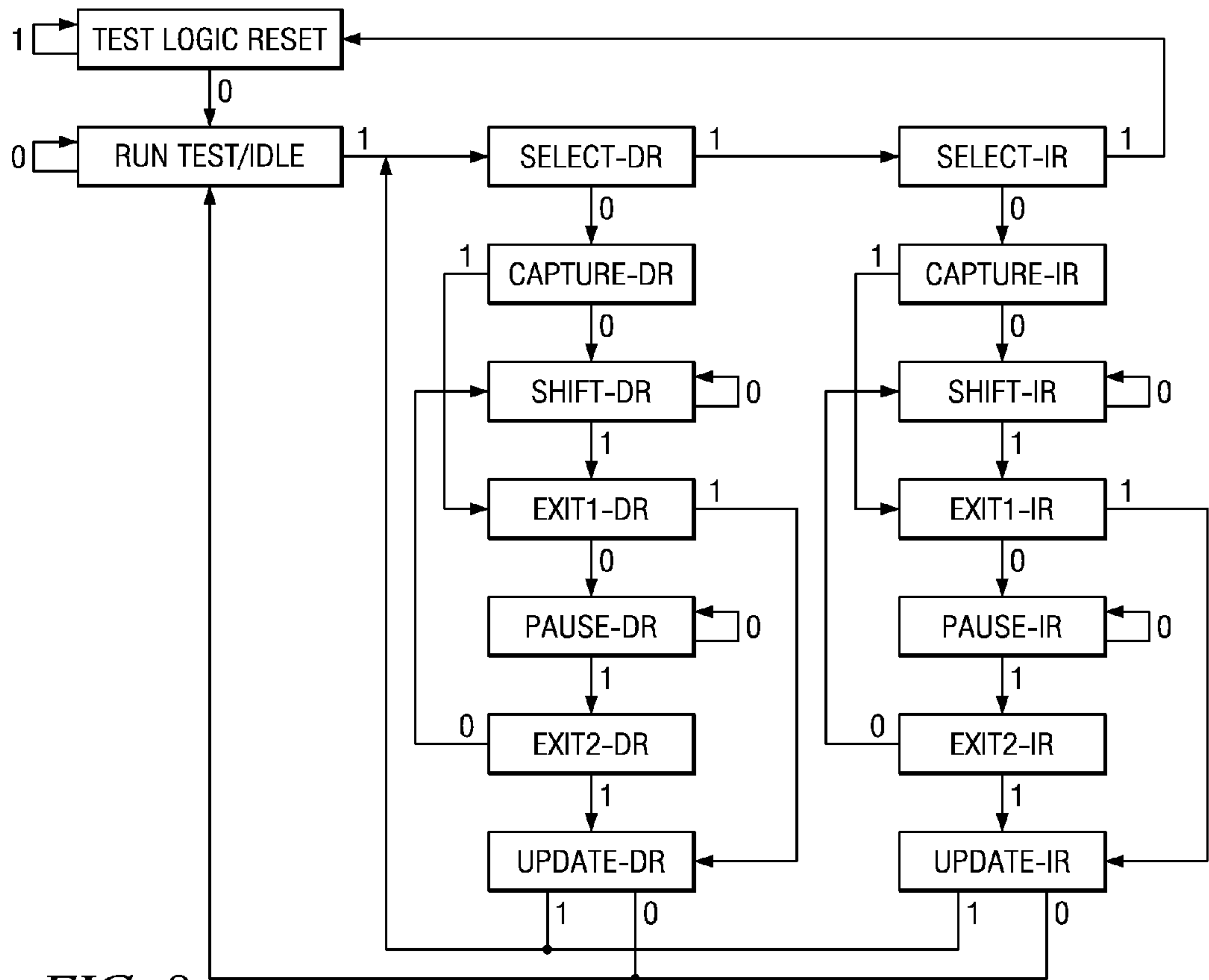
FIG. 8 (PRIOR ART)
