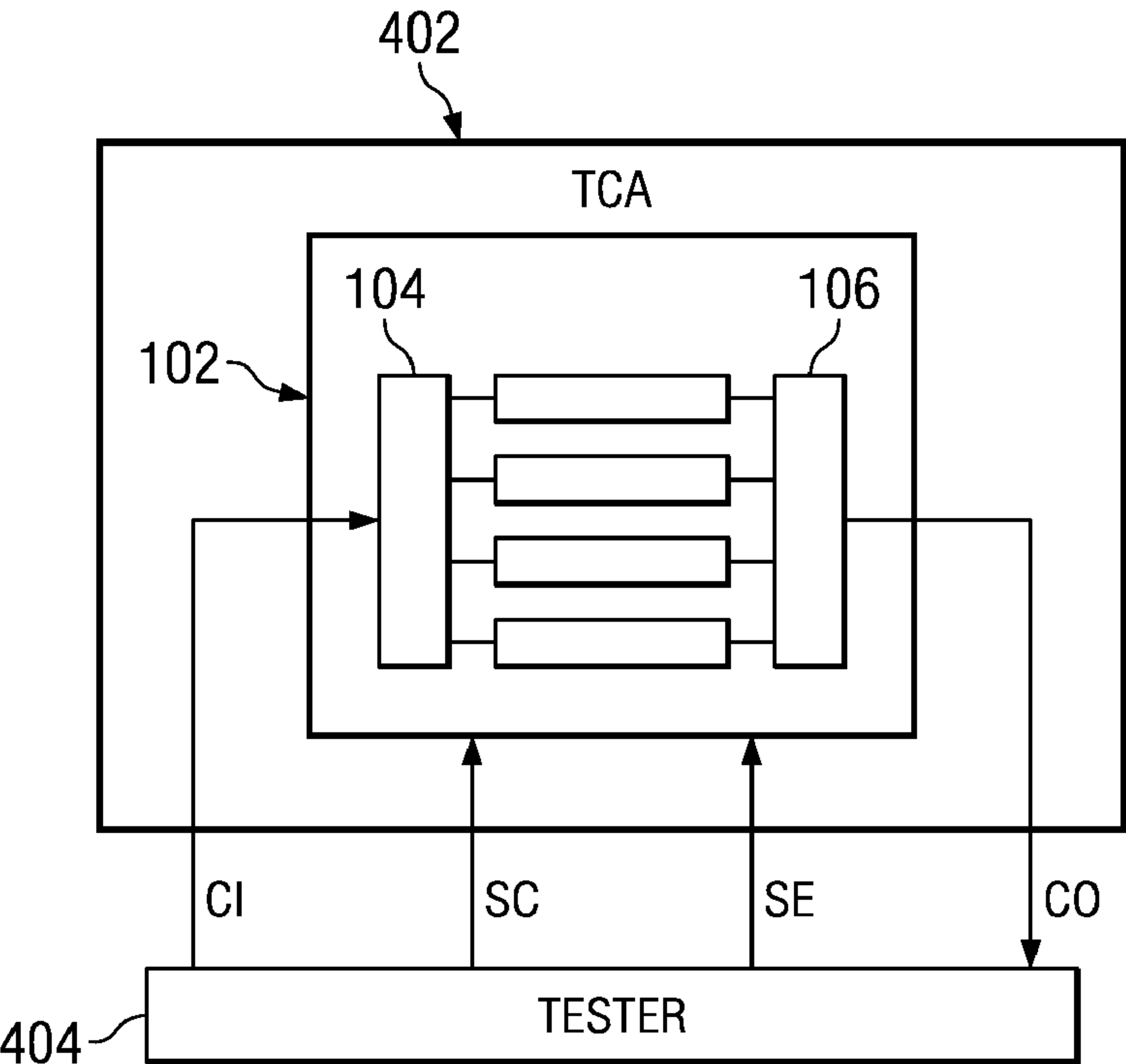
FIG. 4 (PRIOR ART)
