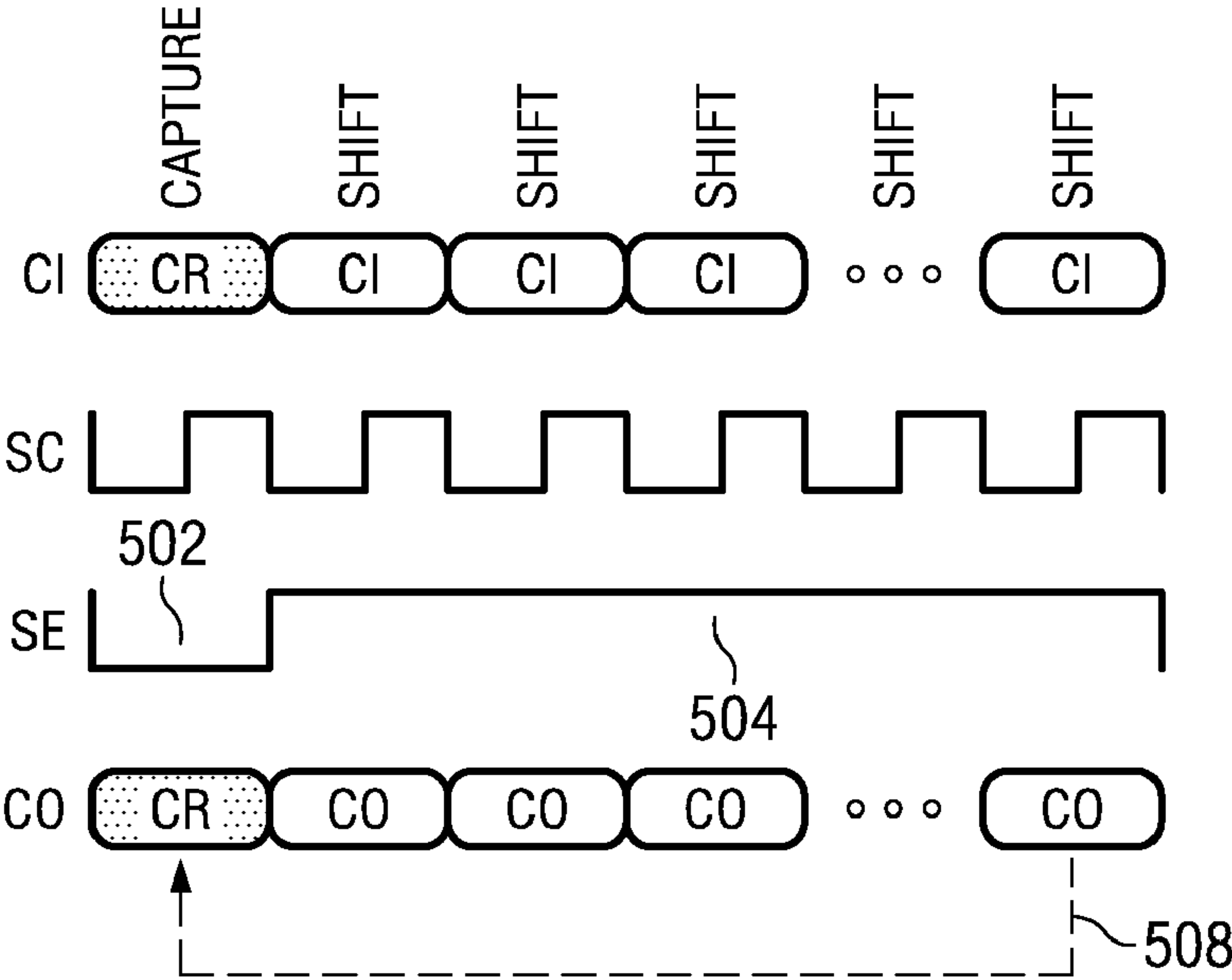
FIG. 5 (PRIOR ART)
