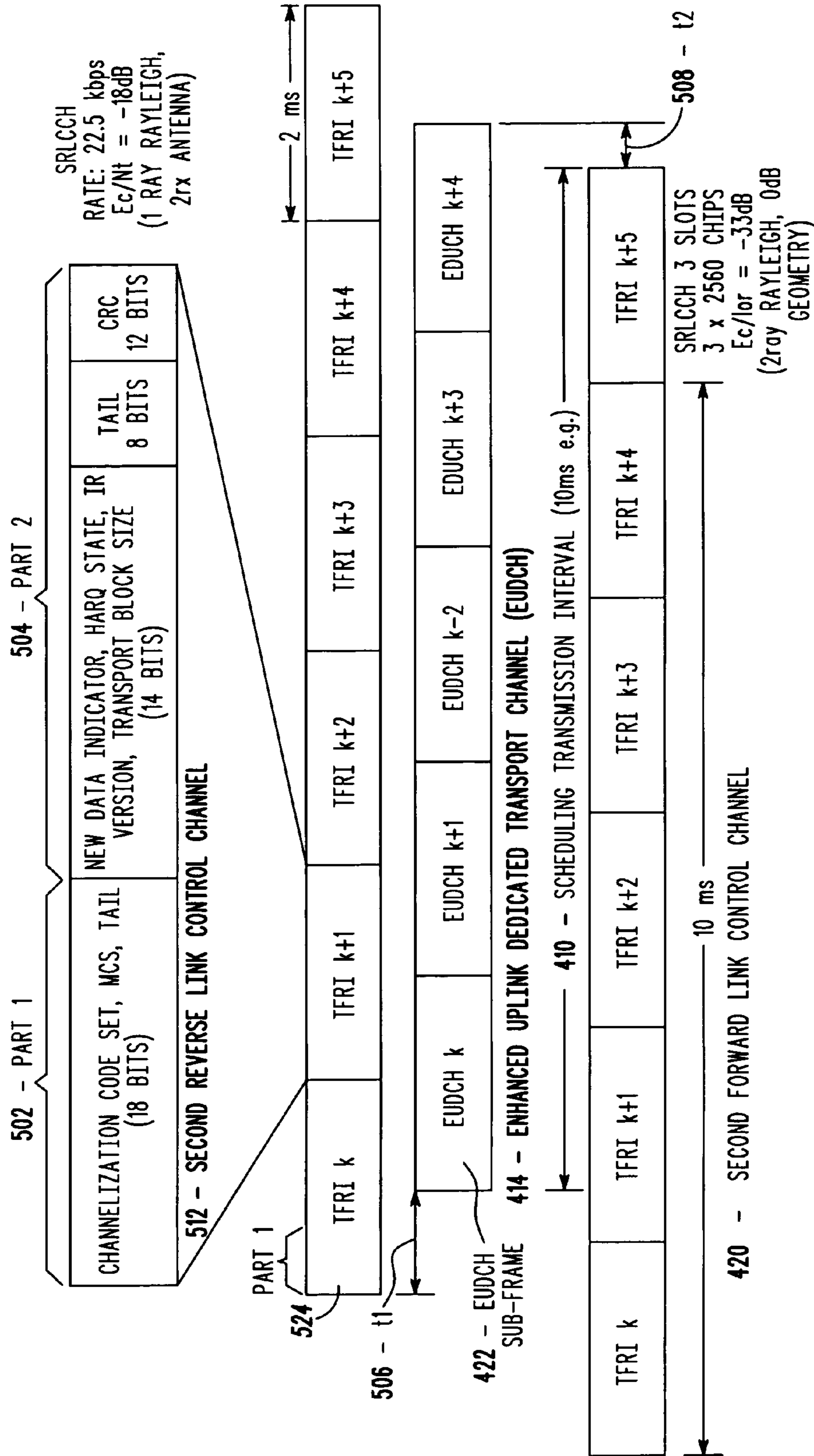
FIG. 5A SECOND REVERSE LINK CONTROL CHANNEL WITH FIRST AND SECOND PARTS
