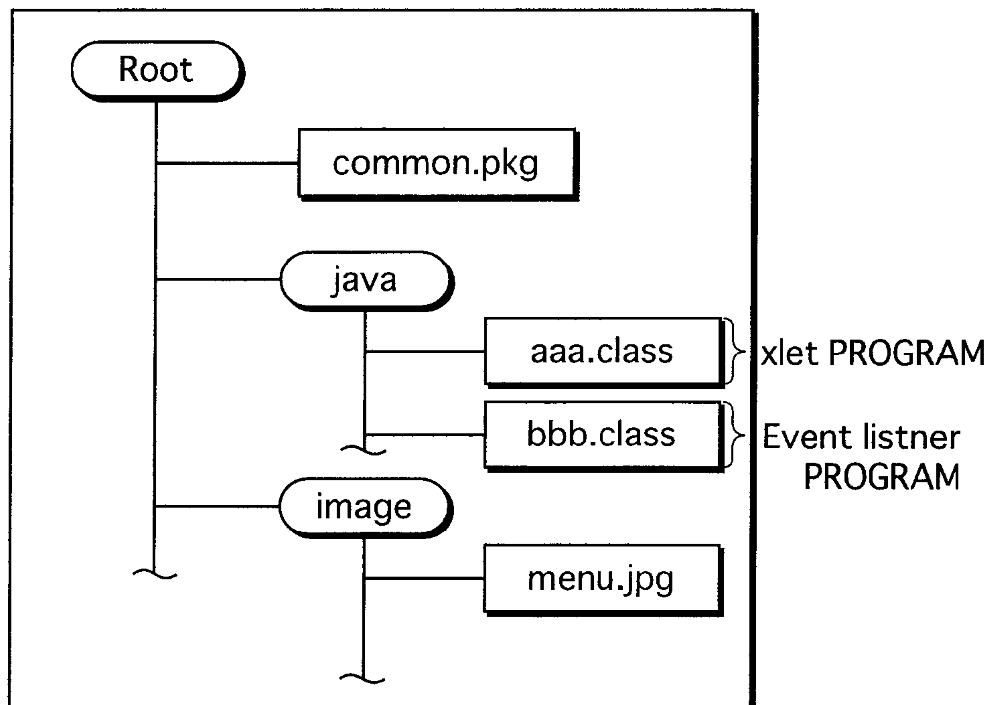
JAR FILE
