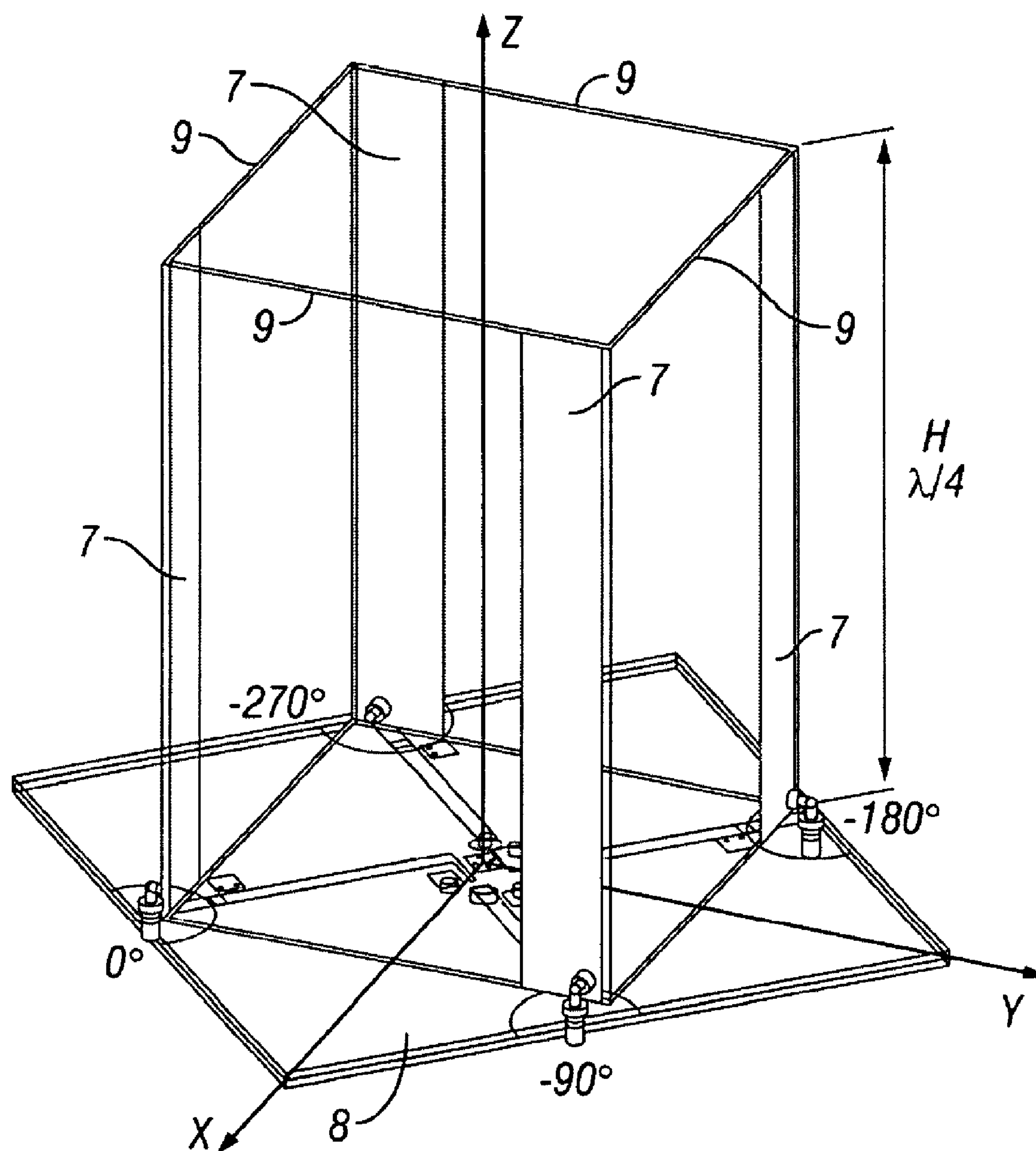
FIG. 4 (Prior Art)
