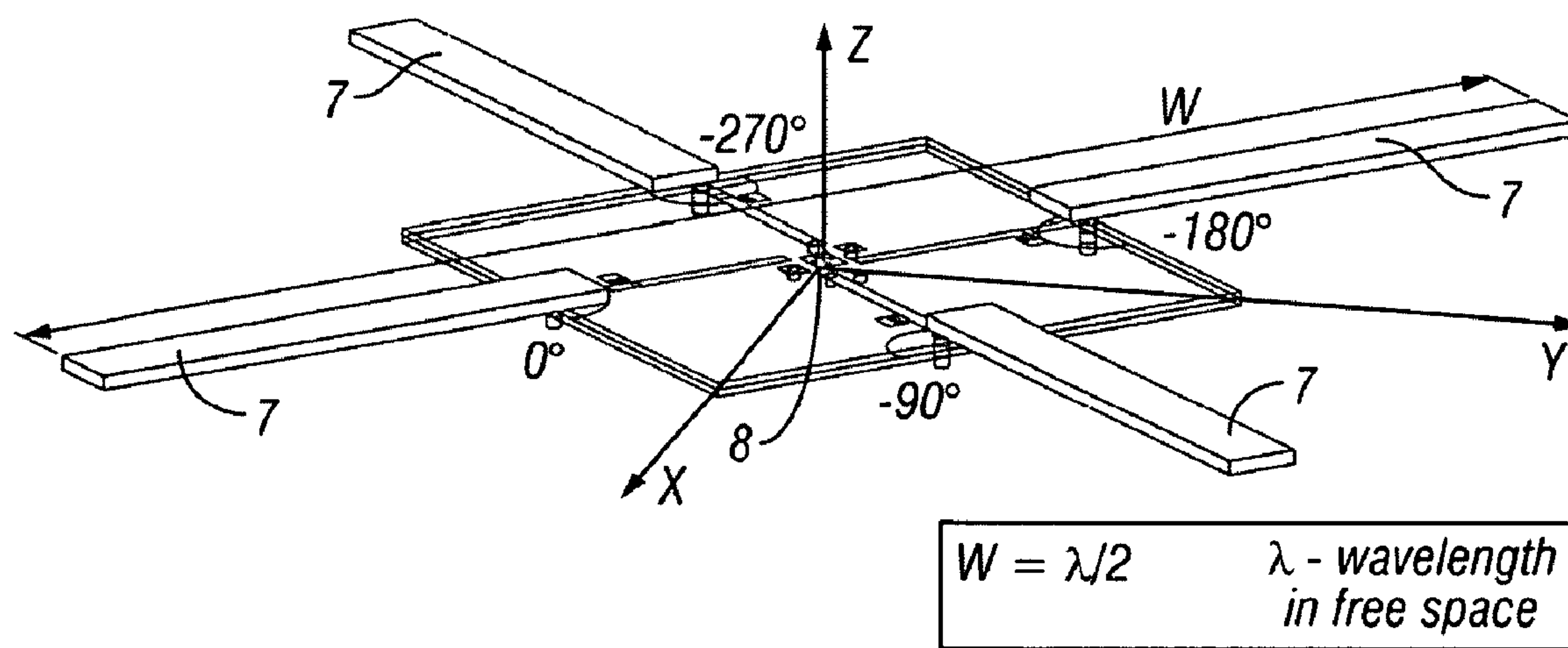
FIG. 2 (Prior Art)
