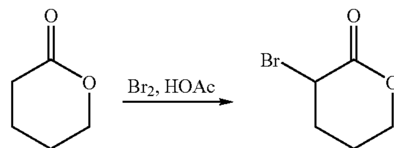
Scheme 12A
