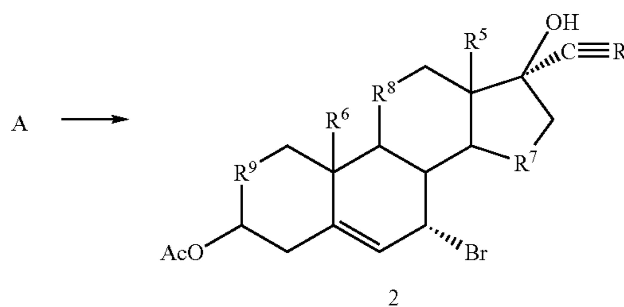
Scheme 2
