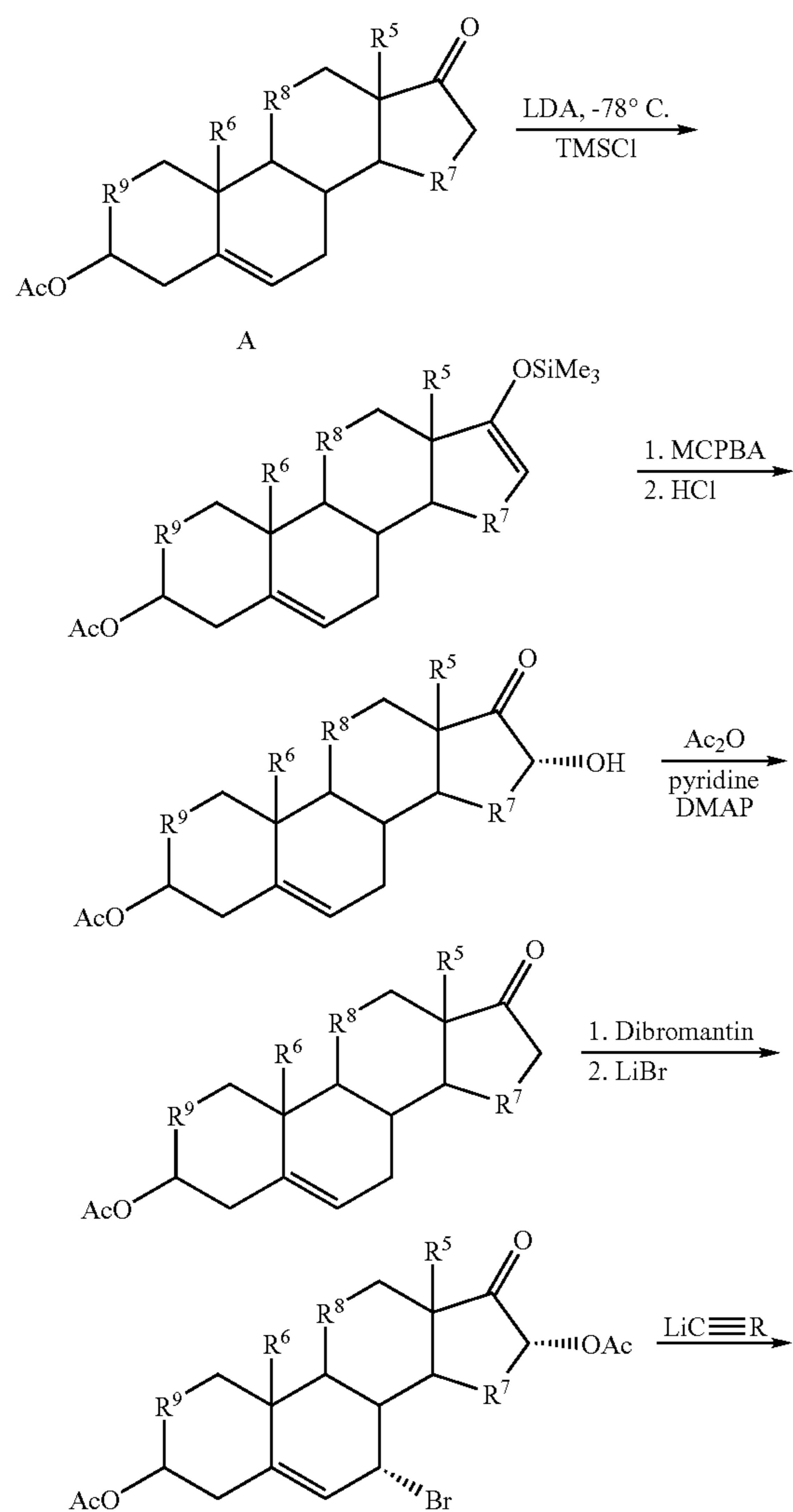
Scheme 1
