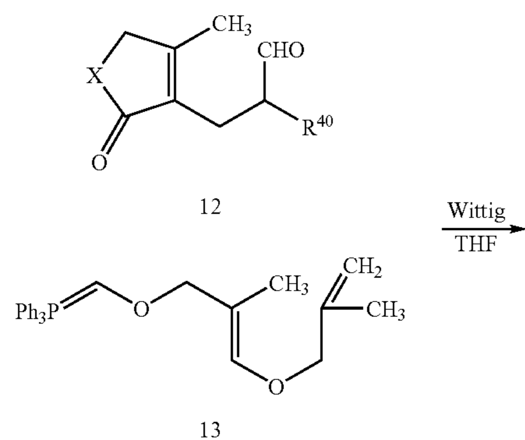
Scheme 11
