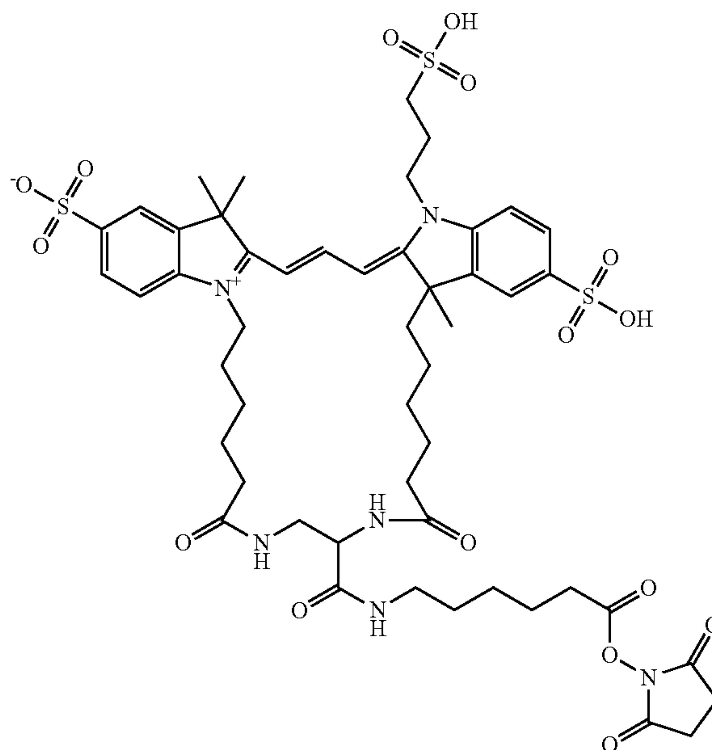
Compound 20
