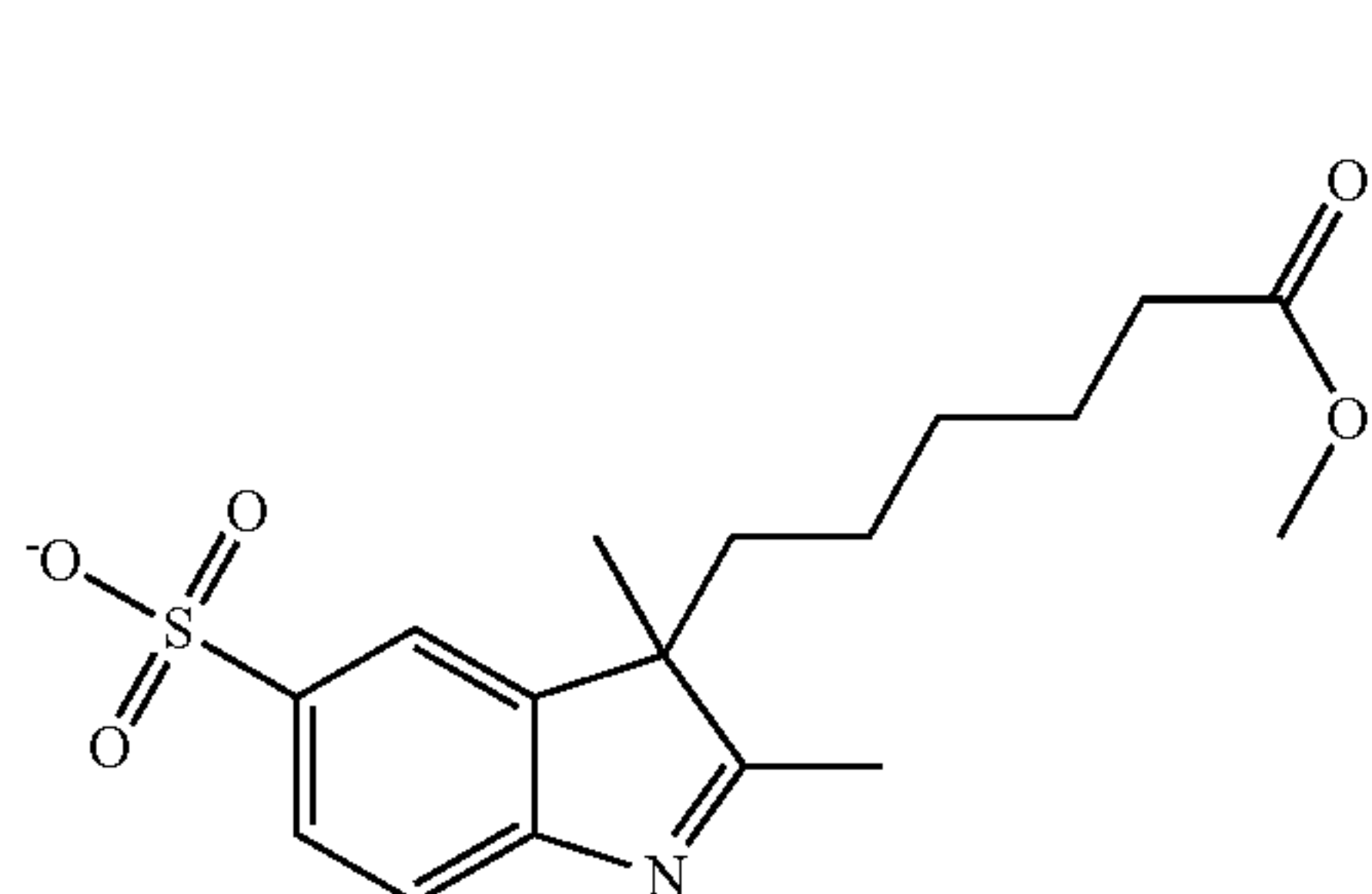
Compound 5
