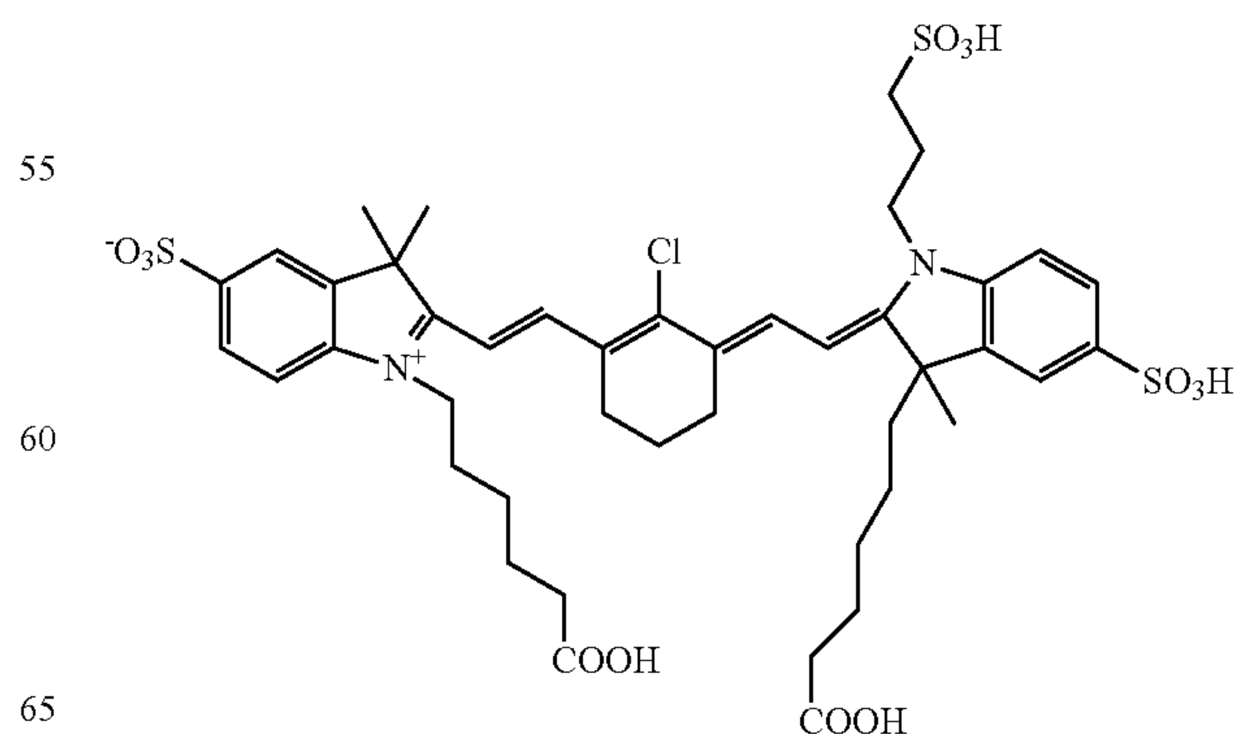
Compound 32
