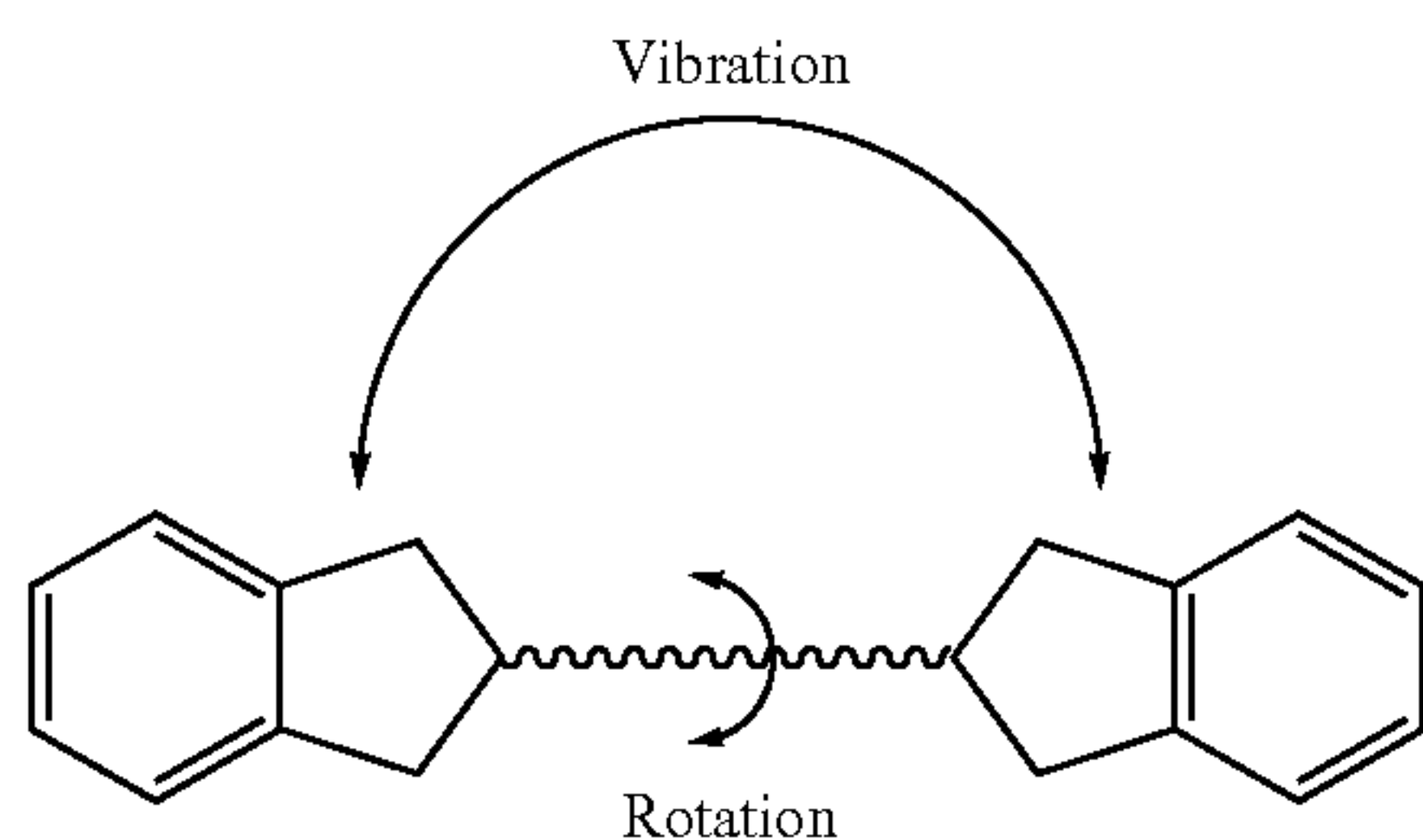
Scheme 1. 'Loose Belt Effect' through vibration and rotation around the middle conjugated double bonds
