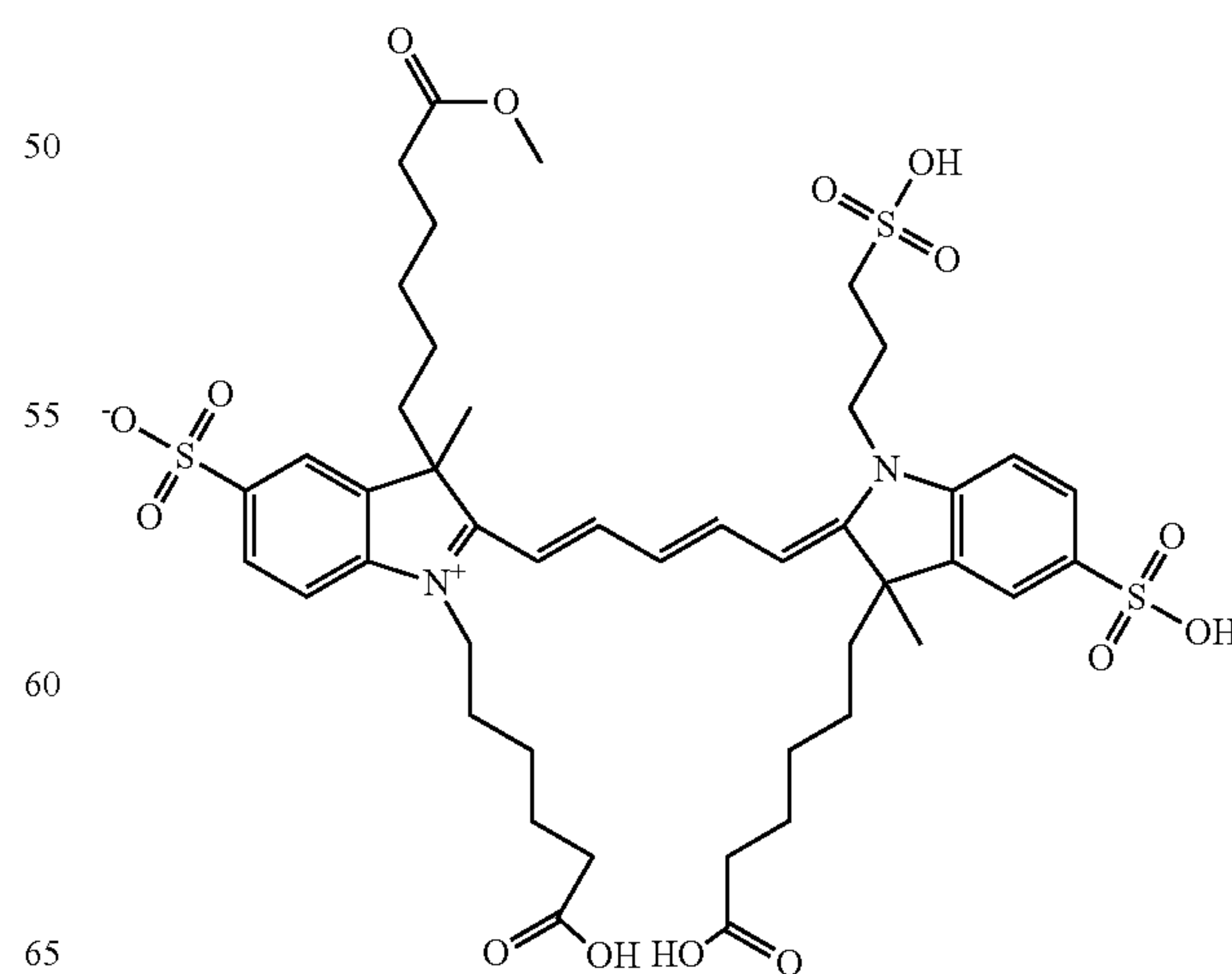
Compound 15
