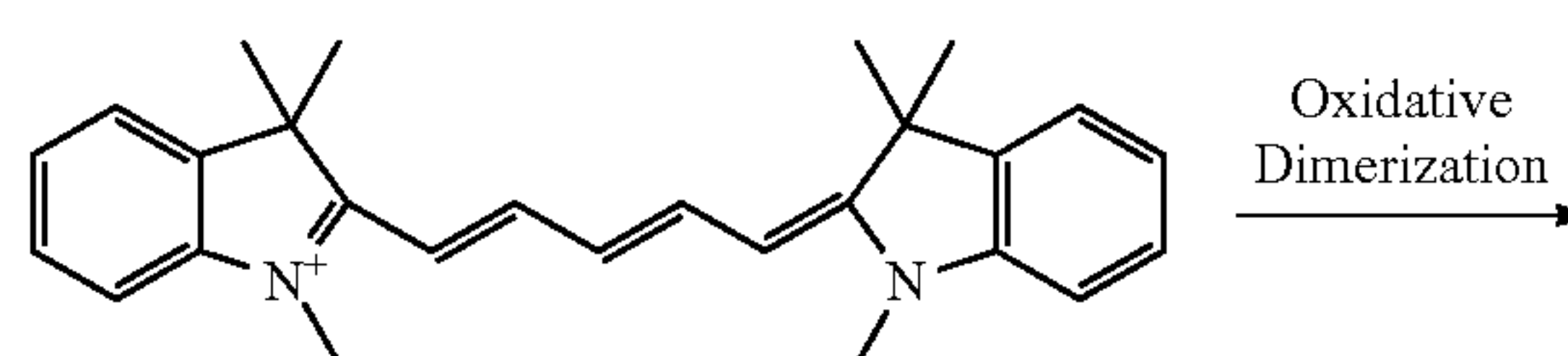
Scheme 2. Oxidative dimerization of carbocyanines
