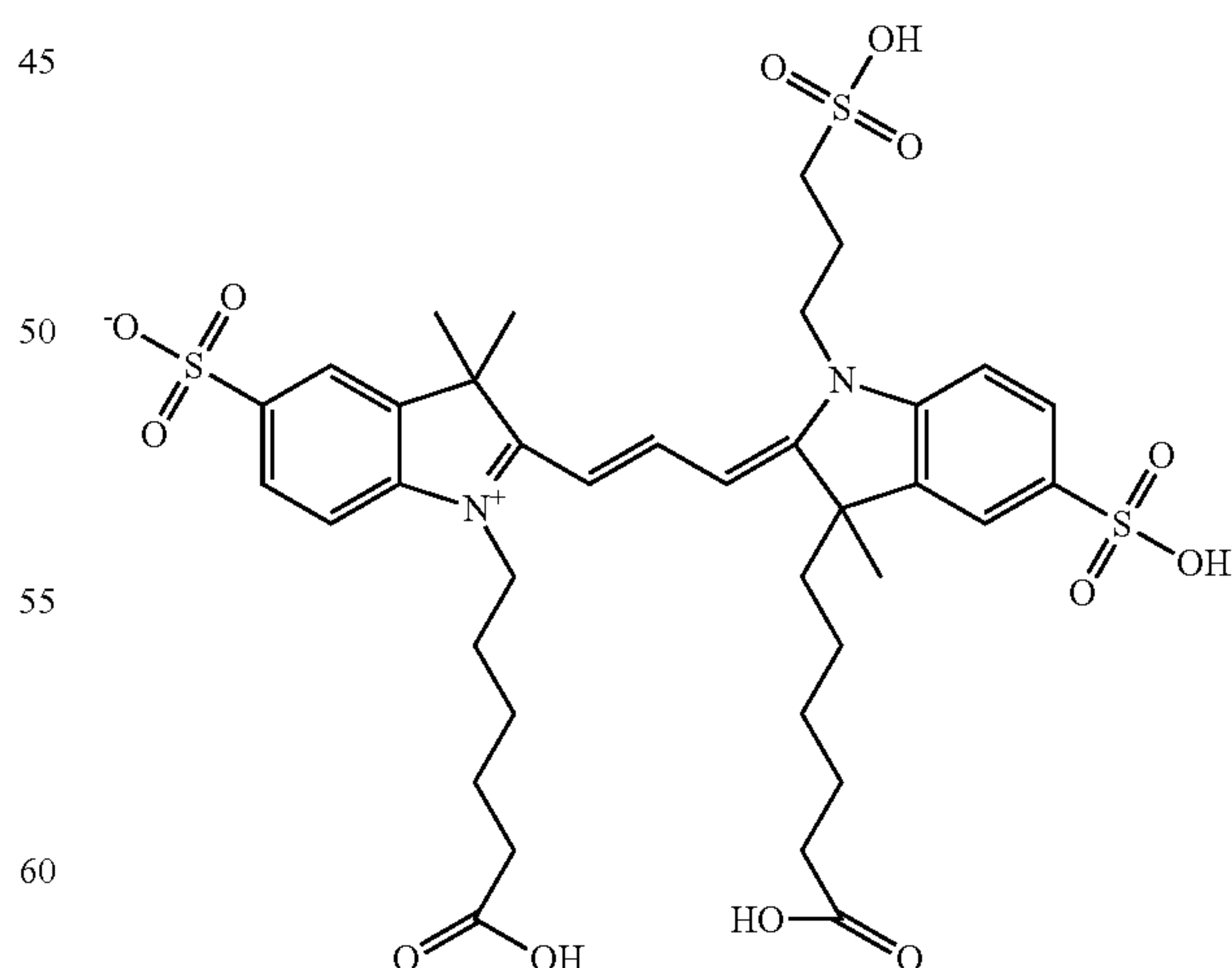
Compound 18
