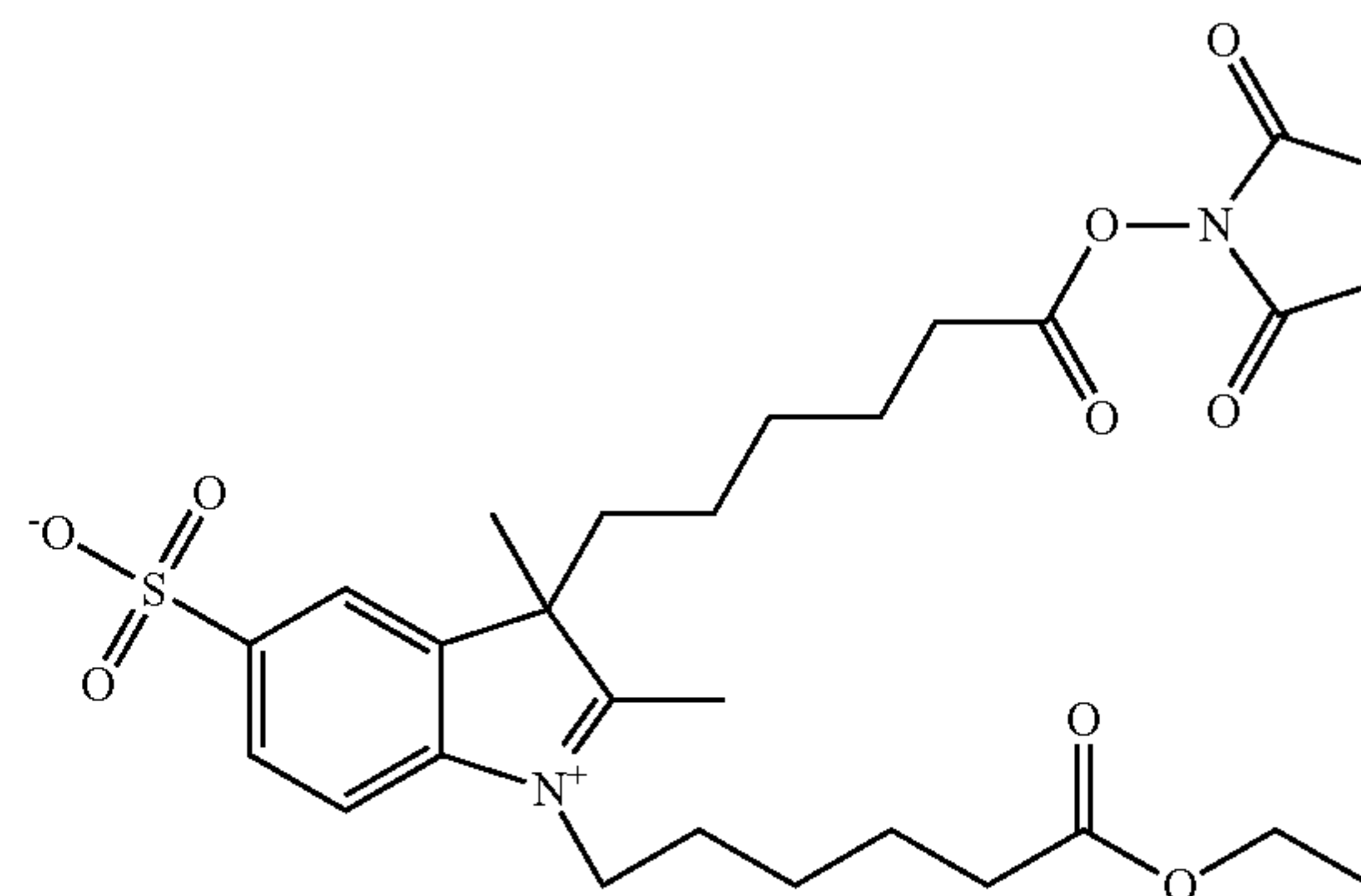
Compound 39
