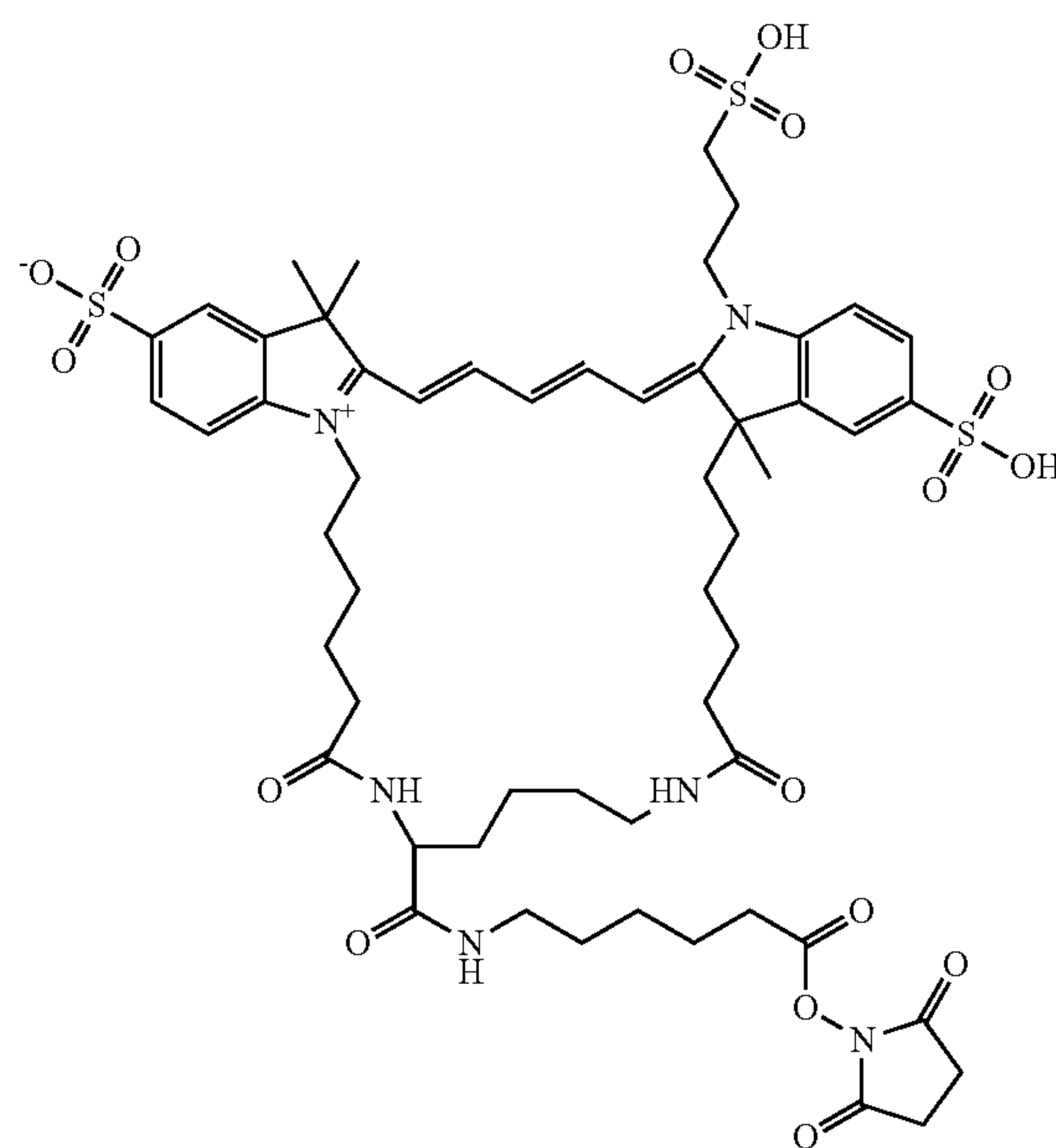
Compound 14
