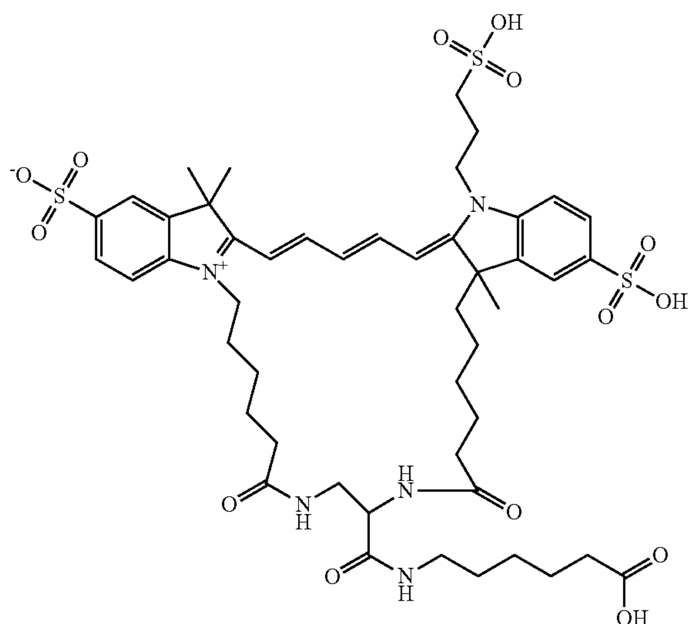
Compound 19
