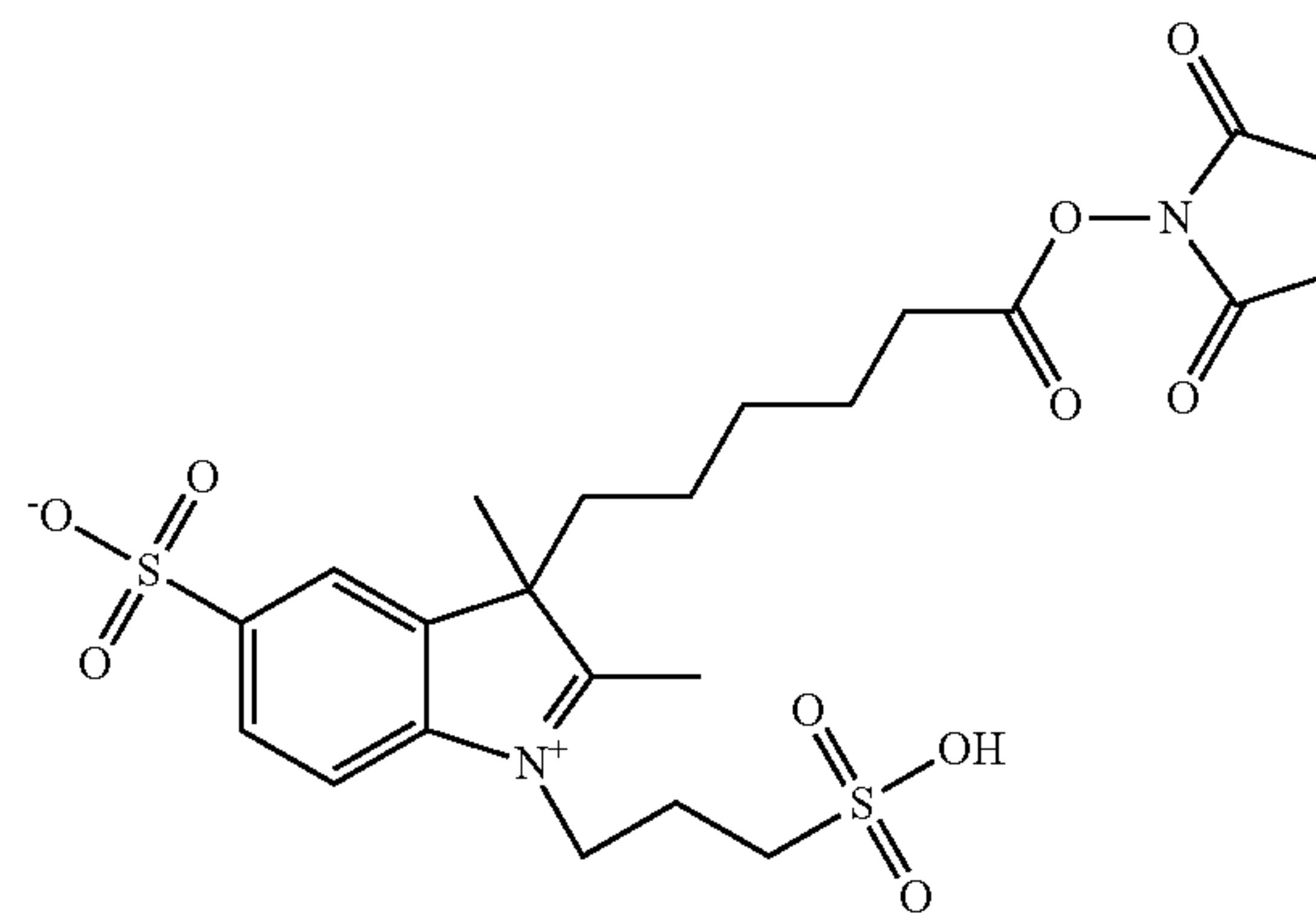
Compound 40
