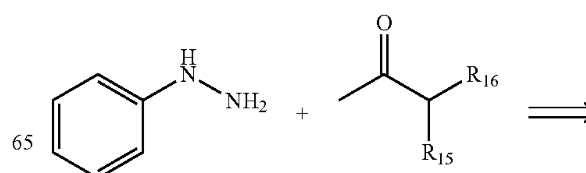
Scheme 3. Typical synthesis of indolium intermediate
