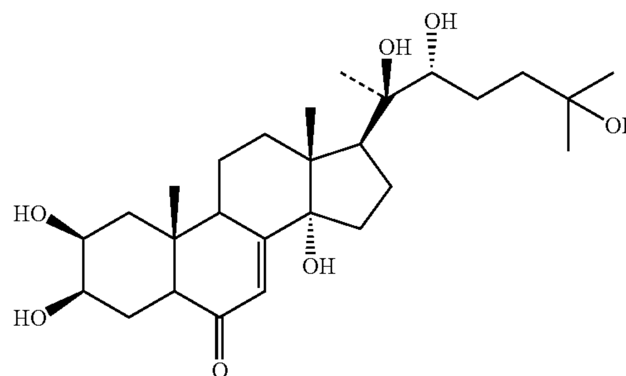
20-hydroxyecdysone
