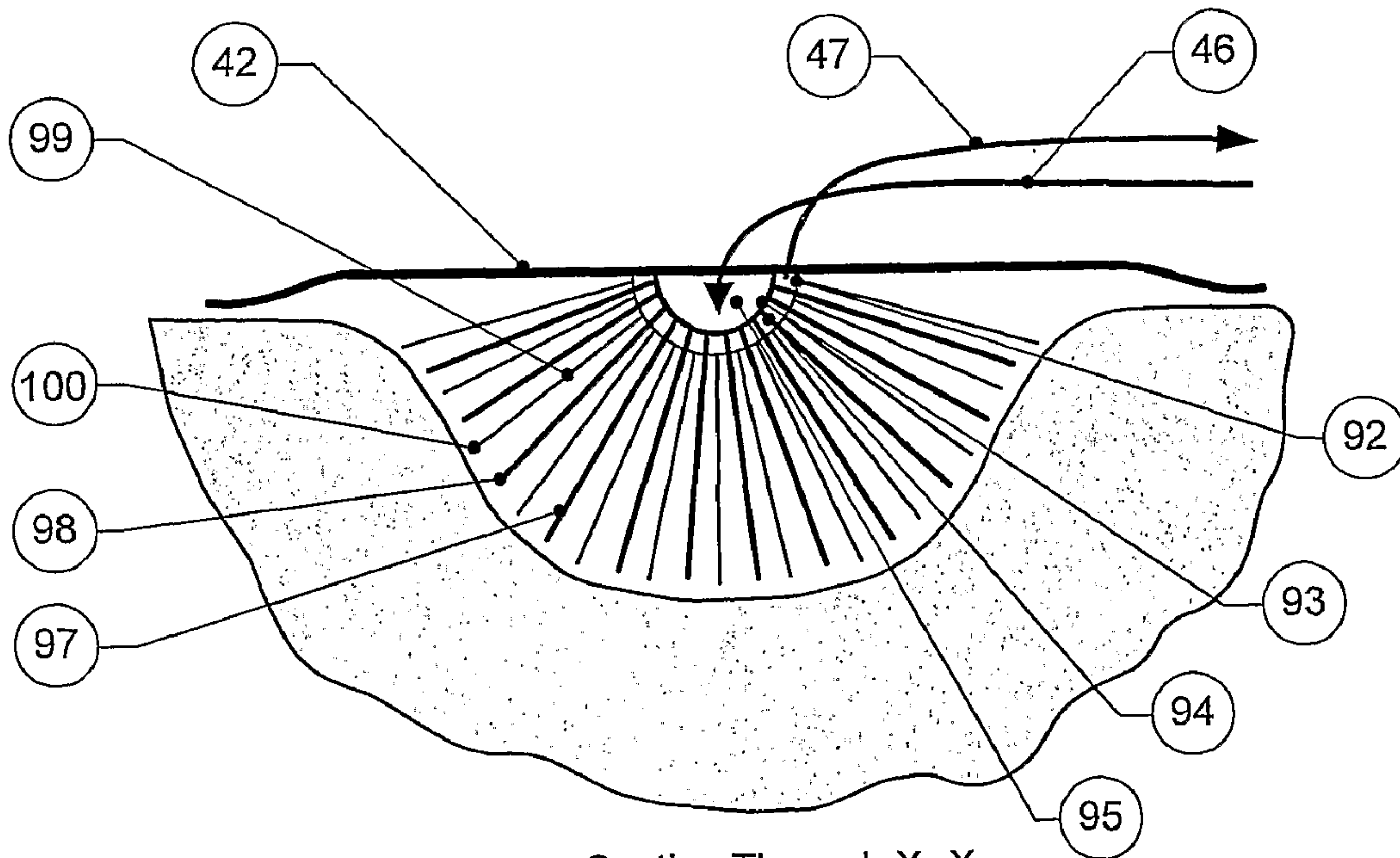
Section Through X-X
