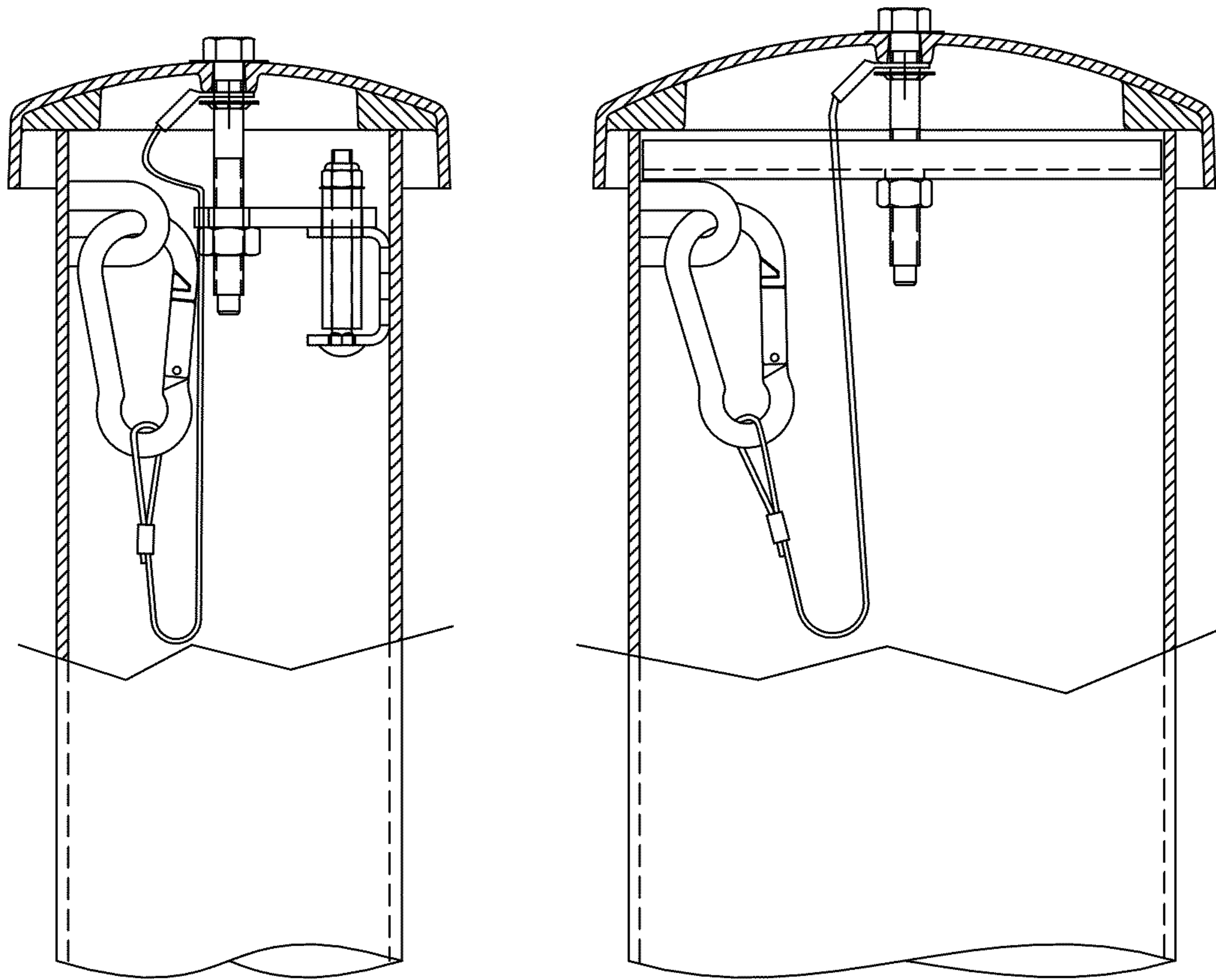
DETAIL B
