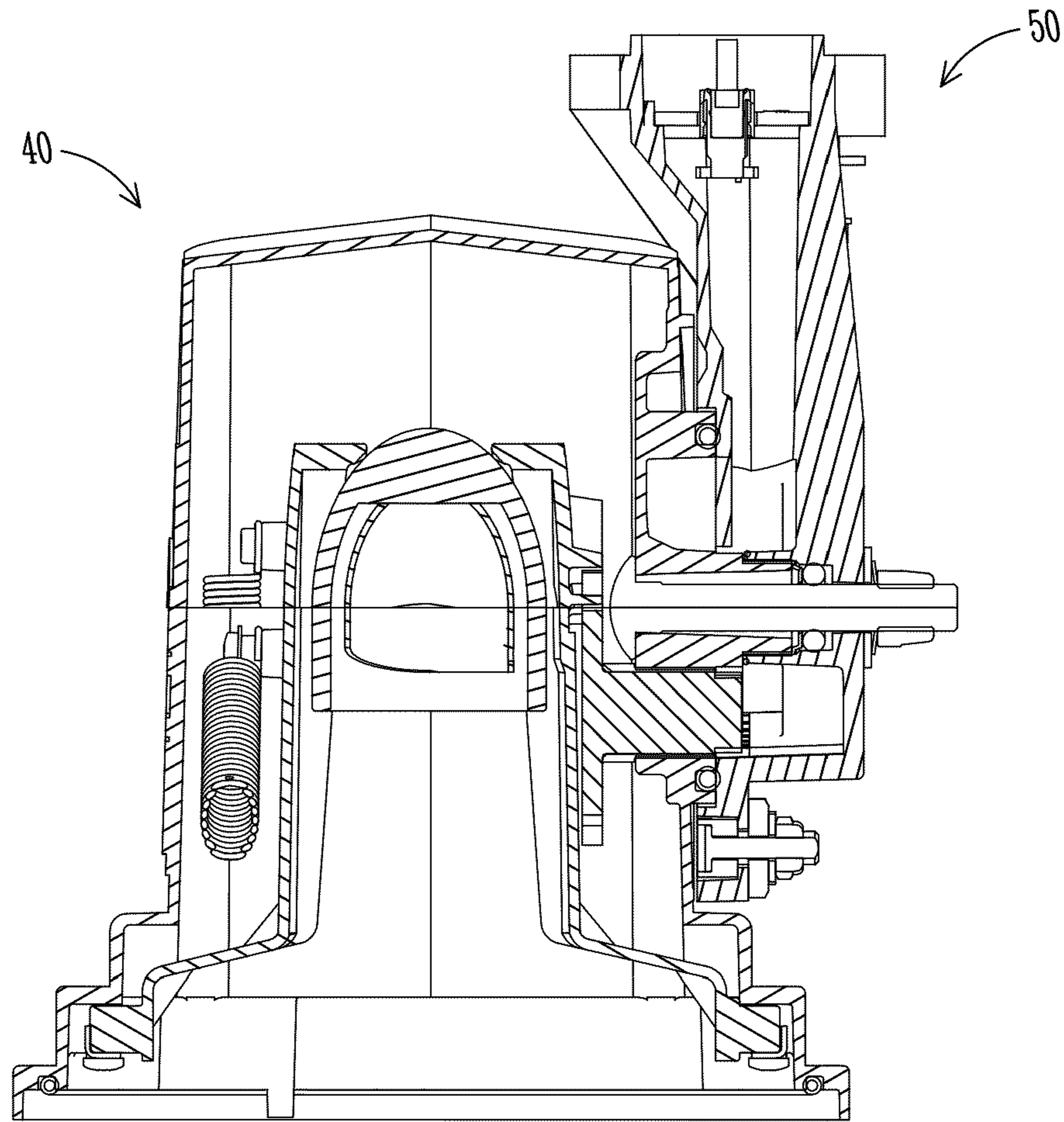
SECTION G-G
