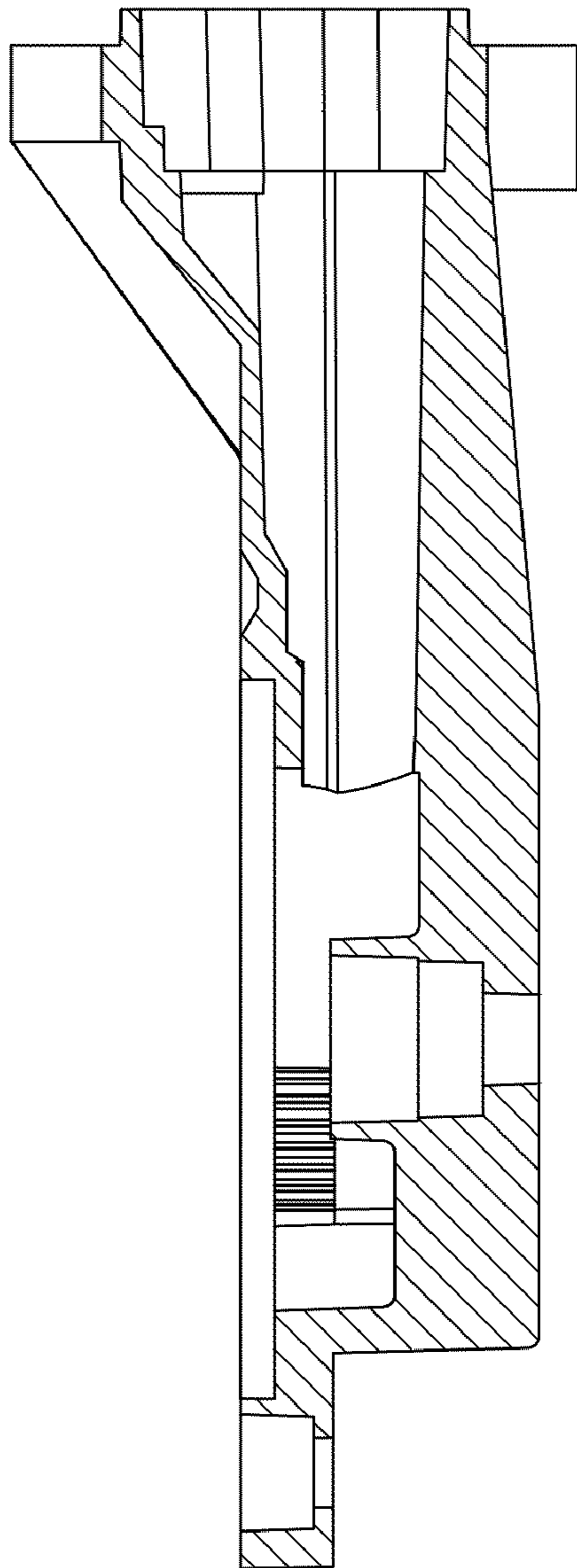
SECTION J-J
