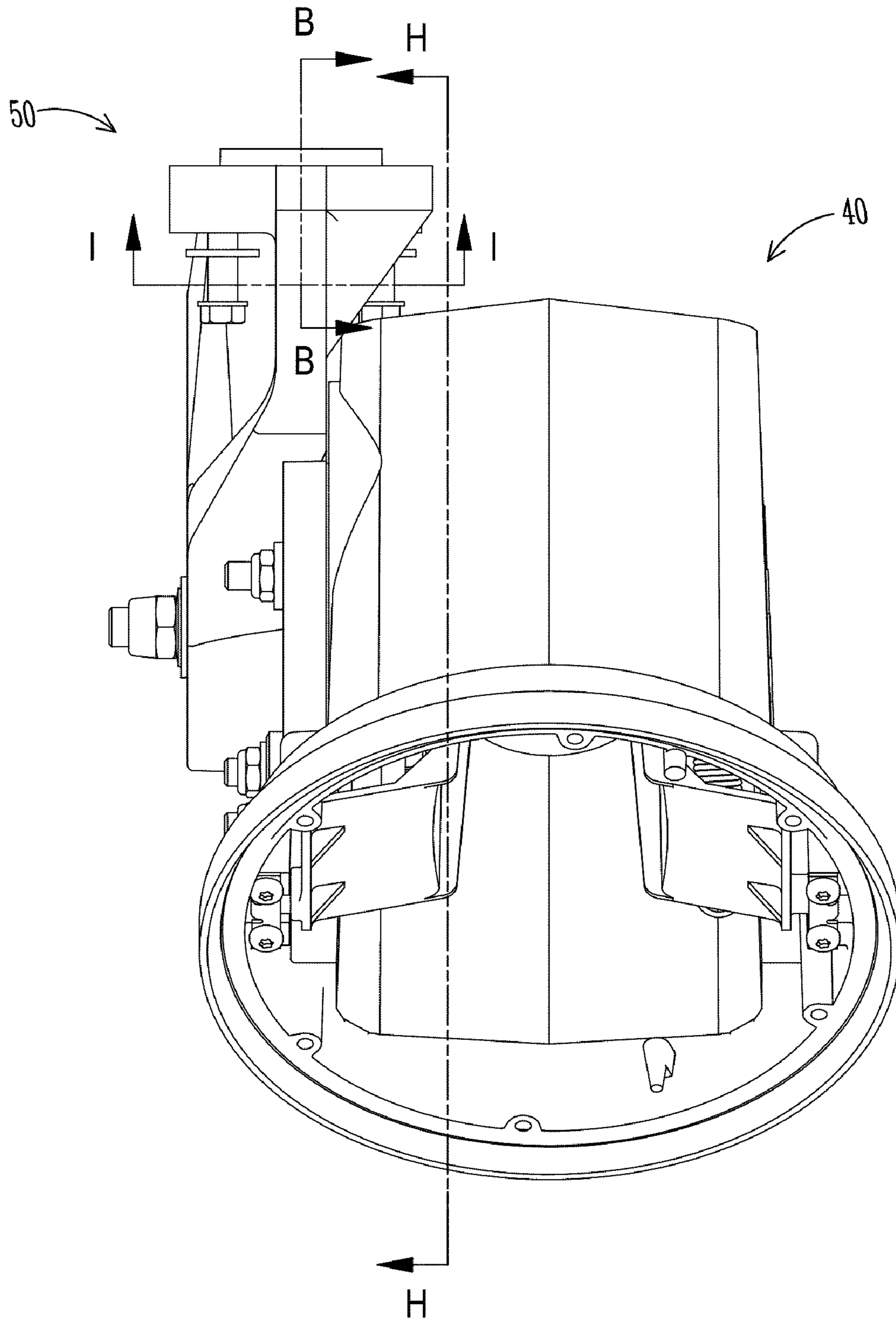
FRONT VIEW
