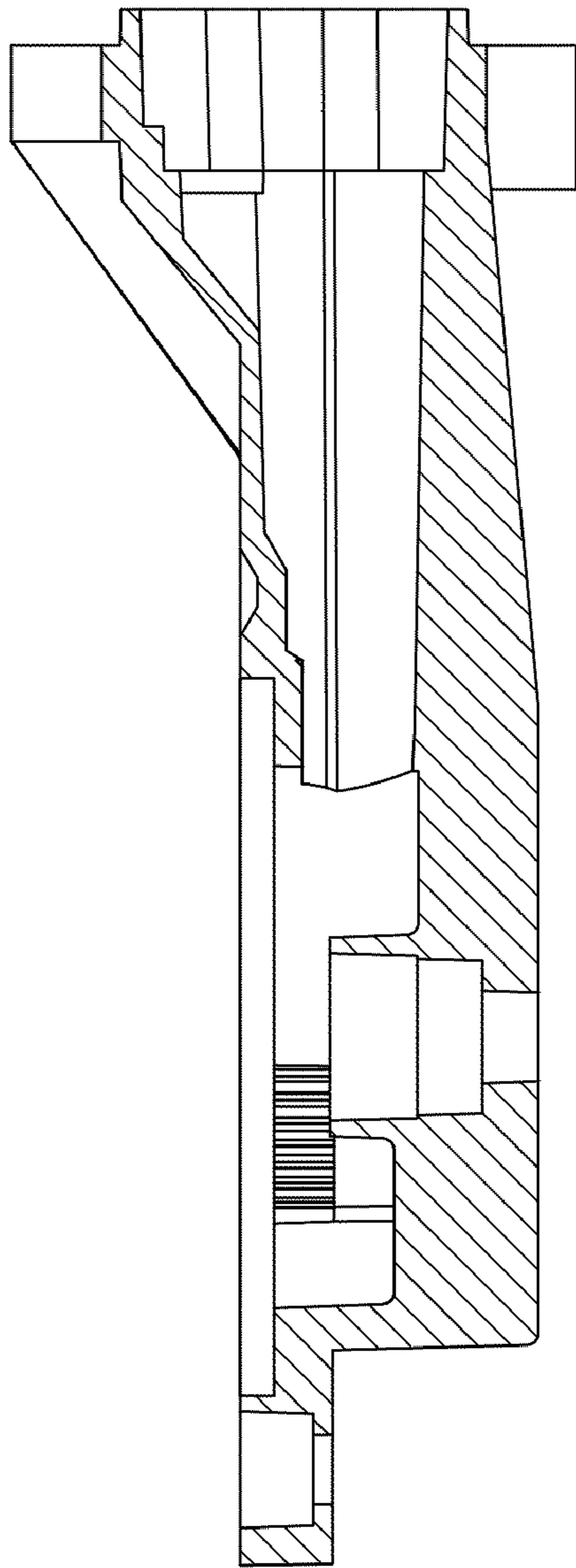
SECTION J-J
