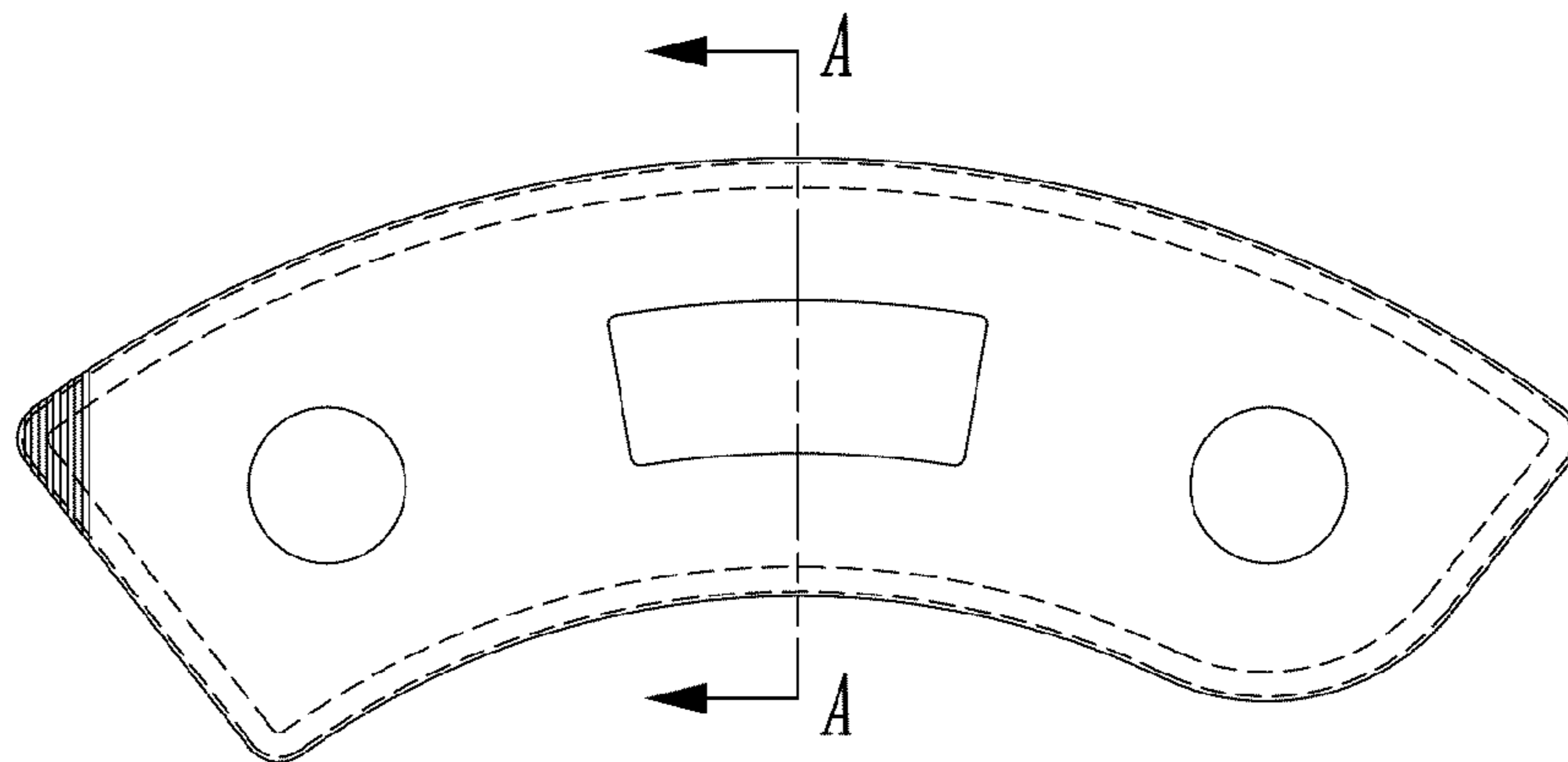
FRONT VIEW
