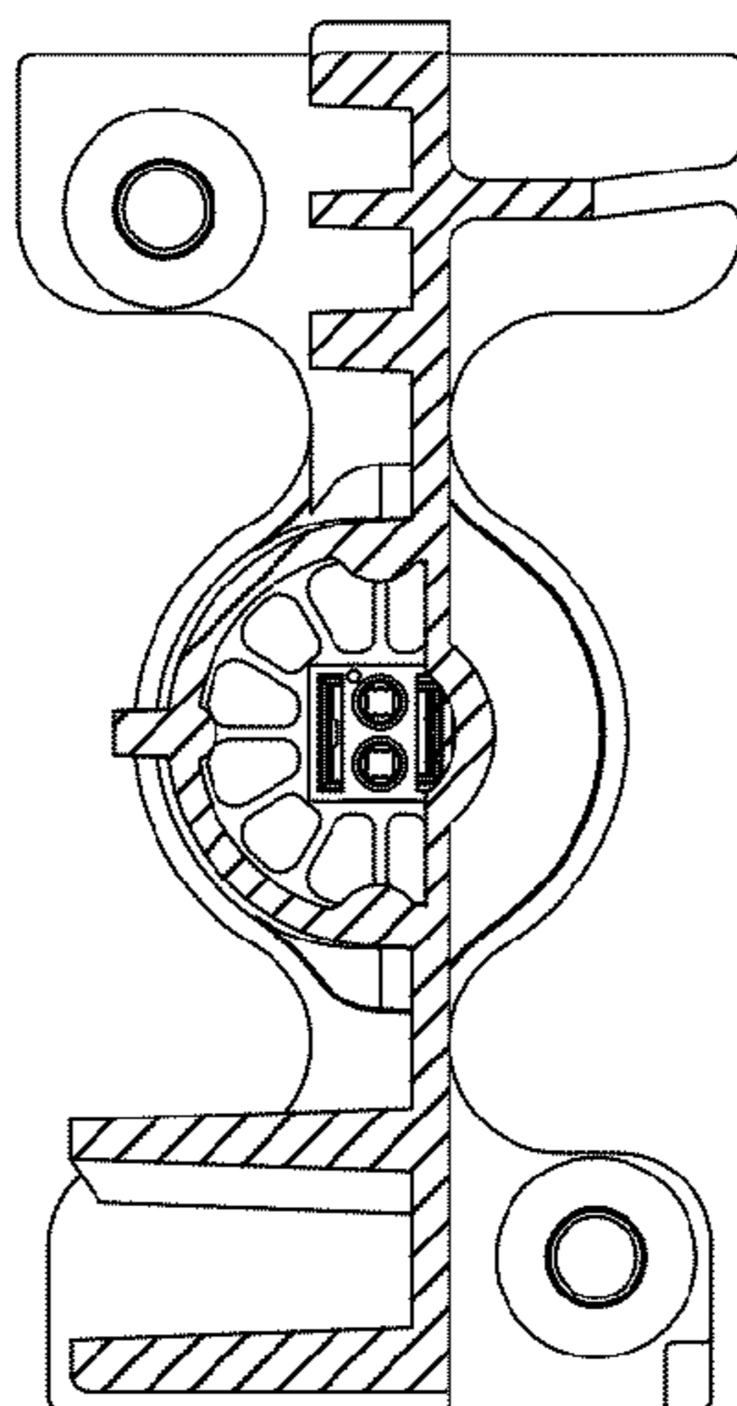
SECTION I-I
