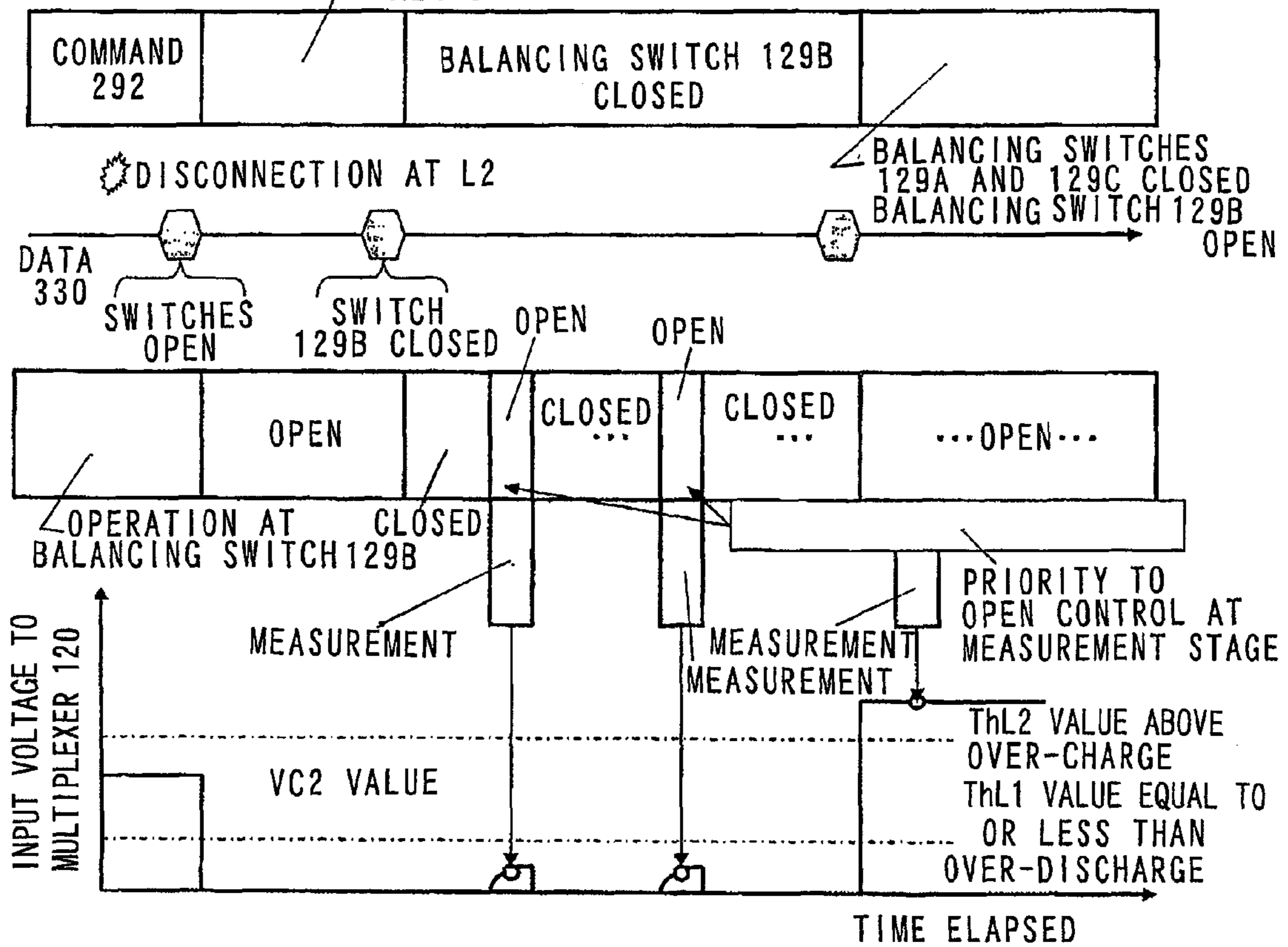
FIG.29 BALANCING SWITCHES 129 ALL OPEN
