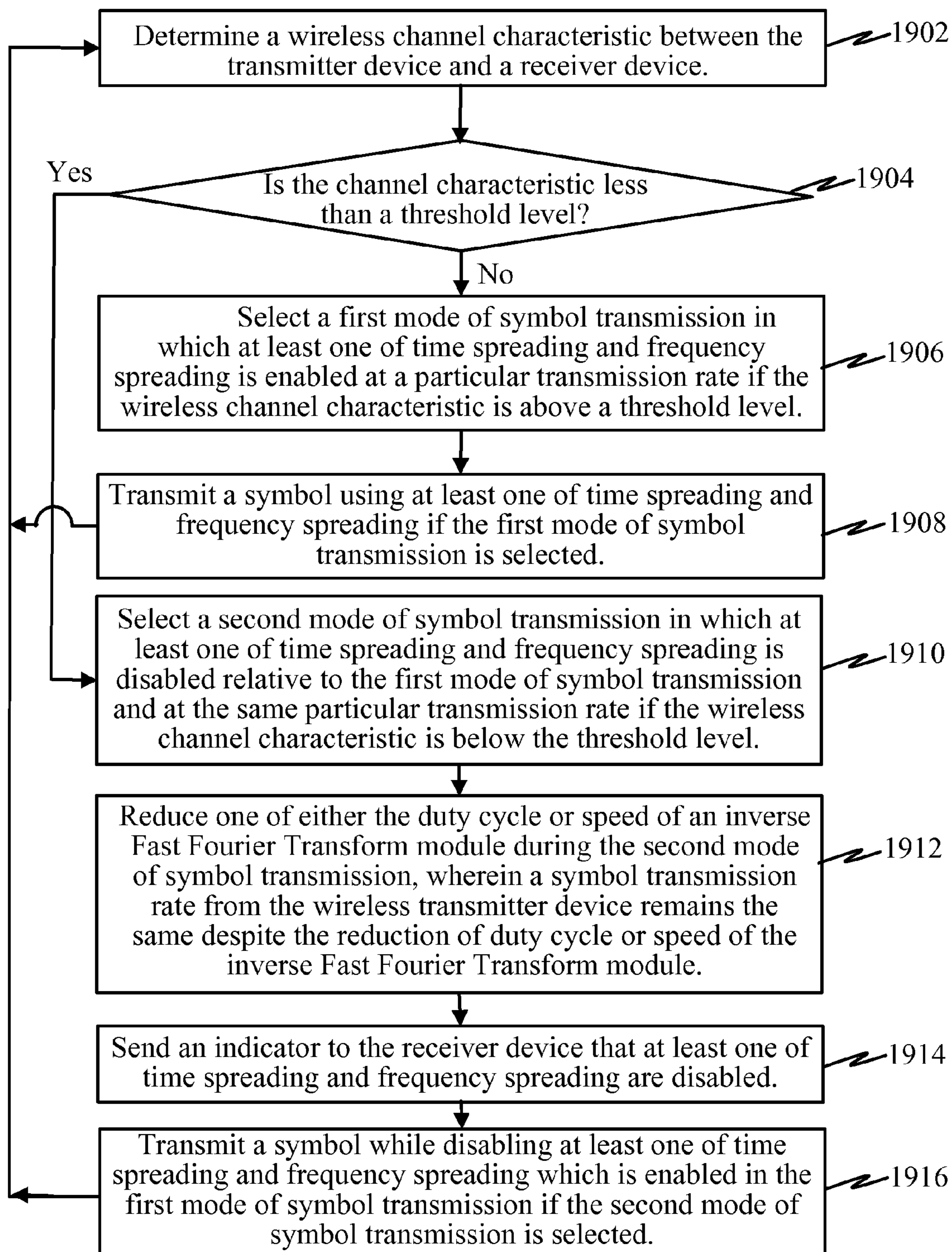
FIGURE 19 LOW-POWER TRANSMISSION METHOD
