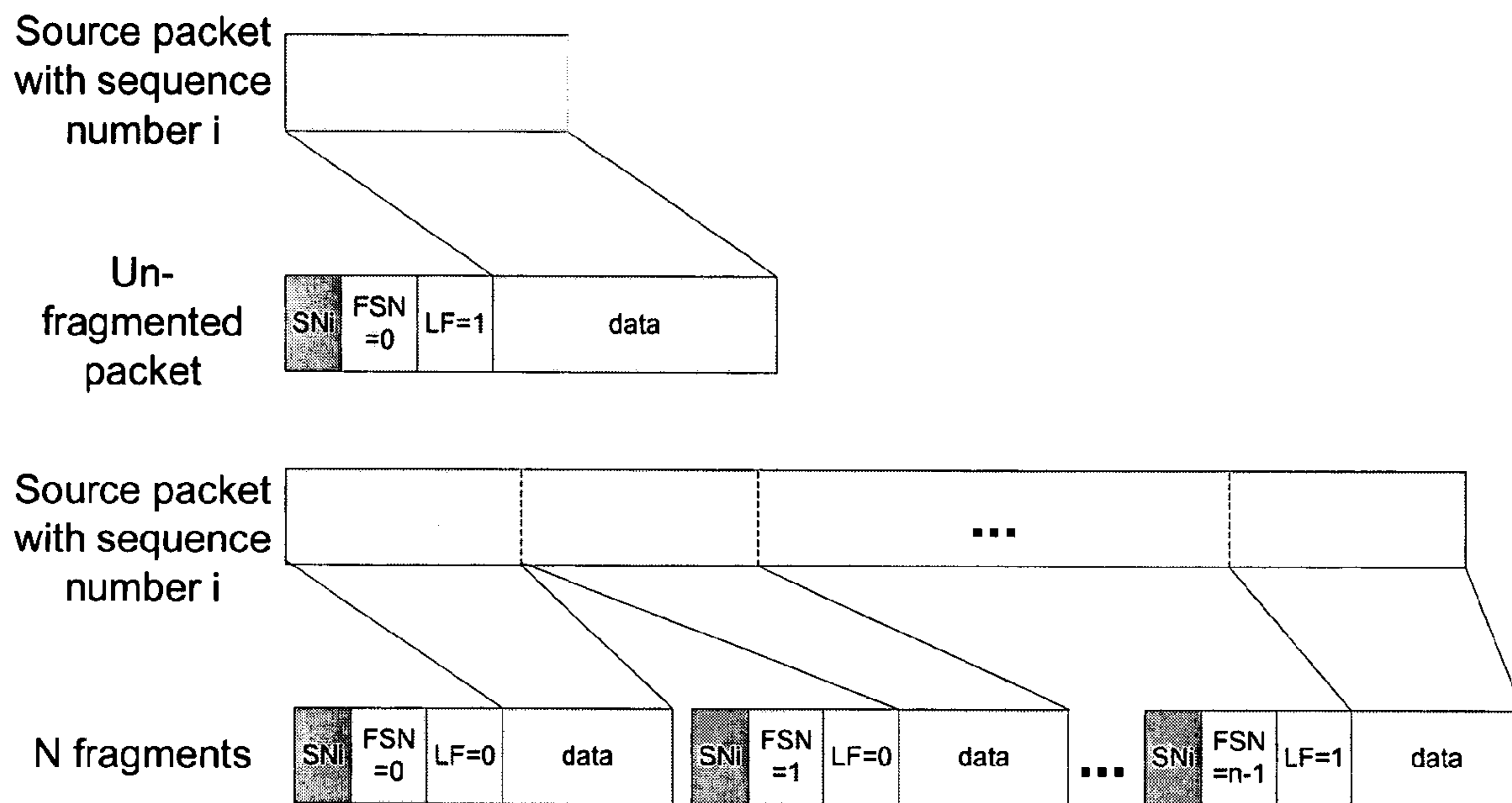
Figure 3 - SAR signaling by fragment numbering
