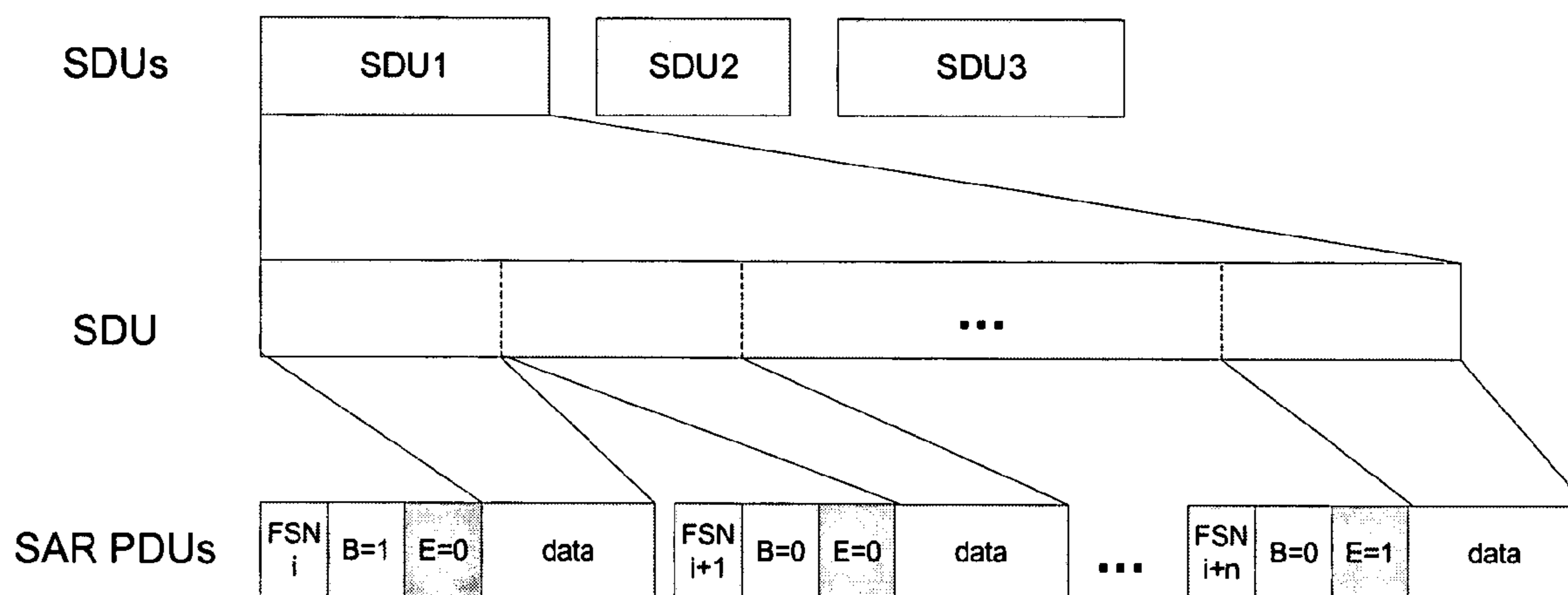
Figure 4 - SAR signaling with Beginning and End flags
