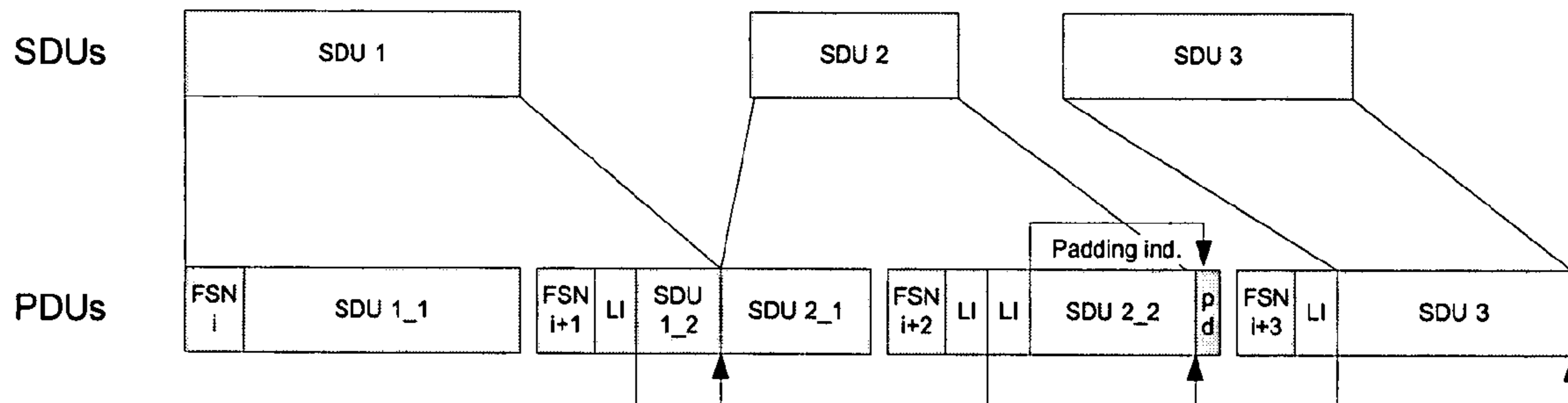
Figure 5 - SAR signaling with length indicators
