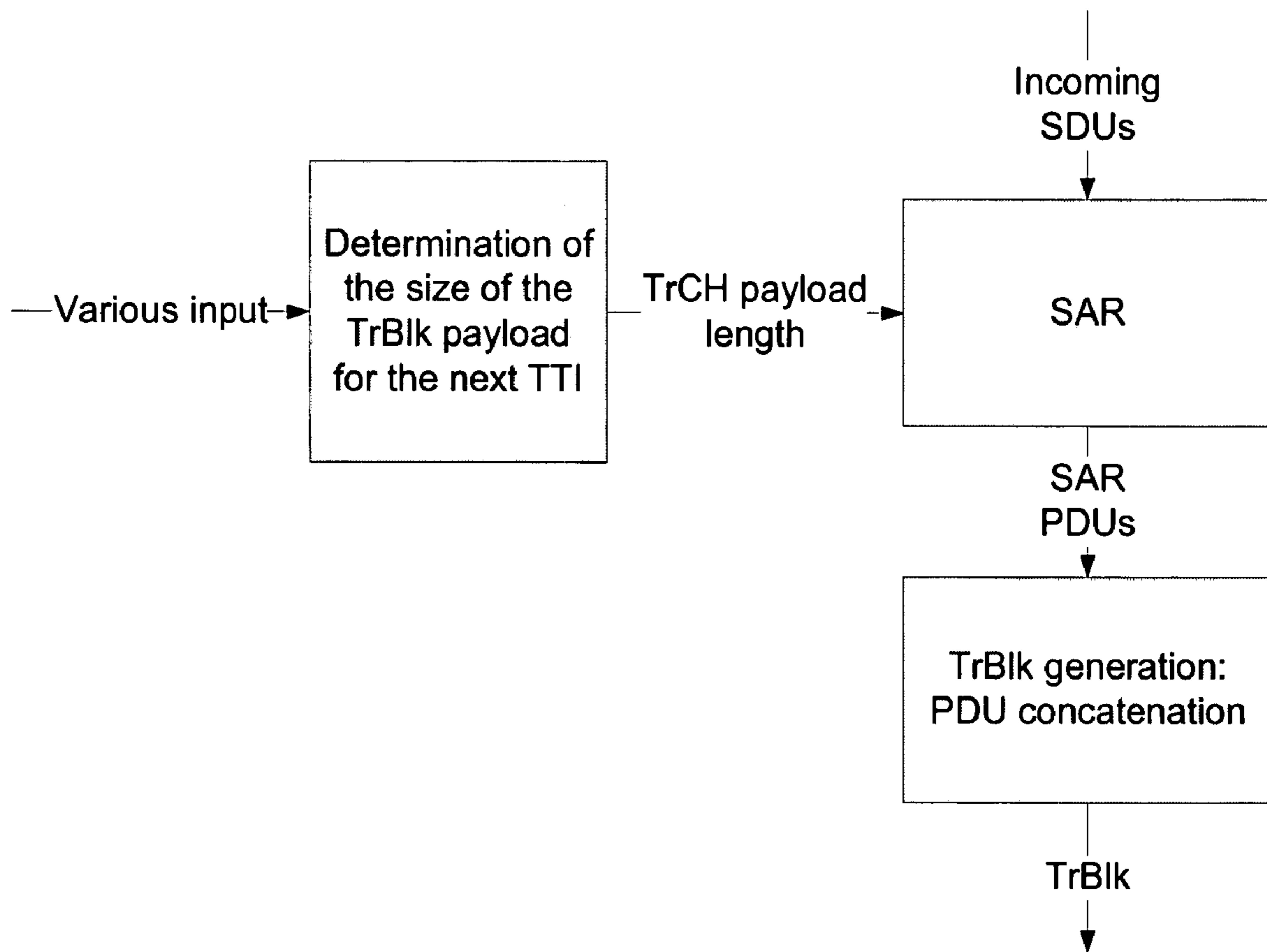
Figure 9 - Proposed SAR and concatenation processes
