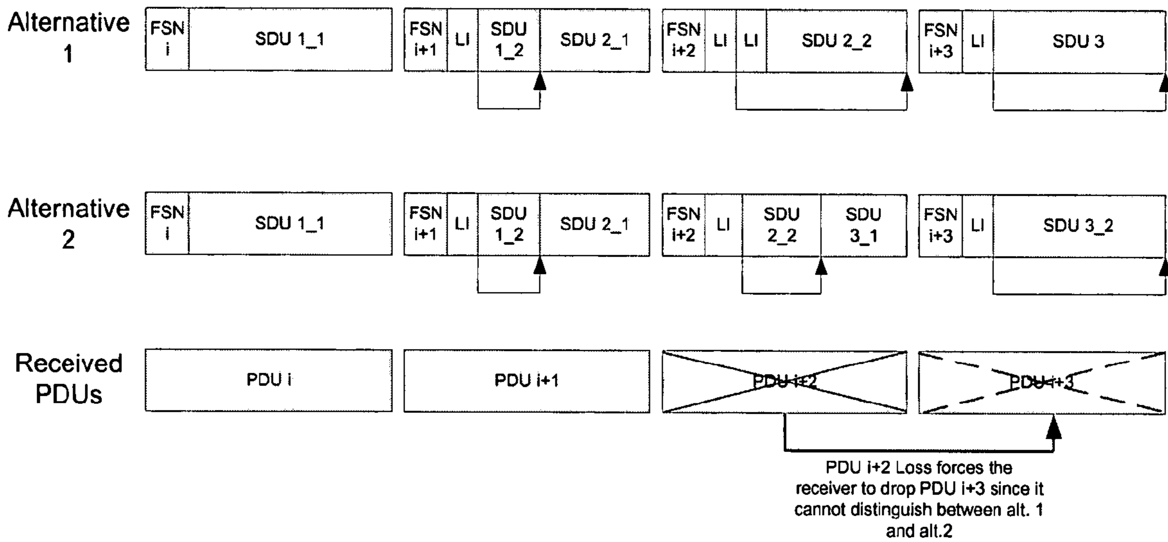
Figure 8 - Error propagation in UMTS R99
