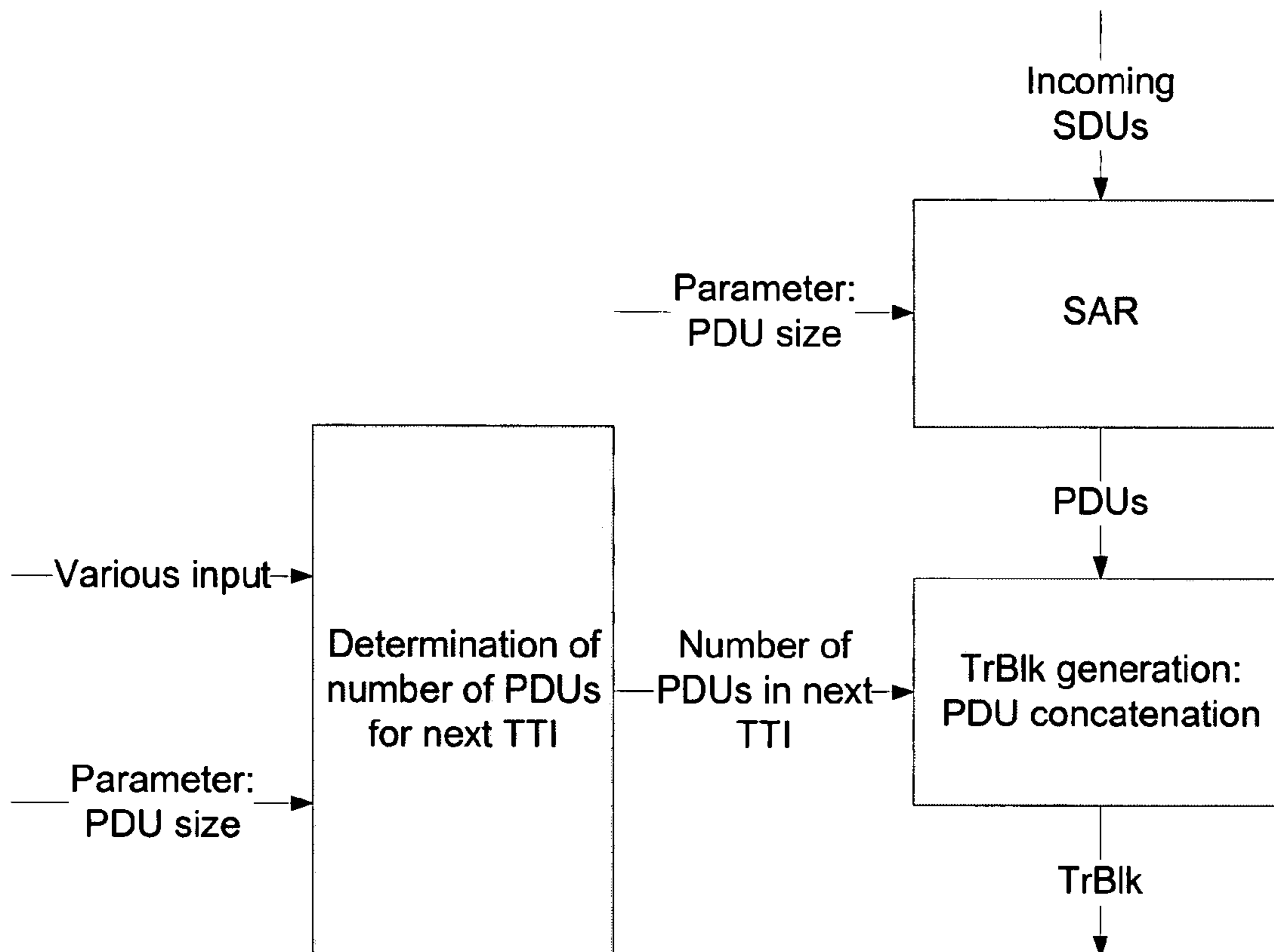
Figure 6 - SDU Segmentation and PDU concatenation Processes
