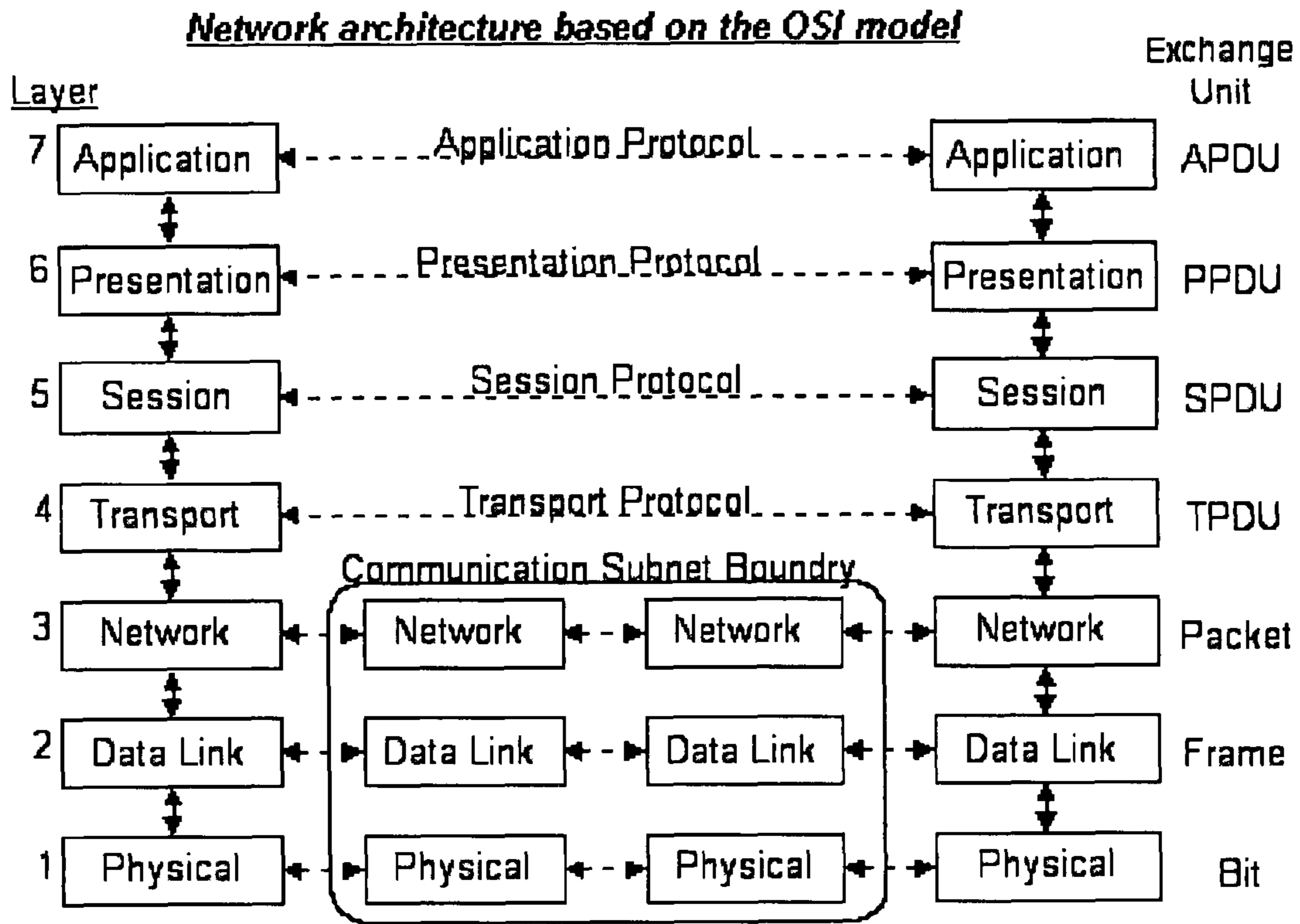
Figure 1 - OSI layer model
