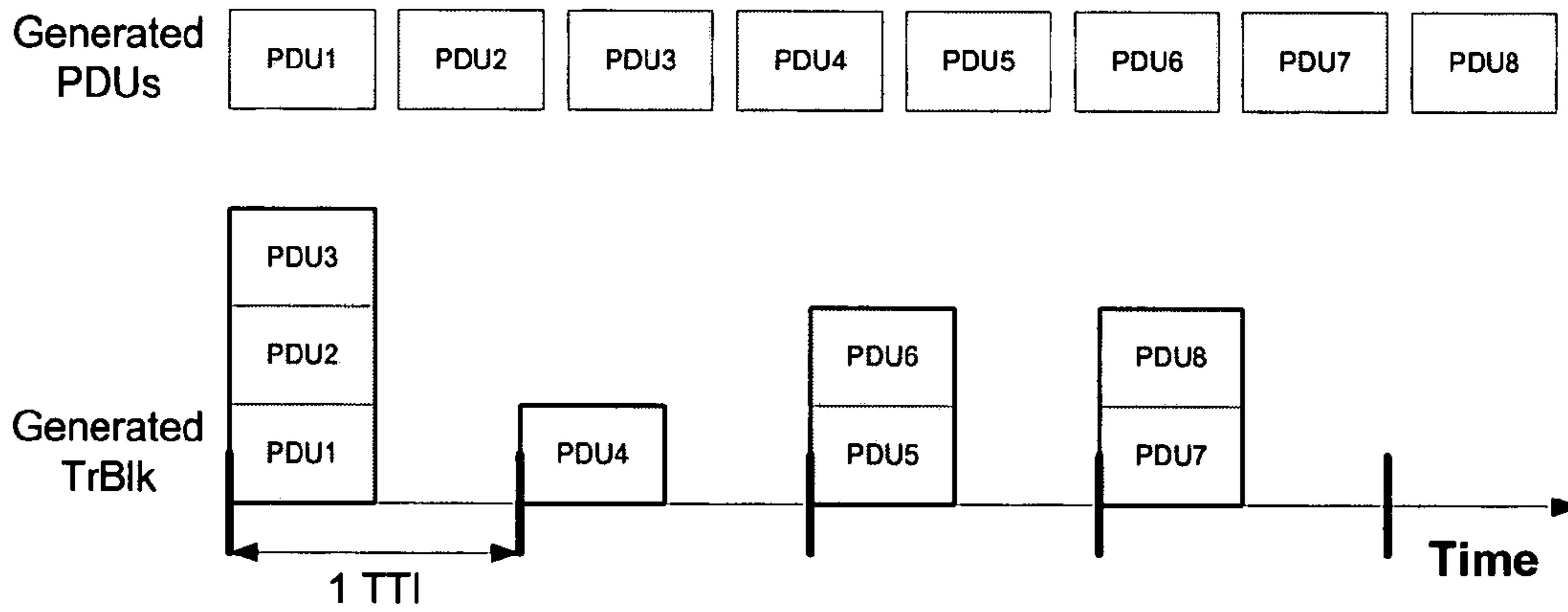
Figure 7 - Transport Channel Block generation
