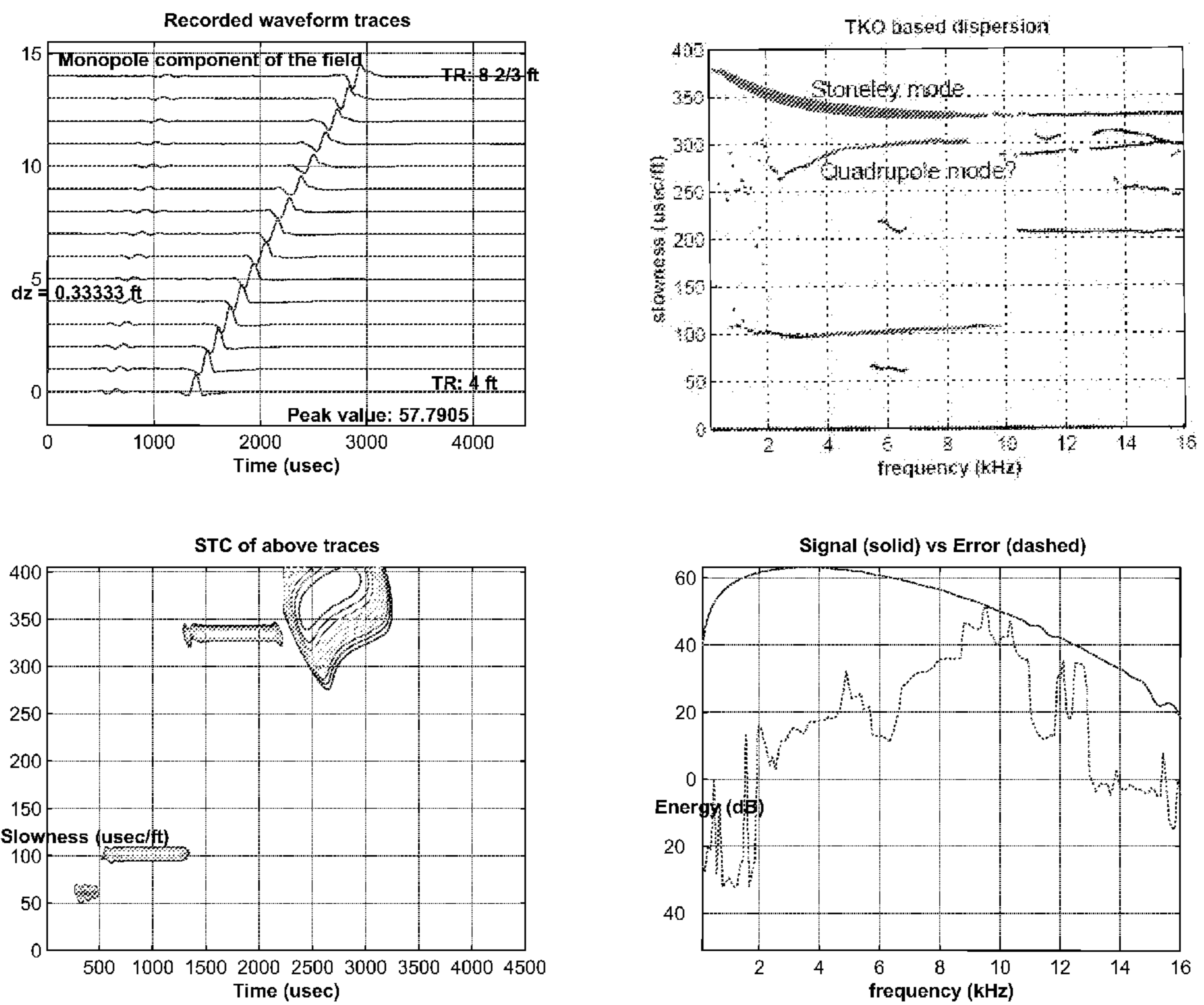
Smooth collar in a vertical borehole with intrinsic HTI formation: Simulation with a "Monopole ring" source
