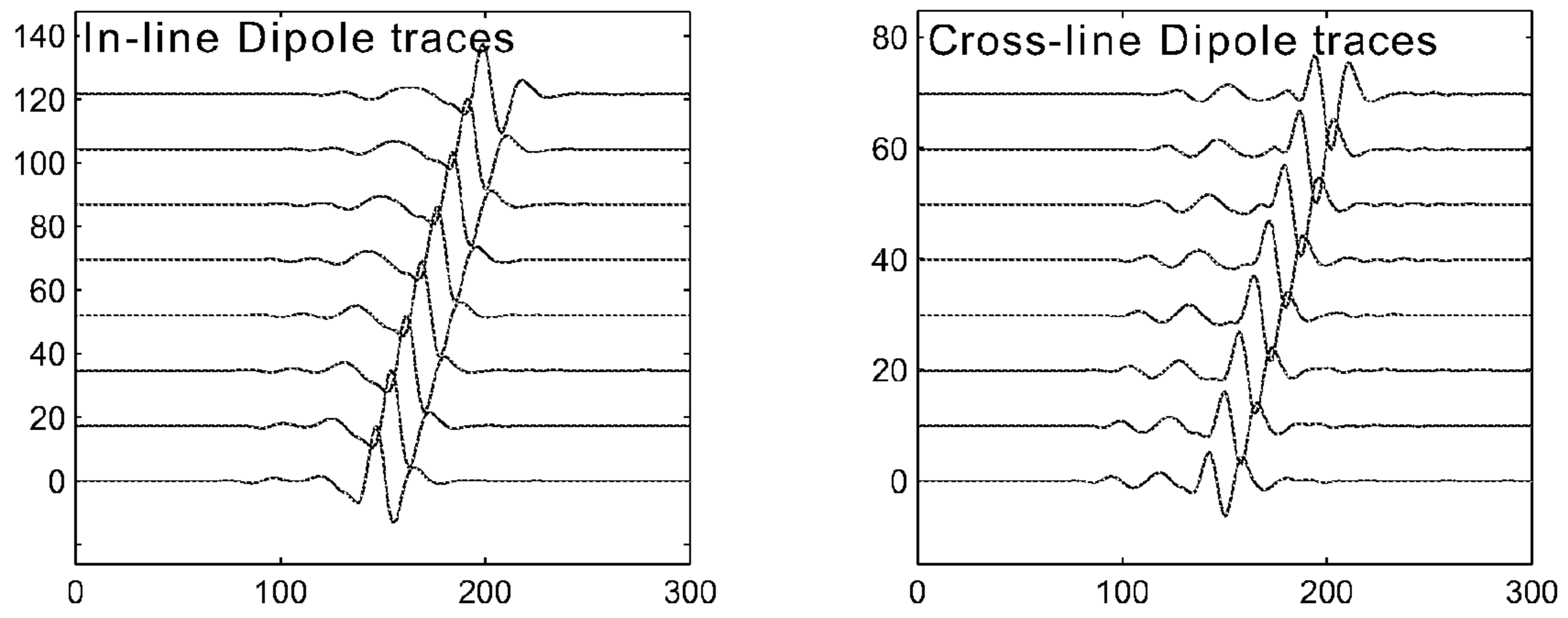
Dipole source axis at 30 deg relative to FAST direction
