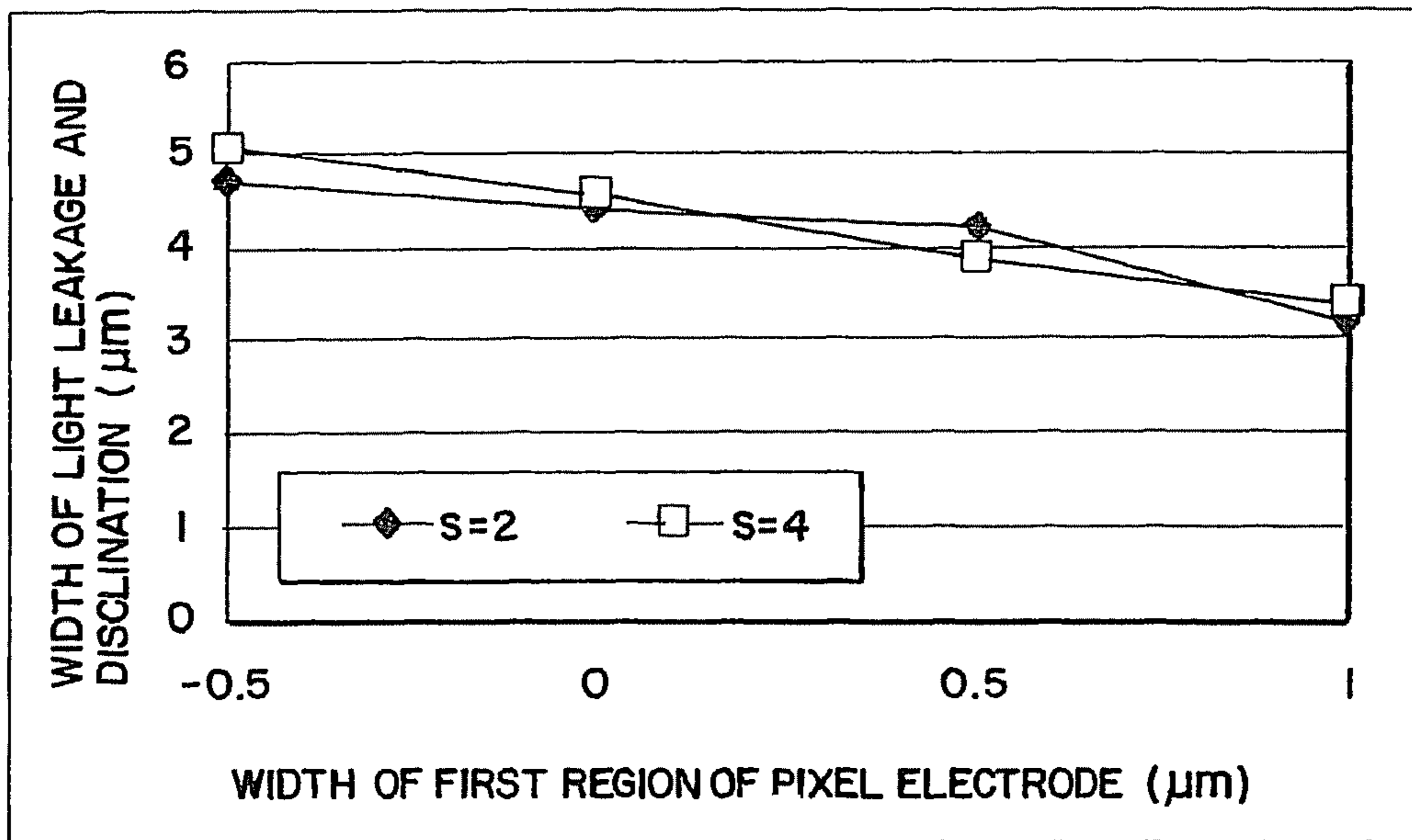
THE RELATION BETWEEN WIDTH OF FIRST REGION OF PIXEL ELECTRODE AND WIDTH OF DISCLINATION AND LIGHT LEAKAGE DISTANCE BETWEEN PIXEL ELECTRODES: 2.0 μm (s=2), 4.0 μm (s=4)
