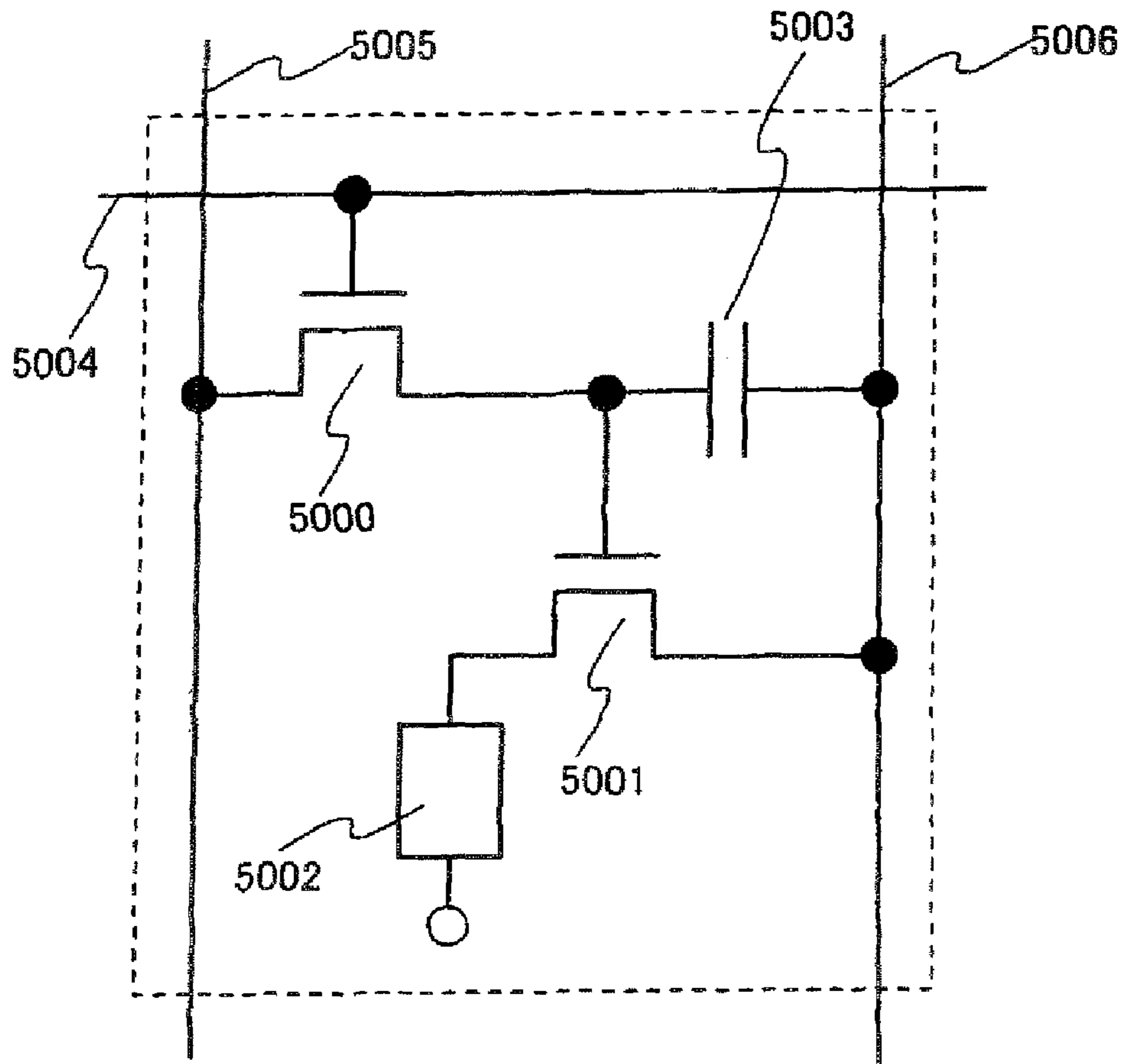
Fig. 18 PRIOR ART
