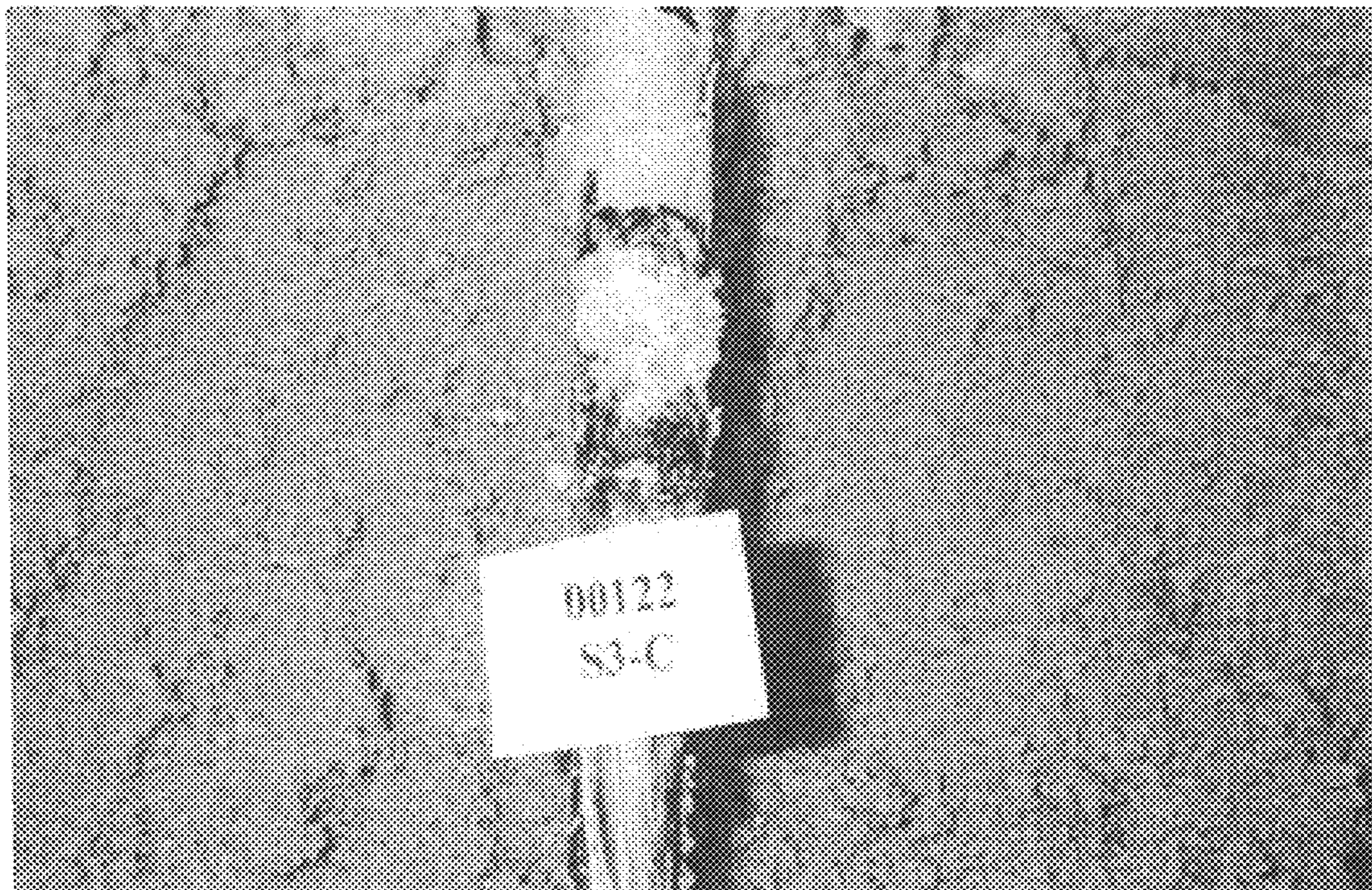
Figure 10 Sample 3 (Control) with significant corrosion after 91 days in test
