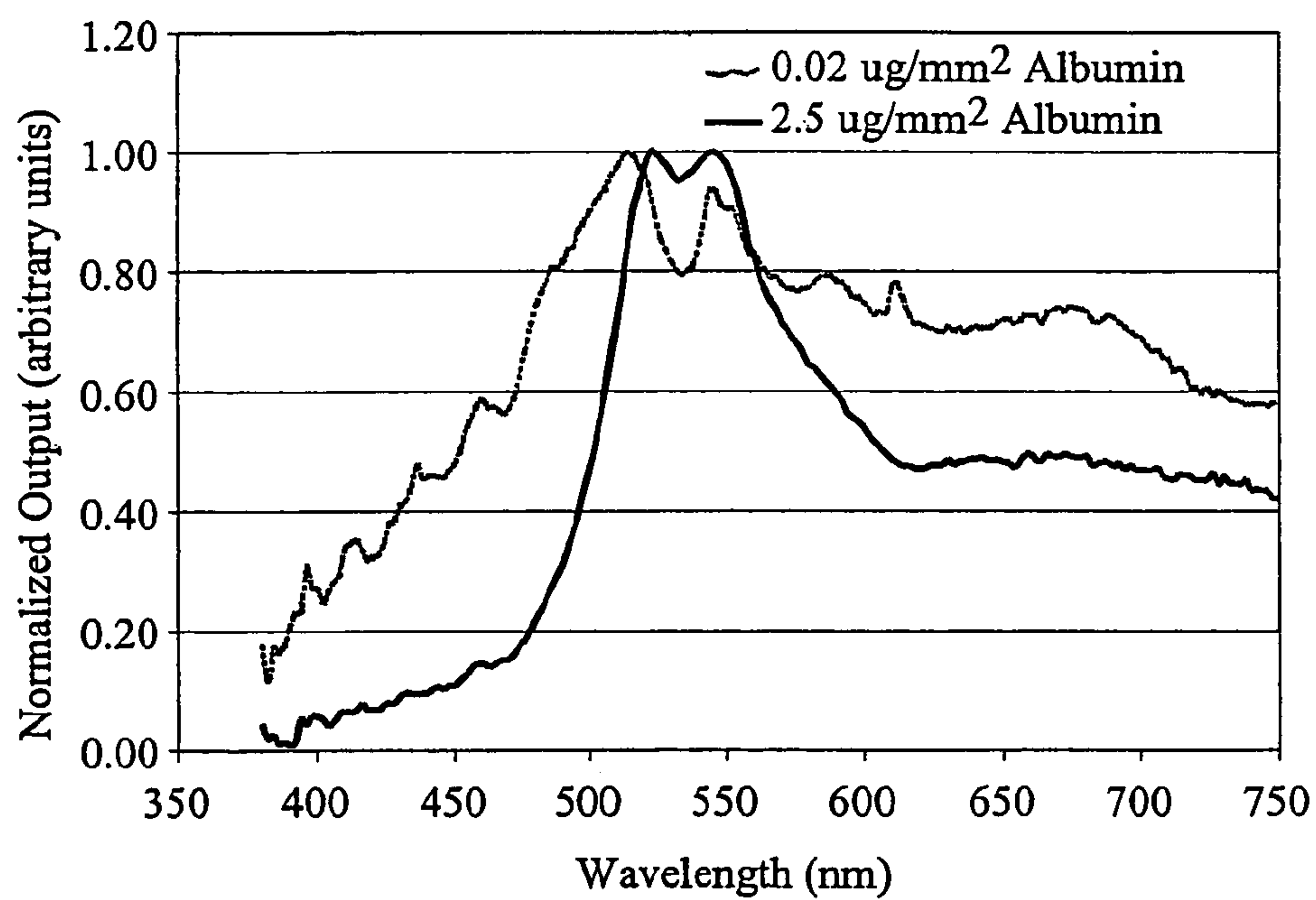
Albumin Deposition on Resonant Reflector
