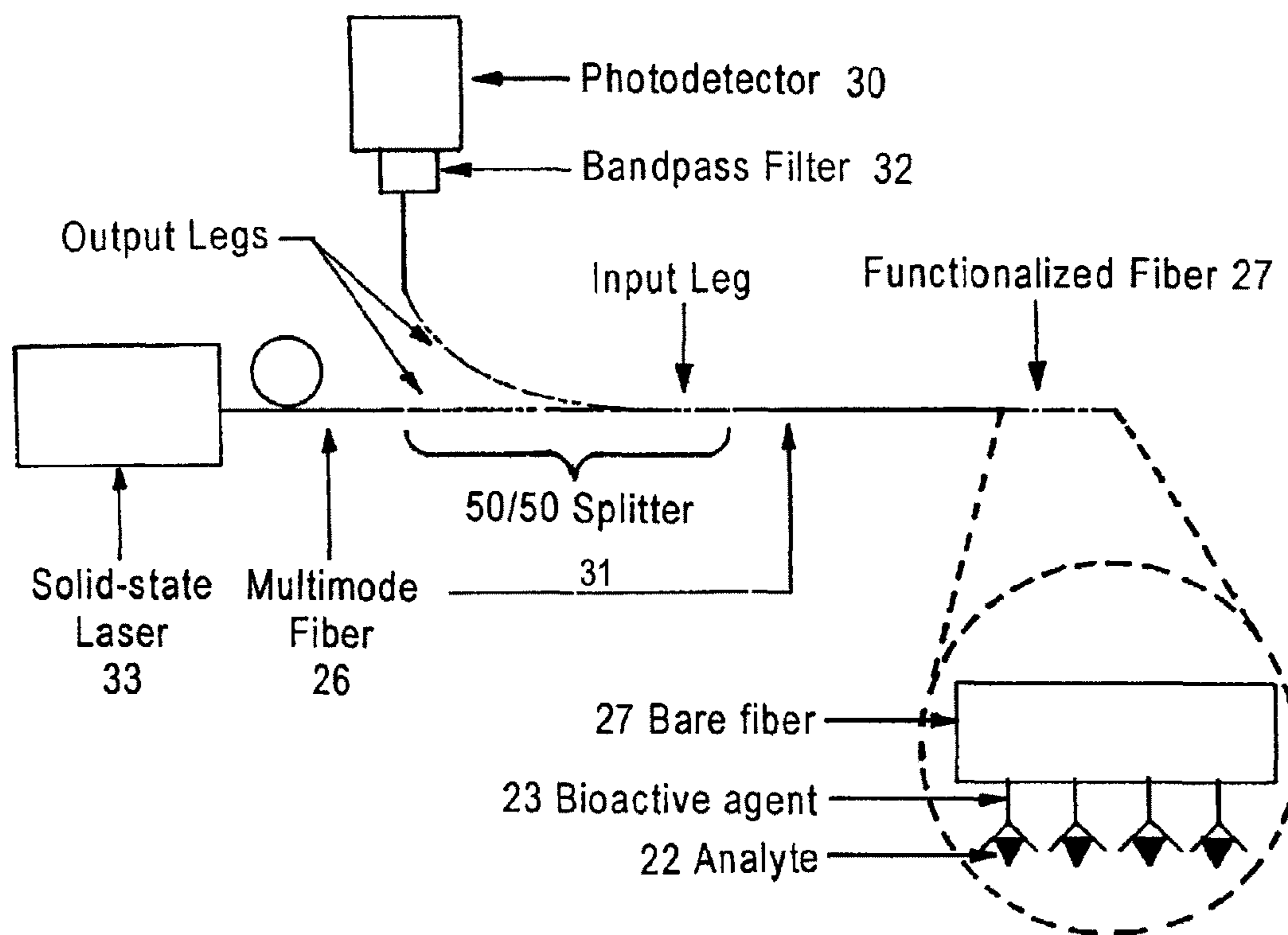
Schematic diagram of fiber optic TIRF sensor. Incoming laser light is directed through the output leg of a 50:50 fiber optic splitter onto the functionalized fiber. Emitted fluorescence couples back into the fiber and propagates towards the detector with little interference from the laser light.
