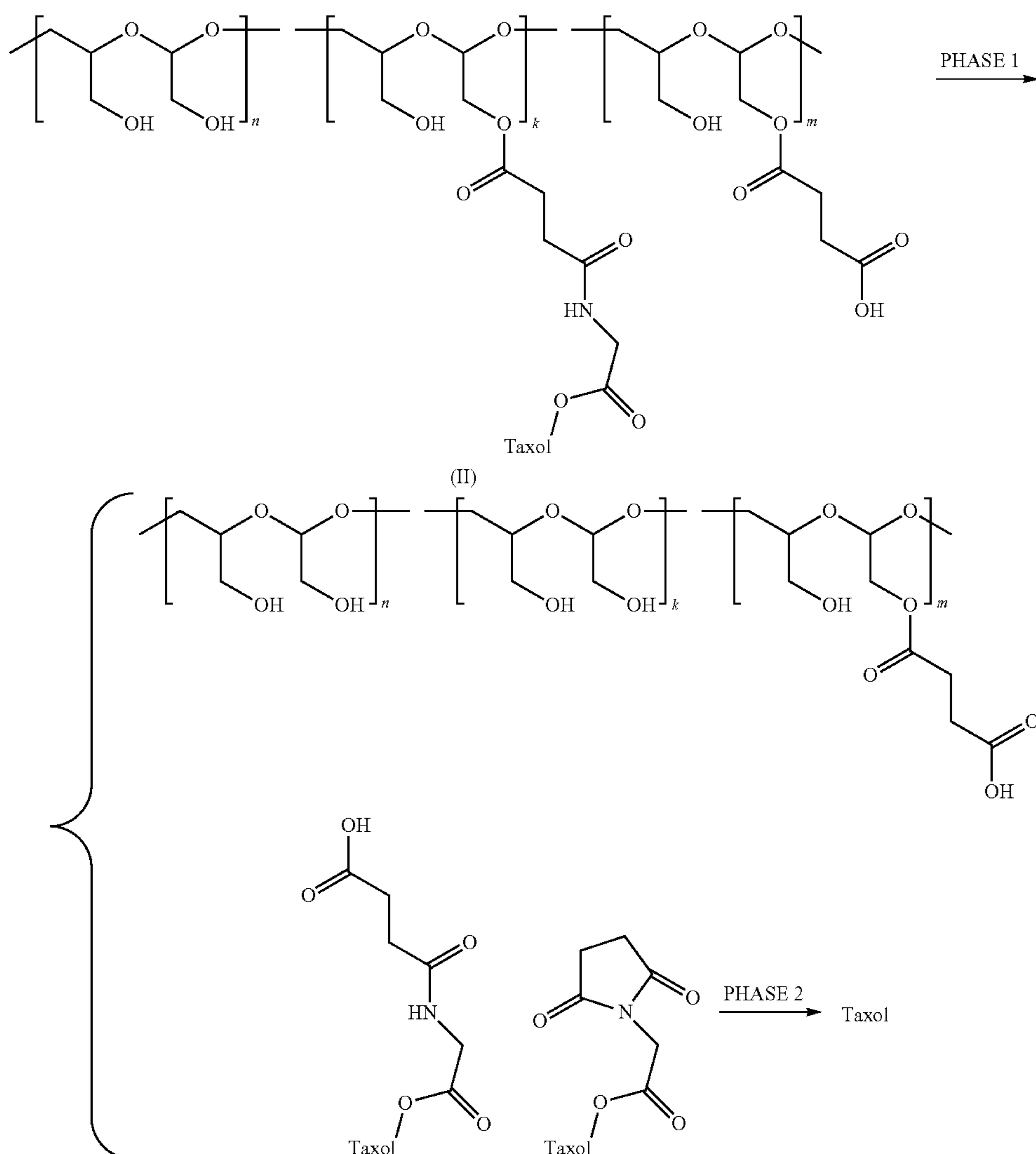
Scheme 4
