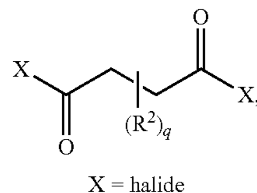
20 succinic ester
