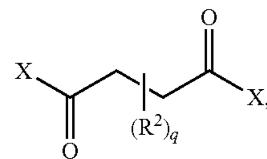
20 succinic ester
