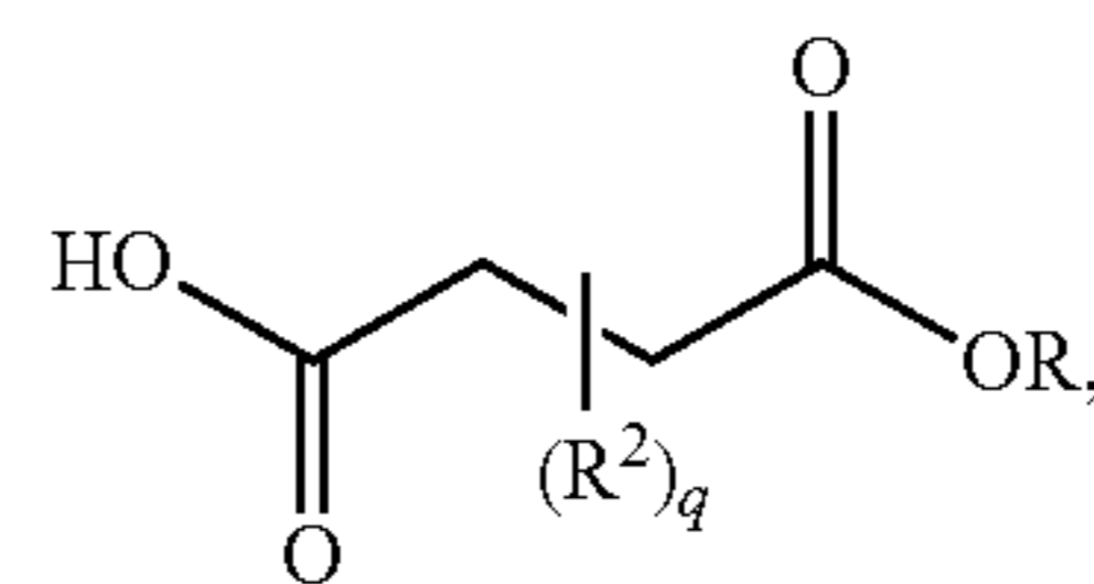
20 succinic ester
