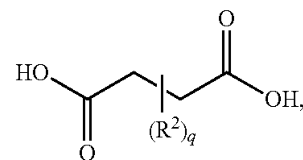
10 succinyl dihaloanhydride
