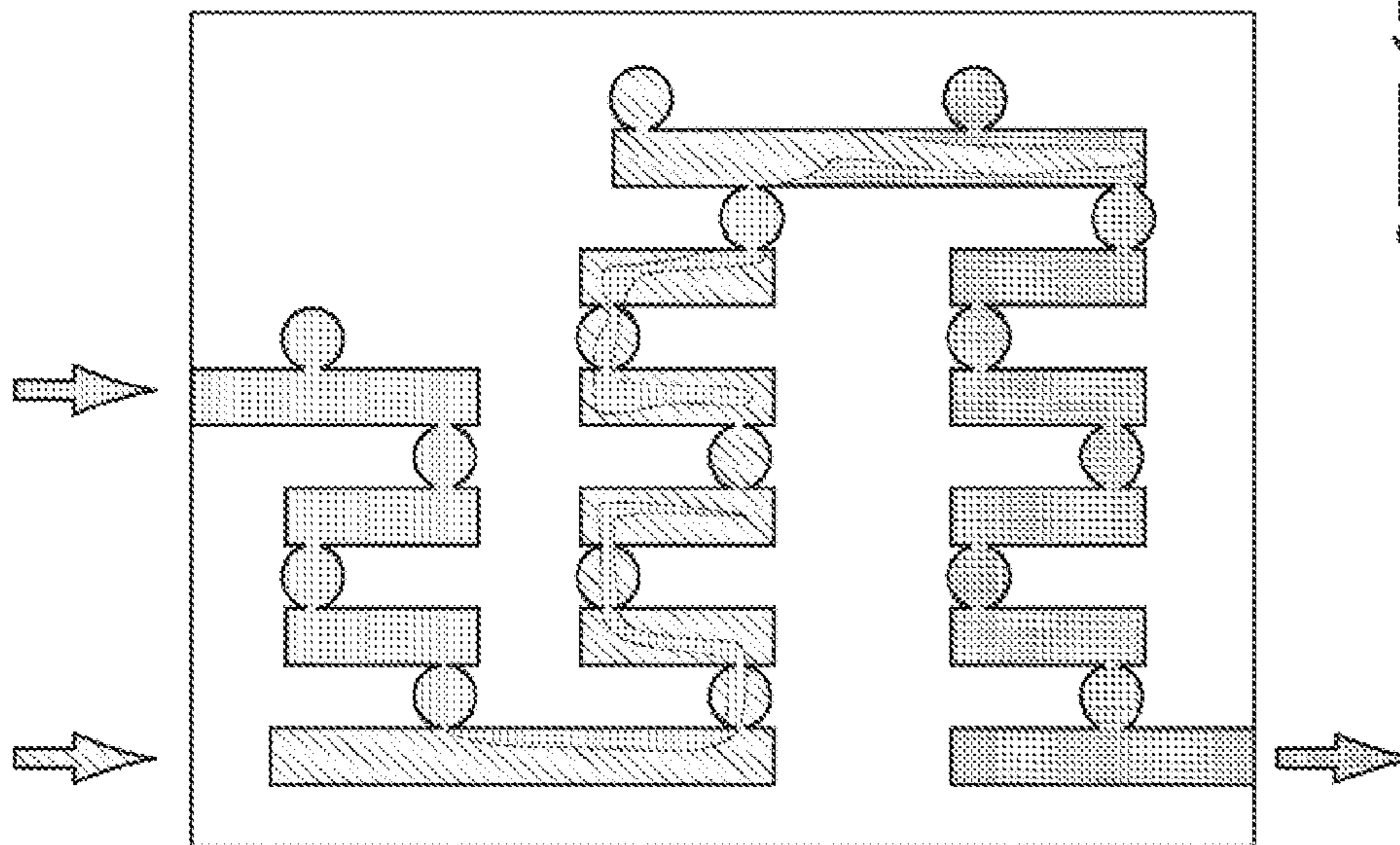
Series Of Mixing Towers (3-D)
