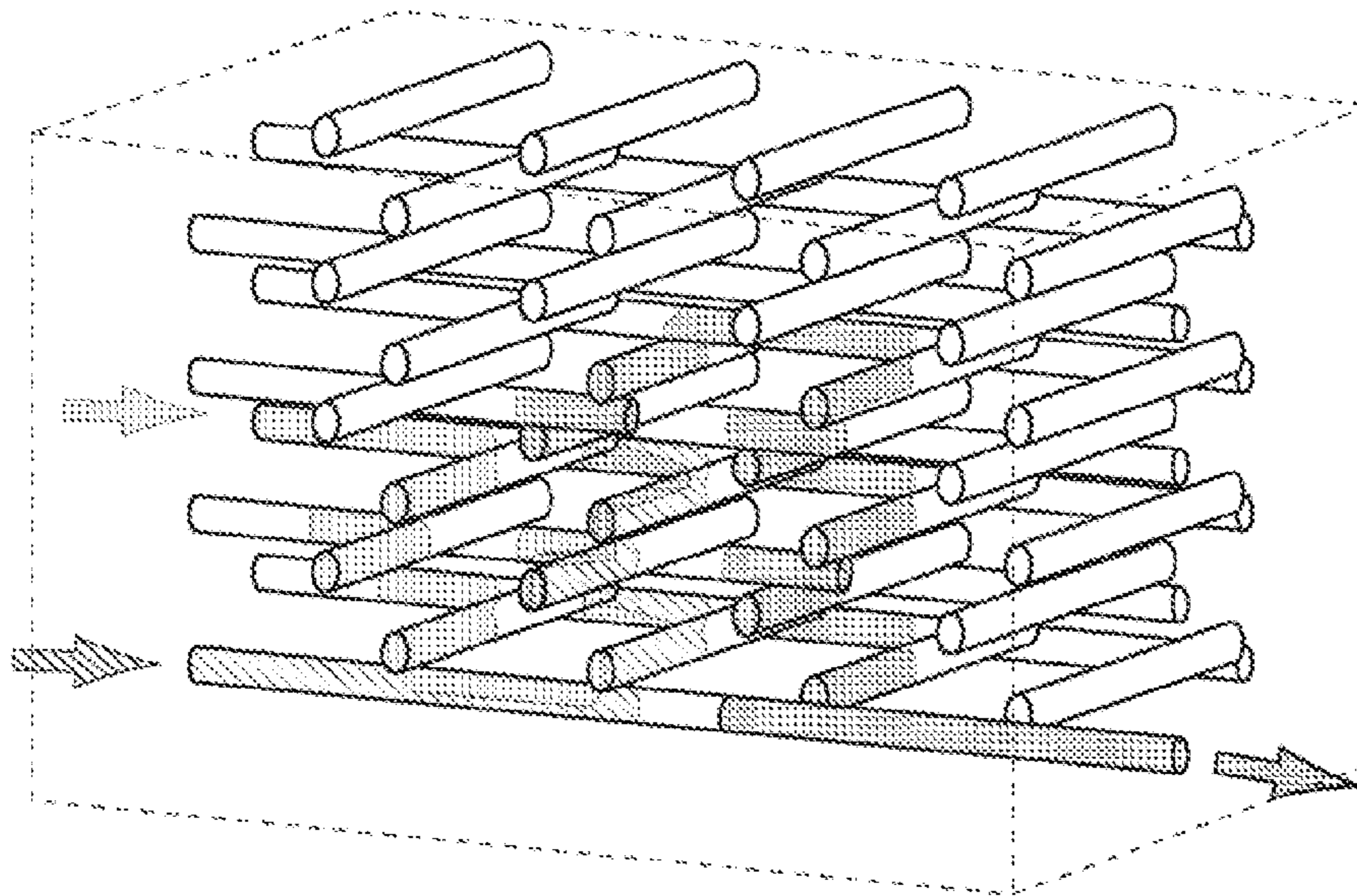
Series Of Mixing Towers (3-D)
