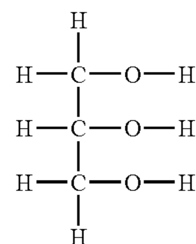
GLYCEROL C 3 H 8 O 3
