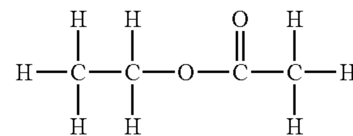
ETHYL ACETATE [AN ESTER] C 4 H 8 O 2
