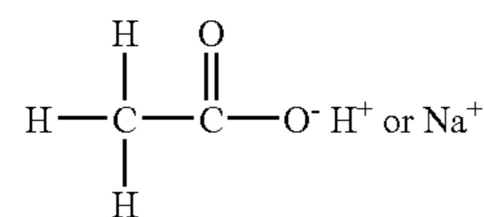
ACETATE ION C 2 H 3 O 2 -
