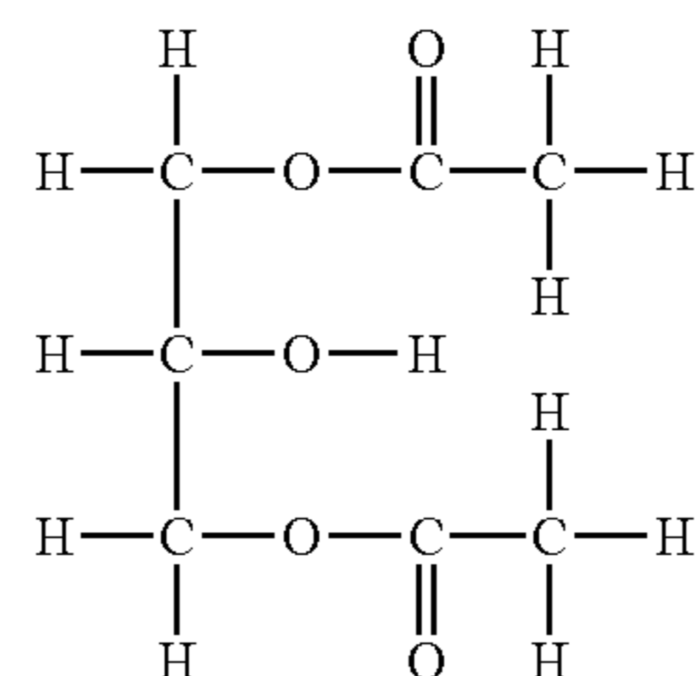
1,3-DIACETIN OR 1,3-GLYCEROL DIACETATE C 7 H 12 O 5
