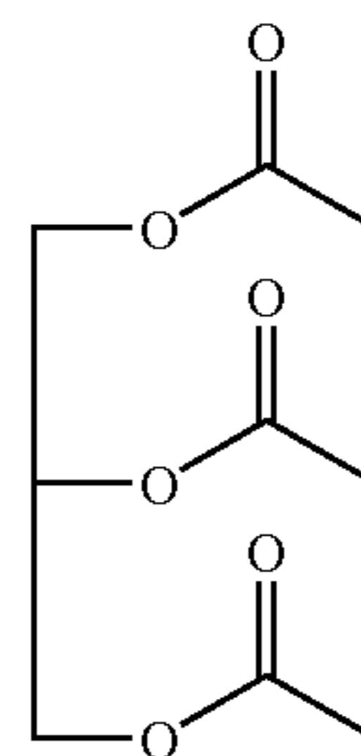
TRIACTIN
