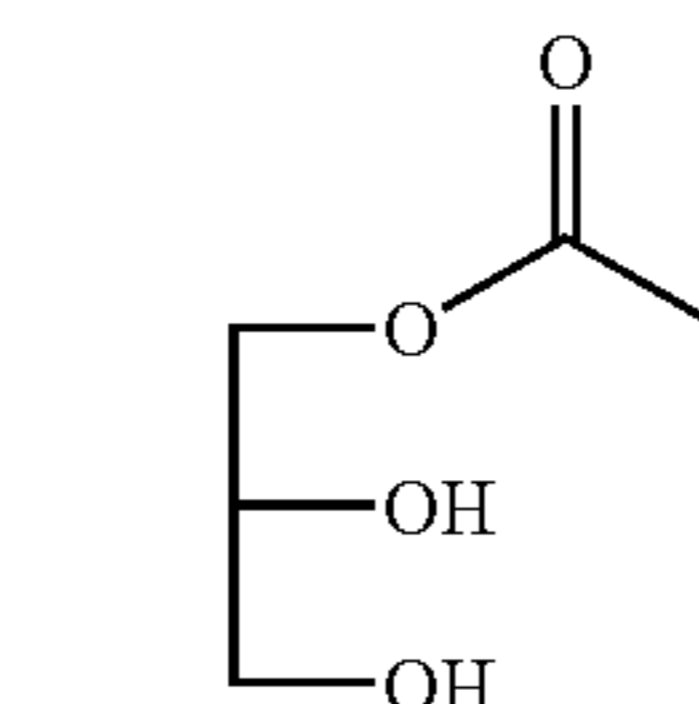
GLYCEROL-1-ACETATE
