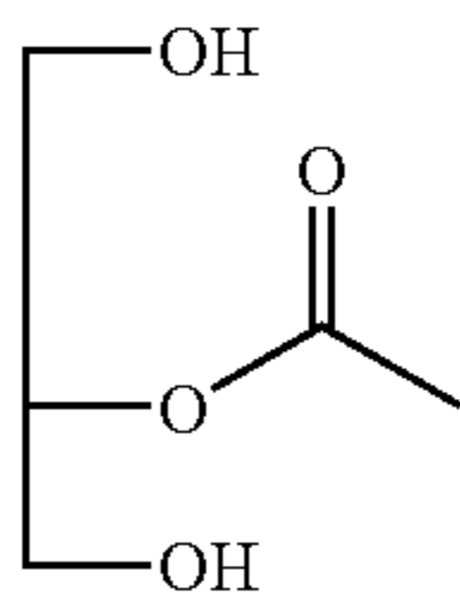
GLYCEROL-2-ACETATE
