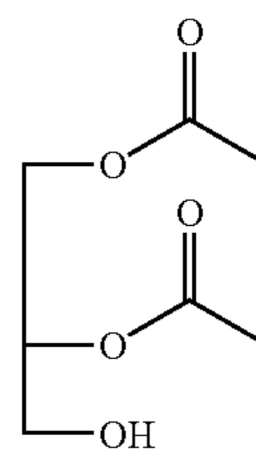
1,2-DIACETIN
