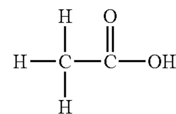
ACETIC ACID C 2 H 4 O 2
