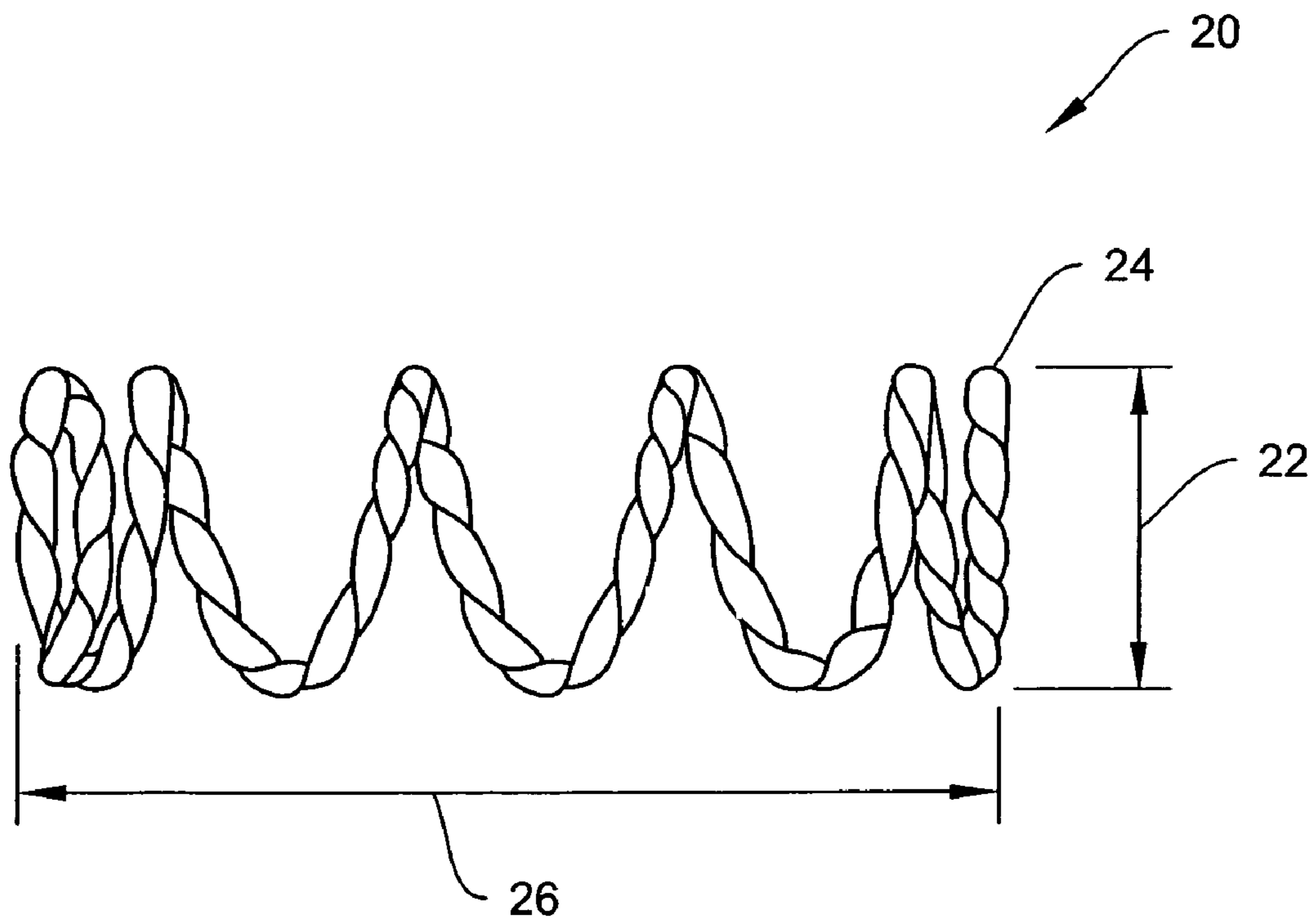
Figure 2, Stranded Wire Coil
