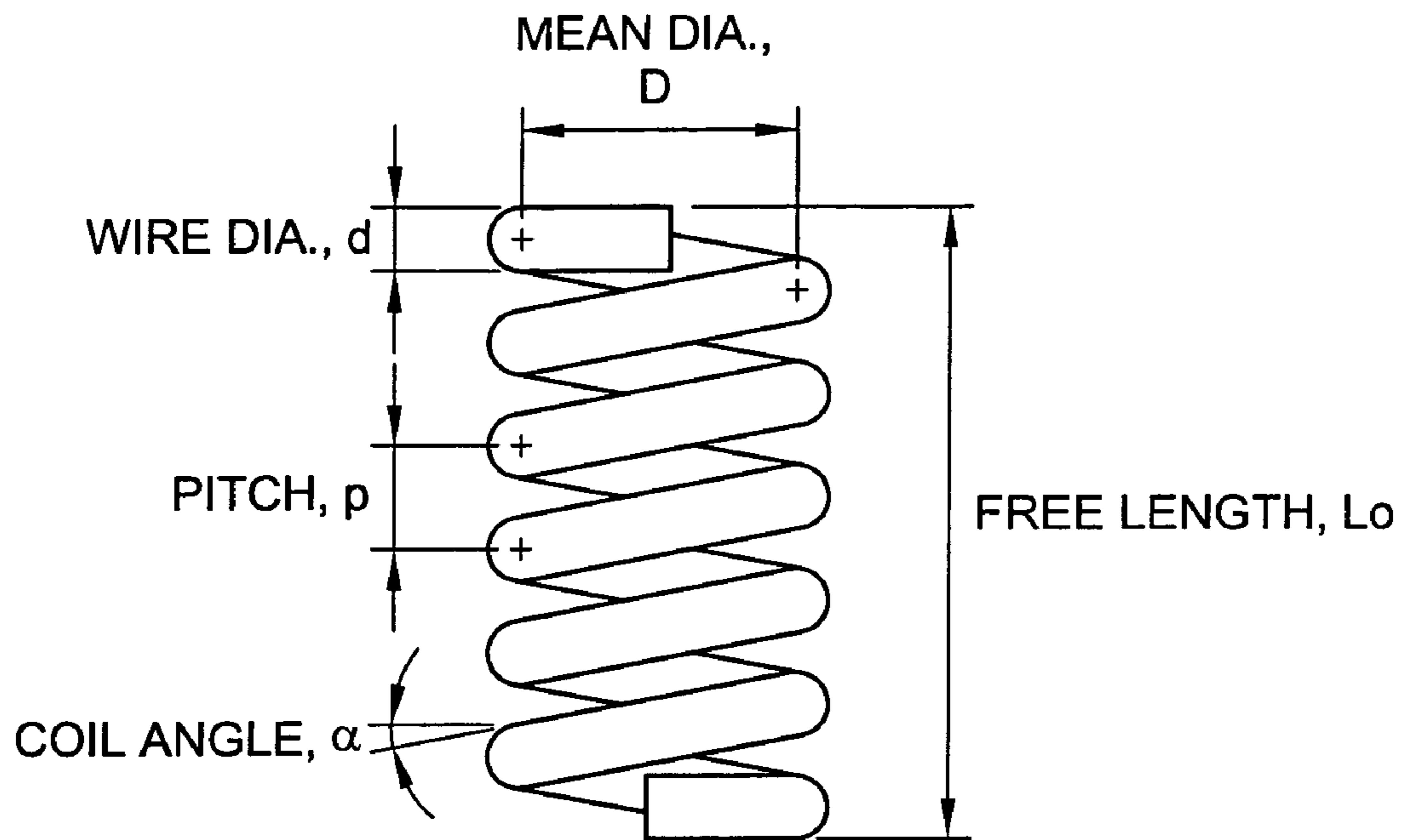
Figure 1, Conventional Compression Spring
