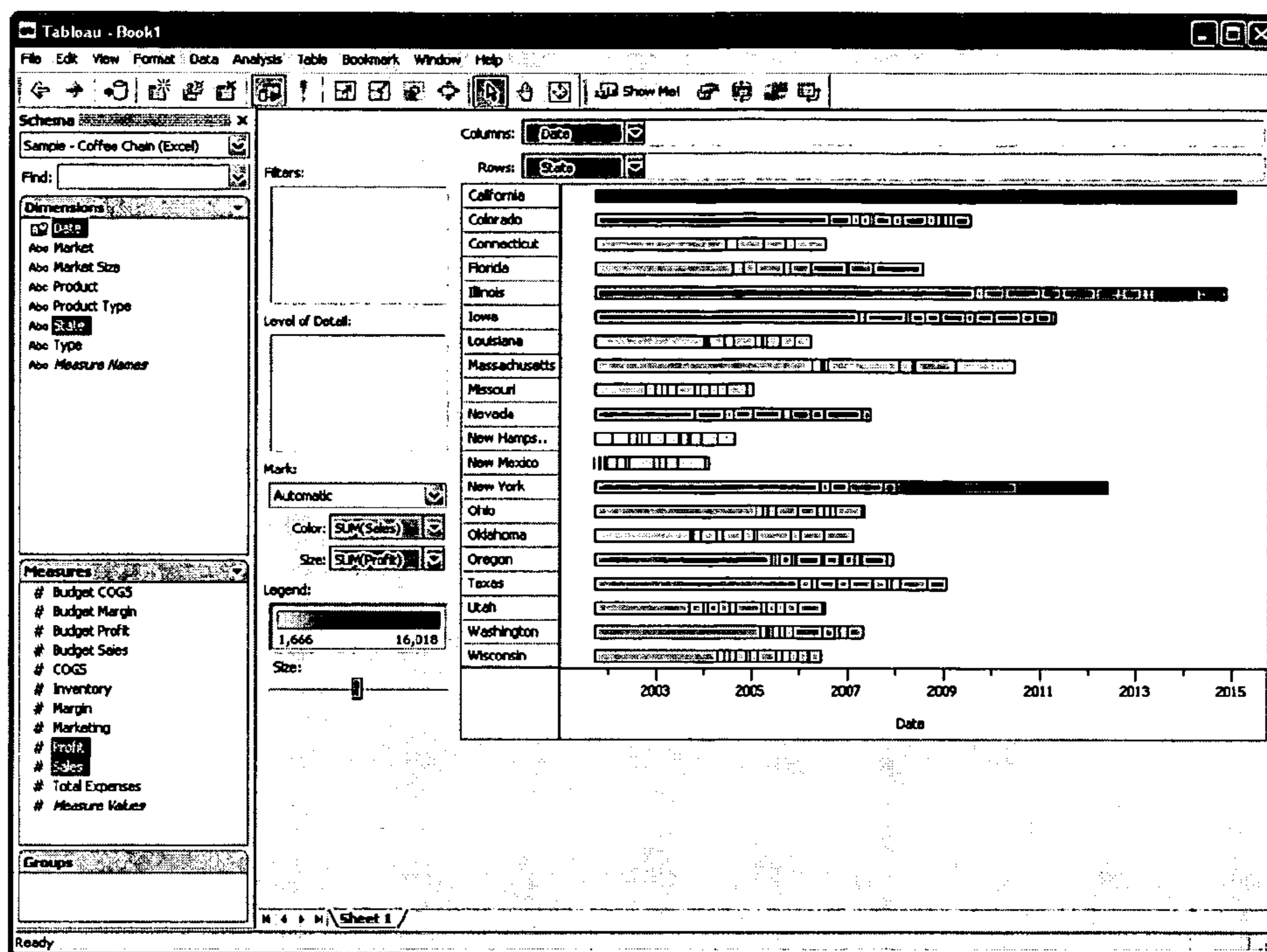
Figure 8i (Gantt)
