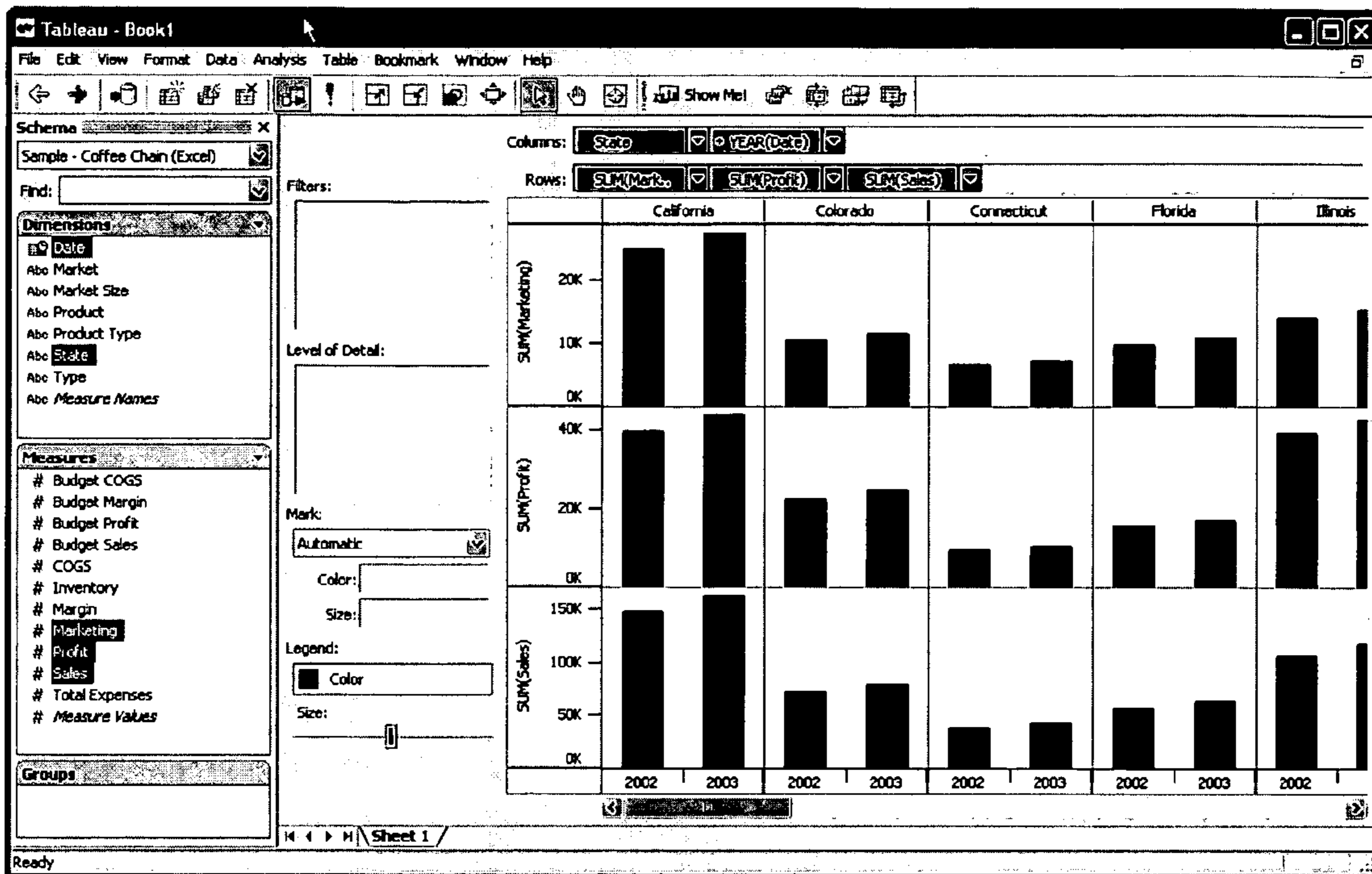
Figure 8c (Side-By-Side Bar)
