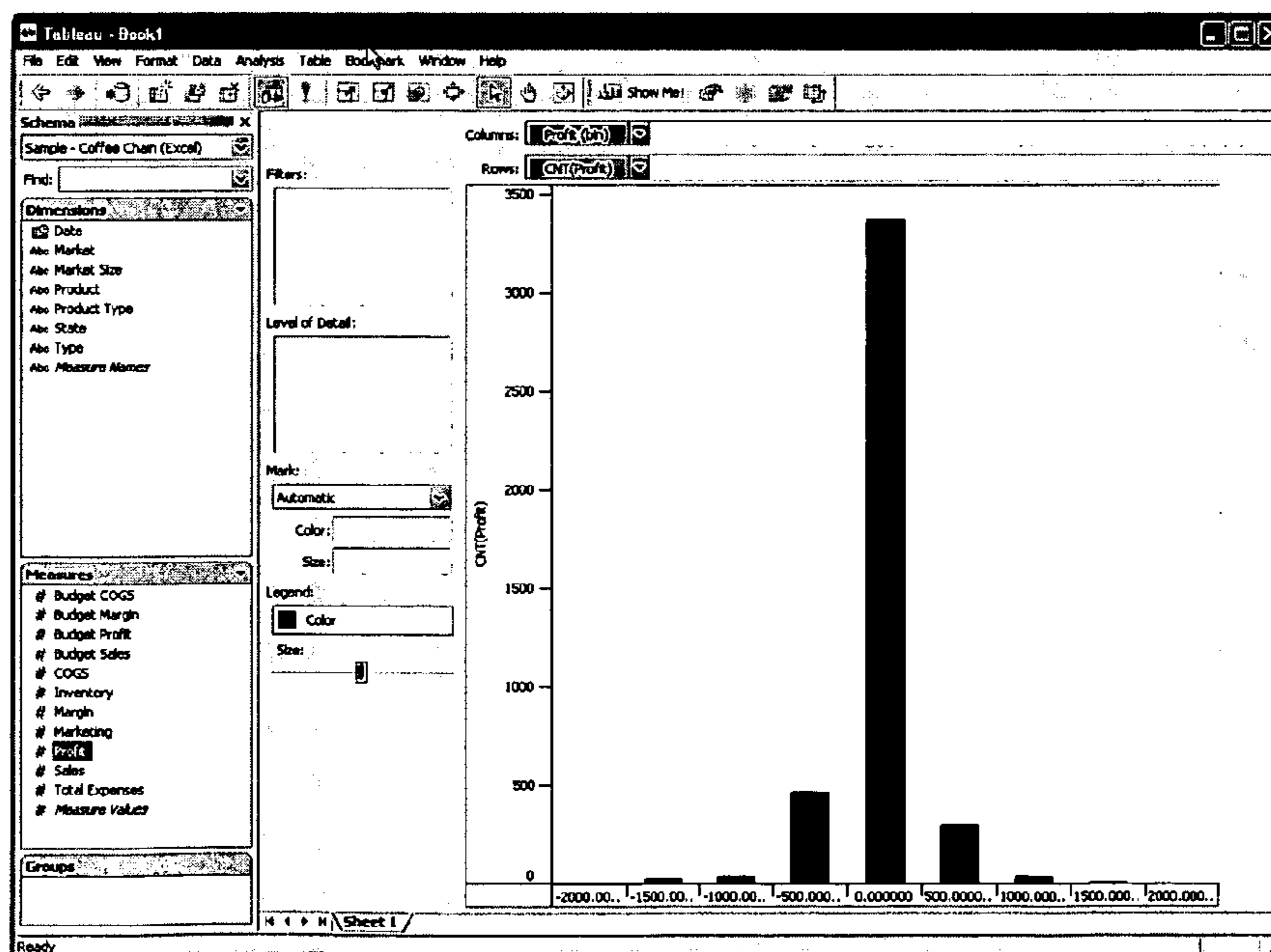
Figure 8l (Histogram)
