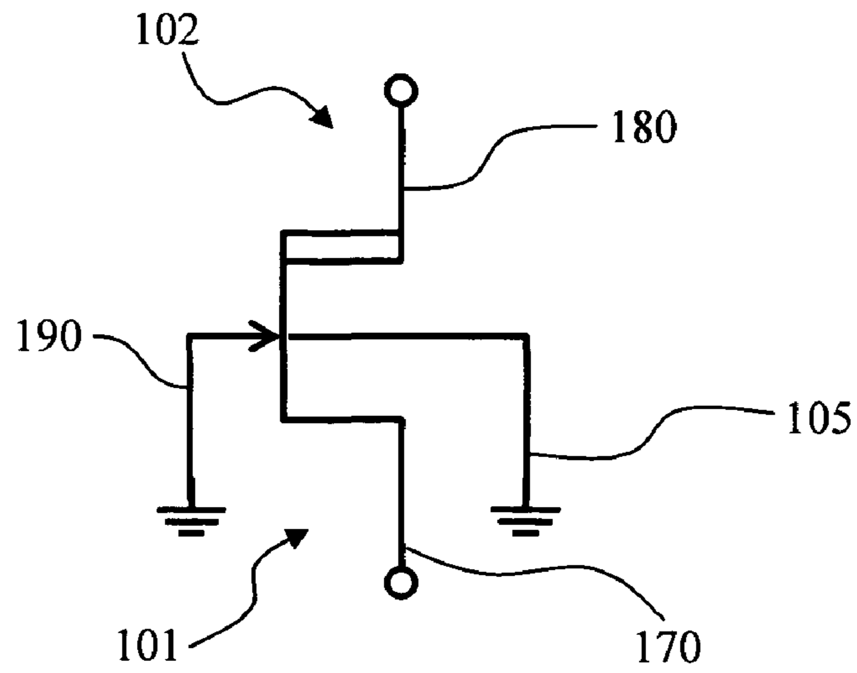
Fig. 3B Present Invention
