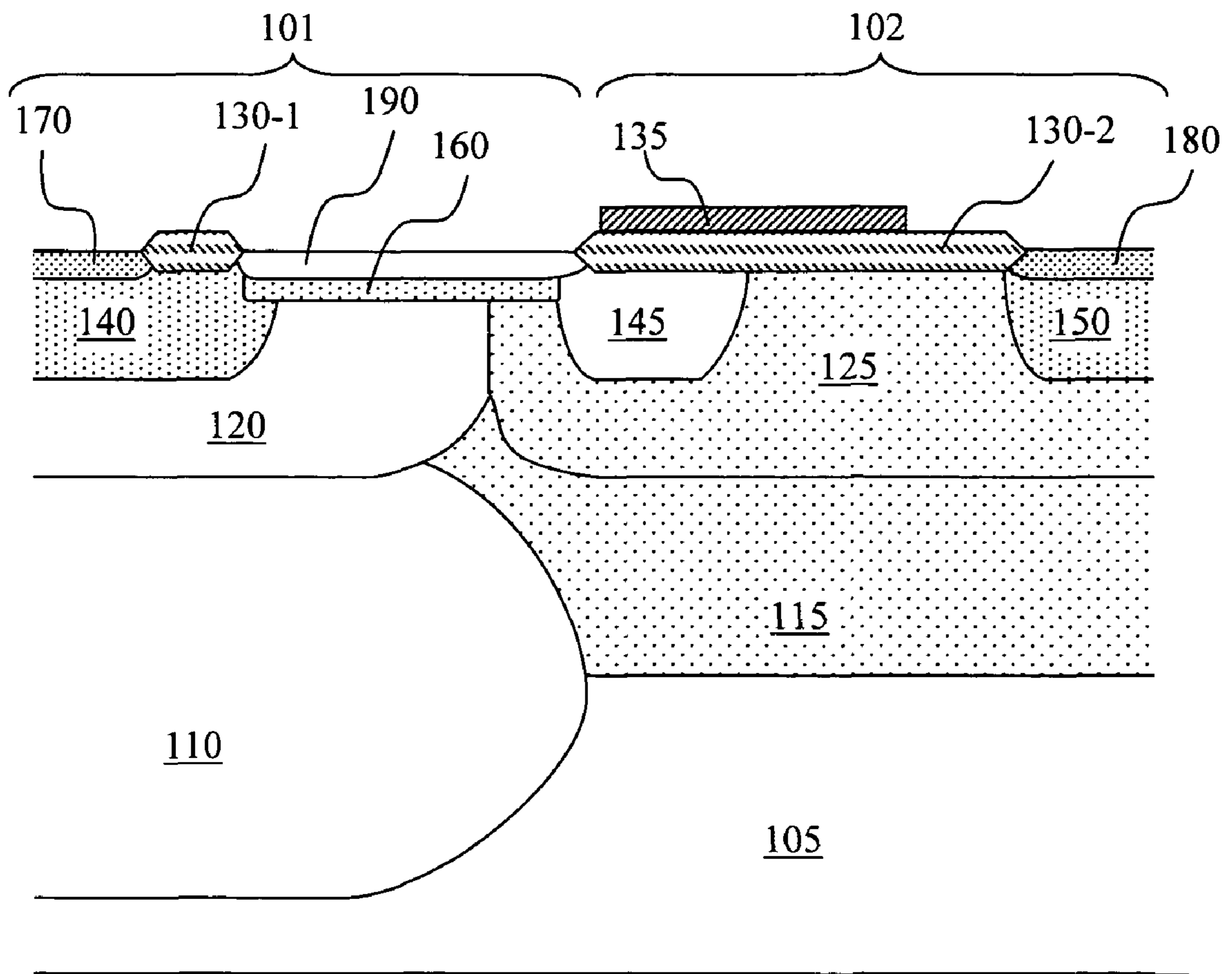
Fig. 5F Present Invention
