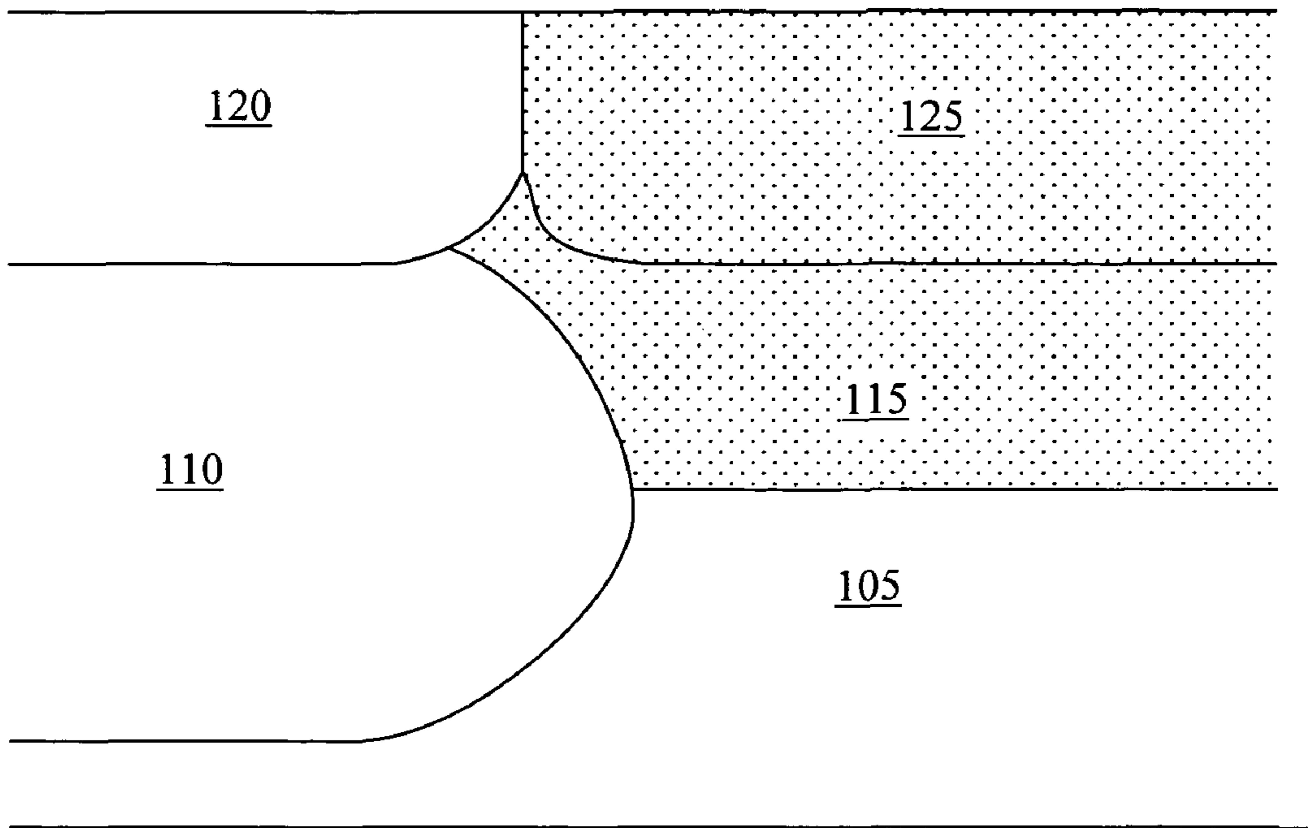
Fig. 5C Present Invention
