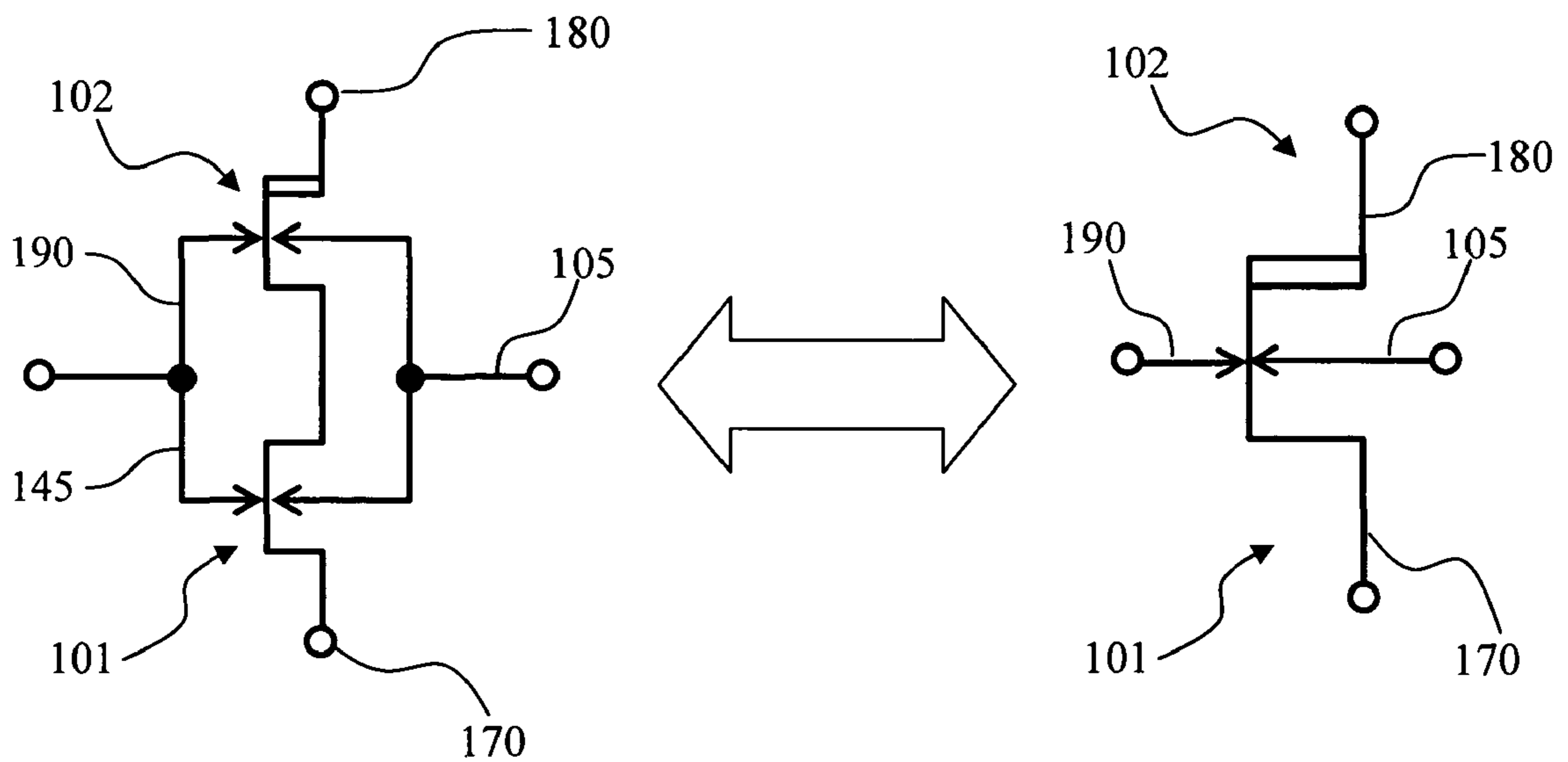
Fig. 2B Present Invention
