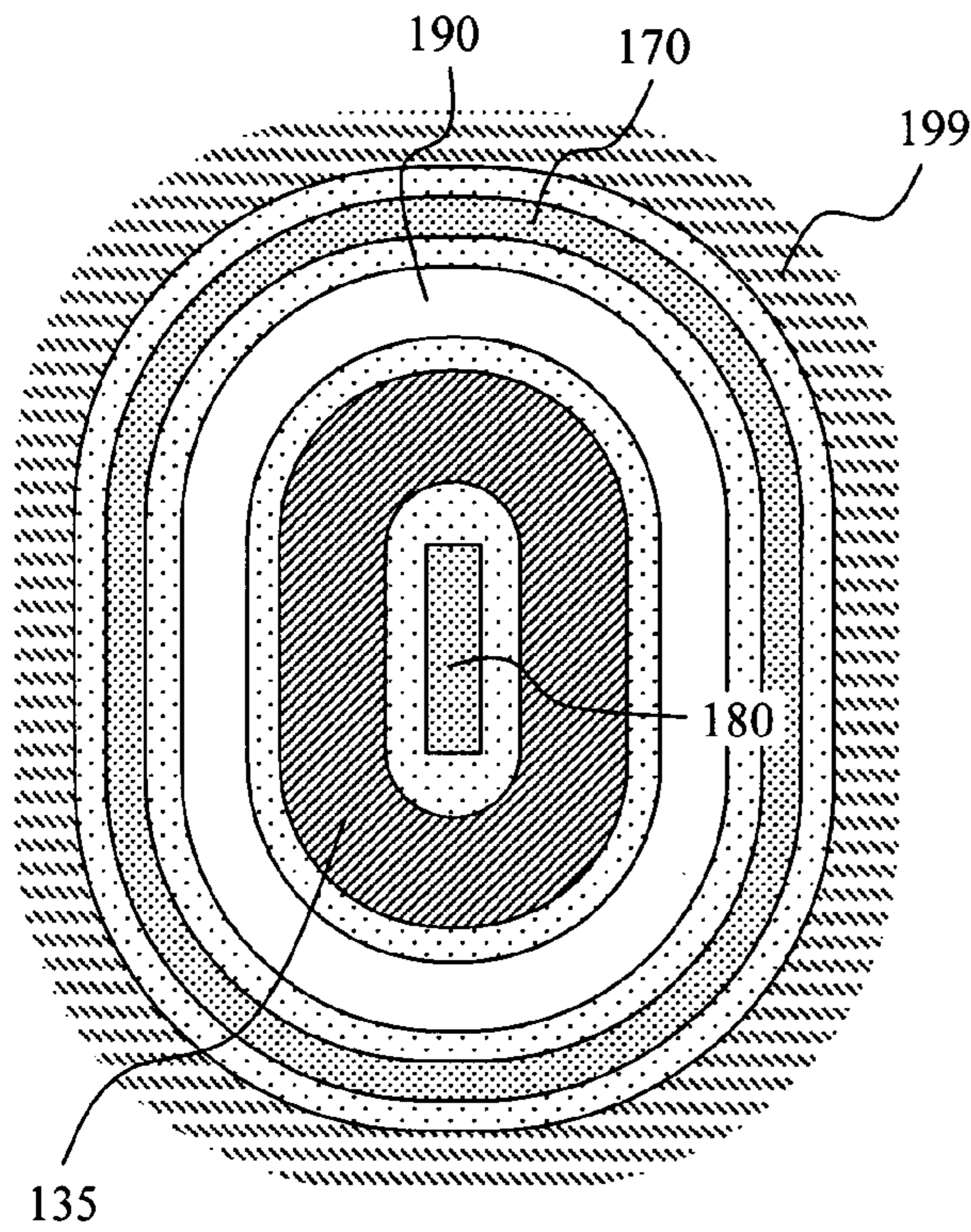
Fig. 4A Present Invention
