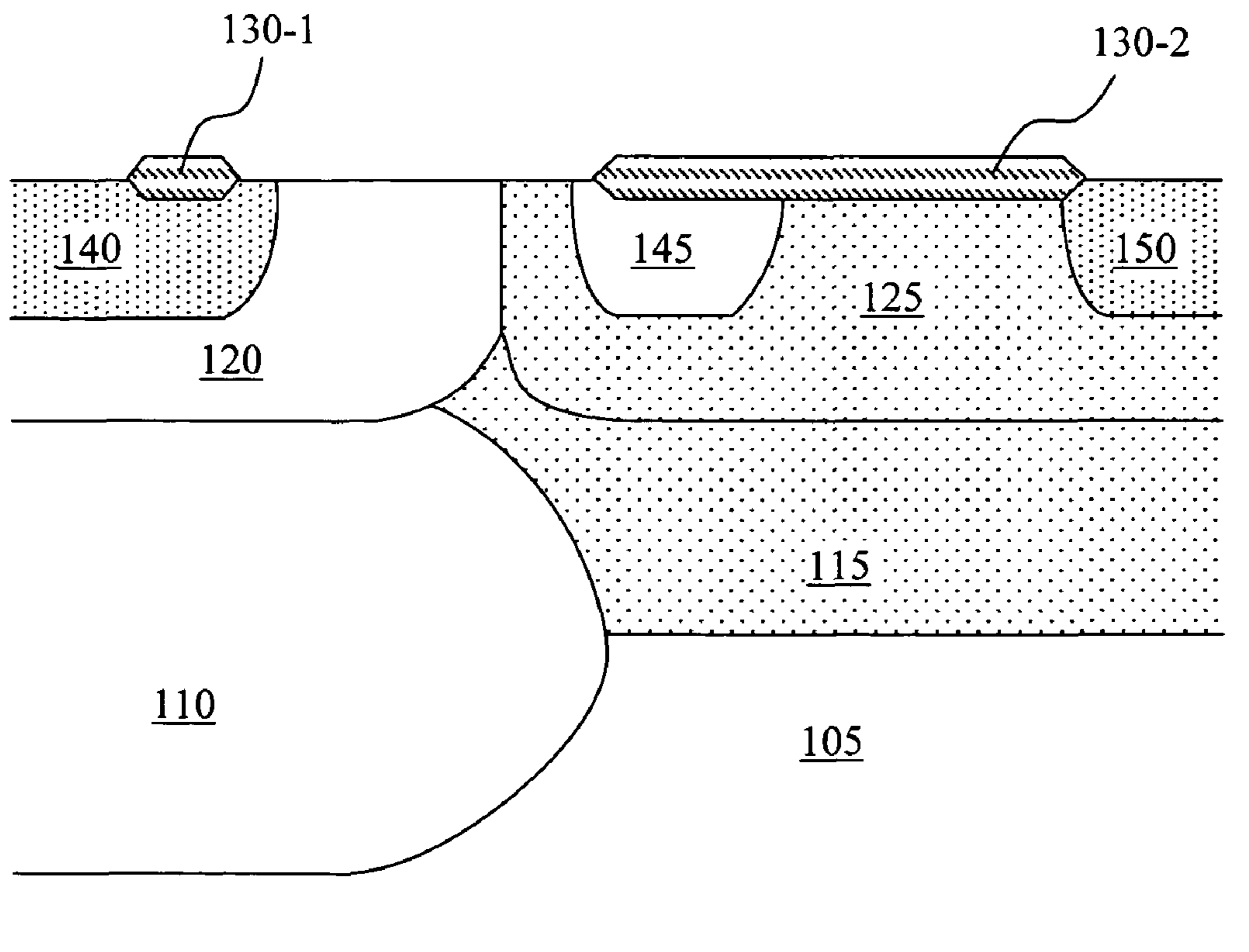
Fig. 5D Present Invention
