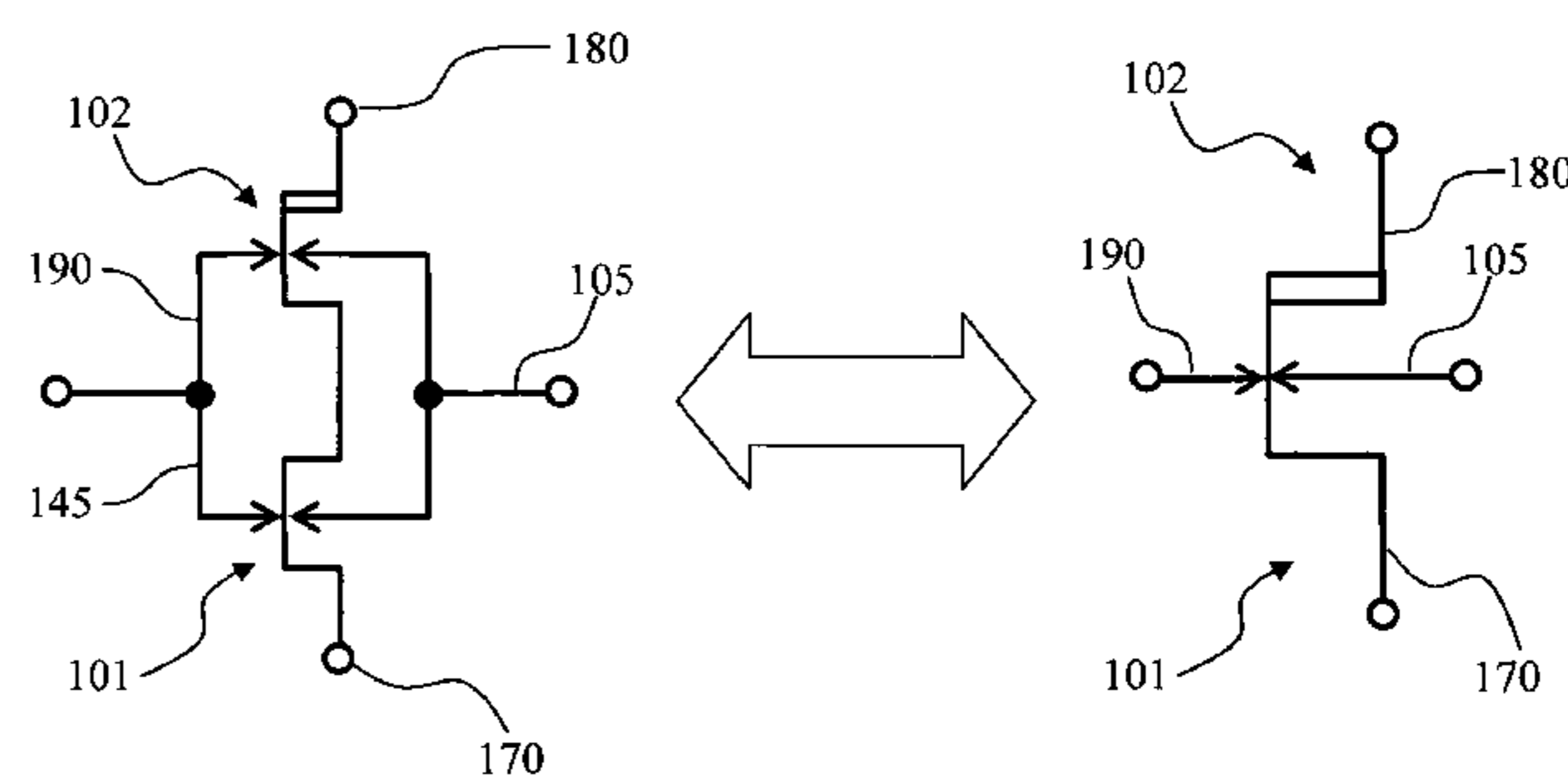
Present Invention
