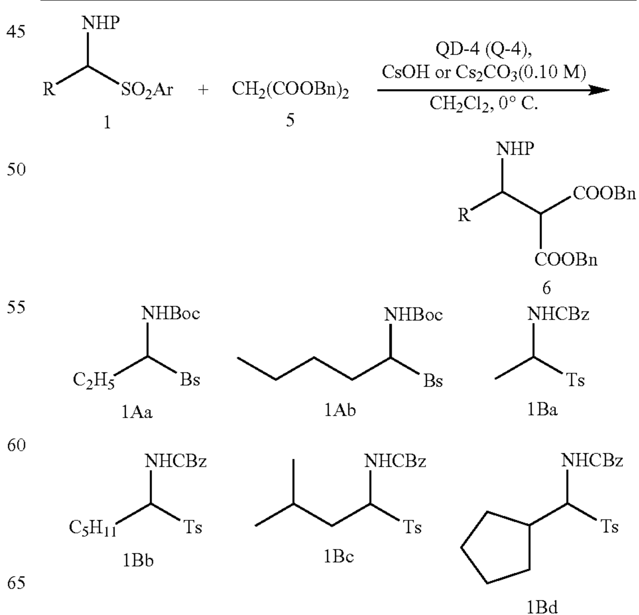
Reactions of Malonate 5 with \alpha -Amido Sulfones Prepared from Aliphatic Aldehydes
