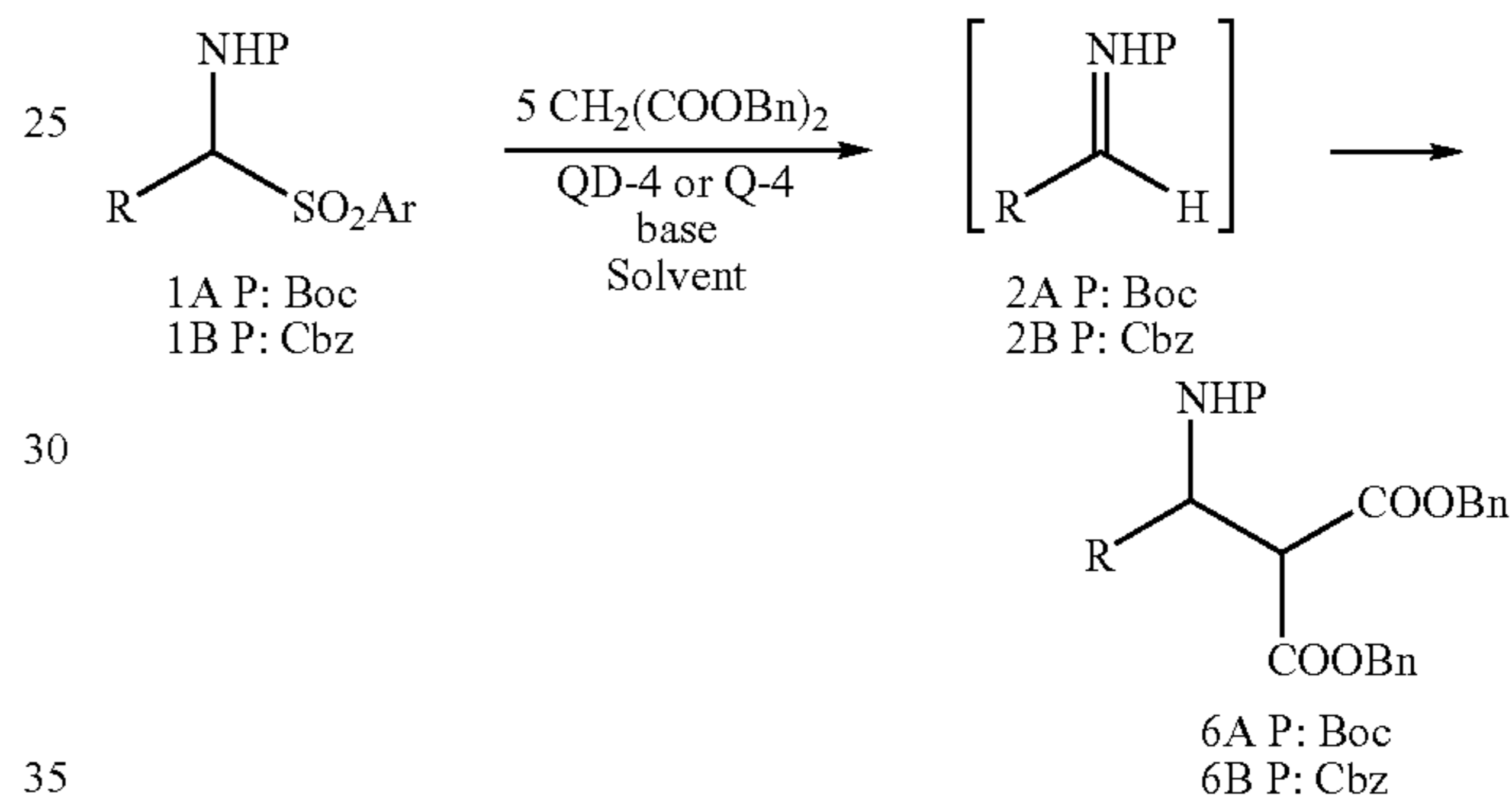
Scheme 2. Mannich reaction of malonate 5 with in situ generated N-carbamate imines 2
