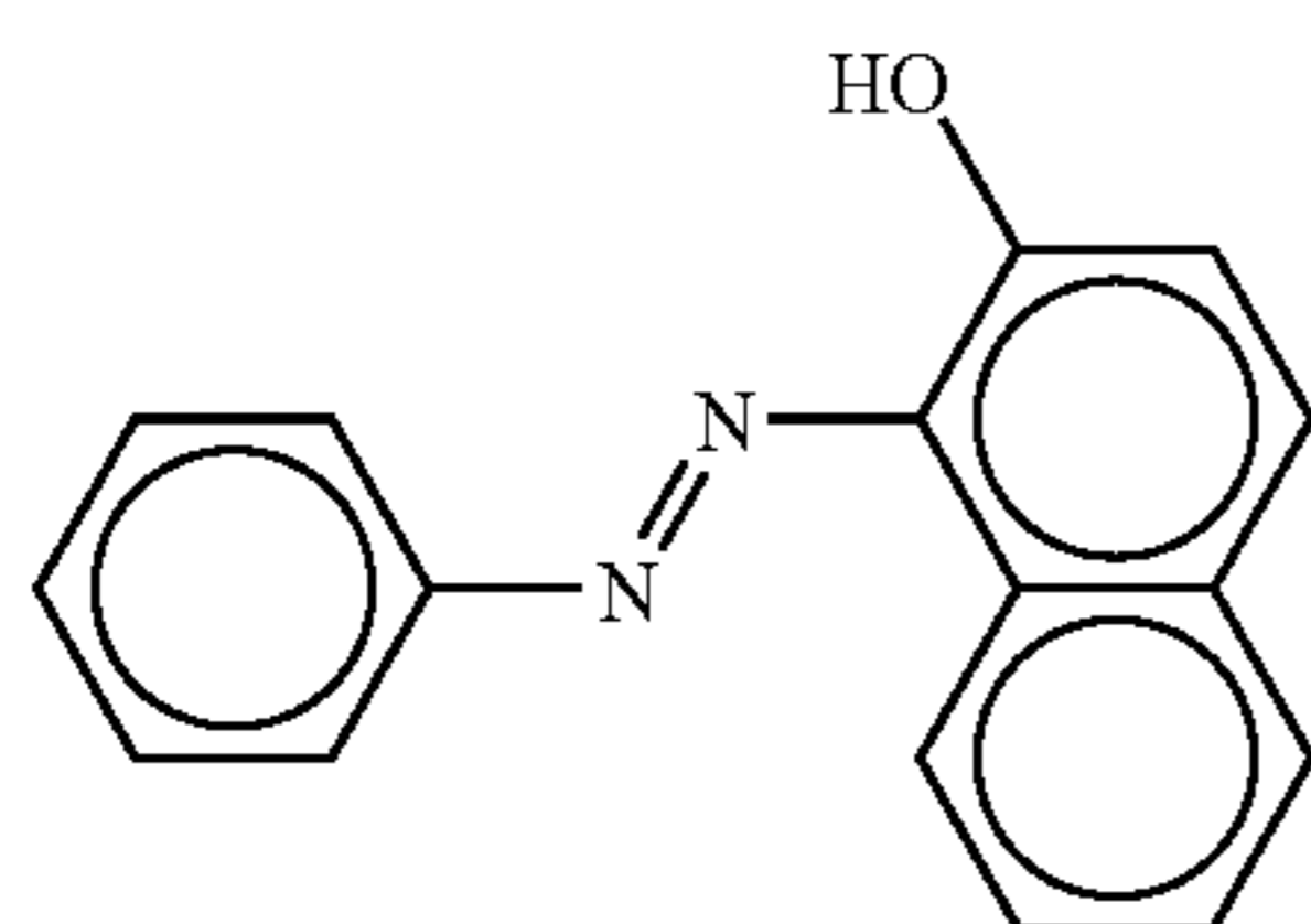
Solvent Yellow 14
