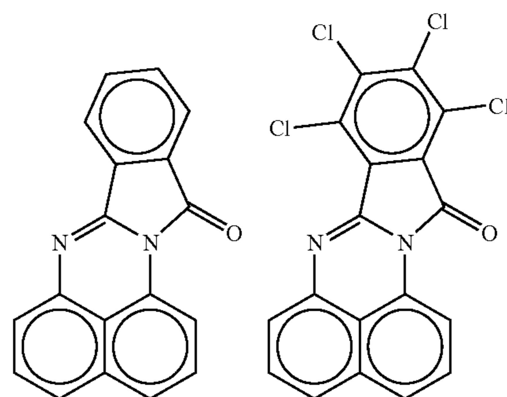
Solvent Orange 60
