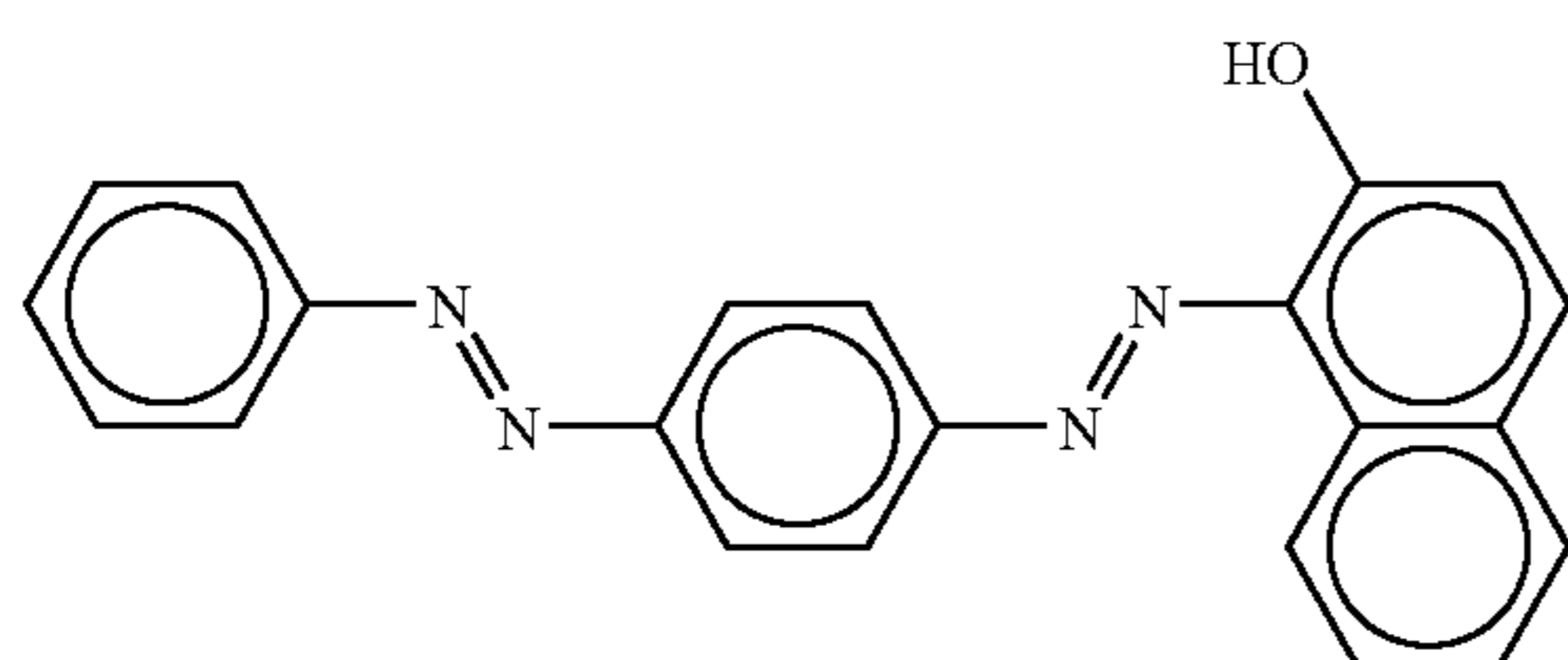
Solvent Red 23
