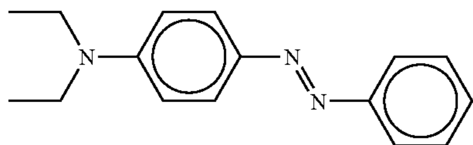
Solvent Yellow 56
