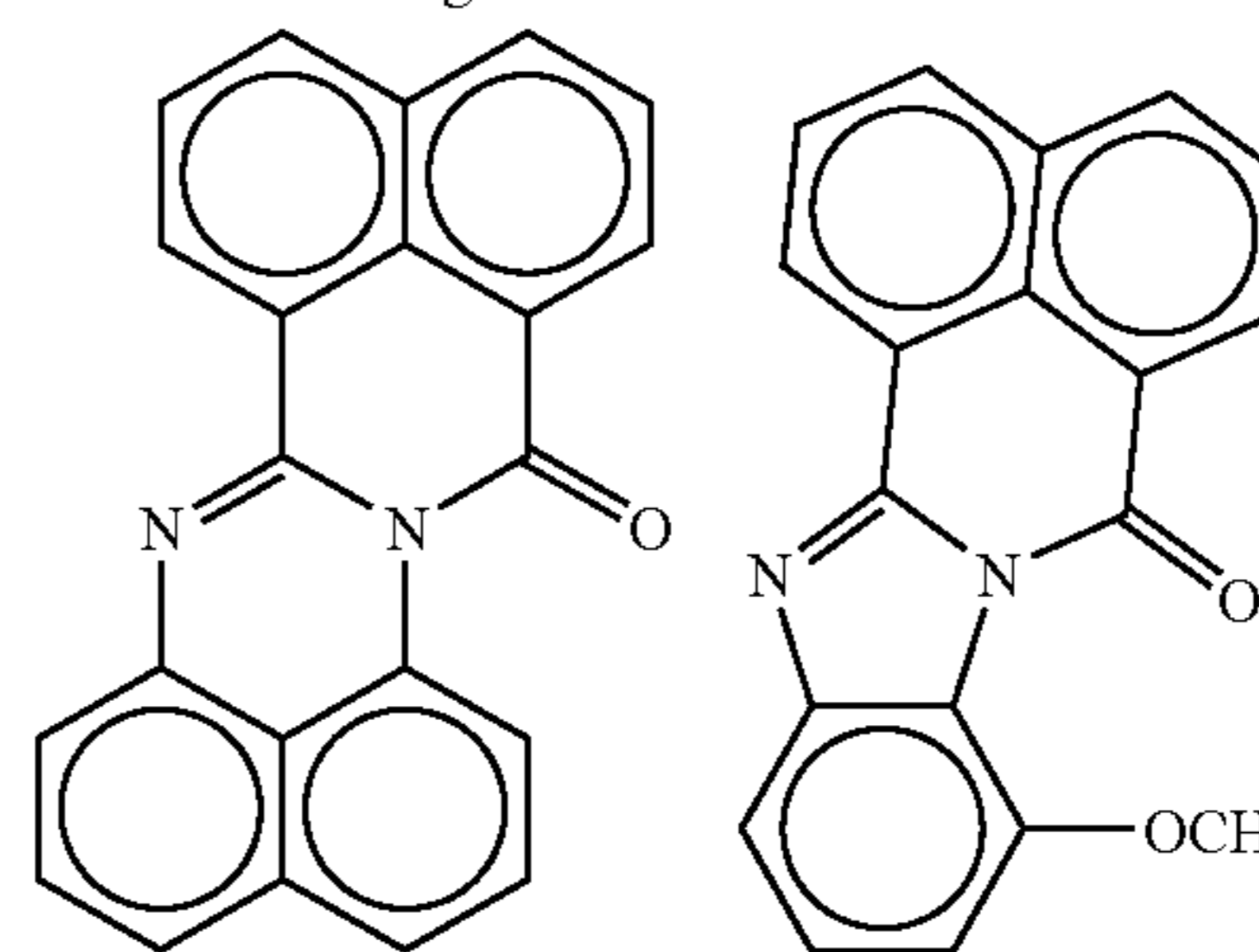
Solvent Red 179
