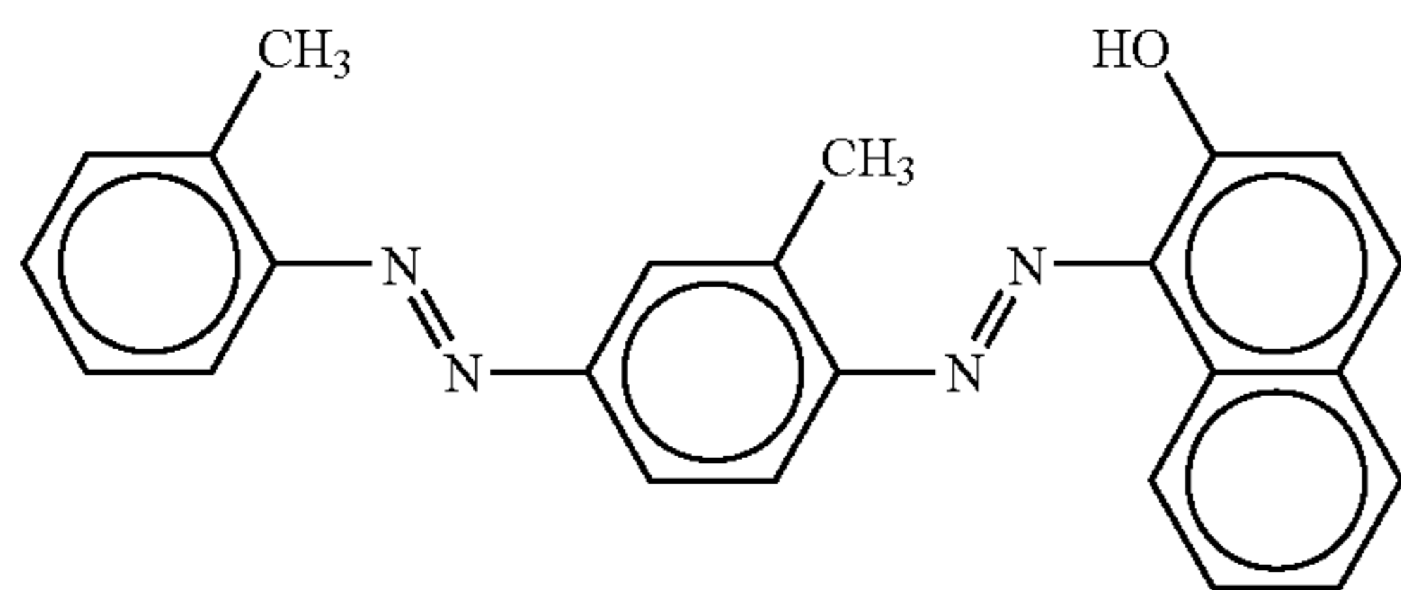
Solvent Red 24
