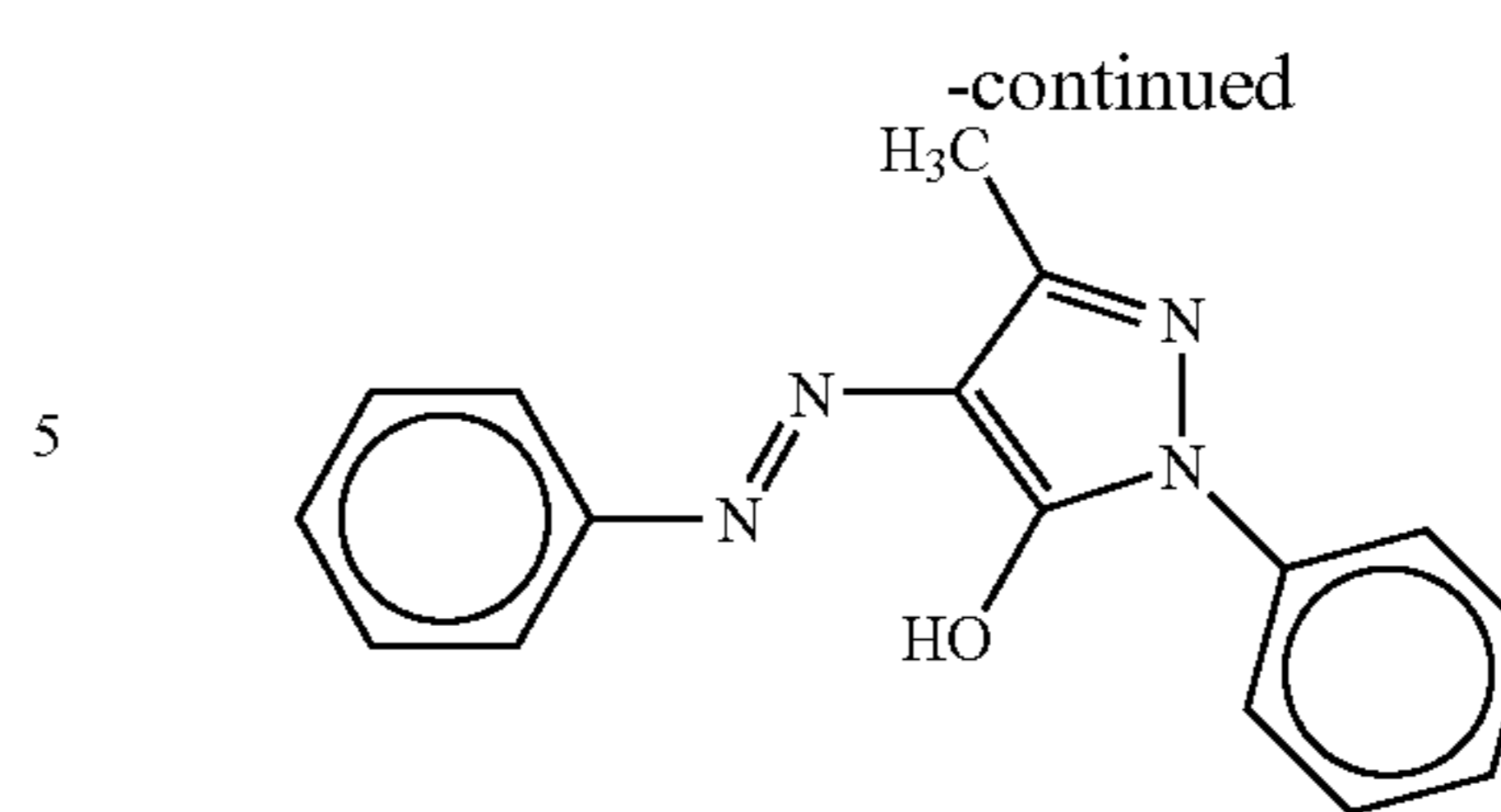
Solvent Yellow 16
