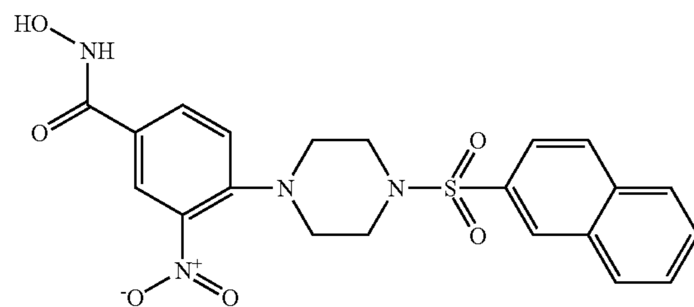
\text{C}_2\text{HF}_3\text{O}_2 (1:1), Co. No. 21; Ex. [B1]; ms. 457
