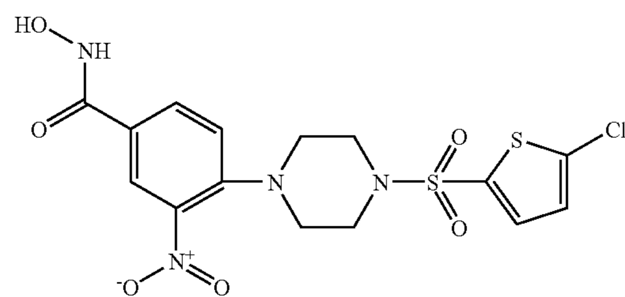
\text{C}_2\text{HF}_3\text{O}_2 (1:1), Co. No. 20; Ex. [B1]; ms. 447
