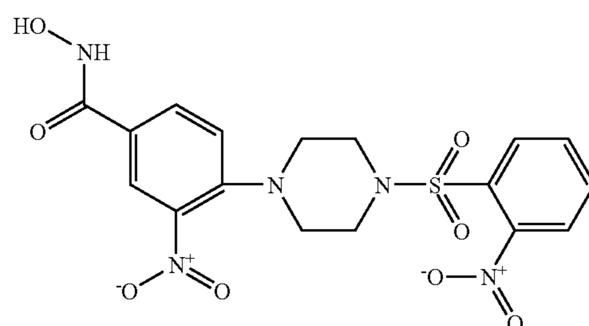
\text{C}_2\text{HF}_3\text{O}_2 (1:1), Co. No. 23; Ex. [B1]; ms. 452
