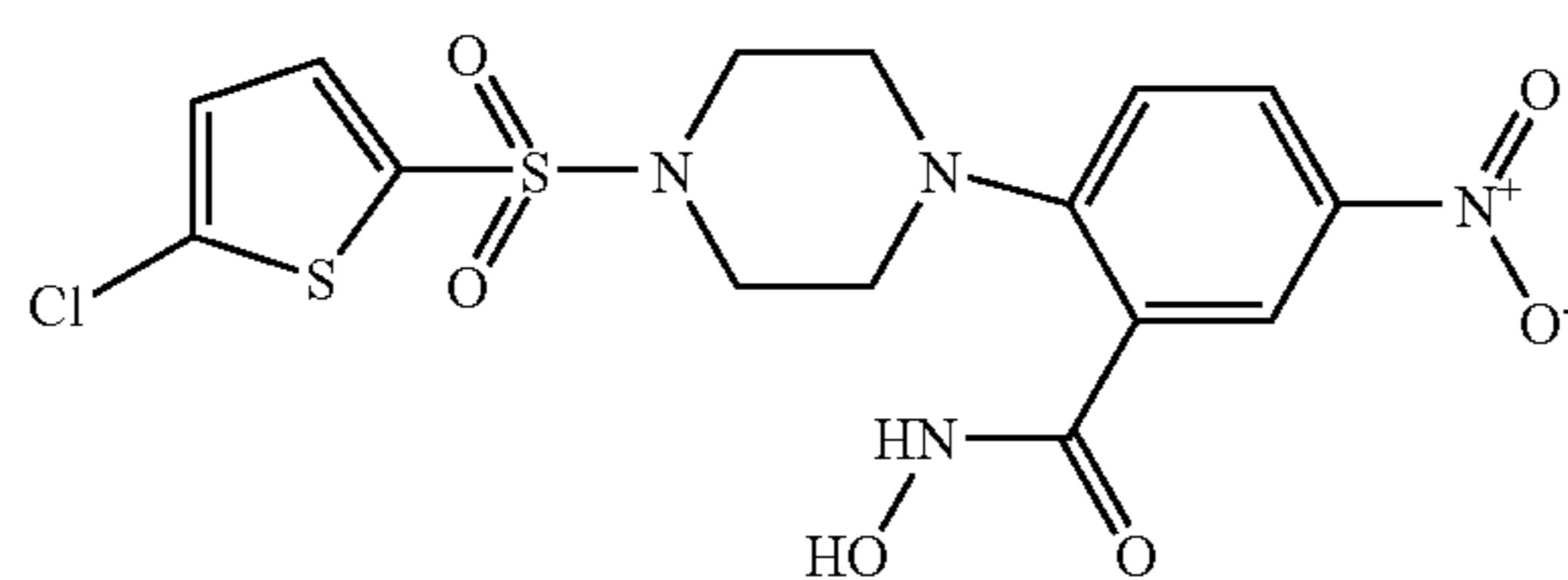
\text{C}_2\text{HF}_3\text{O}_2 (1:1), Co. No. 22; Ex. [B1]; ms. 447
