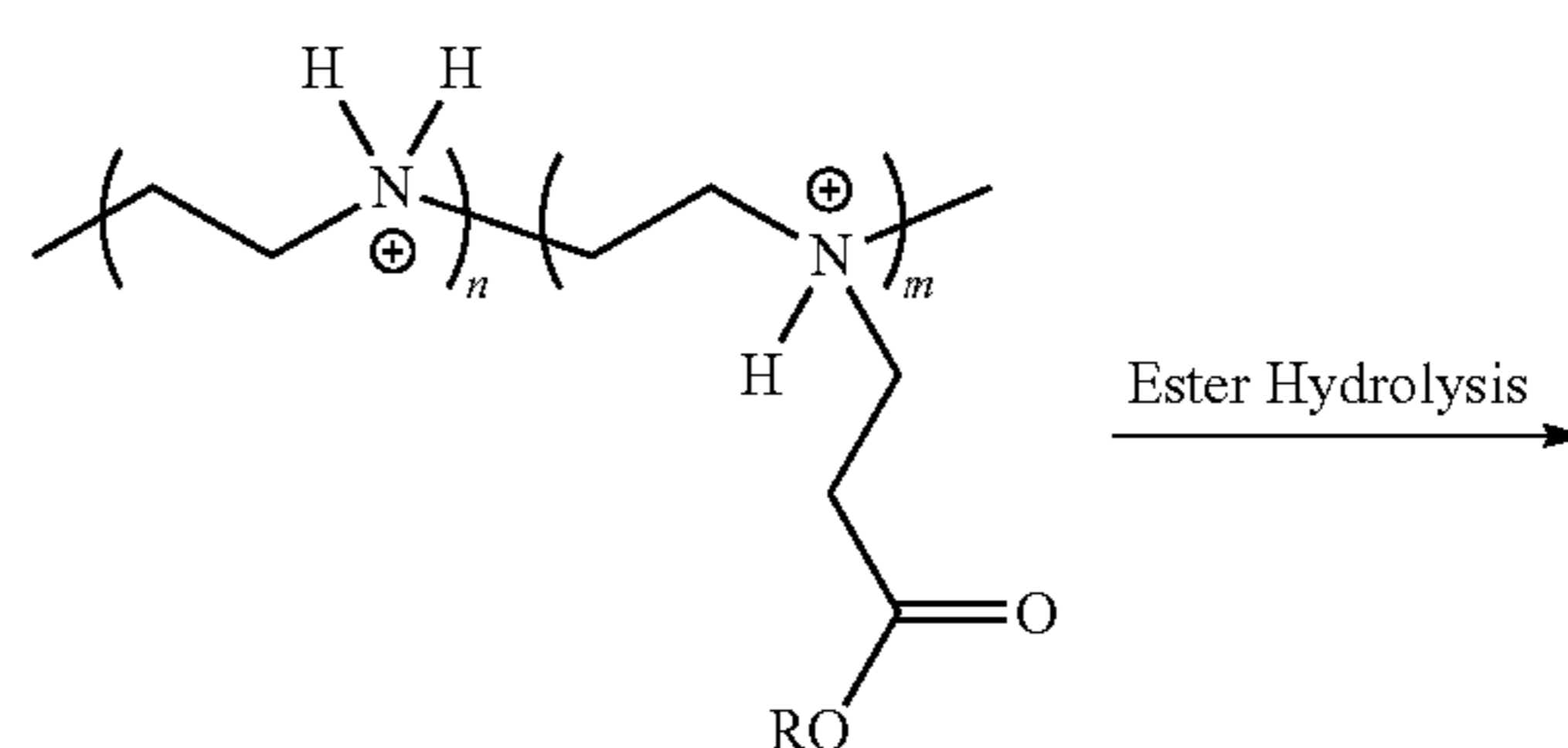
Polymer 1
