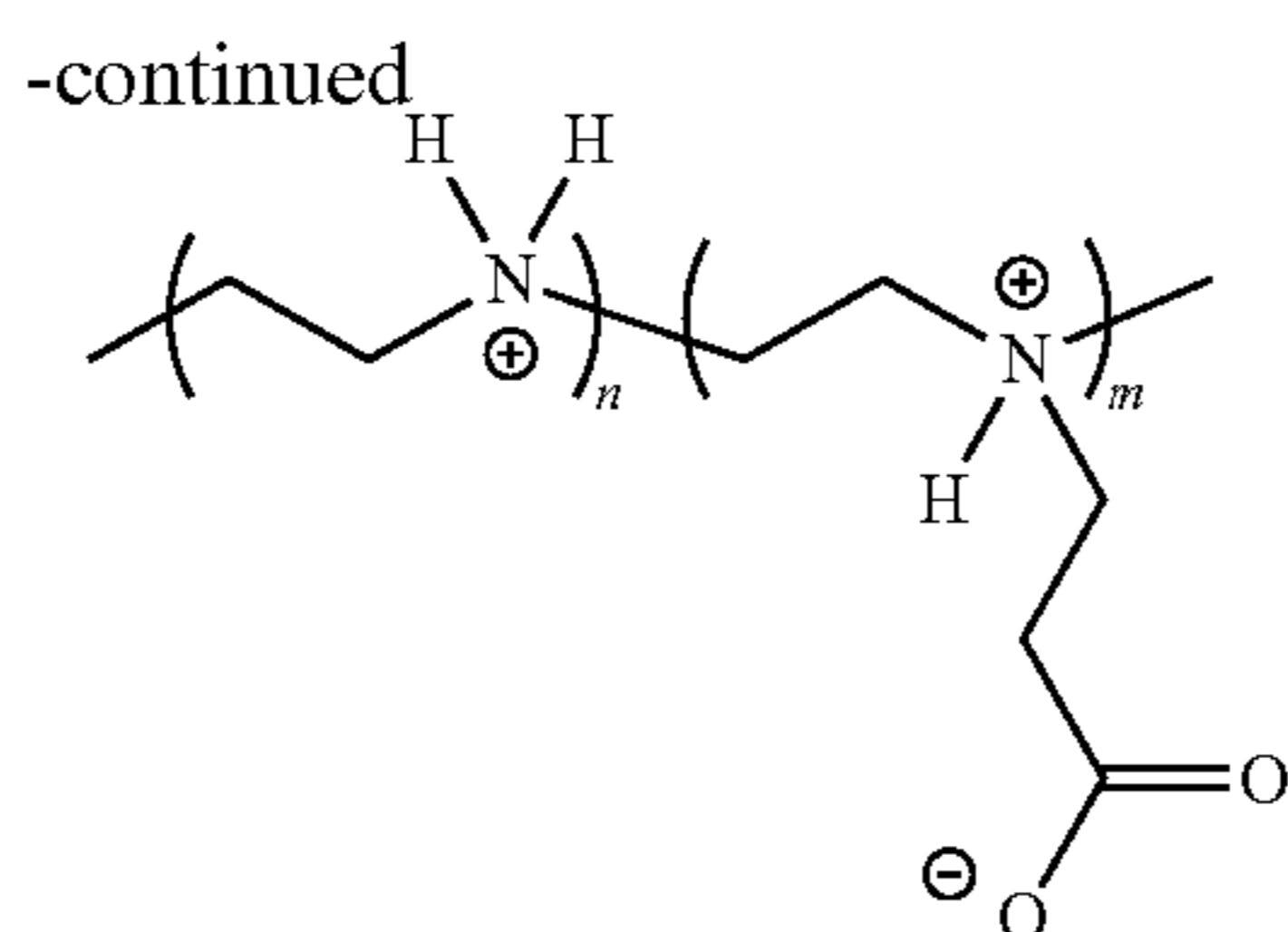
Polymer 2
