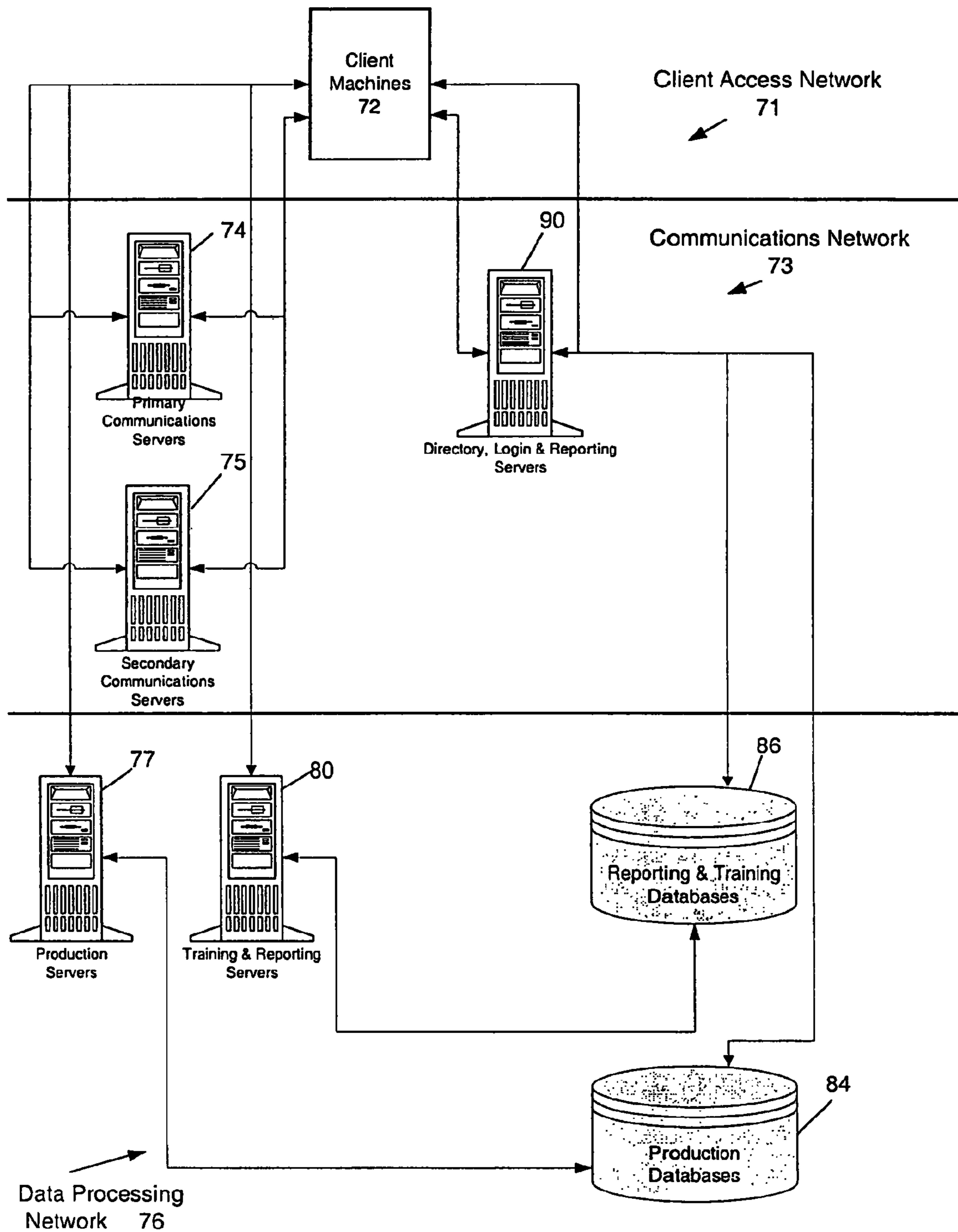
FIG. 4 AUCTION NETWORK 70
