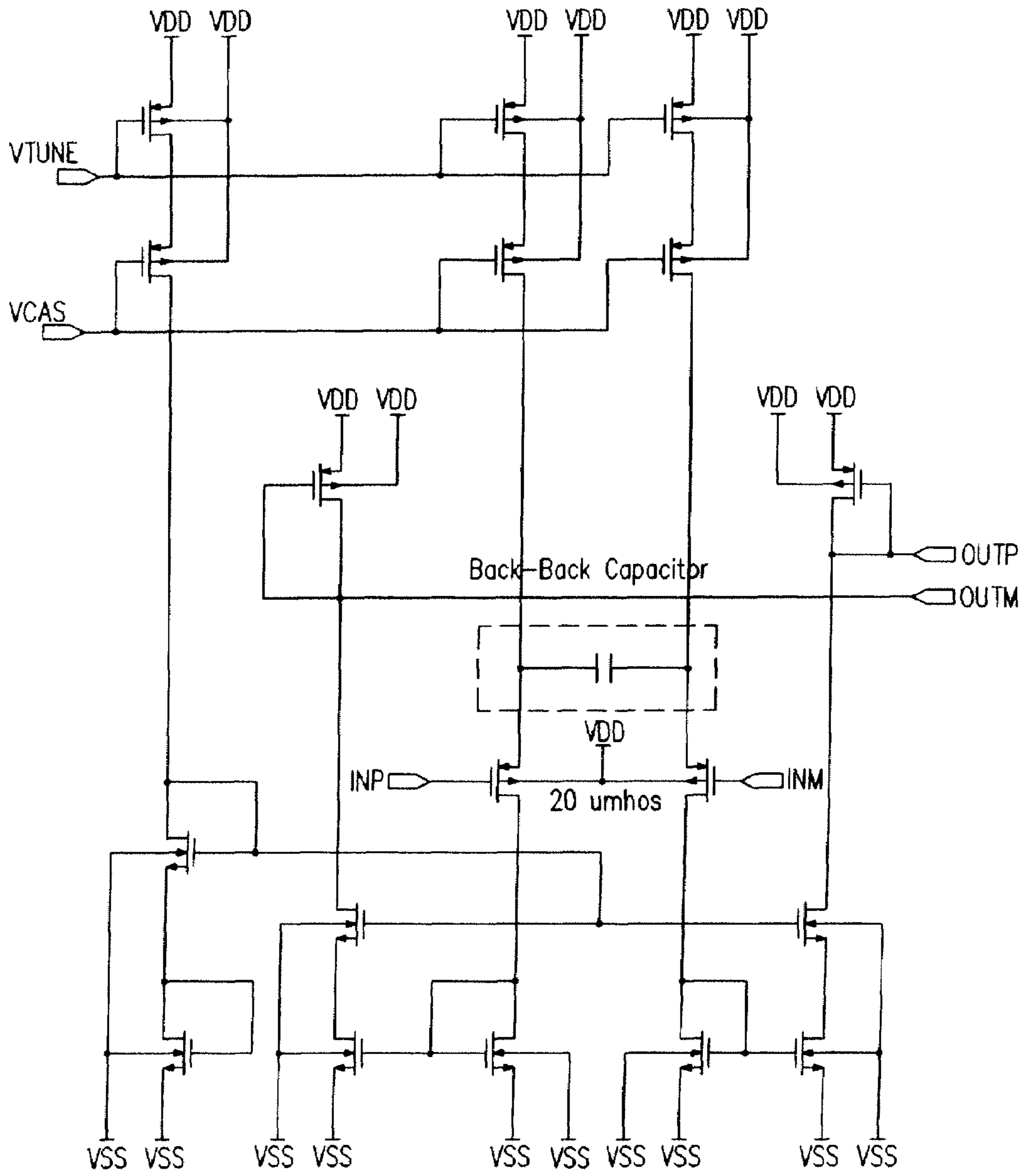
Differential AC-coupled Voltage Amplifier
