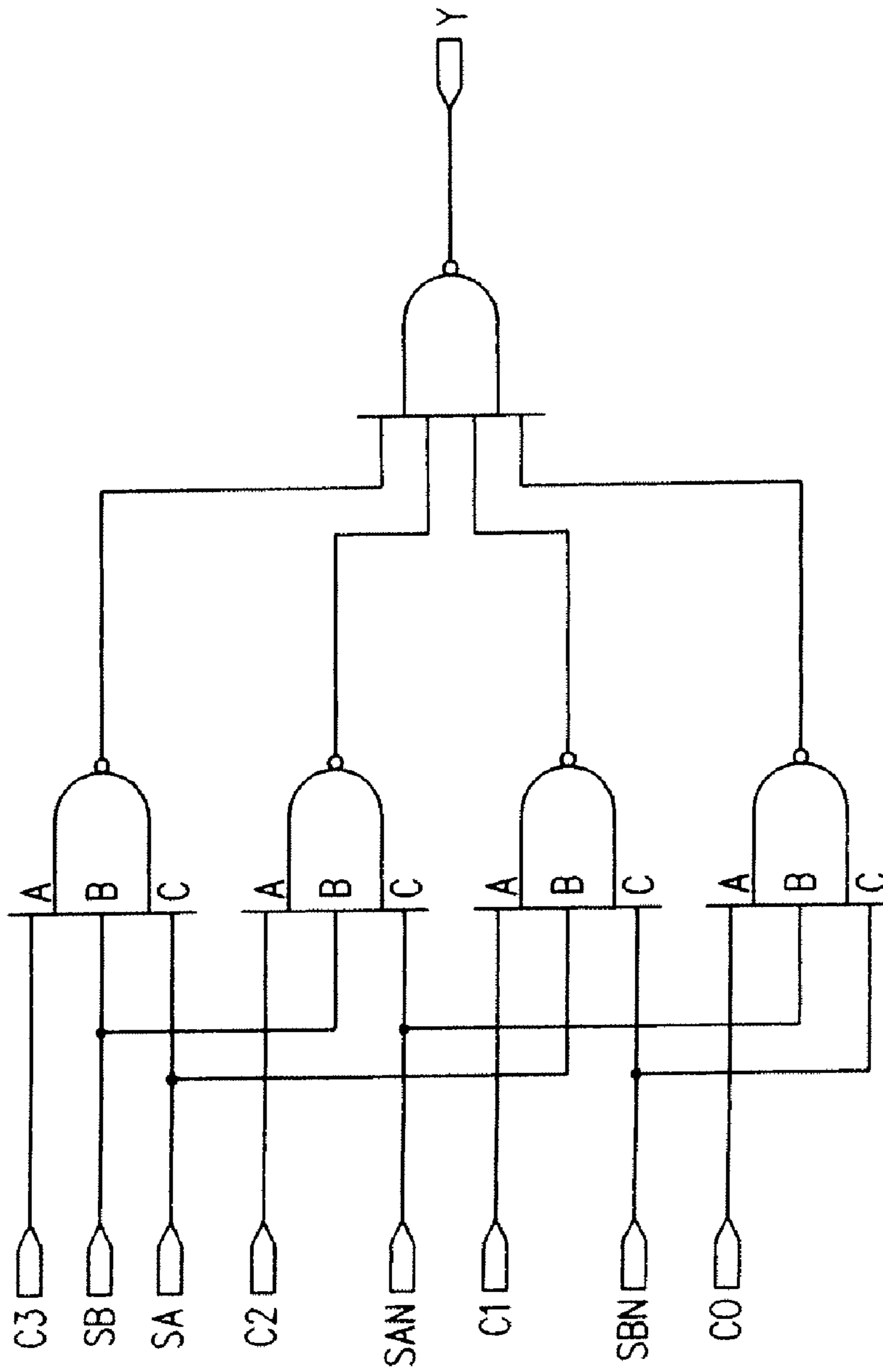
4:1 SELECTOR
