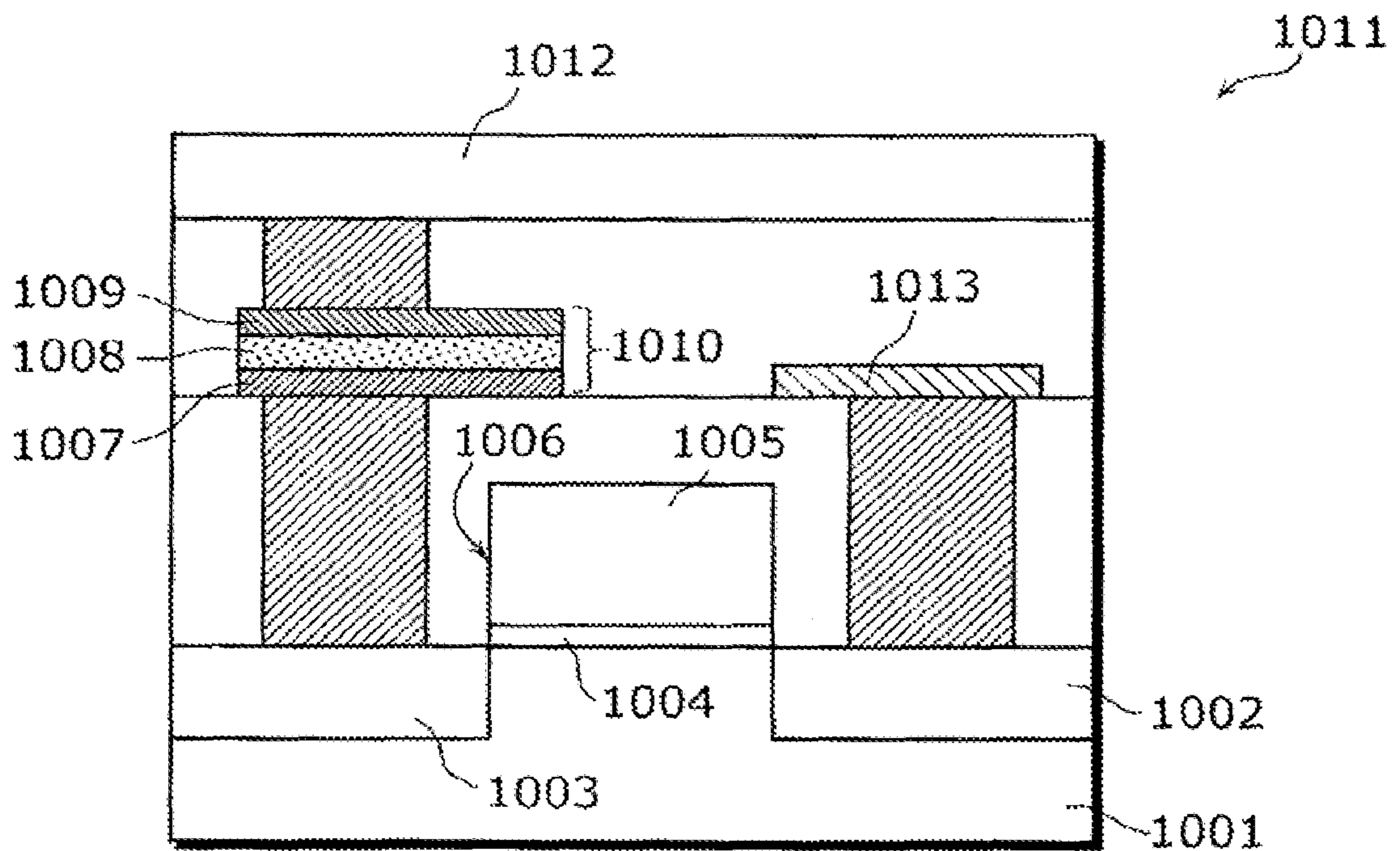
Fig. 28 - PRIOR ART
