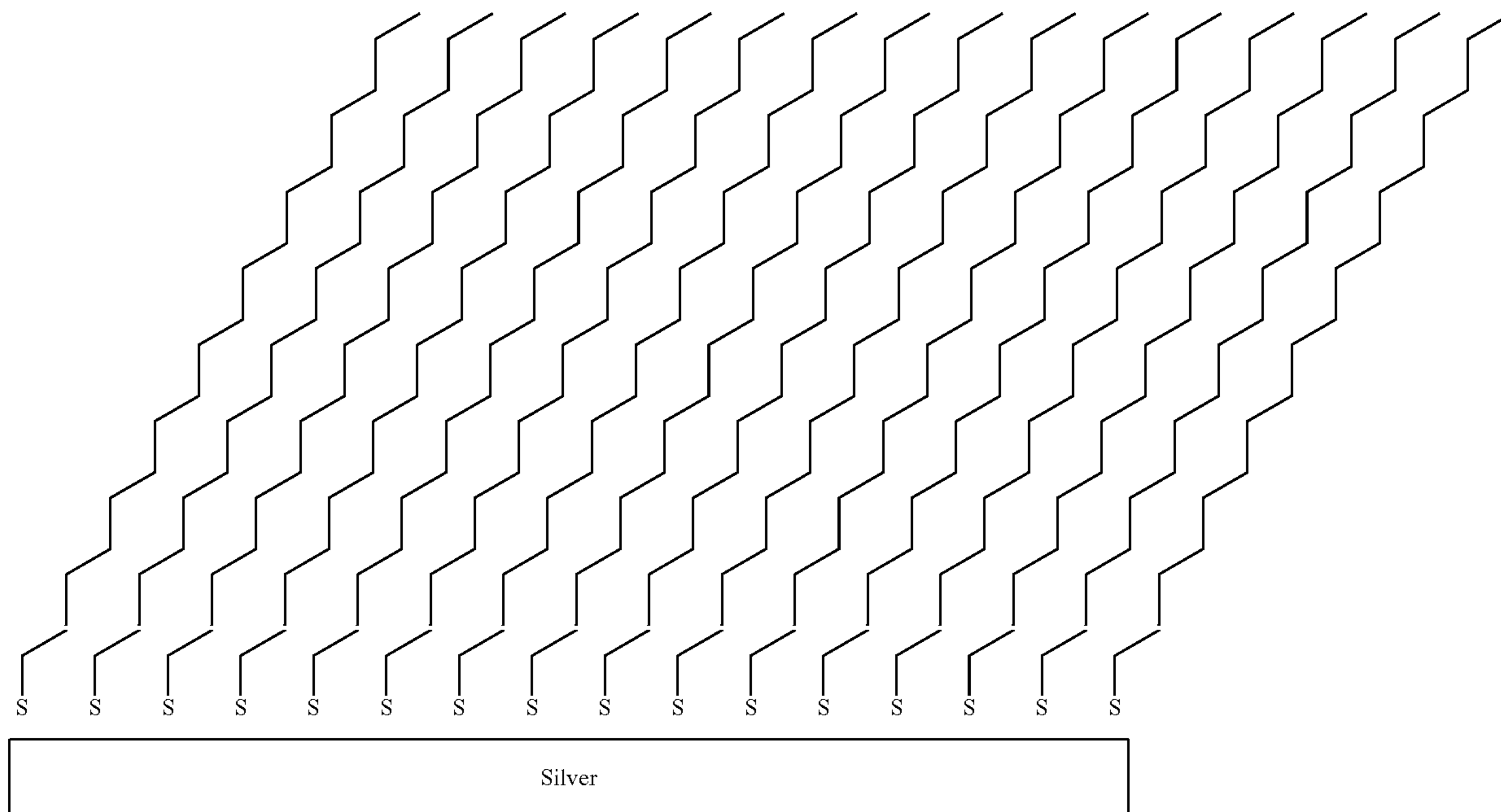
SCHEME 2
