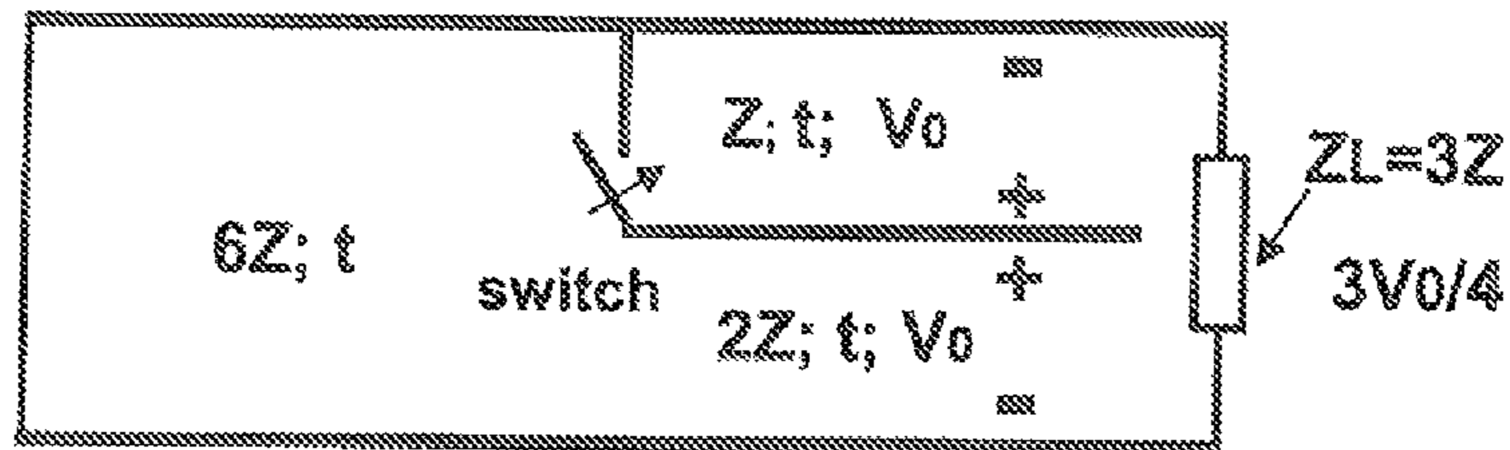
FIGURE 2 (PRIOR ART)
