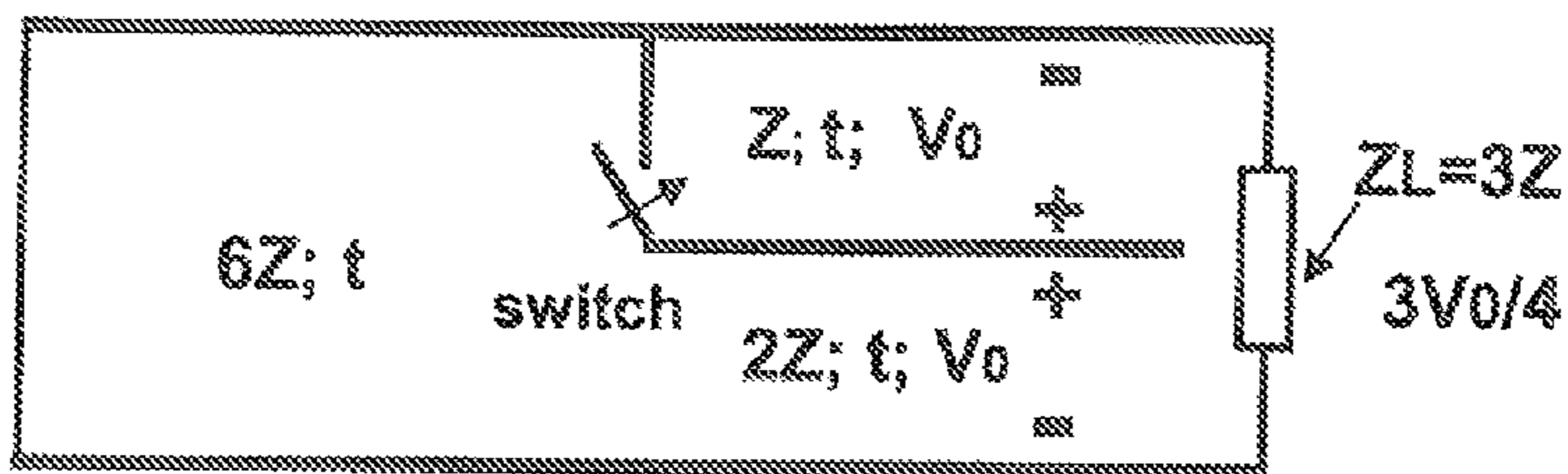
FIGURE 2 (PRIOR ART)
