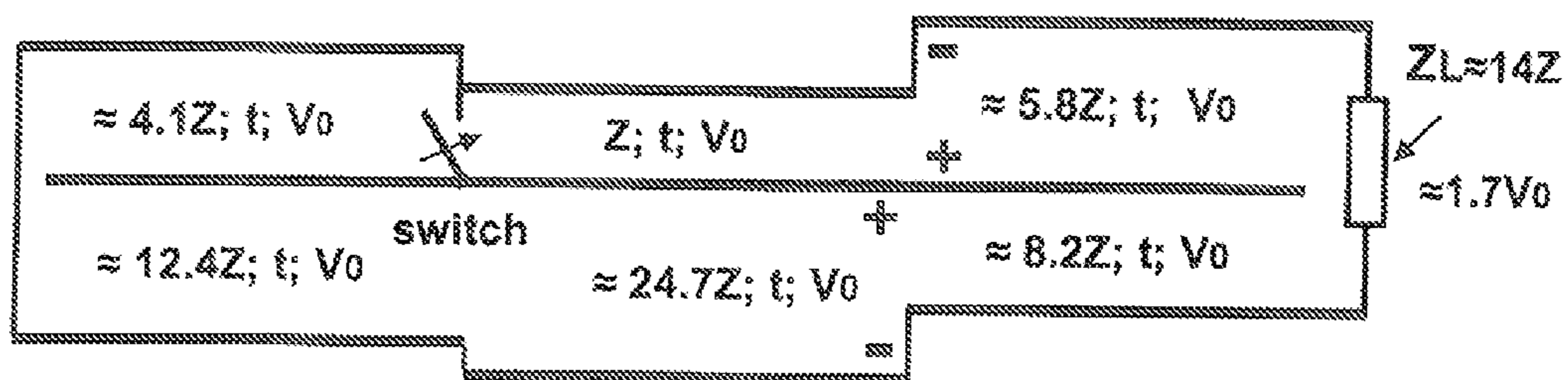
FIGURE 3 (PRIOR ART)
