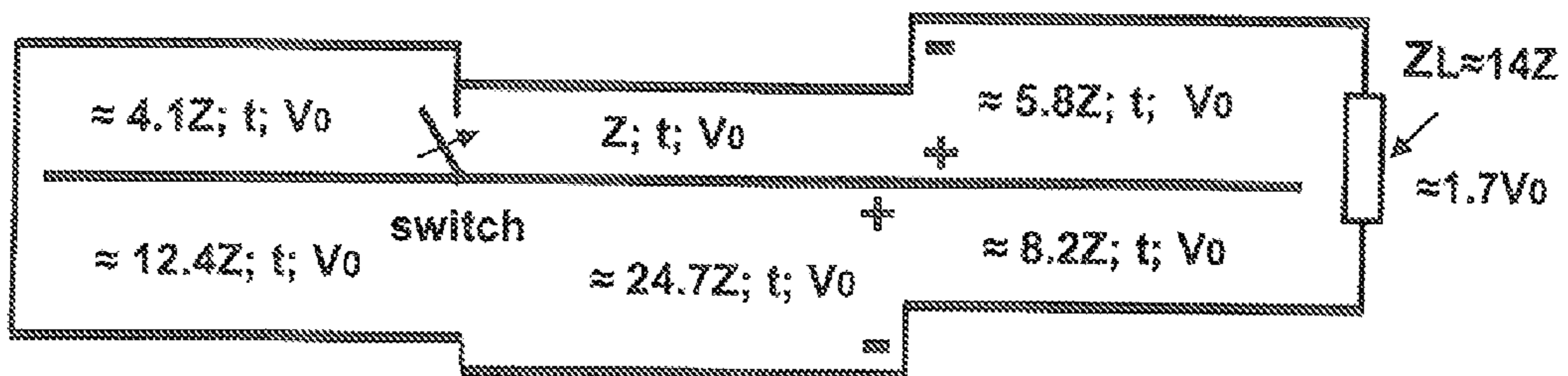
FIGURE 3 (PRIOR ART)
