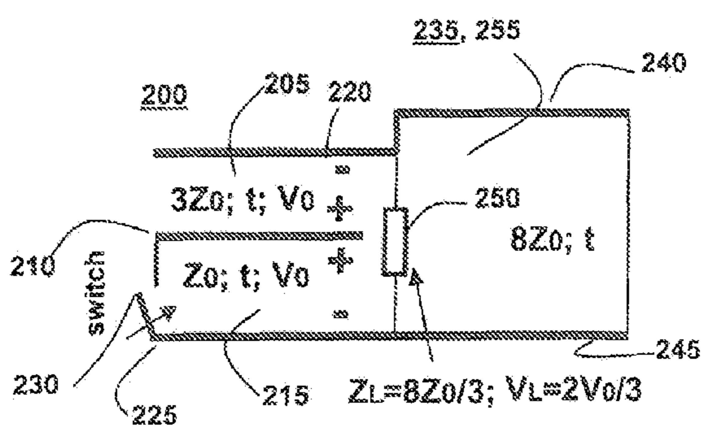
FIGURE 5A
