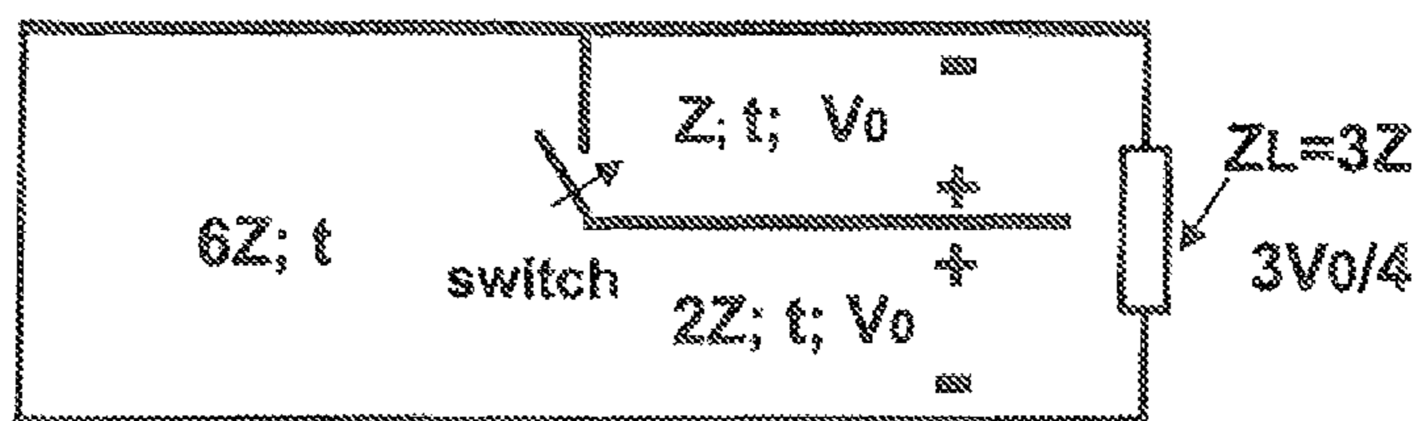
FIGURE 2 (PRIOR ART)
