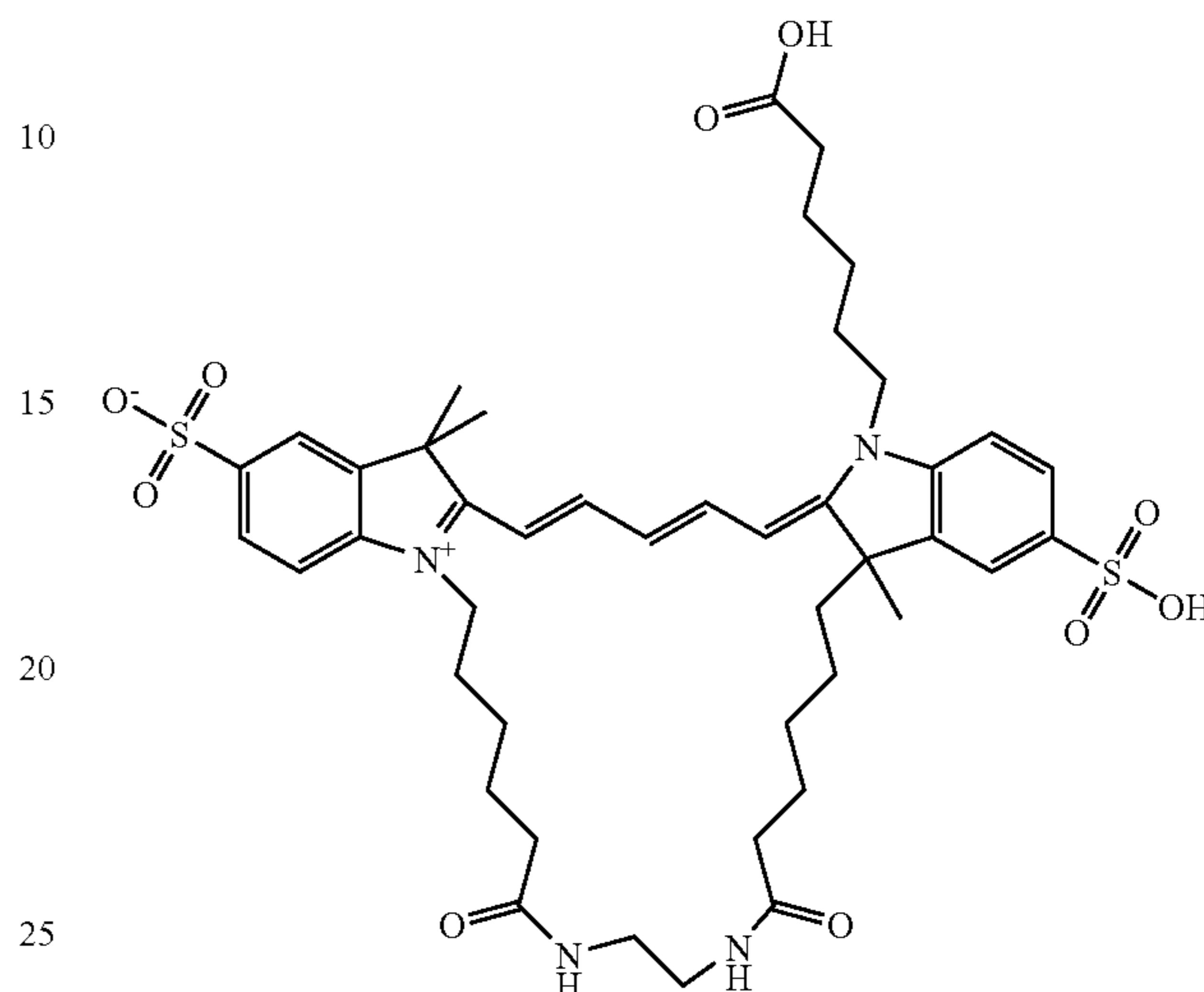
Compound 24
