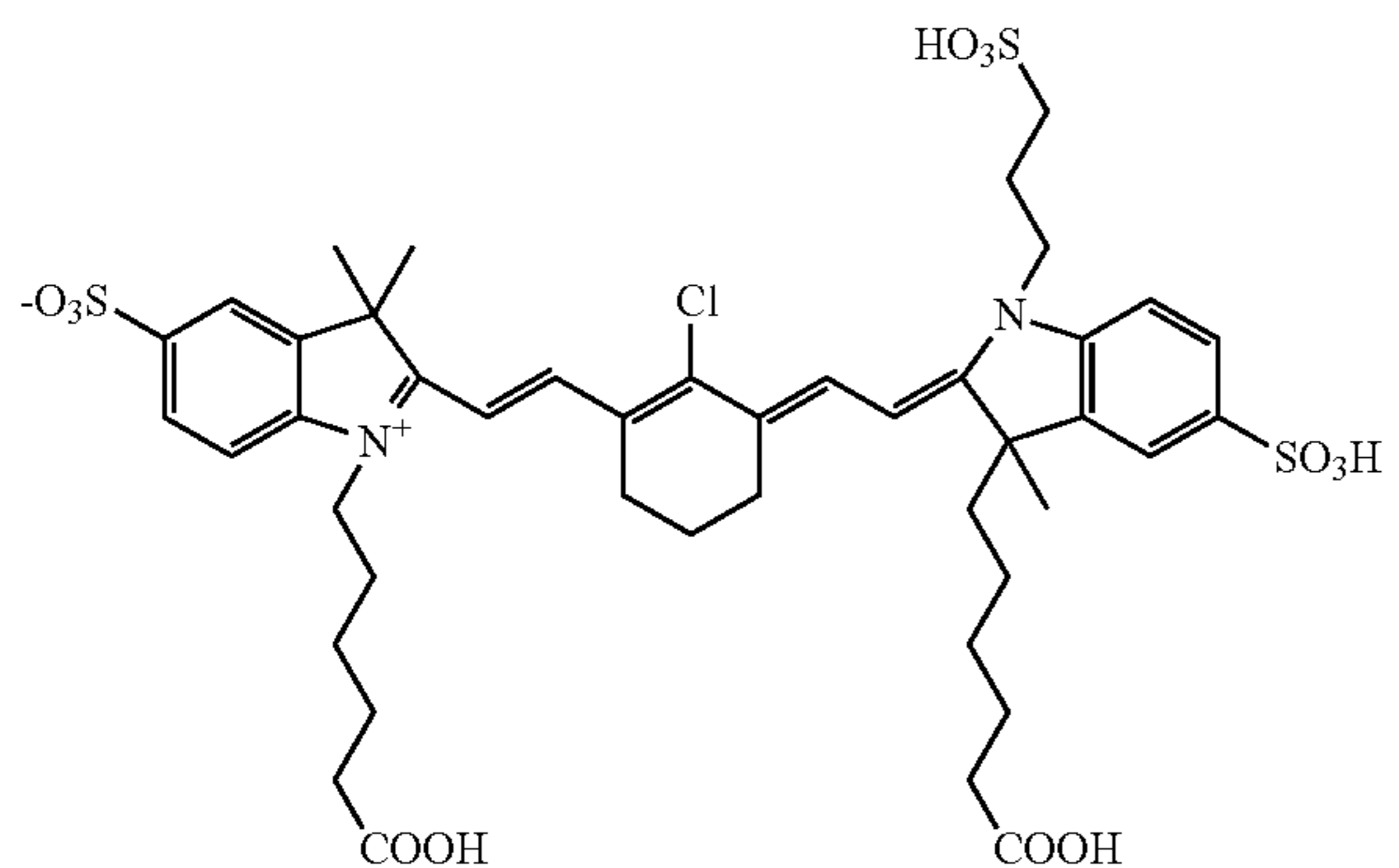
Compound 32
