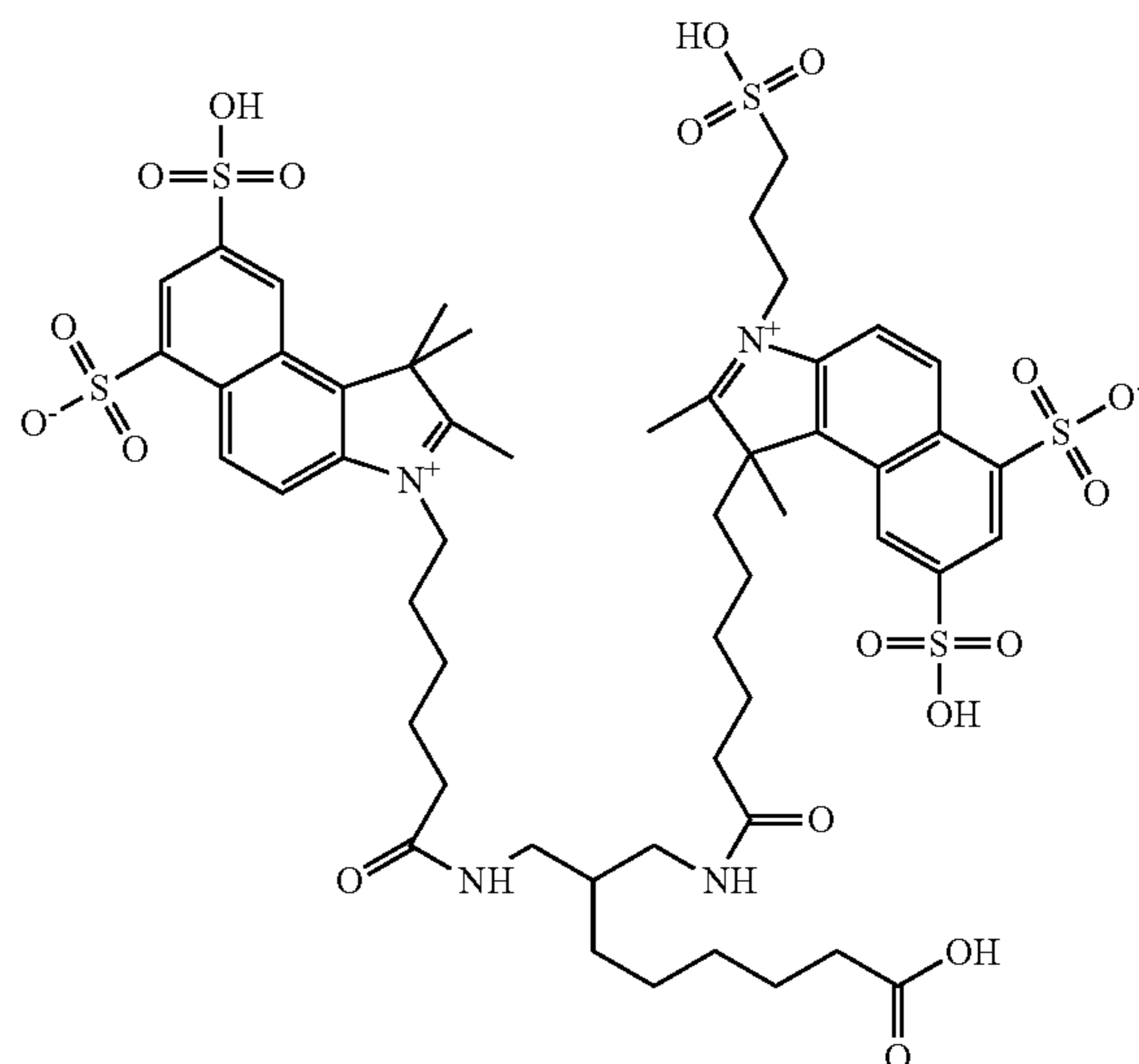
Compound 47
