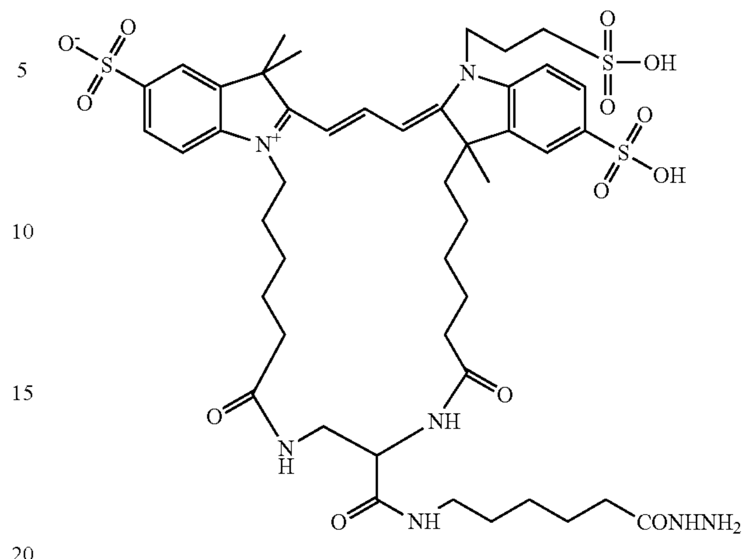
Compound 35
