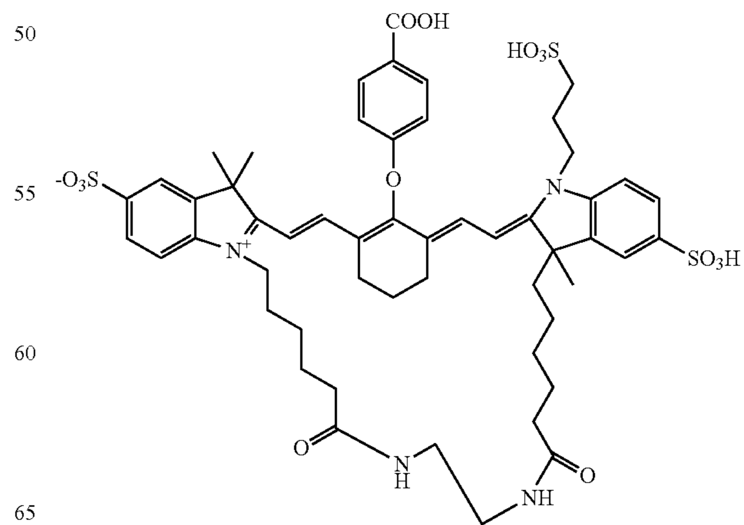
Compound 33
