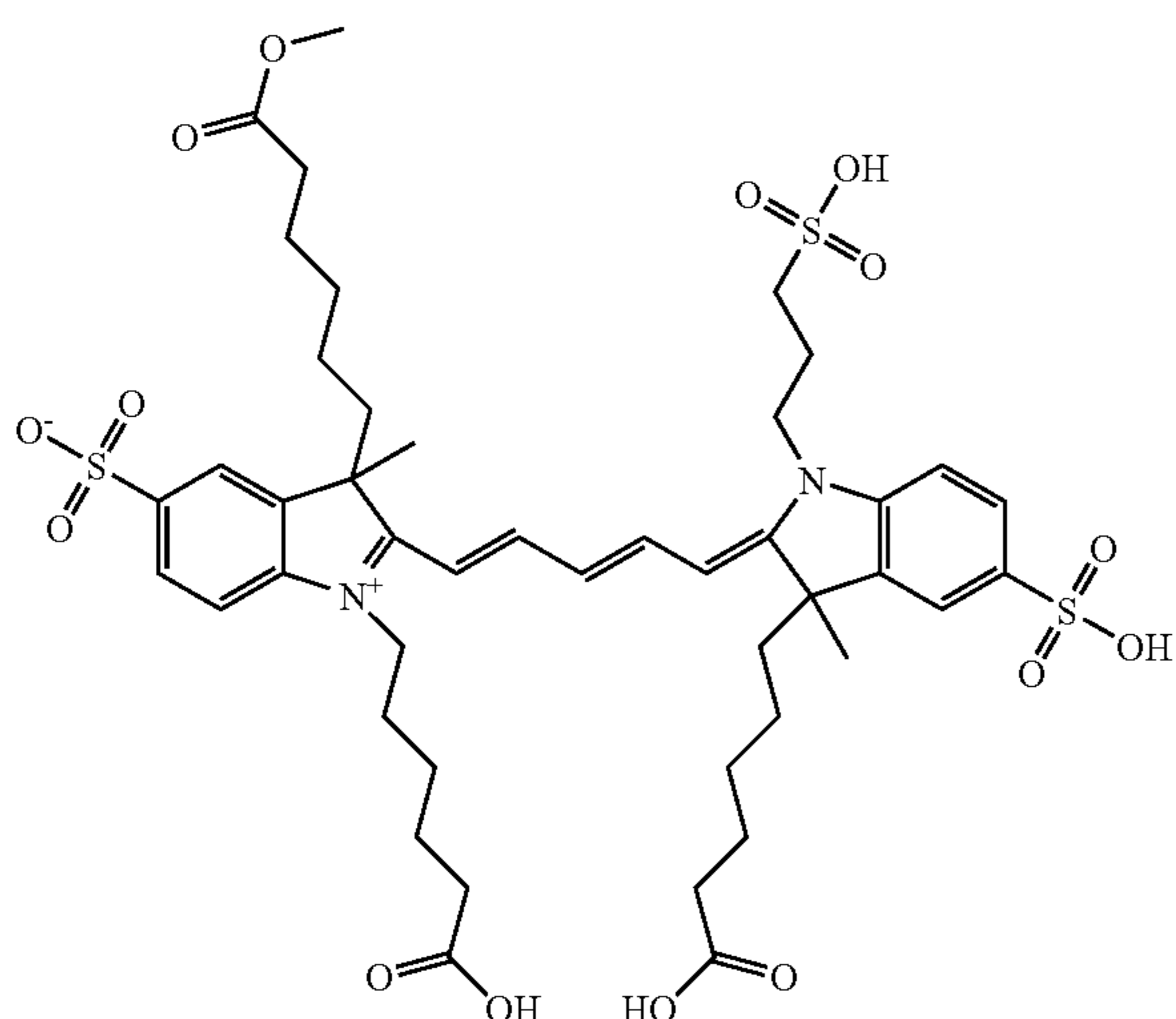
Compound 15
