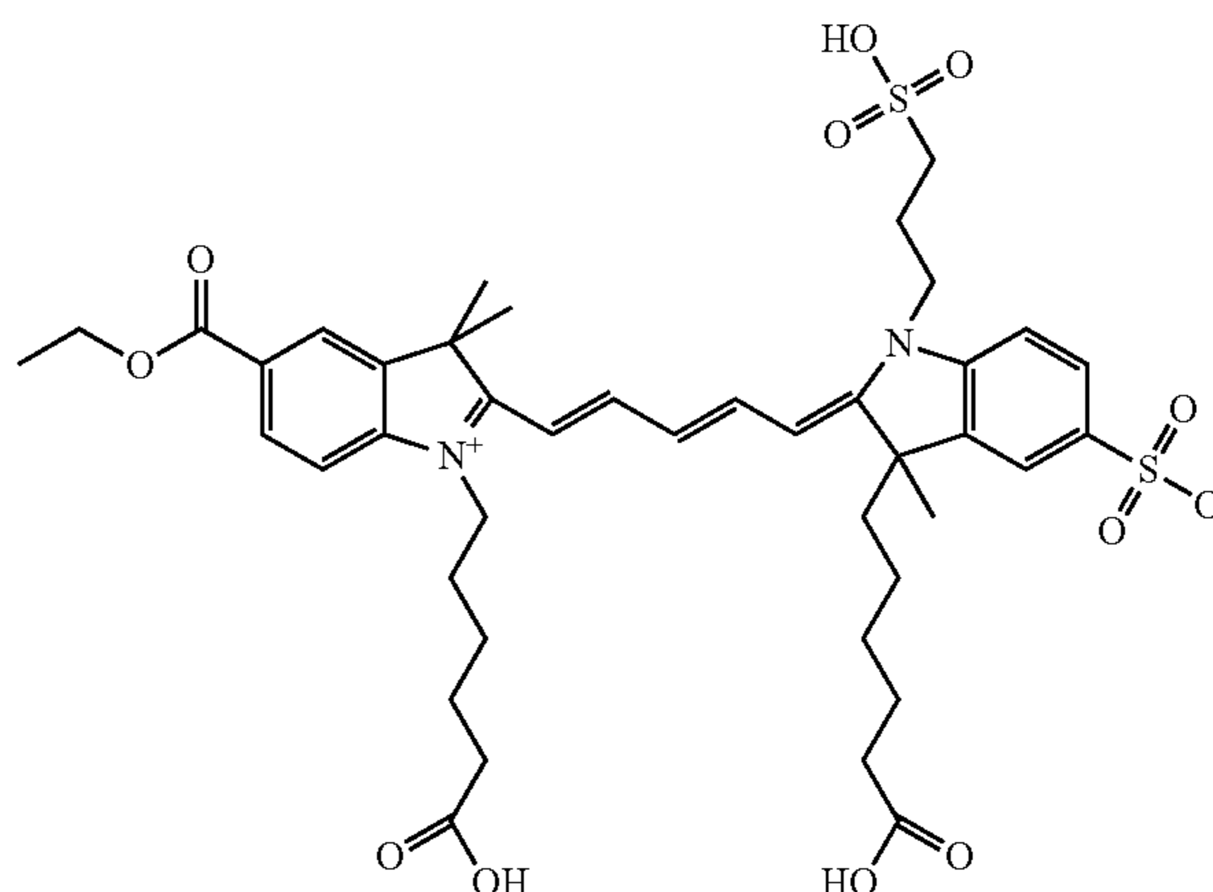
Compound 25
