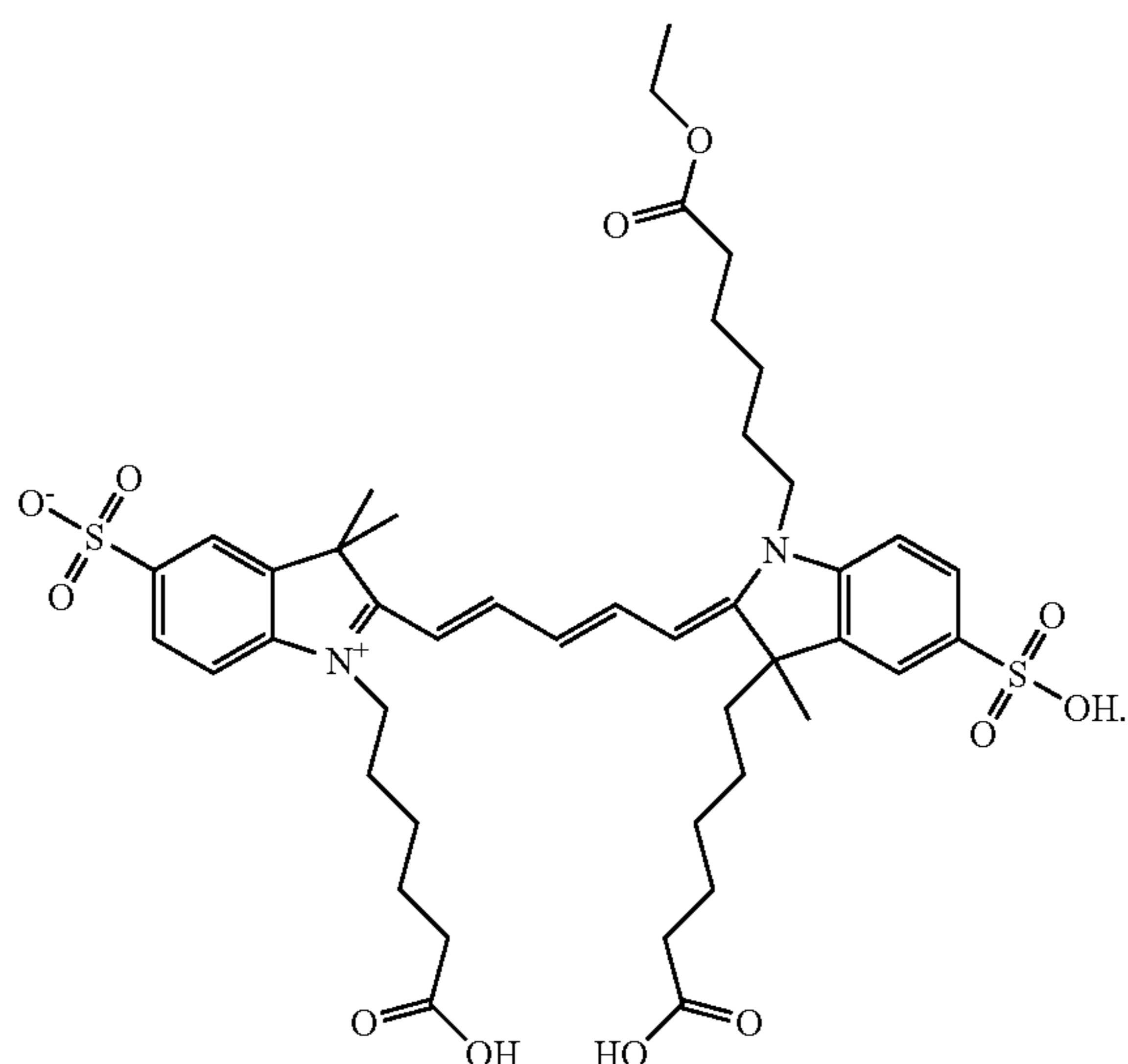
Compound 23
